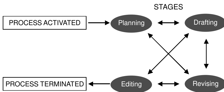
Figure 2.2 Writing Process
