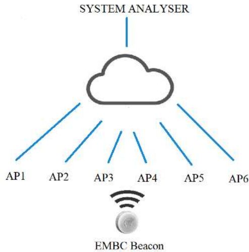
Figure 4.1: System structure
