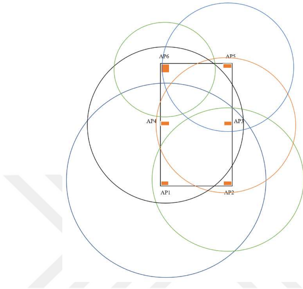
Figure 4.20: Circles of Test.3
