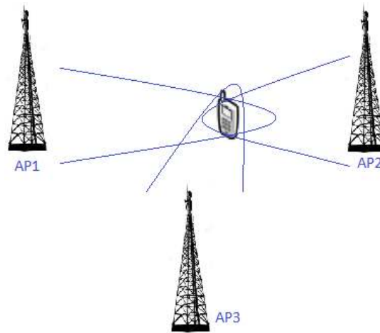
Figure 3.9: TDOA
