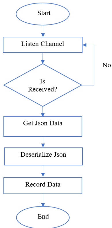
Figure 4.7: Service flowchart
