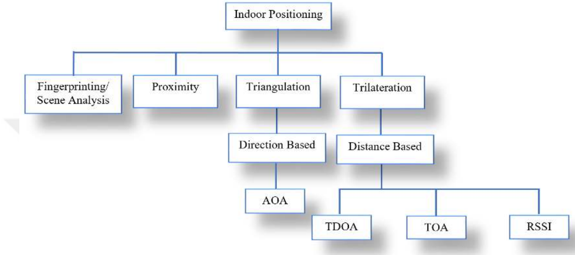
Figure 3.5: Positioning techniques
