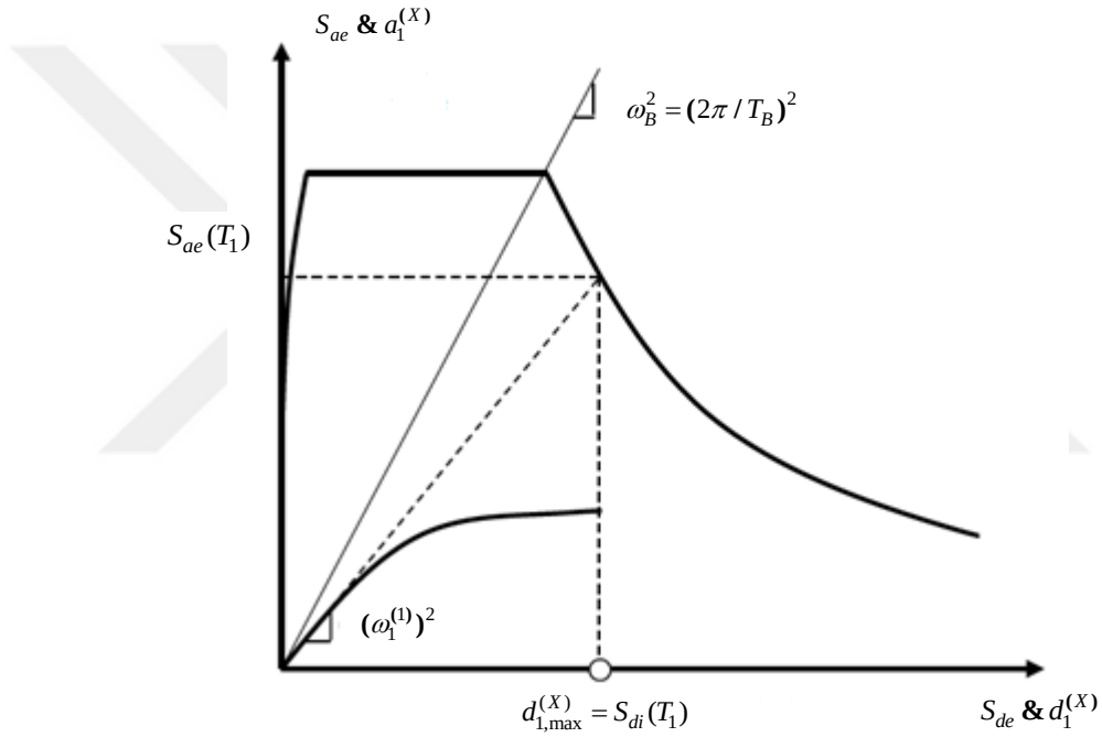
Figure 4.10. Illustration of the modal capacity curve and demand diagram in ADRS format
