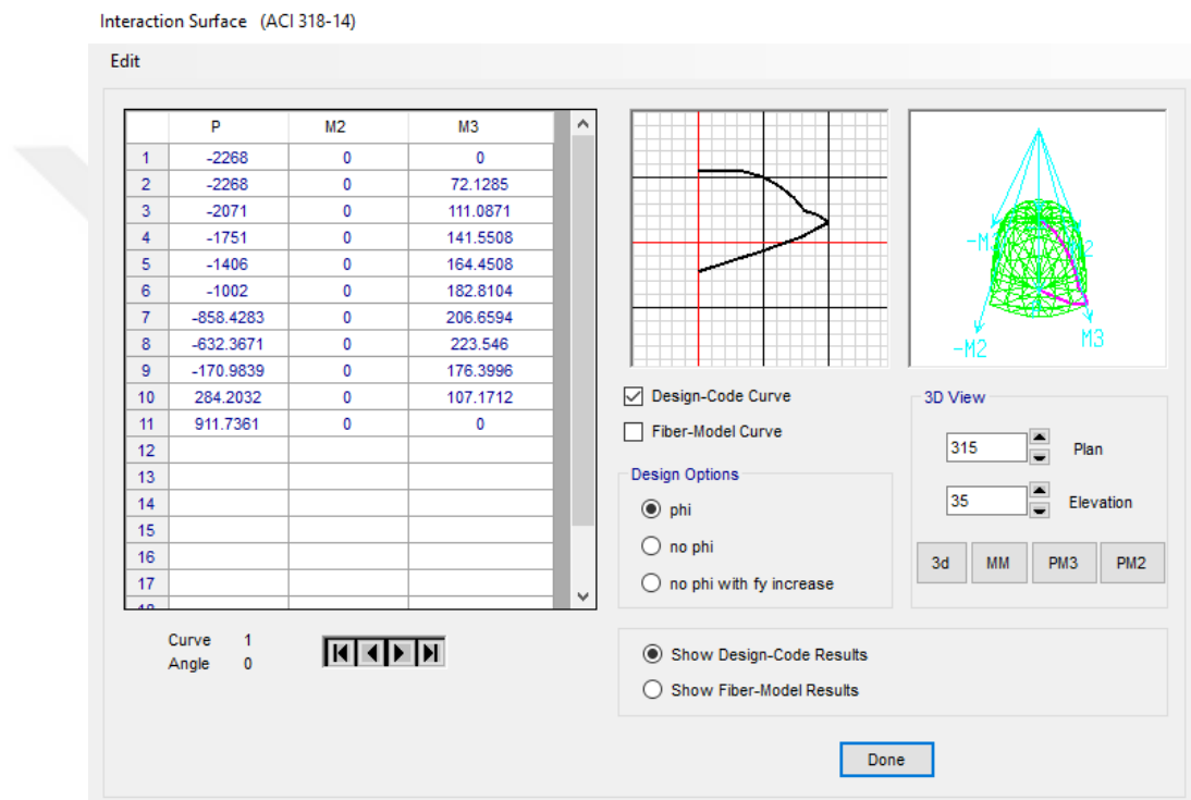
Figure 5.8. Normal force moment interaction surface (P-M3) for the columns
