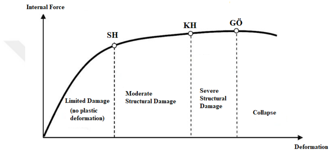
Figure 2.1. Structural element damage levels and regions [24]
