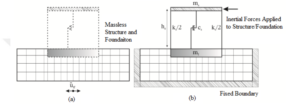
Figure 3.4. Soil structure interaction analysis using substructure approach: (a) kinematic; (b) inertial interaction [2]
