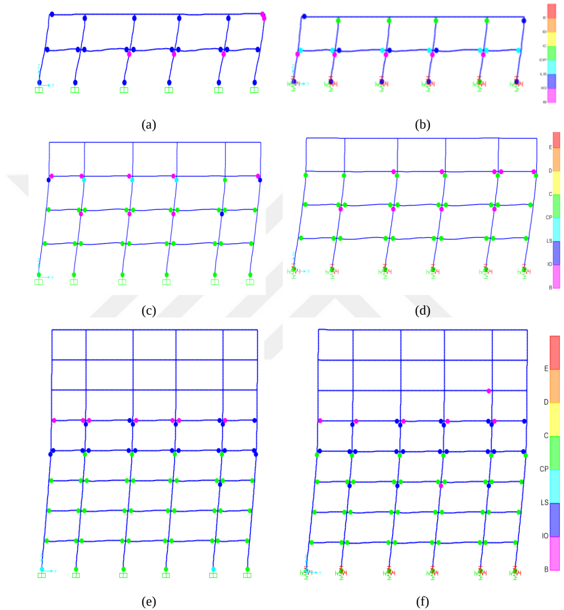
Figure 5.35. Comparison of plastic hinge formations for 2, 4 and 8 story models in the y-direction; (a), (c), (e) shows flexible base and (b), (d), (f) represent fixed base conditions
