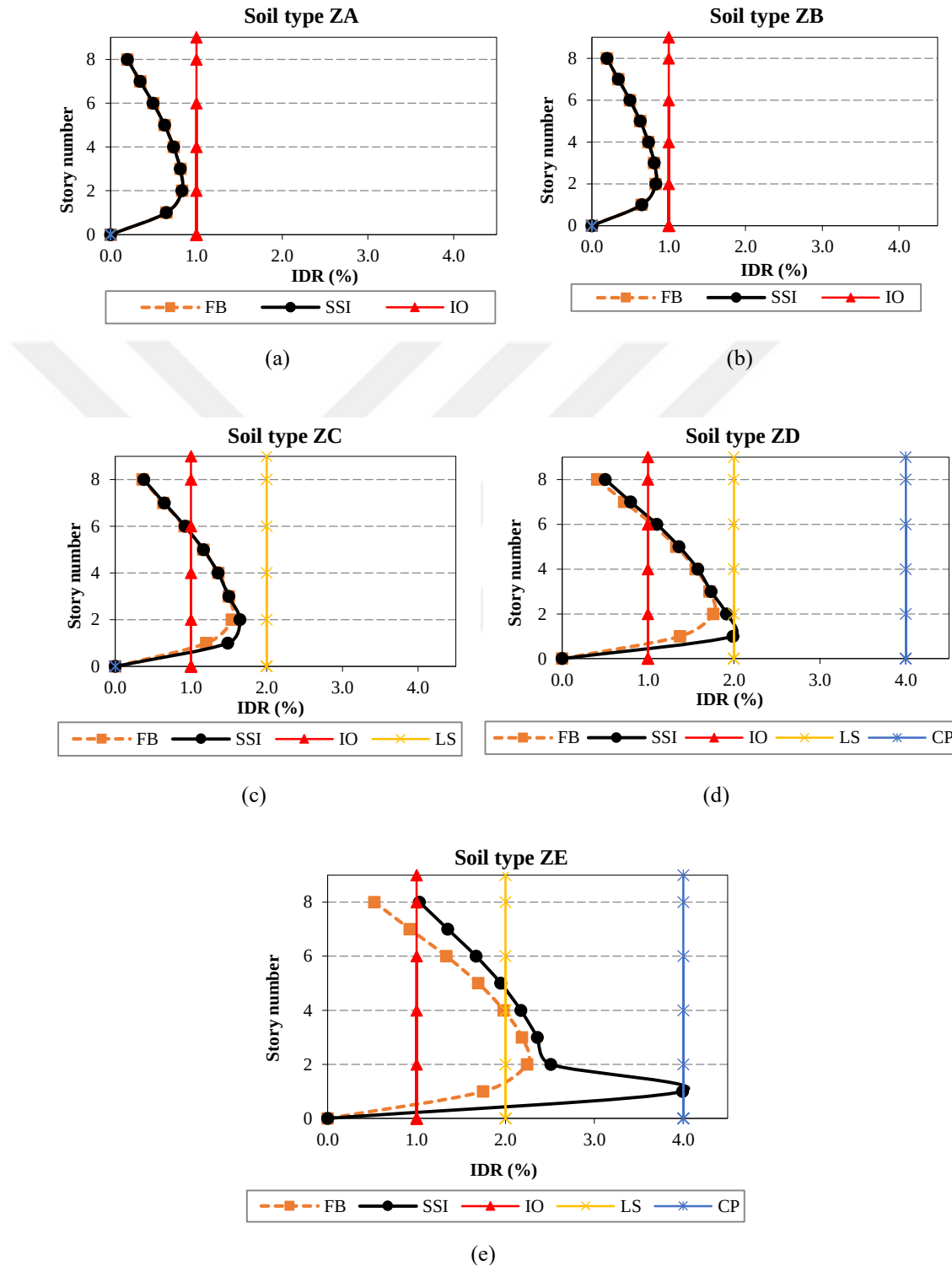
Figure 5.29. Inter-story drift ratios for the 8-Story models; comparison between FB and SSI conditions for different soil classes
