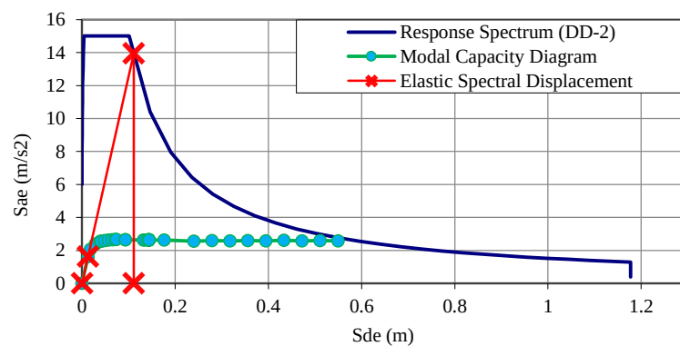
Figure 5.20. Determination of modal displacement demand for 4-story model
