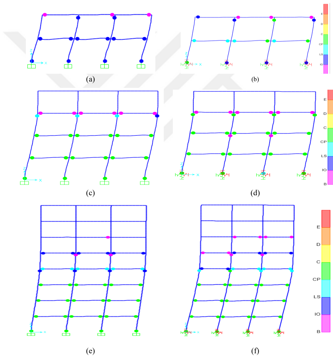
Figure 5.34. Comparison of plastic hinge formations for 2, 4 and 8 story models in the x-direction; (a), (c), (e) shows fixed base and (b), (d), (f) represent flexible base condition
