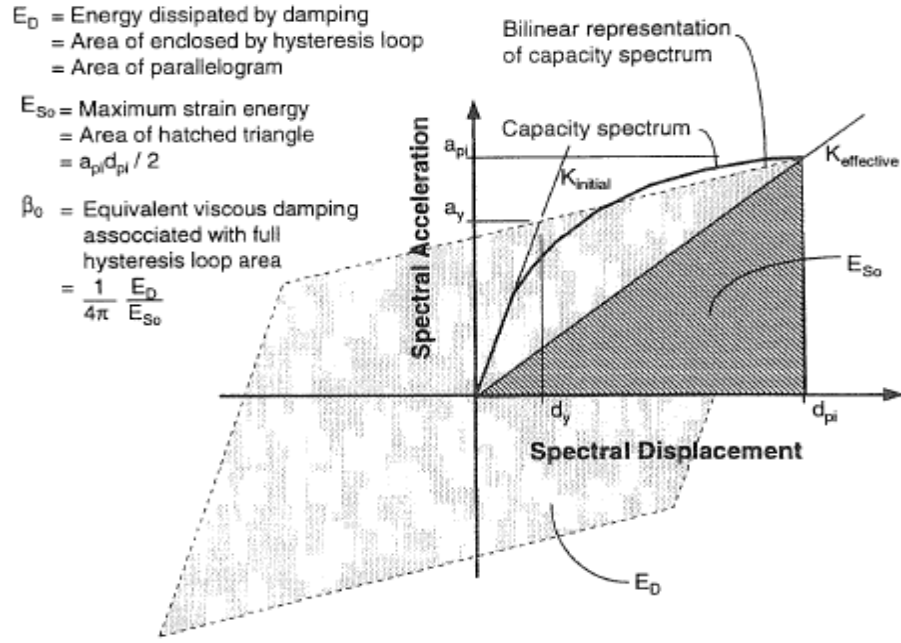
Figure 4.5. Derivation of damping for spectrum reduction [5]
