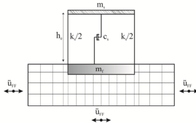
Figure 3.3. Soil-structure interaction analysis using the direct method [2]
