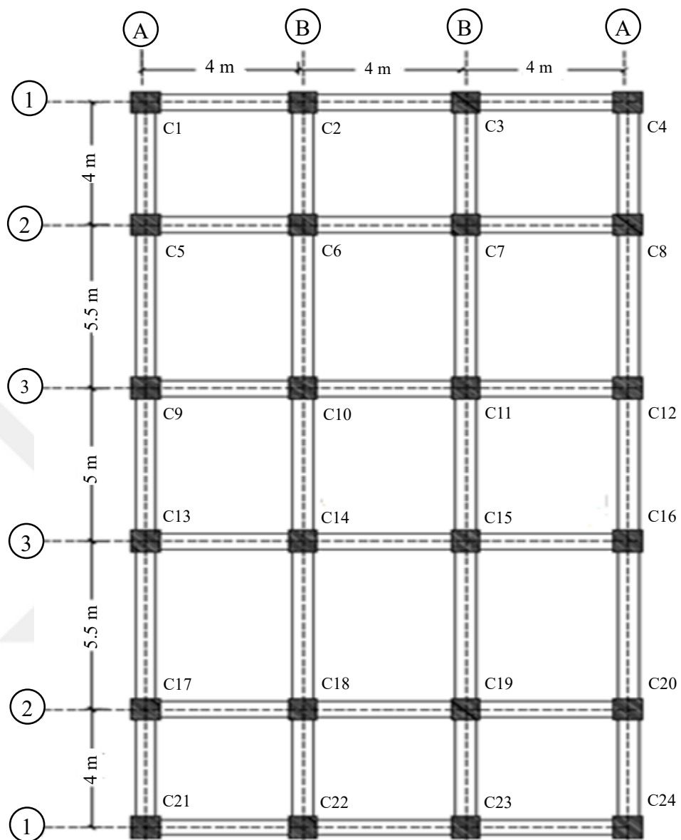
Figure 5.1. Plan view of the reference structures
