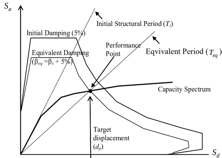
Figure 4.4. Graphical demonstration of the capacity spectrum method [5]
