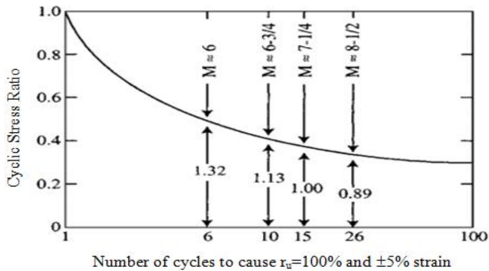
Figure 2.14 Relationship between number of cycles to cause liquefaction and CSR (Reproduced by Youd & Idris, 2001)
