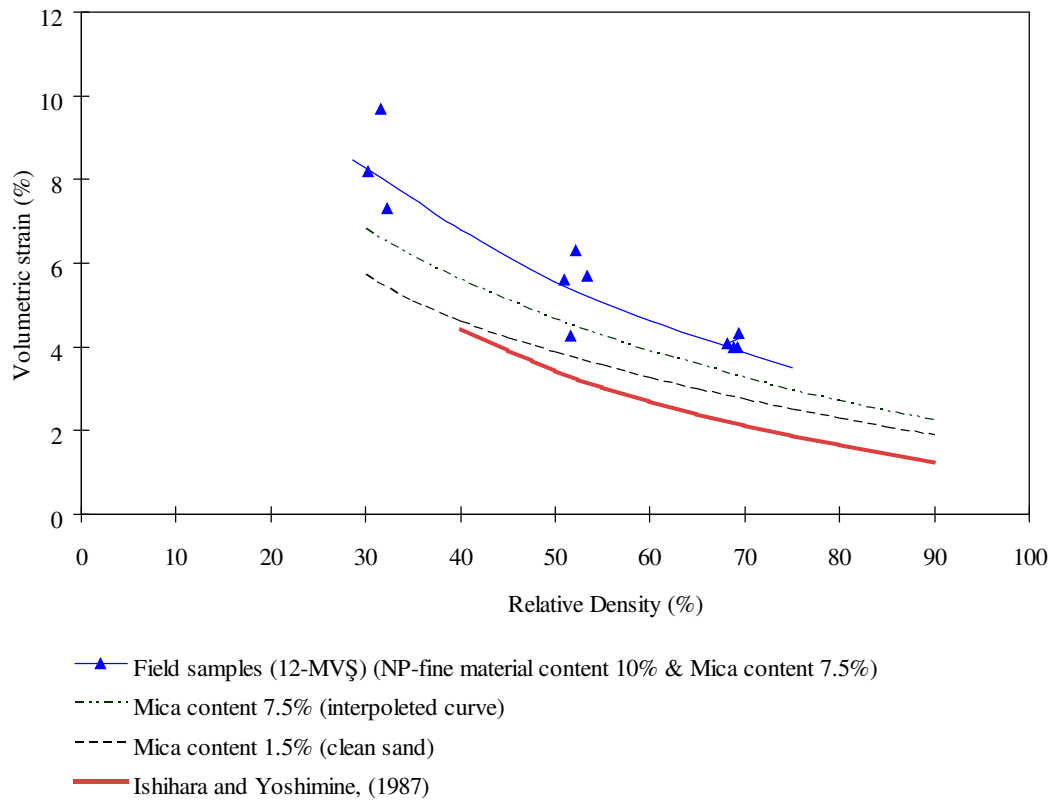
Figure 5.23 Post-liquefaction volumetric strain ( \epsilon_v ) of 12-MVŞ field samples containing 7.5% mica and 10% non-plastic fine materials ( \epsilon_{axial} > 8\% )
