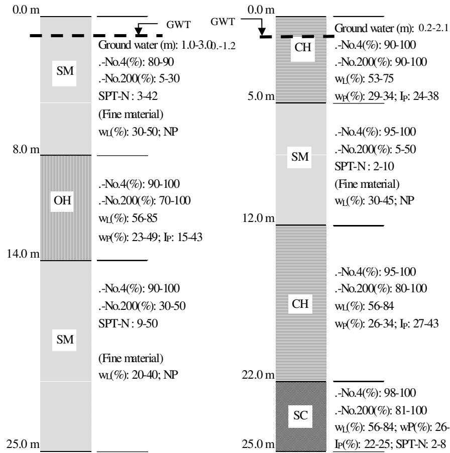
Figure 3.8 Geotechnical profile for the Karşıyaka coastline and Mavişehir-Bostanlı regions
