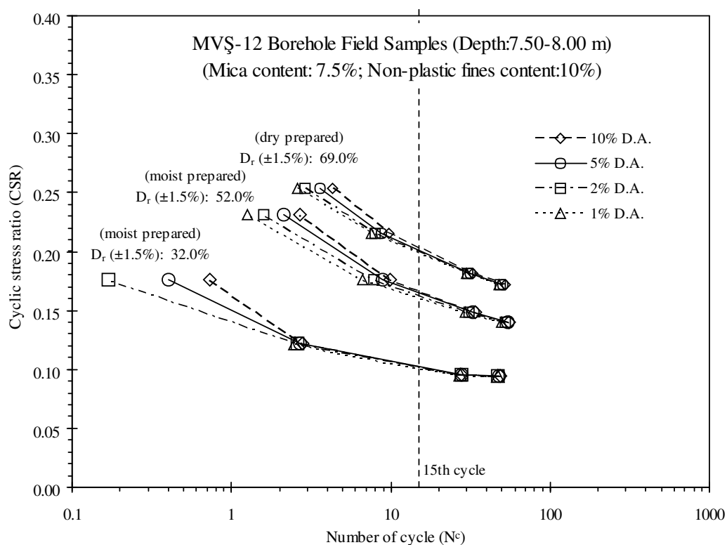
Figure 5.28 Cyclic stress ratio (CSR) versus number of cycles ( N_c ) for 1%, 2%, 5%, 10% double amplitudes (D.A.) and different relative densities for MVŞ-12 borehole field samples (Mica content: 7.5 %, non-plastic fines content: 10%)
