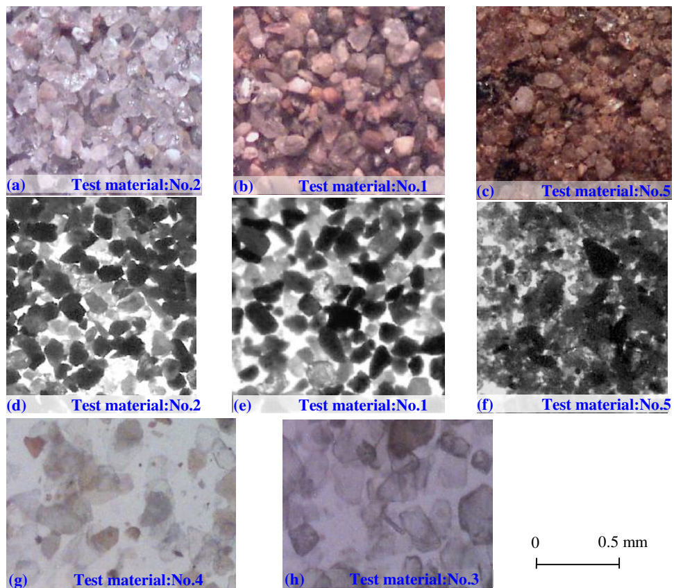
Figure 4.3 Images of test materials, (a), (d) Separated sand (No.2), (b), (e) Gediz River sand (No.1), (c), (f) 12-MVŞ (7.50m-8.0m) boreholes sandy sample (No.5), (g) Separated mica (No.4), (h) Commercially supplied mica (No.3)
