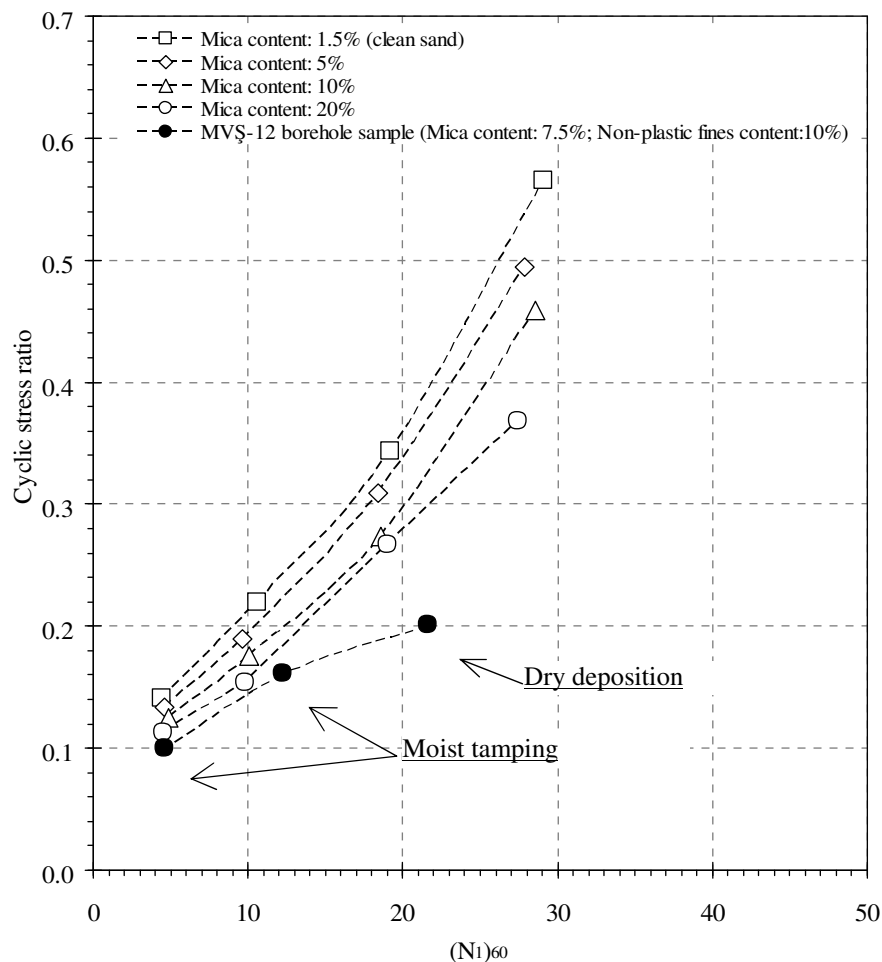
Figure 5.38 Cyclic resistance ratio (required 5% D.A. at 15 th cycle) versus equivalent (N_1)_{60} values for 1.5%, 5%, 10%, 20% mica contents and the MVŞ-12 sample
