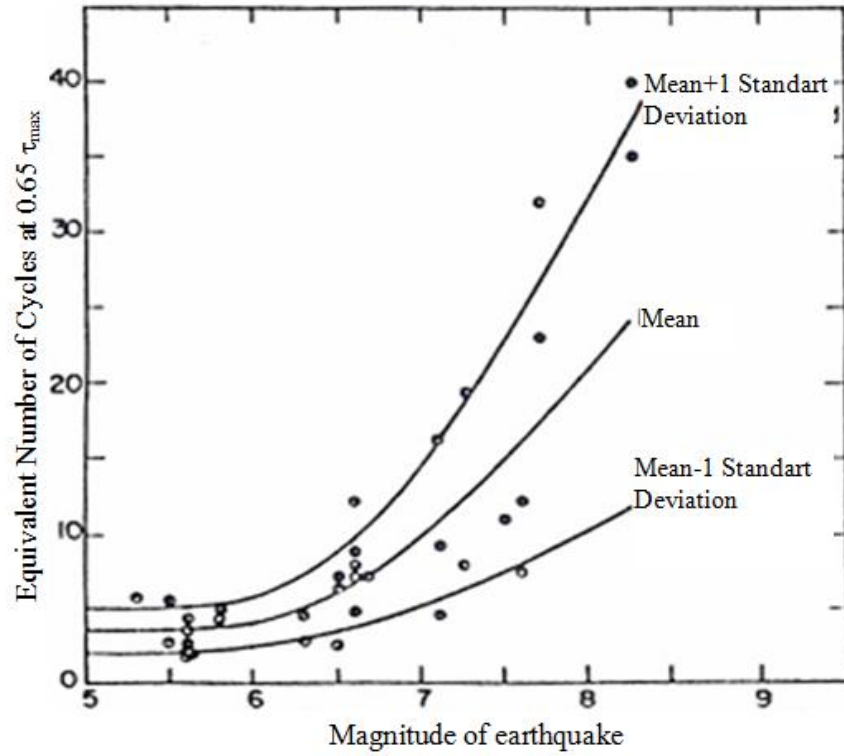
Figure 2.13 Relation between equivalent number of cycles at 0.65 \tau_{\max} and earthquake magnitude (Seed, 1979)
