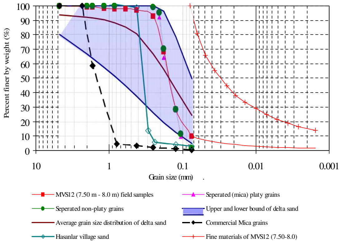
Figure 4.1 Grain size distribution curves of test materials
