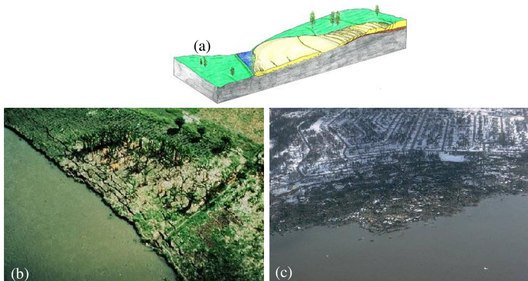
Figure 2.5 Lateral spreading due to liquefaction in (b) Motagua River, Guatemala Earthquake 1976 (c) Alaska, 1964 Alaska Earthquake
