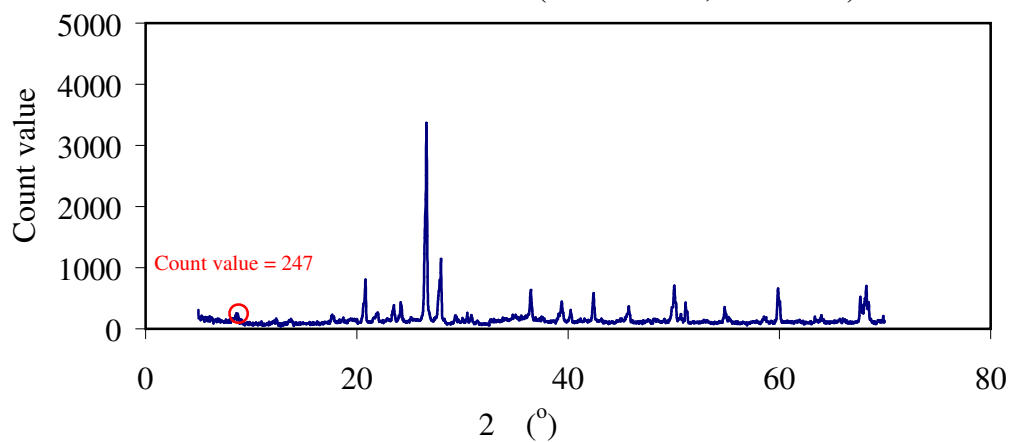
Sand-Mica Mixture (Sand=100%; Mica=0%)
