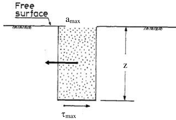
Figure 2.10 Equilibrium of forces near the surface (Seed & Idriss, 1971; Ishihara, 2003; Das, 1992)
