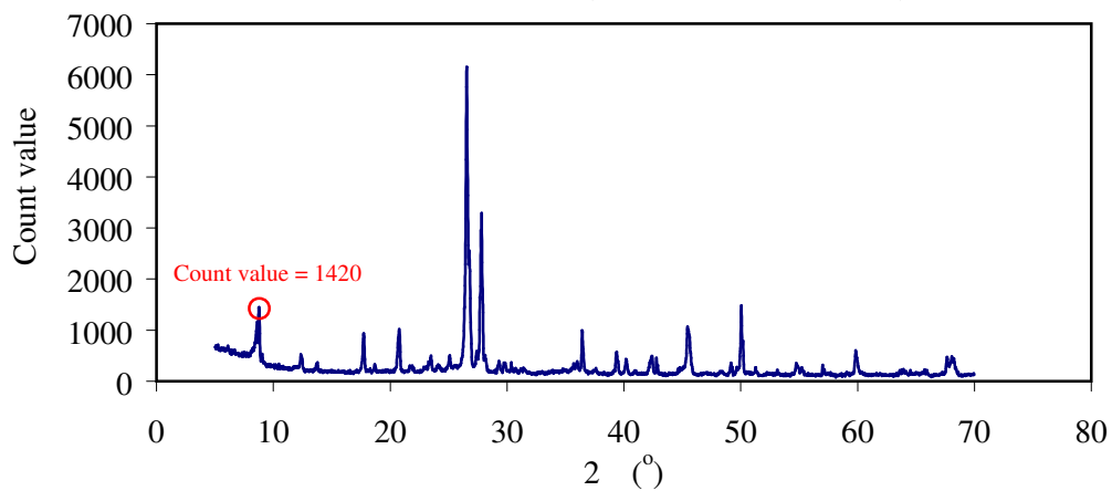
Sand-Mica Mixture (Sand=90%; Mica=10%)
