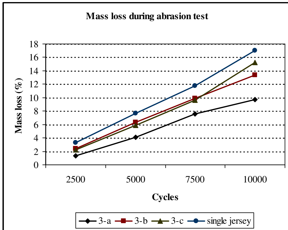
Figure C.3 Mass loss diagram for 3rd group gray samples
