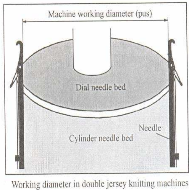
Figure 2.11 Diameter of circular knitting machine [24].
