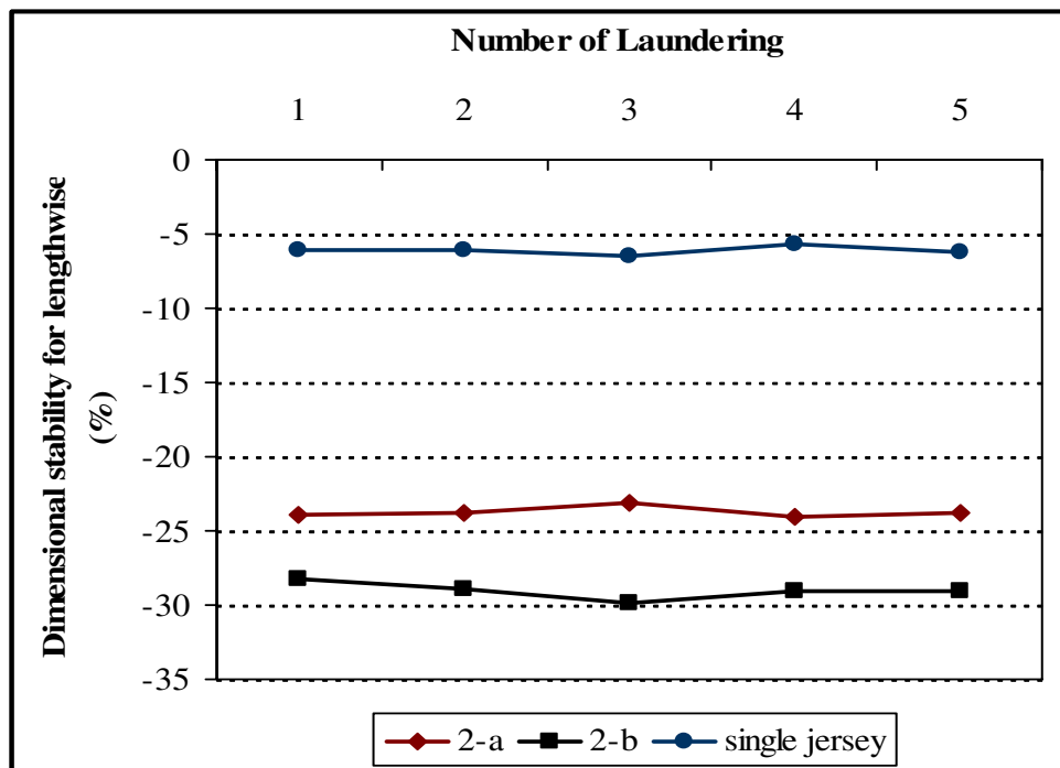
Figure B.2 Dimensional stability diagram for 2nd group gray samples
