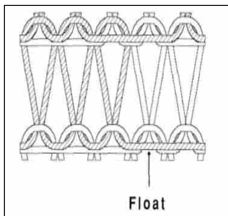
Figure 2.24 Floats [8].
