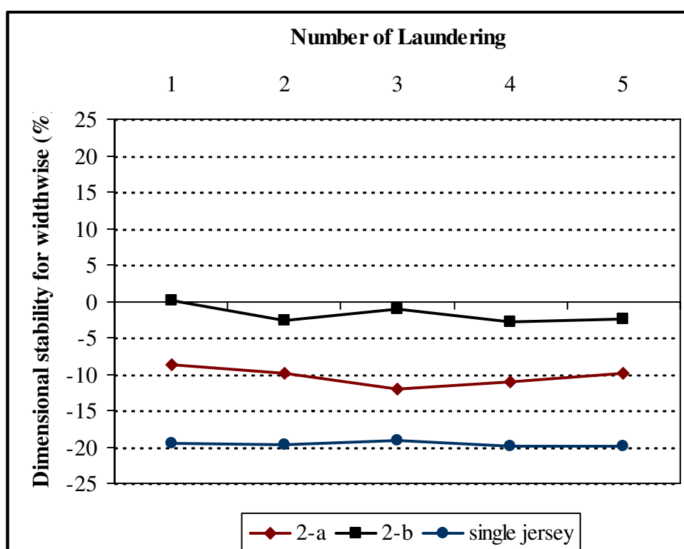
Figure B.6 Dimensional stability diagram for 2nd group gray samples
