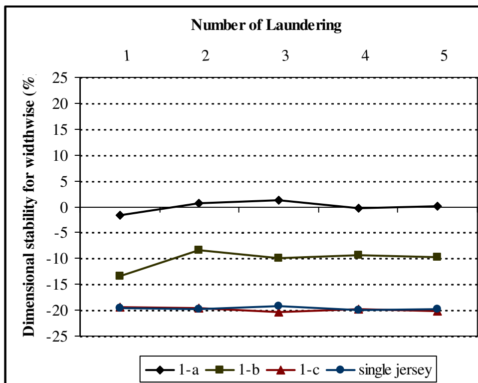
Figure B.5 Dimensional stability diagram for 1st group gray samples
