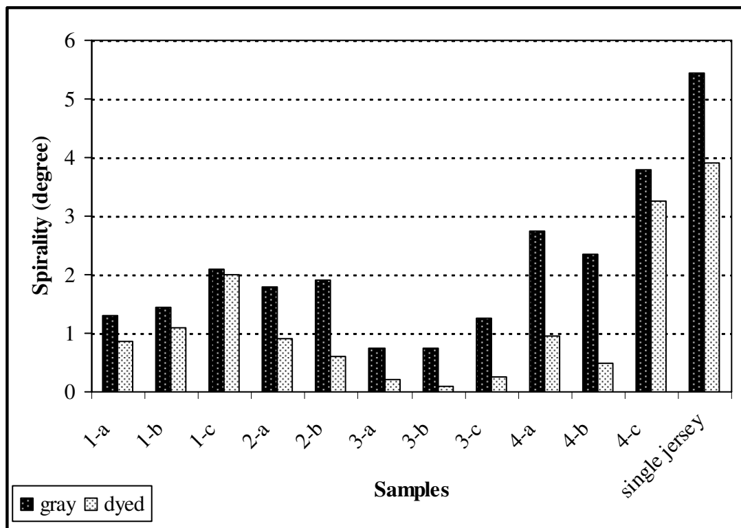
Figure 4.35 Spirality values of gray and dyed samples
