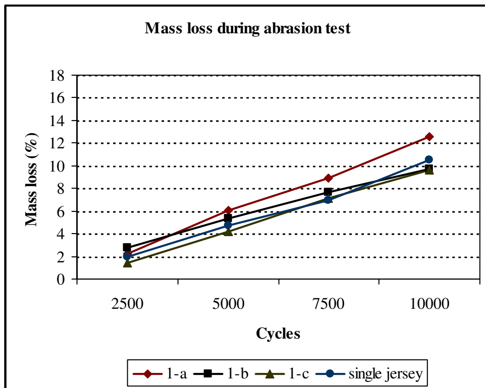
Figure C.5 Mass loss diagram for 1st group dyed samples
