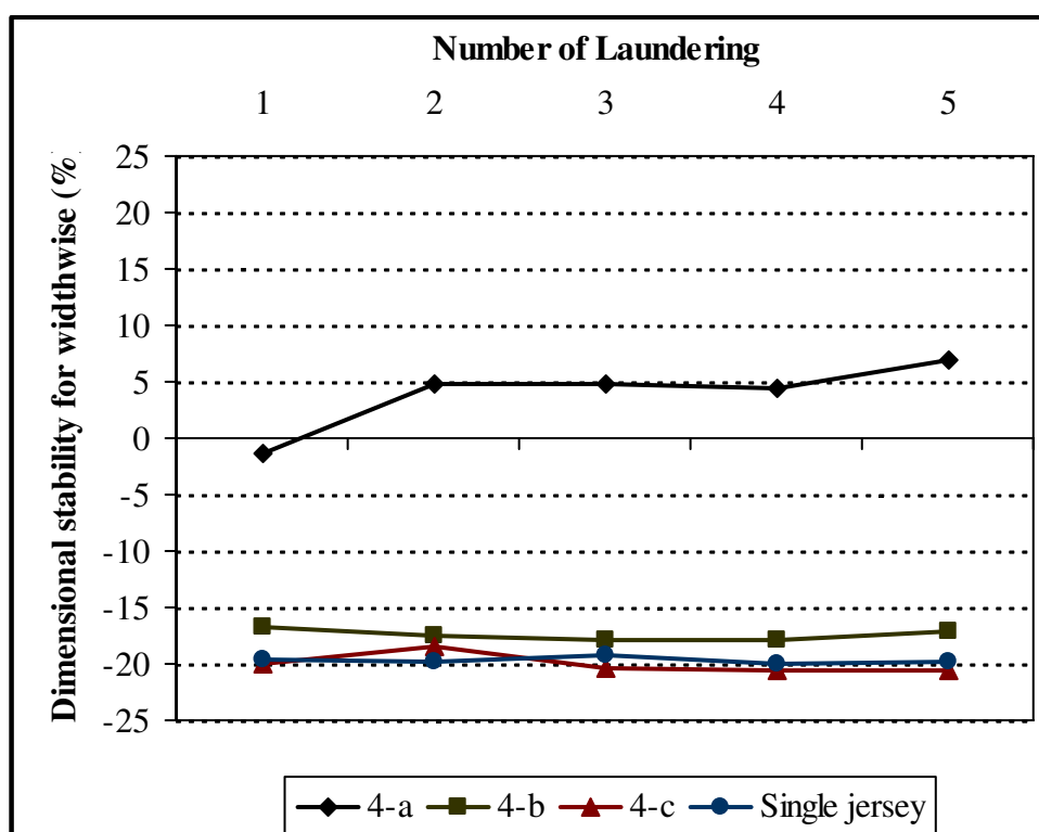
Figure B.8 Dimensional stability diagram for 4th group gray samples
