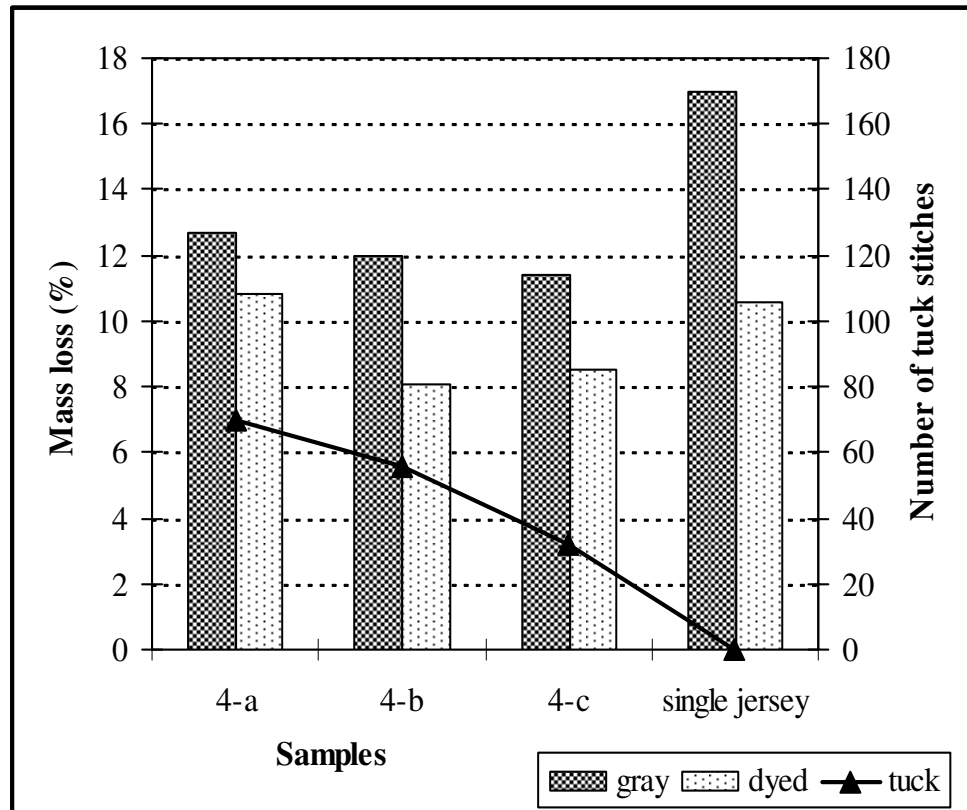
Figure 4.19 Abrasion resistance of the 4th group after 10000 cycles
