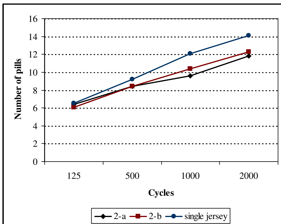
Figure D.6 Pill formation diagram for 2nd group dyed samples
