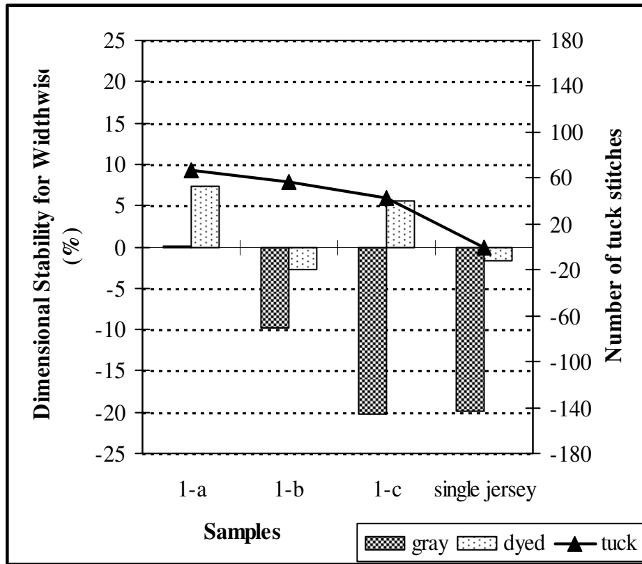
Figure 4.5 Dimensional stability of the 1st group after 5 laundering
