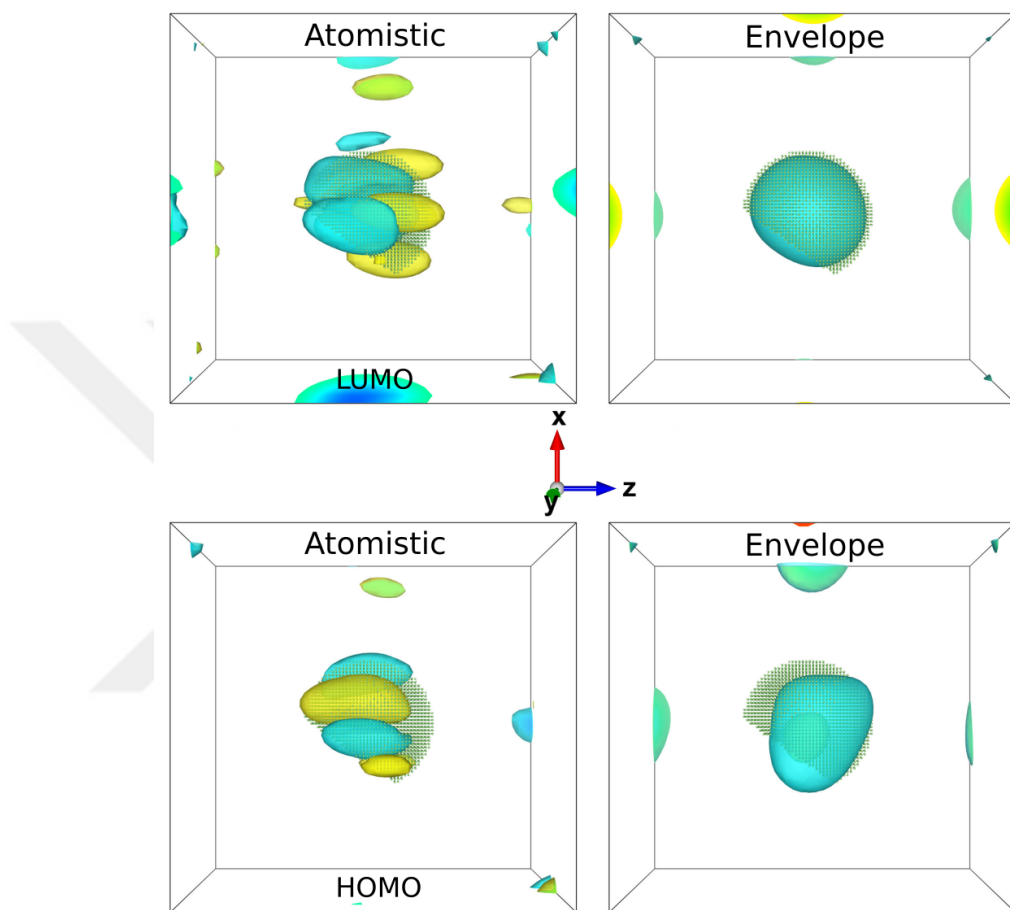
Figure 4.3: Same as the previous figure but for a QD with hydrophobic geometry.
