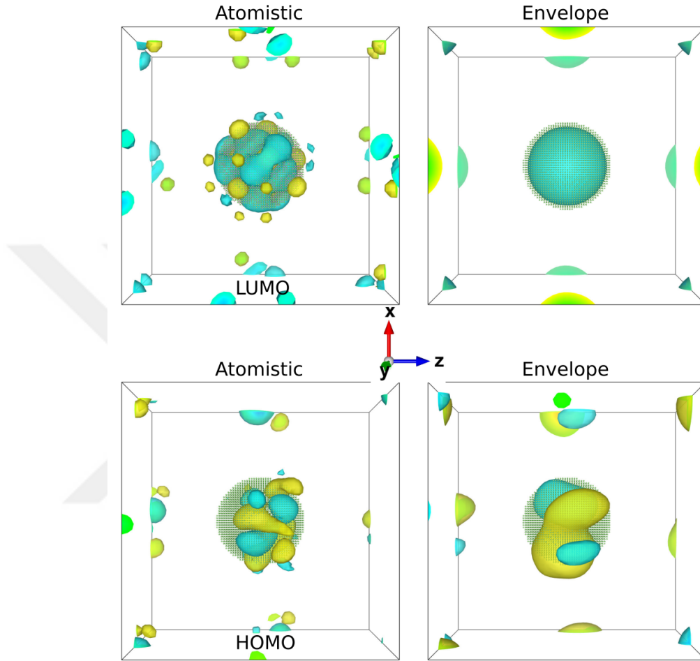
Figure 4.2: Atomistic wave functions and their extracted envelopes for HOMO and LUMO of the spherical \text{In}_{0.25}\text{Ga}_{0.75}\text{As}/\text{GaAs} SAQD. The wave functions and envelope isosurfaces are at a confidence interval of 99%. The green dots are in the positions of arsenic atoms of the QD.
