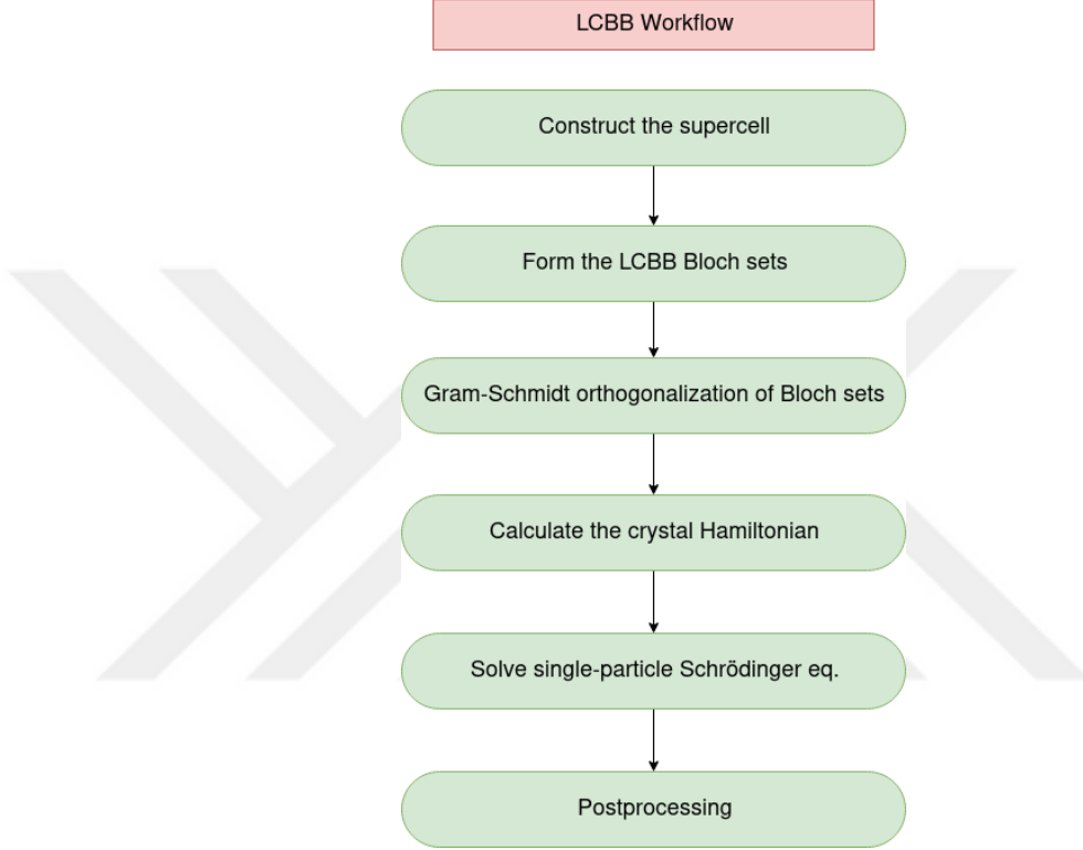
Figure 2.1: Workflow of LCBB method to calculate atomistic electronic structure of a nanostructure.
