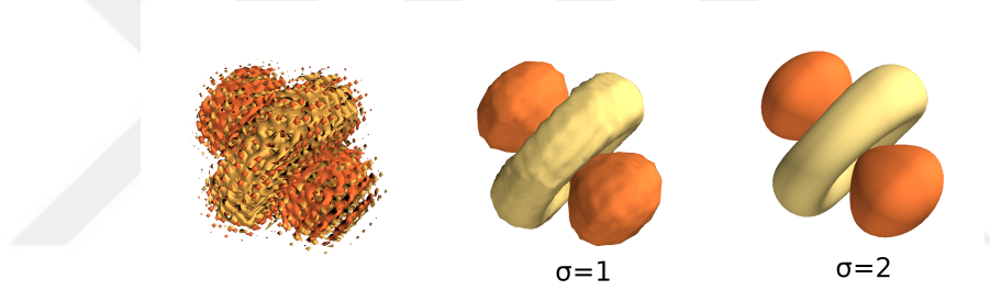
Figure 3.2: An atomistic wave function (left) and its envelopes after applying Gaussian filter with different \sigma values.
