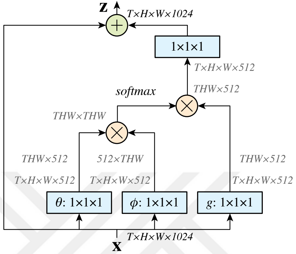
Figure 2.14: Non-local block [72]
