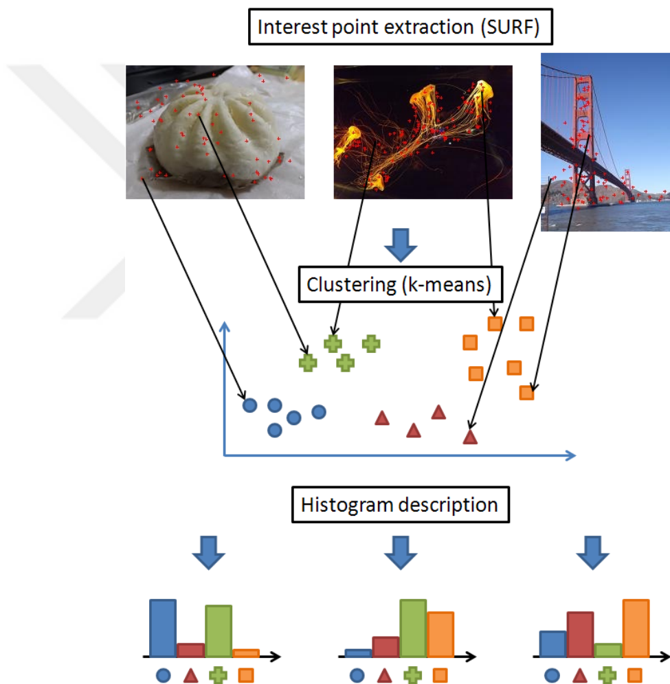
Figure 2.2: The general approach for hand-crafted based learning methods
