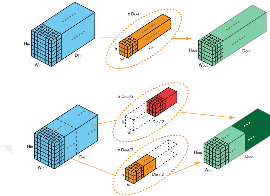
Figure 2.6: Conventional (Top) and group (Bottom) convolution operations. The image is from Towards data science: Comprehensive introduction to different types of convolutions in deep learning
