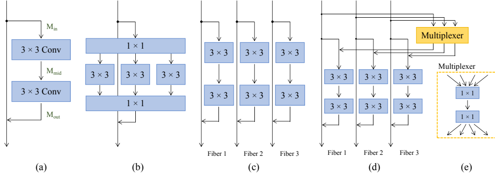
Figure 2.18: Possible bottleneck blocks implementations to ResNet architecture. (a) Basic Block. (b) Bottleneck block of ResNeXt architecture. (c) Multi-Fiber architecture. (d) Multi-fiber with multiplexer. (e) Multiplexer
