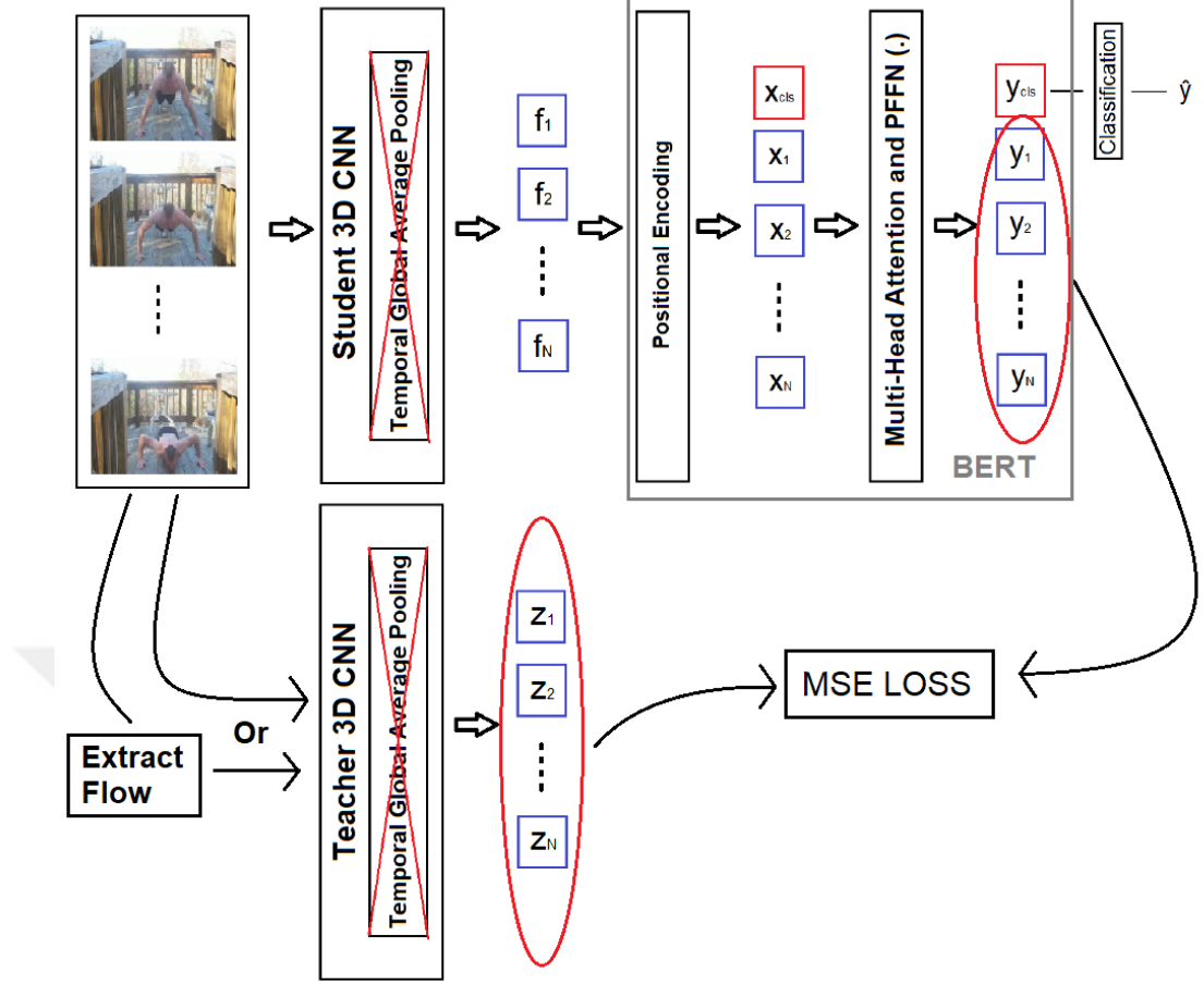
Figure 5.1: BERT-based Distillation
