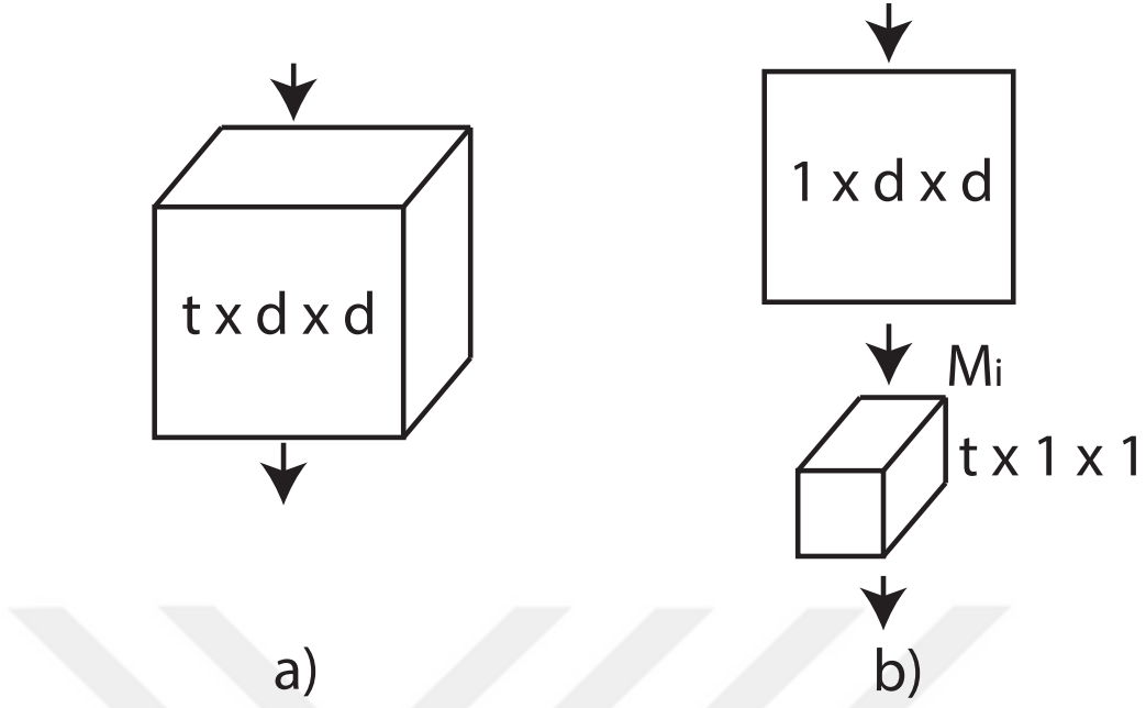
Figure 2.12: (a) Conventional 3D convolution. (b) Separable 3D Convolution [64]
