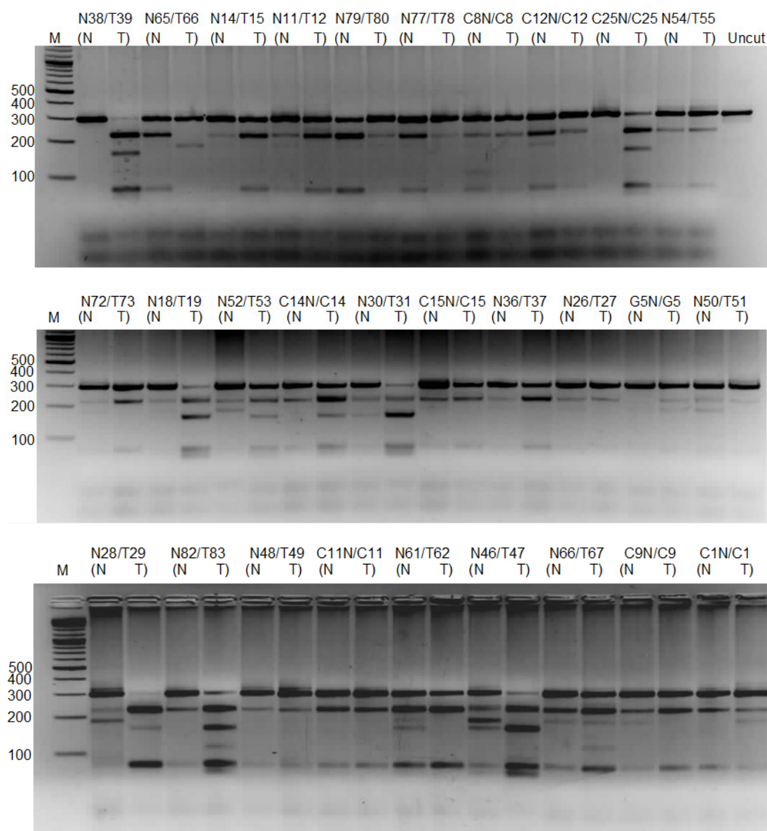
Figure 4.1.11 : Bst UI restriction analysis of P1 region amplified by SIPM1dF / SIPM1iyR1 and SIPM1iF / SIPM1iyR1 semi-nested primer pairs. 14 out of 29 normal-tumor paired samples (48%) were methylated. M, marker (bp).
