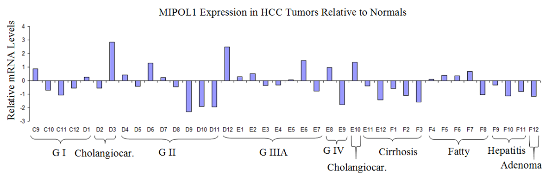
Figure 4.8.5 : MIPOL1 mRNA expression in HCC tumors relative to normals.
