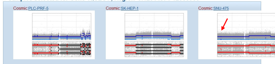
Figure 1.8.3 : Copy number analysis of chromosome 3 in PLC, SkHep1 and Snu475 HCC cell lines. LOH (red arrow) was described in the region containing IQSEC1 gene. Data and the photograph obtained from SANGER CONAN: Copy Number Analysis. ( http://www.sanger.ac.uk/cgi-bin/genetics/CGP/conan/search.cgi ).
