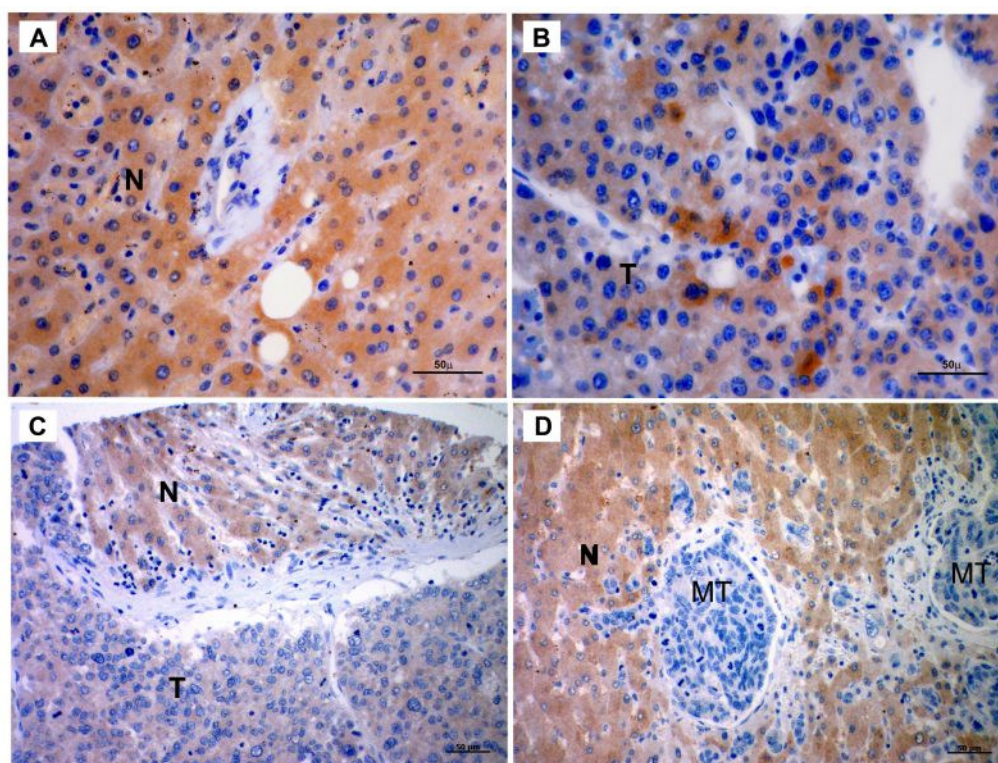
Figure 4.1.6: Representative photographs of immunohistochemistry of SIP1 in human liver tissues. A; Normal tissue shows strong, uniform cytoplasmic staining (brown) throughout the tissue. B; HCC specimen shows faint SIP1 immunoreactivity. C; Tissue array case shows differential expression pattern of SIP1 in HCC and non tumoral-normal hepatocytes. D; A metastatic adenoma case in normal liver tissue. Metastatic tumor cells shows negative staining of SIP1, but extensive SIP1 expression is seen in normal area. N, Normal liver hepatocytes; T, HCC tumor cells; MT, Metastatic adenocarcinoma cells (Scale Bars: 50µm).
