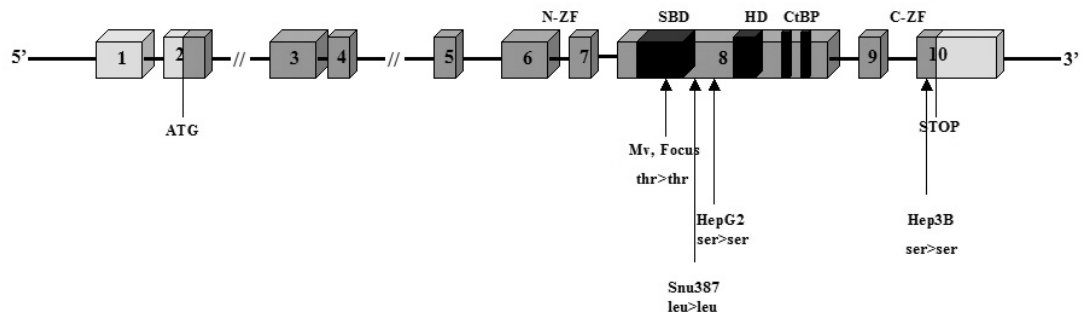
Figure 4.1.7: SIP1 silent mutations was found in HCC cell lines and their locations are indicated (GeneID:9839, Ensembl:ENSG00000169554).
