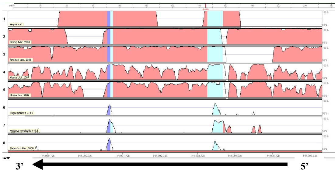
Figure 4.1.9: Conservation of 5' region of SIP1 gene according to GenomeVista analysis. (1:Human, 2:Chimp, 3:Rhesus, 4:Mouse, 5:Horse, 6:Fugu, 7: Xenopus, 8: Zebrafish) Light blue boxes shows UTR, blue boxes shows exons (1 st exon UTR and 2 nd exon, respectively).
