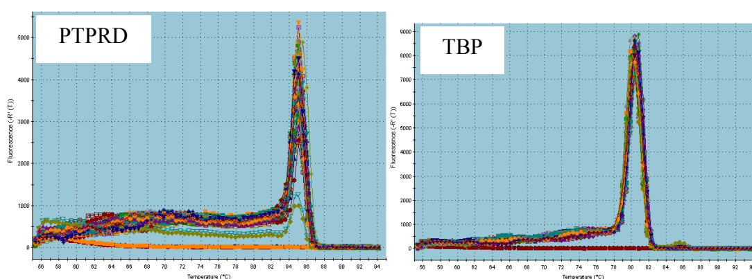
Figure 4.2.4.: PTPRD mRNA expression in HCC samples. PTPRDcd4F / PTPRDcd3R primer pair was used. cDNAs from human liver tissues of normal and various stages of liver cancers were subjected to real-time reverse transcription–PCR for detection of PTPRD mRNA expression. The data represent mRNA levels of PTPRD normalized to TBP . Dissociation curves of both genes are also presented.
