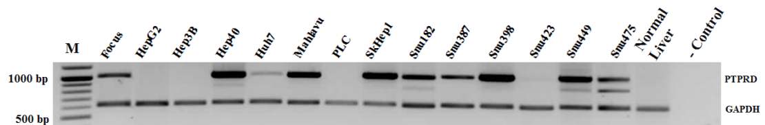
Figure 4.2.2 : Multiplex semi-quantitative RT-PCR of PTPRD in HCC Cell Lines. GAPDH was used as an internal control. M, marker (bp).
