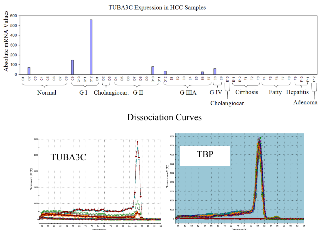
Figure 4.6.5 : TUBA3C mRNA expression in HCC samples. cDNAs from human liver tissues of normal and various stages of liver cancers were subjected to real-time reverse transcription–PCR for detection of TUBA3C mRNA expression. Tuba3CRTF / Tuba3CRTR primer pair was used. The data represent mRNA levels of TUBA3C mRNA normalized to TBP . Dissociation curves of both genes are also presented.
