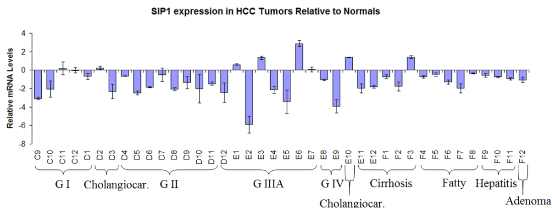
Figure 4.1.5 : SIP1 mRNA expression in HCC tumors relative to normals.
