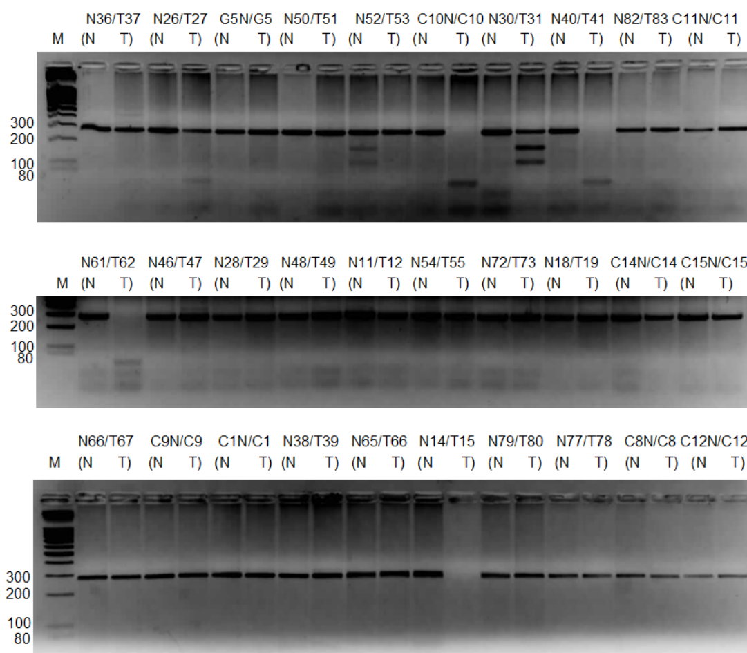
Figure 4.1.12 : Bst UI restriction analysis of P2 region amplified by SIPM2iyF1 / SIPM2iR and SIPM2iyF1 / SIPM2iyR2 semi-nested primer pairs. 1 out of 26 normal-tumor paired samples (4%) were methylated. M, marker (bp).
