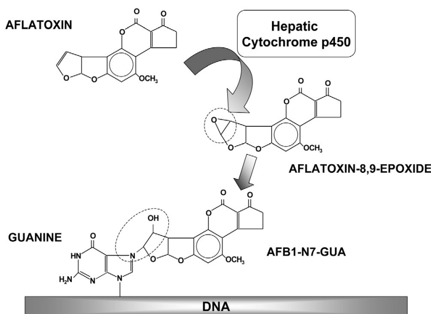
Figure 1.1.2 : Metabolic conversion of aflatoxin B1 to the 8,9-epoxide by cytochrome p450 and subsequent DNA adduct formation (from “Smela et al. , 2001” with permission).
