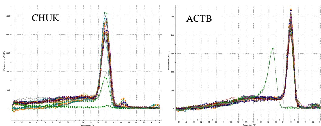
Figure 4.9.1: Quantitative Real-Time Analysis of CHUK in 14 HCC cell lines. ACTB was used as an internal control. Experiment conducted two times and standart deviations are indicated. Dissociation curves of CHUK and ACTB primers are also presented.
