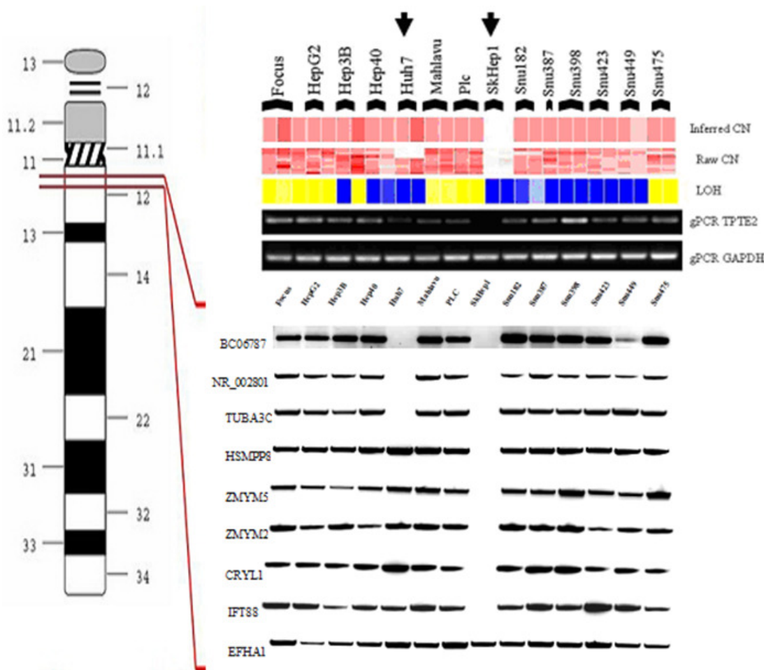
Figure 4.6.1: PCR results of the genes located in the deleted region (Figure was adapted from Kubilay Demir, M.Sc.).
