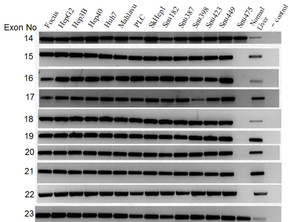
Figure 4.2.10: Homozygous deletion on Snu475 HCC cell line between exons 15-22.
