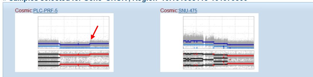
Figure 1.10.2 : Copy number analysis of chromosome 10 in PLC and Snu475 HCC cell lines. LOH (red arrow) was described in the region containing CHUK gene. Data and the photograph obtained from SANGER CONAN: Copy Number Analysis. ( http://www.sanger.ac.uk/cgi-bin/genetics/CGP/conan/search.cgi ).
