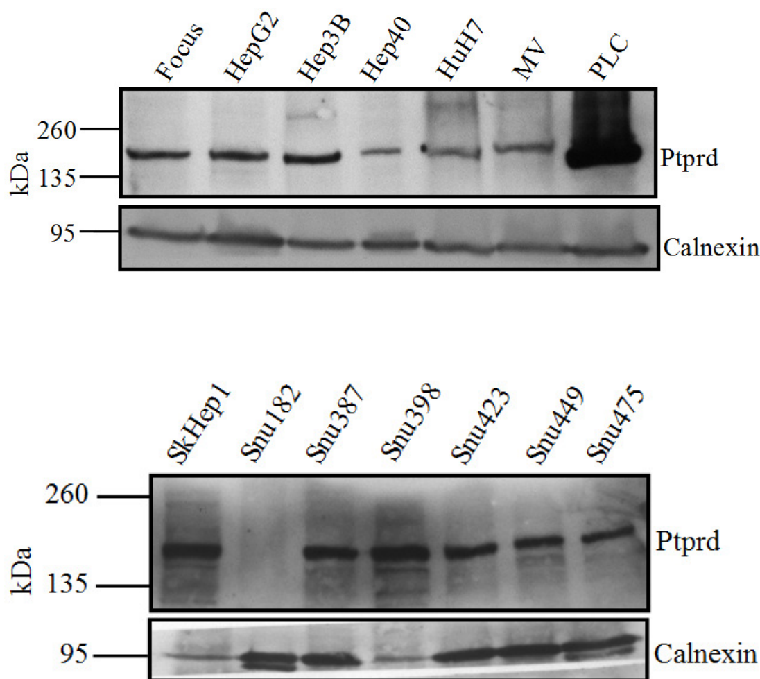
Figure 4.2.3 : Western blot analysis of PTPRD in 14 HCC Cell lines. PTPRD was expected to give band at 175 kDa. Calnexin (90 kDa) was used as a loading control. 35 µg protein were loaded each well. Spectra TM Multicolor Broad Range Protein Ladder (Fermentas, USA) was used as a marker.
