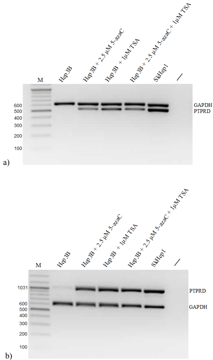
Figure 4.2.13 : Restoration of PTPRD mRNA expression in Hep3B cell line after 5'-AzaC and/or TSA treatment shown by multiplex semi-quantitative RT-PCR. M, marker (bp); (-), negative control. SkHep1 cell line was used as a PTPRD positive control. GAPDH (with an expected product size of 611 bp) was used as an internal control. a) PTPRDcd3F/PTPRDcd3R primer pair with an expected product size of 517 bp and b) PTPRDcd9F / PTPRDcd9R primer pair with an expected product size of 1004 bp was used.
