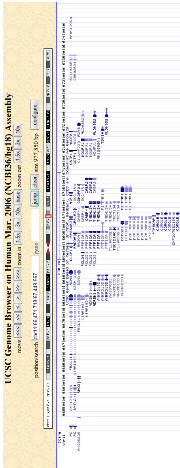
Figure 1.6.1 : Graphical view of chromosome 11(q13.1-q13.2) region and the genes reside in this region (UCSC Genome Browser: http://genome.ucsc.edu/cgi-bin/hgTracks )
