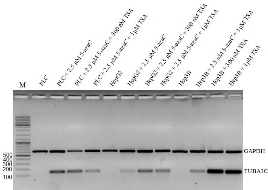
Figure 4.6.7: Restoration of TUBA3C mRNA expression after 5'-AzaC and TSA treatments. Tuba3CRTF/tuba3CRTR primer pair with an expected product size of 145 bp and GAPDH RTF/GAPDH RTR pair with an expected product size of 611 bp were used. M, marker (bp); GAPDH was used as an internal control.
