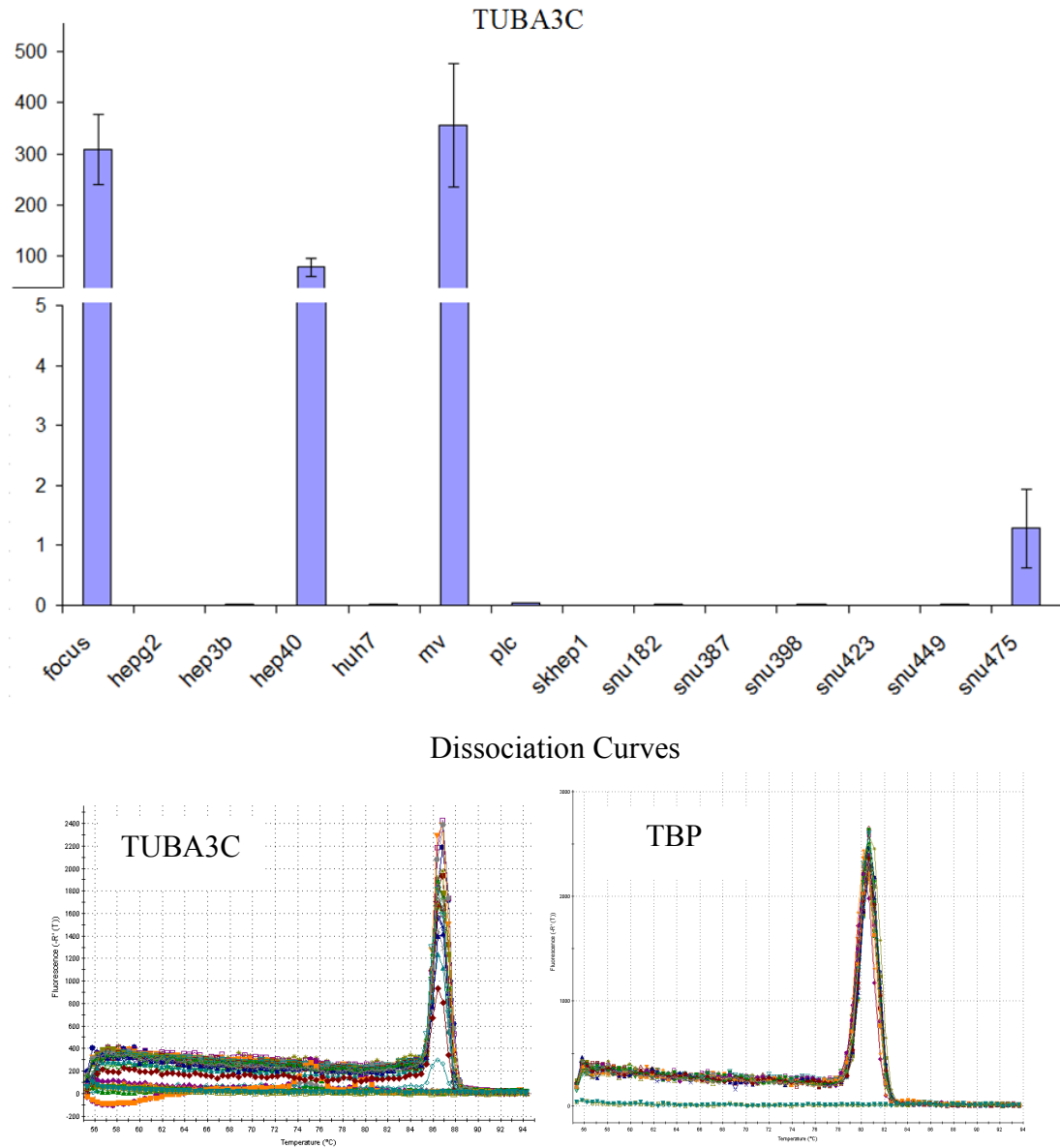
Figure 4.6.4 : Quantitative Real-Time Analysis of TUBA3C in HCC cell lines. Tuba3CRTF / tuba3CRTR primer pair was used. TBP was used as an internal control. Experiment conducted two times and standart deviations are indicated. Dissociation curves of TUBA3C and TBP primers are also presented.
