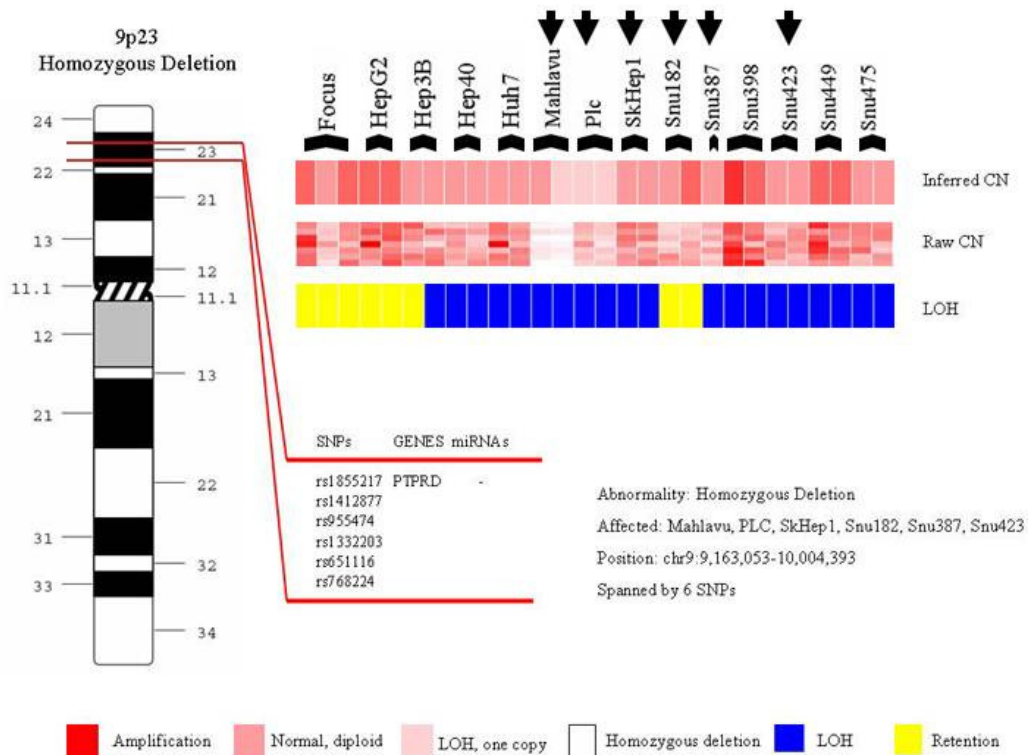
Figure 1.3.1 : Homozygous deletion at 9p23 in Mahlavu, PLC, SkHep1, Snu182, Snu387 and Snu423 HCC cell lines (adapted from Kubilay Demir thesis study).
