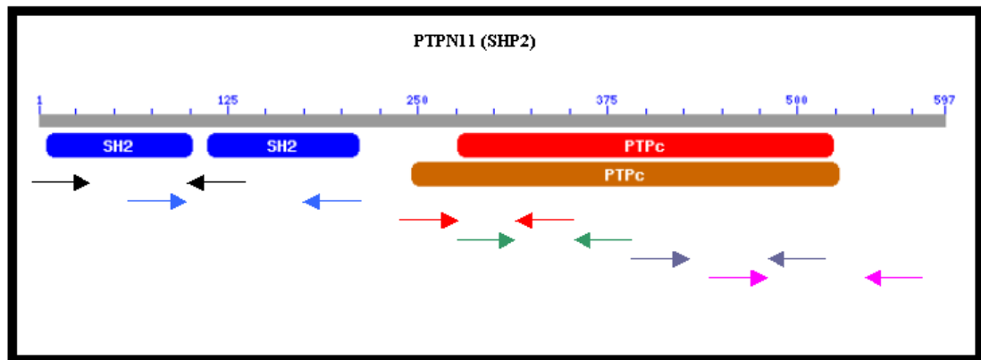
Figure 4.4.2: Representative figure showing functional domains and locations of the primers used to amplify PTPN11 gene. Each F/R primer pairs specific for exons 3, 4, 7, 8, 12, 13 are represented in same color.
