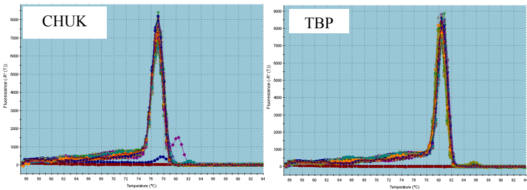
Figure 4.9.2: CHUK mRNA expression in HCC samples. cDNAs from human liver tissues of normal and various stages of liver cancers were subjected to real-time reverse transcription–PCR for detection of CHUK mRNA expression. The data represent mRNA levels of CHUK mRNA normalized to TBP . Dissociation curves of both genes are also presented.
