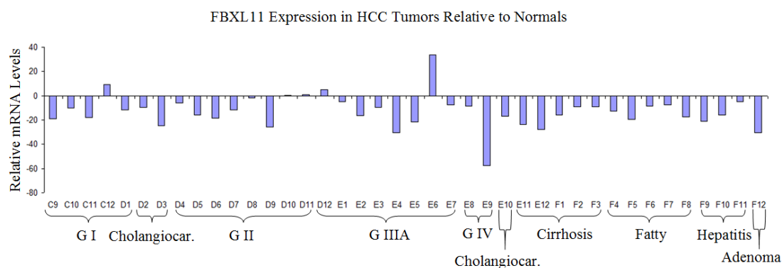
Figure 4.5.4 : FBXL11 mRNA expression in HCC tumors relative to normals.
