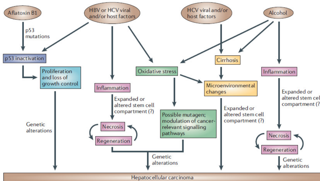
Figure 1.1.5 : Mechanisms of hepatocarcinogenesis for the various aetiologic factors (from “Farazi,P.A. and DePinho,R.A. 2006” with permission)
