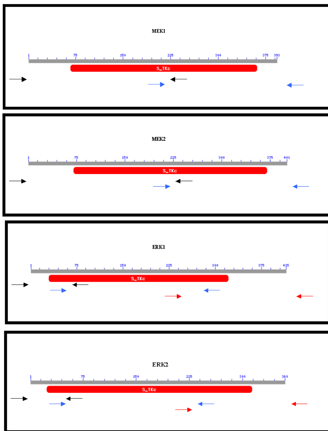
Figure 4.4.1: Representative figures showing functional domains and locations of the primers used for amplification of each gene cDNA. Each F/R primer pairs represented in same color.
