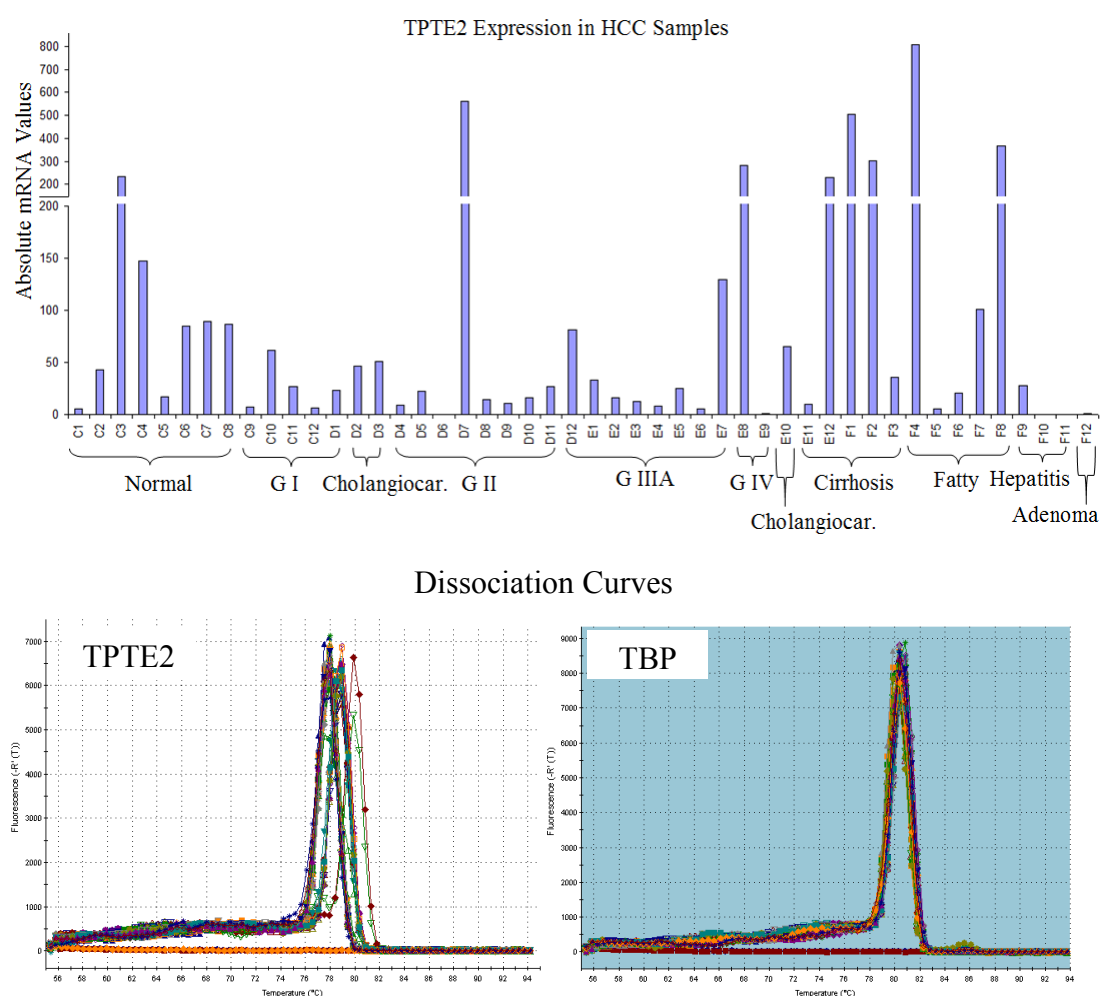
Figure 4.6.11 : TPTE2 mRNA expression in HCC samples. cDNAs from human liver tissues of normal and various stages of liver cancers were subjected to real-time reverse transcription–PCR for detection of TPTE2 mRNA expression. TPTE2F /TPTE2R primer pair was used. The data represent mRNA levels of TPTE2 mRNA normalized to TBP . Dissociation curves of both genes are also presented.
