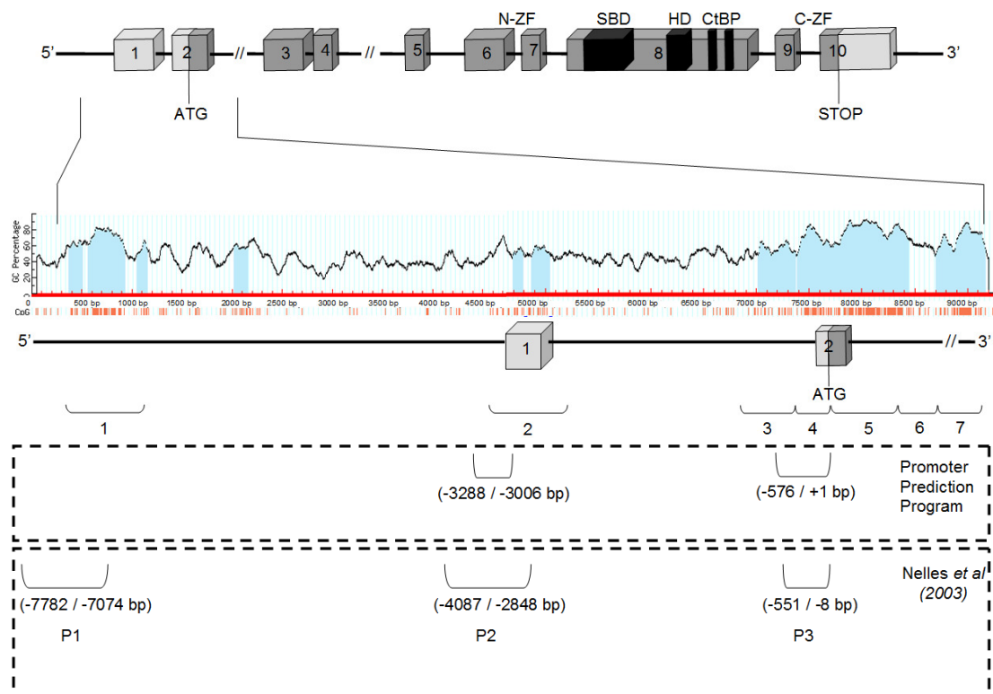
Figure 4.1.8: In Silico analysis of CpG-rich SIP1 promoter. Genomic structure, CpG island prediction (MethPrimer) and promoter predictions (Promoter2.0 and Nelles et al. , 2003 study) were represented.
