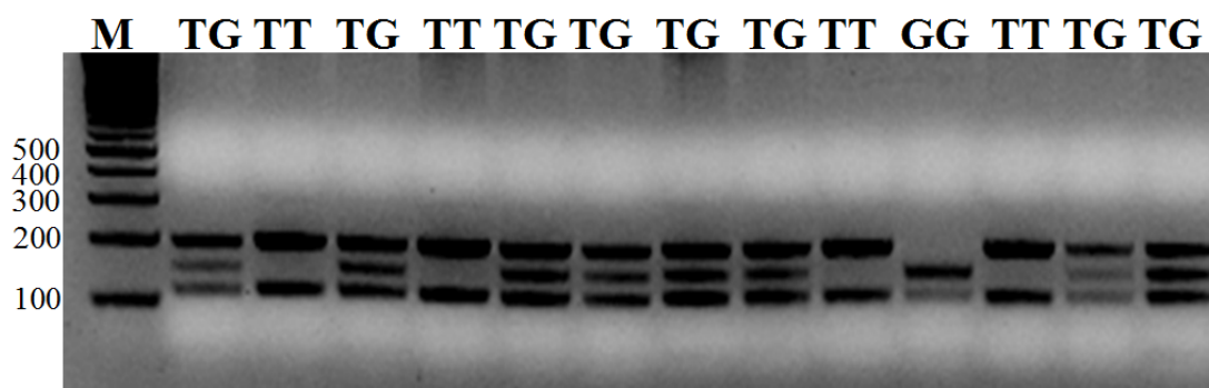
Figure 4.3.1: Representative photograph of MspAII digested PCR products of HCC samples resolved on 3% agarose gel. Three distinct patterns were observed representing T/T wild type, T/G heterozygote, G/G homozygote. M, marker (bp).
