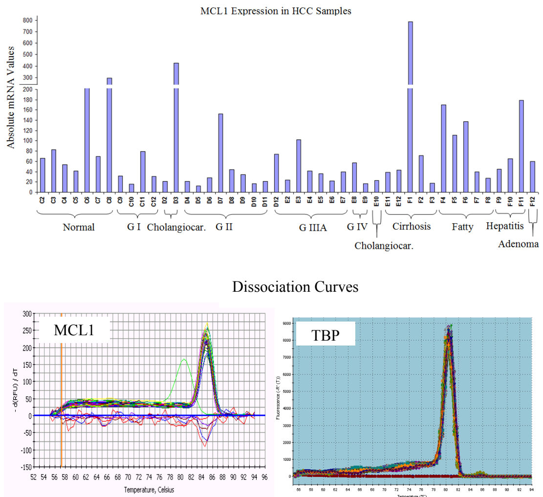
Figure 4.10.3: MCL1 mRNA expression in HCC samples. cDNAs from human liver tissues of normal and various stages of liver cancers were subjected to real-time reverse transcription–PCR for detection of MCL1 mRNA expression. The data represent mRNA levels of MCL1 mRNA normalized to TBP . Dissociation curves of both genes are also presented.
