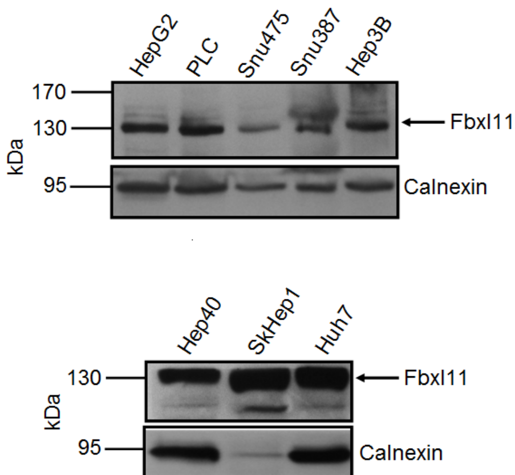
Figure 4.5.2 : Western blot analysis of FBXL11 in HCC cell lines. FBXL11 was expected to give band at 132 kDa. Calnexin (90 kDa) was used as a loading control. 35 \mu g protein were loaded each well. PageRuler™ Prestained Protein Ladder (Fermentas, USA) was used as a marker.
