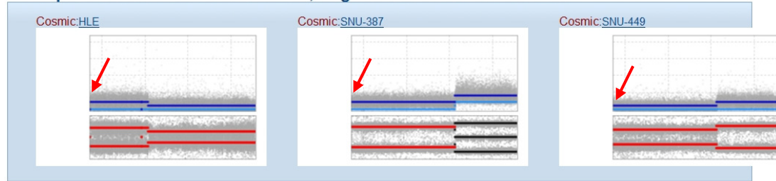
Figure 1.7.3 : Copy number analysis of chromosome 13 in HLE, Snu387 and Snu449 HCC cell lines. LOH (red arrows) was described in the region containing ZNF198 ( ZMYM2 ) and TPTE2 genes.
