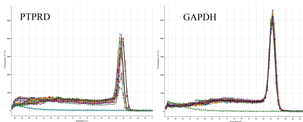
Figure 4.2.1 : Quantitative Real-Time Analysis of PTPRD in HCC Cell lines. PTPRDcd4F / PTPRDcd3R primer pair was used. GAPDH was used as an internal control. Experiment conducted two times and standart deviations are indicated. Dissociation curves of both genes are also presented.
