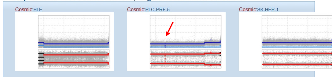
Figure 1.9.2 : Copy number analysis of chromosome 14 in HLE, PLC and SkHep1 HCC cell lines. LOH (red arrow) was described in the region containing MIPOL1 gene. Data and the photograph obtained from SANGER CONAN: Copy Number Analysis. ( http://www.sanger.ac.uk/cgi-bin/genetics/CGP/conan/search.cgi ).
