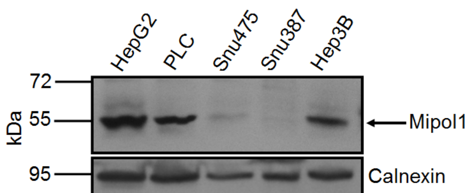
Figure 4.8.2 : Western blot analysis of MIPOL1 in 5 HCC cell lines. MIPOL1 was expected to give band at 50 kDa. Calnexin (90 kDa) was used as a loading control. 35 µg protein were loaded each well. PageRuler™ Prestained Protein Ladder (Fermentas, USA) was used as a marker.
