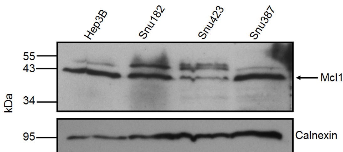
Figure 4.10.2 : Western blot analysis of MCL1 in 4 HCC cell lines. MCL1 was expected to give band at 37 kDa. Calnexin (90 kDa) was used as a loading control. 35 µg protein were loaded each well. PageRuler™ Prestained Protein Ladder (Fermentas, USA) was used as a marker.
