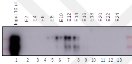
Figure 9: Purification of the recombinant His:Rpb1 Protein: A) Size exclusion chromatography of recombinant His-RPB1 subunit of Pol II via 20 ml Superose 6 column using ÄKTA system. The numbers corresponds to the 500 ul fractions collected at a given time point. B) Western blot analysis of Superose 6 purified His-RPB1. The numbers indicate collected 500ul fractions during the procedure.
