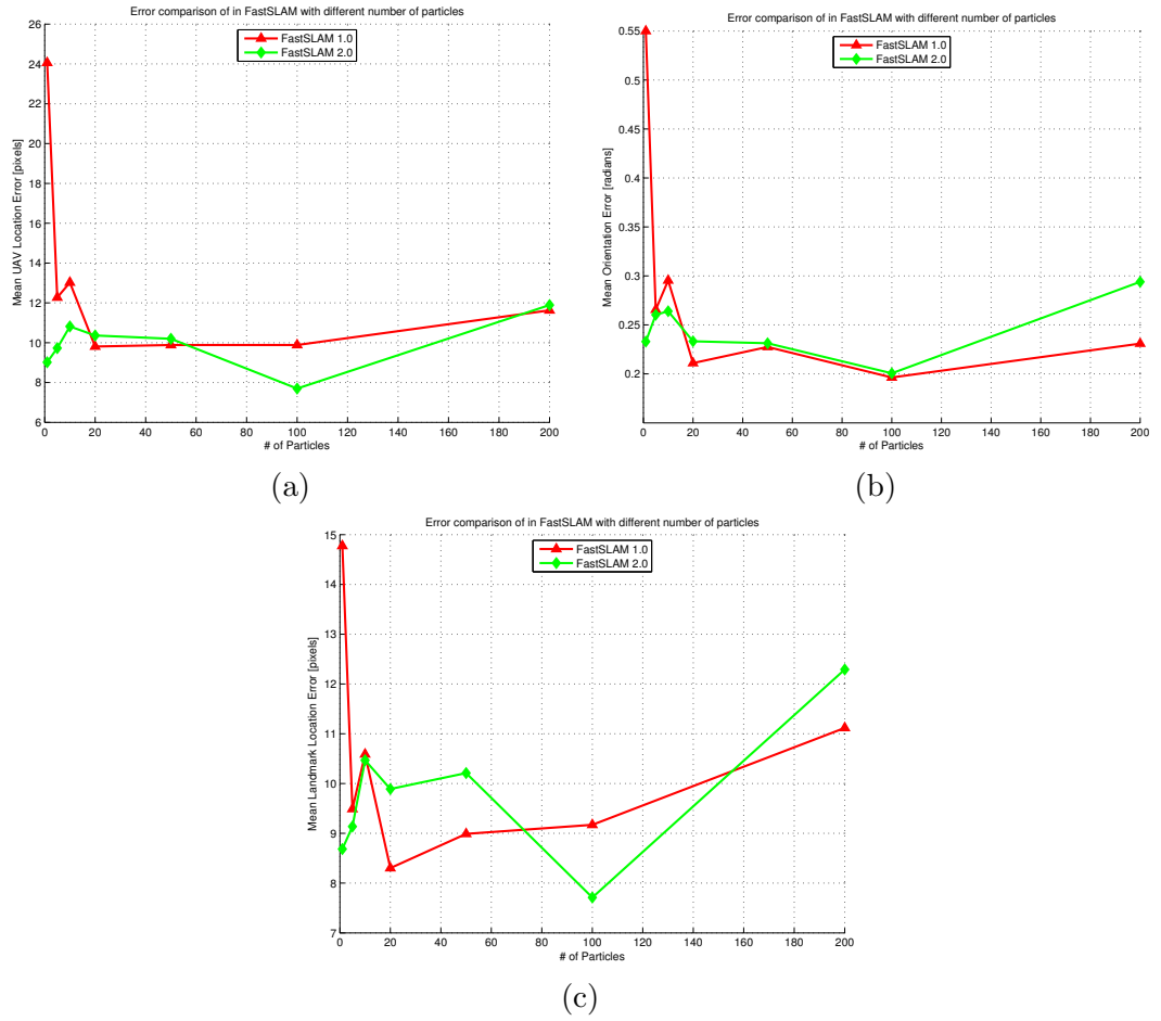
Figure 6.27: Comparison of error levels of the FastSLAM 1.0 and 2.0 algorithms with different number of particles. Part (a) is the error in the estimation of the UAV location, (b) shows the error in estimation of UAV orientation and (c) shows the average landmark position error.
