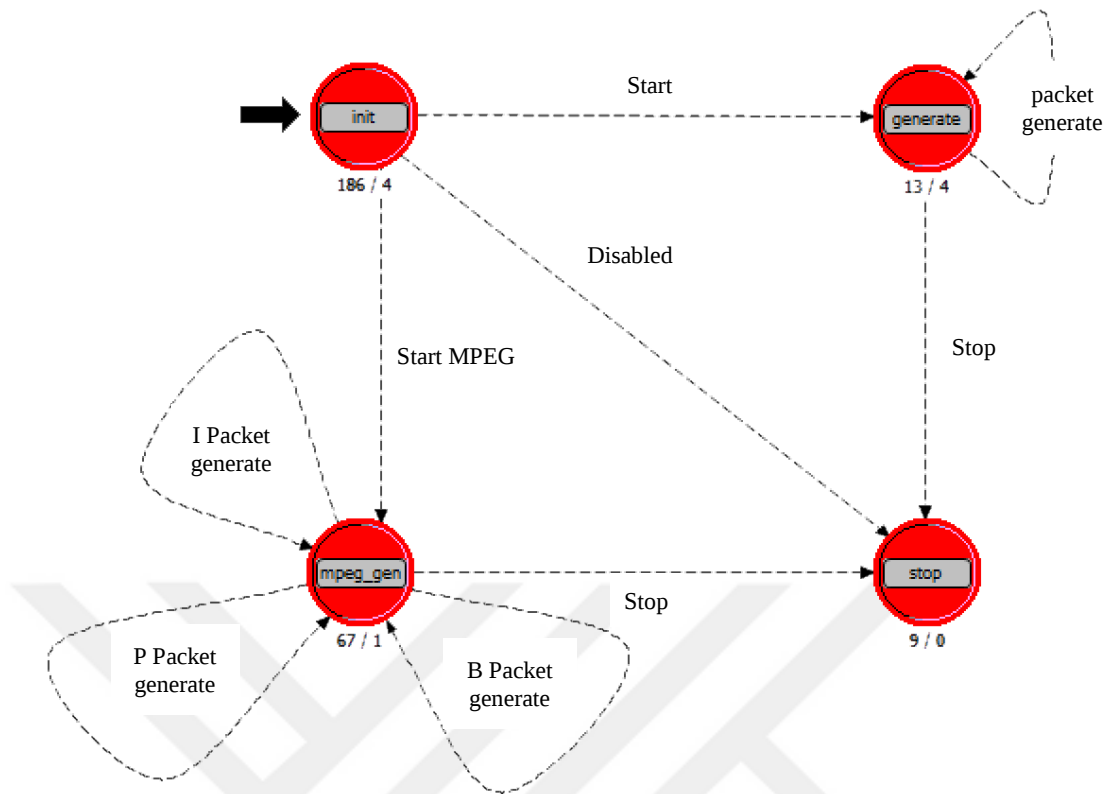
Figure 3.7. Video traffic model OPNET source process module
