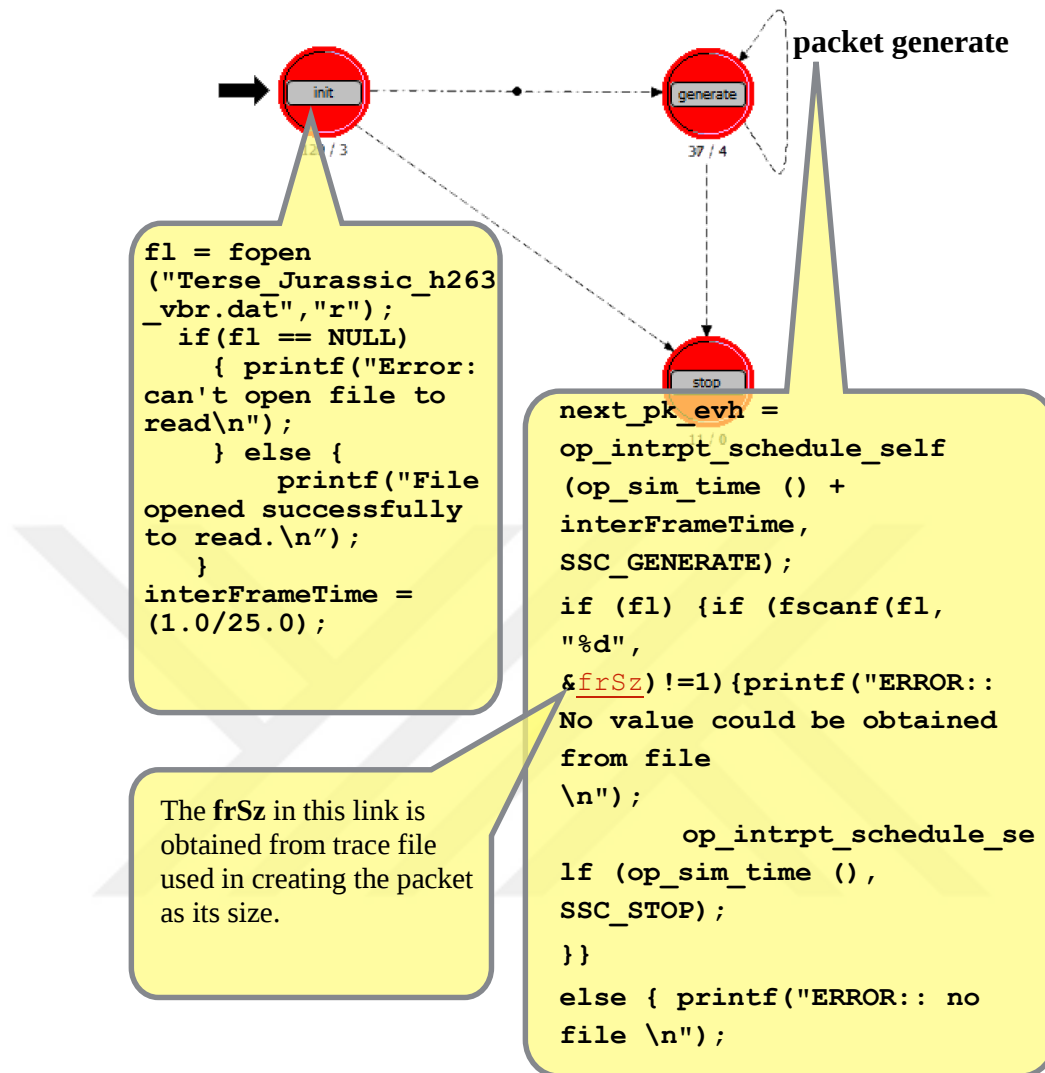
Figure 3.6. OPNET traffic source process module using video frame size trace file
