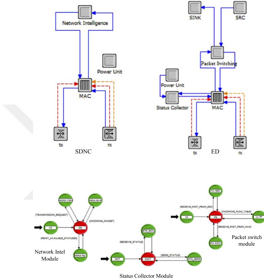
Figure 4.9. Riverbed node models and process models
