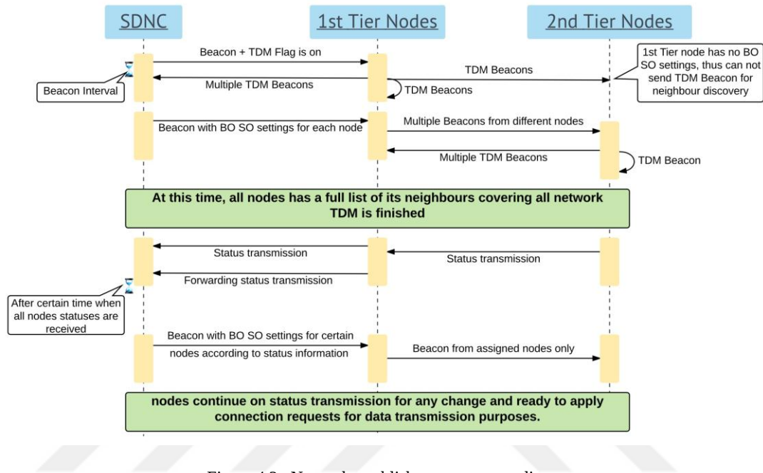
Figure 4.2. Network establishment sequence diagram
