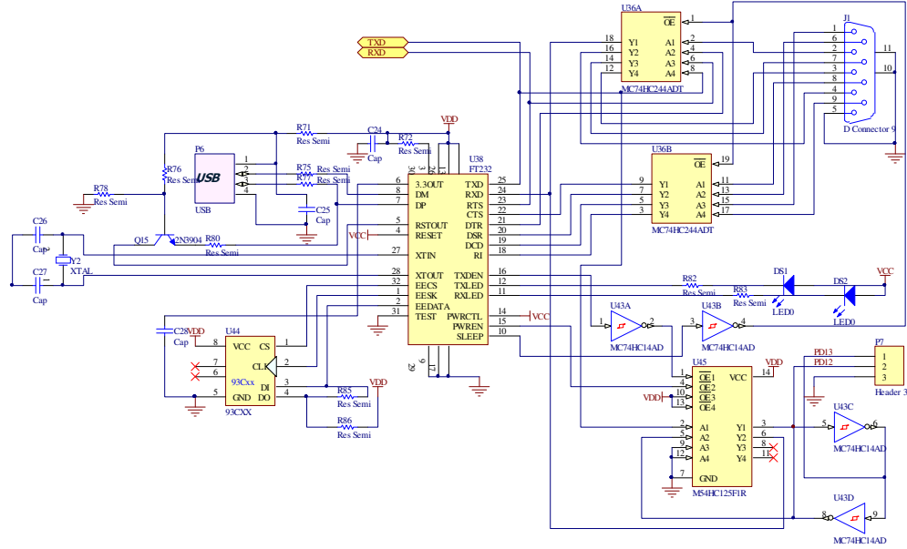
Figure 3.7 USB Part of Design
