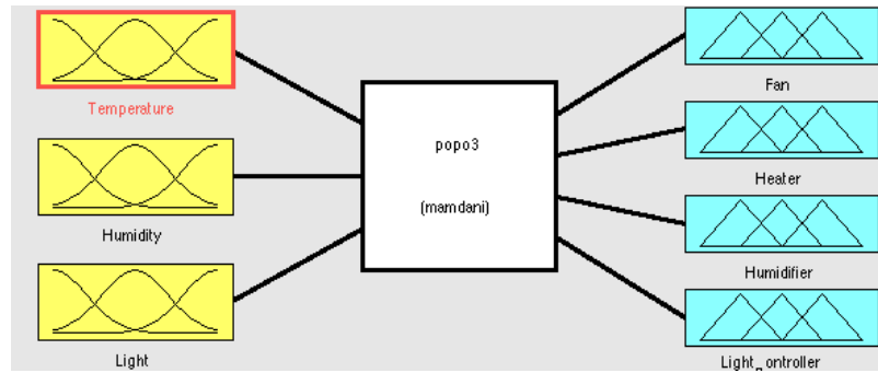
Figure 5.19 Input Output Relation for Greenhouse
