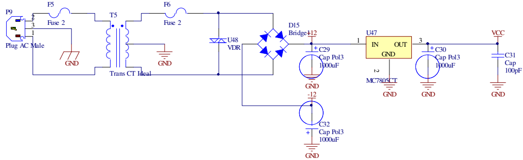
Figure 3.8 Power Part of Design
