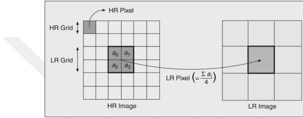
Figure 2.16. Sensor point spread function model [17]
