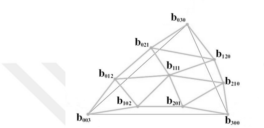
Figure 2.9. 3D view of the control points of a third degree (cubic) Bézier triangle
