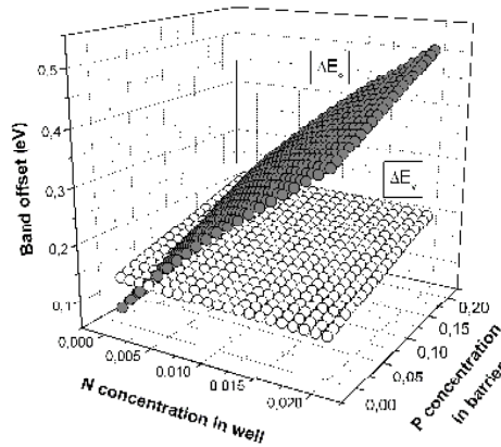
Figure 5.2: The variation of conduction (upper curve) and valance (lower curve) band offsets, \Delta E_c and \Delta E_v , with nitrogen concentration. The strain is compressive in the well whereas it is tension in the barrier of \text{Ga}_{0.70}\text{In}_{0.30}\text{N}_y\text{As}_{1-y}/\text{Ga}_{1-x}\text{AsP}_x/\text{GaAs} QW system.
