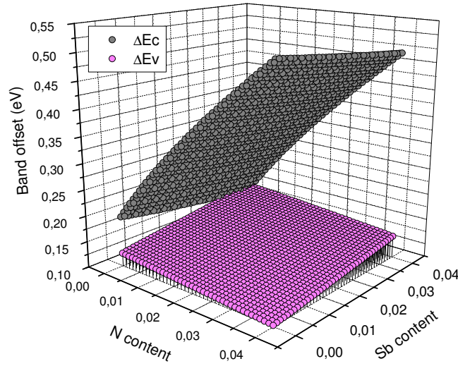
Figure 6.14: The nitrogen and antimonide dependence of valence band offset \Delta E_v and conduction band offset \Delta E_c of the new quinary \text{Ga}_{1-x}\text{In}_x\text{N}_y\text{As}_{1-y-z}\text{Sb}_z /GaAs QW on GaAs substrate.
