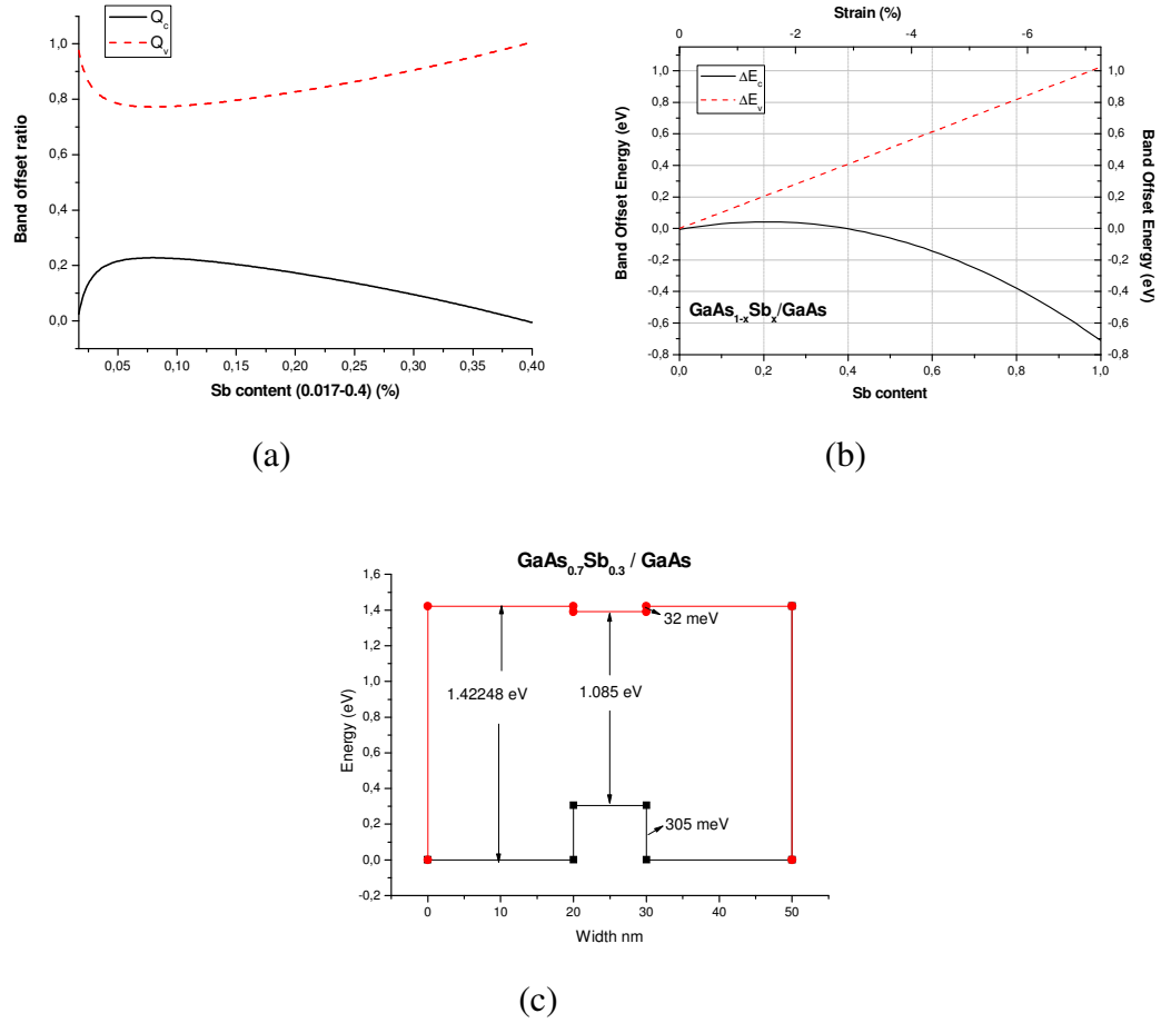
Figure 6.5: The antimony Sb dependence of (a) valence band offset ratio Q_v and conduction band offset ratio Q_c , and (b) conduction band offset \Delta E_c and valence band offset \Delta E_v of \text{GaAs}_{1-x}\text{Sb}_x/\text{GaAs} QWs on GaAs substrates, (c) The band alignment configuration of \text{GaAs}_{0.7}\text{Sb}_{0.3}/\text{GaAs} quantum wells on GaAs substrates.
