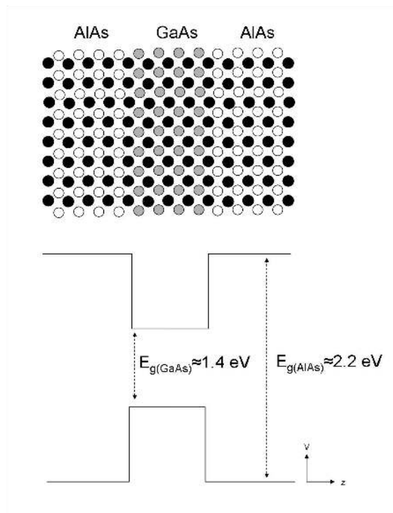
Figure 2.7: Band diagram of AlAs/GaAs heterostructure
