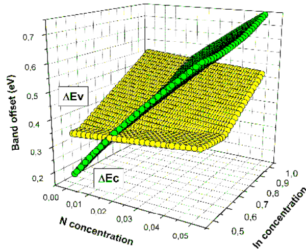
Figure 4.6: The variation of conduction and valence band offsets, \Delta E_c and \Delta E_v , with nitrogen and indium concentration for compressively strained \text{Ga}_{1-x}\text{In}_x\text{N}_y\text{As}_{1-y} quantum wells with InP barrier and InP substrate
