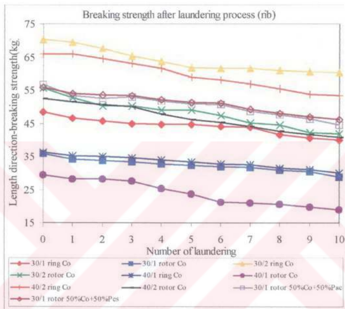
Figure 5.10 Lengthwise direction breaking strength of rib knitted fabrics related to laundering process
