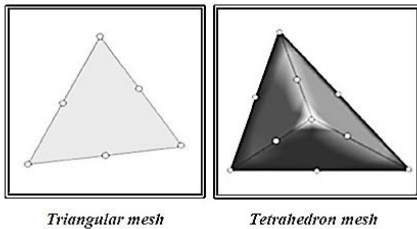
Figure 3.9. Mesh topology
