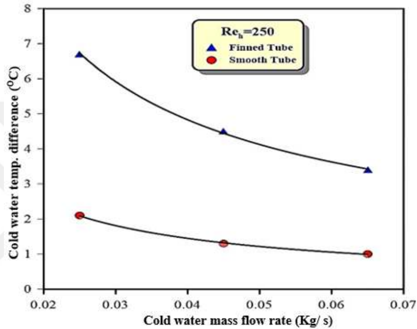
Figure 4.10. Influence of the cold water mass flow rate on the cold water temperature differential at Re_h = 250
