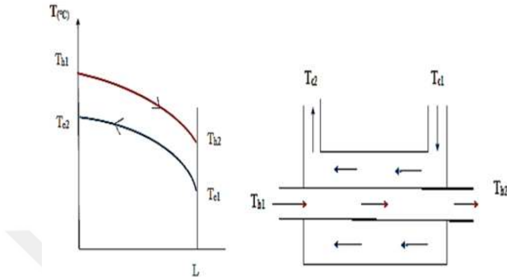
Figure 3.4 The hot and cold fluid direction
