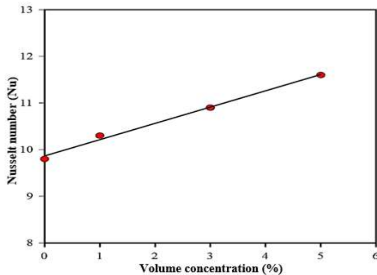
Figure 4.27. Variation of the inner Nusselt number with Alumina-Nano fluid concentrations
