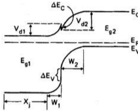
Figure 2.10 Energy band diagram of a typical heterojunction semiconductor in thermal equilibrium [81].
