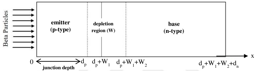
Figure 2.11 Schematic diagram of a heterojunction betavoltaic cell.
