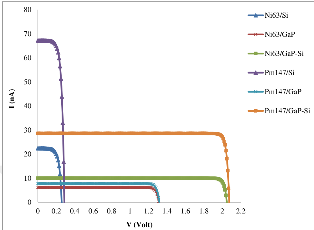
Figure 5.9 Theoretical I–V characteristics of Si, GaP and GaP-Si betavoltaic batteries under 1 mCi/cm 2 Ni63 and Pm147 beta-radiation.
