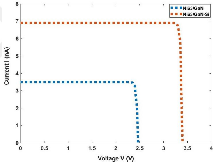
Figure 5.15 Theoretical I-V characteristics of GaN and GaN-Si battery under 1 mCi/cm 2 Ni63 beta-radiation.
