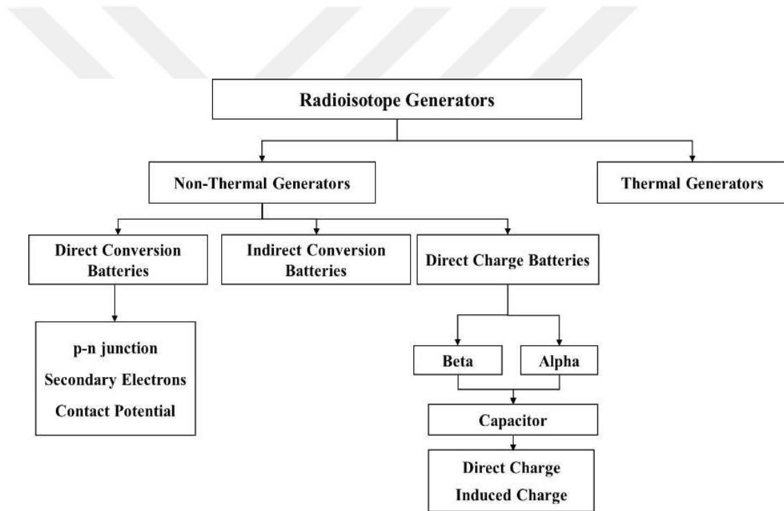
Figure 1.1 Types of nuclear radioisotope generators [20, 23].
