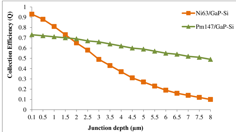
Figure 5.7 Collection efficiency versus the junction depth in the Ni63/GaP-Si and Pm147/GaP-Si n-p betavoltaic battery models.
