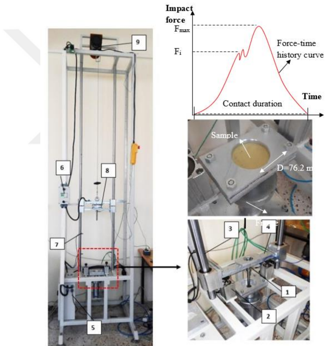
Figure 3.11 Drop weight test machine. (1) Load cell, (2) Rebound breaking system, (3) Guiding rods, (4) Impactor, (5) Control unit, (6) Velocity and time indicator, (7) Optical sensor, (8) Electro-magnet for clamping, (9) Lifting mechanism
