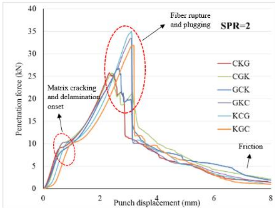
Figure 4.3 Variation of penetration force curves for triple fiber combinations at SPR=2. (a) Non-hybrid composites. (b) Hybrid composites
