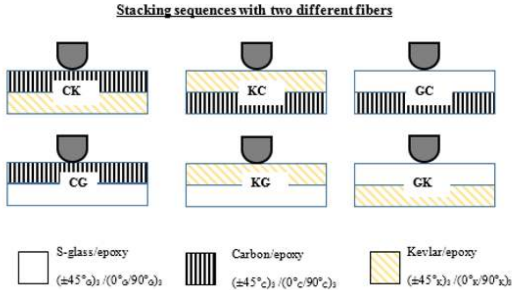
Figure 3.6 Hybrid and non-hybrid configurations of composite laminates for QSI and LVI
