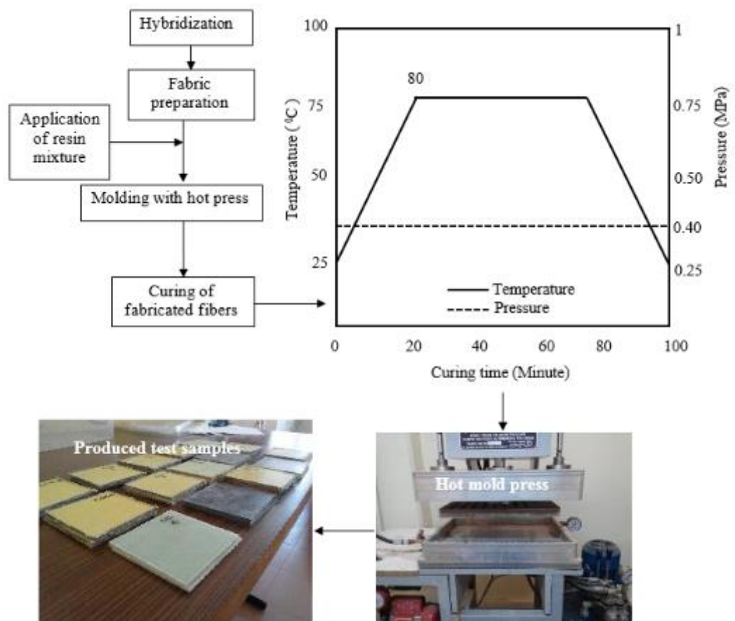
Figure 3.4 Production process
