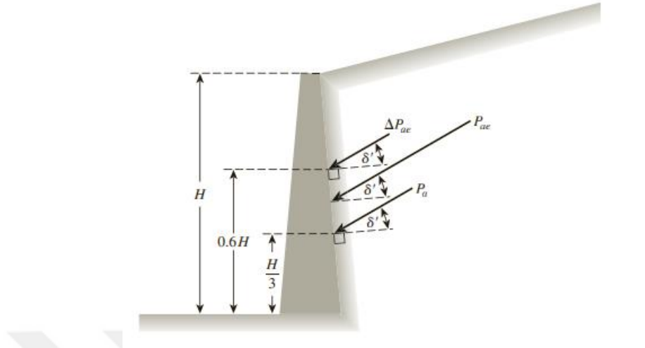
Figure 4.3. Seismic active pressure's point of action (Das and Sobhan, 2018).
