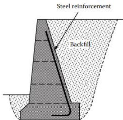
Figure 2.3. Semi-gravity retaining wall (Clayton et al., 2014). Cantilever Retaining Walls
