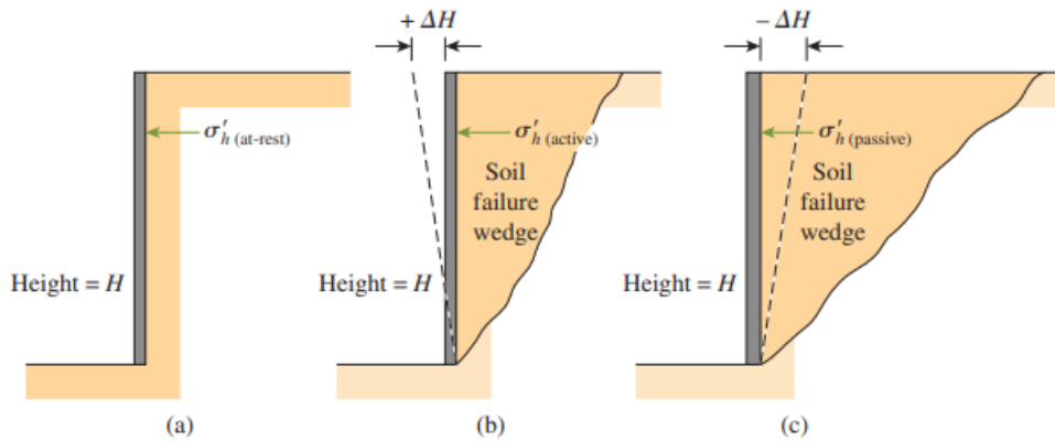
Figure 3.1. The variation of the magnitude of wall movements in the cases of at rest, active and passive situations (Das and Sivakugan, 2018).
