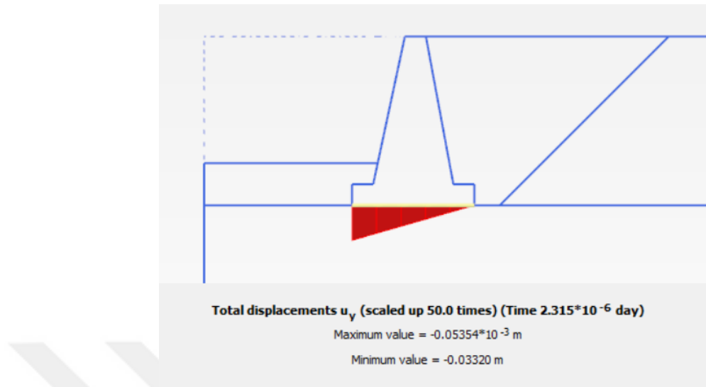
Figure 7.13. Total vertical displacement of the second wall design under dynamic condition.
