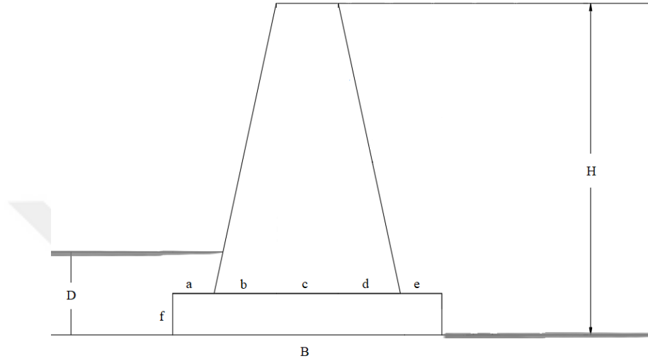
Figure 6.1. Design parameters of the wall model.
