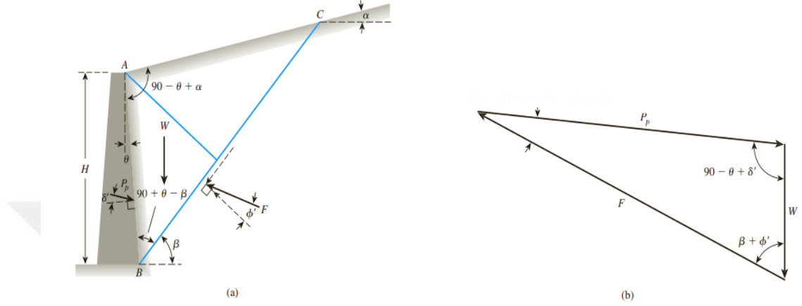
Figure 3.13. Forces included in Coulomb's passive earth pressure (Das and Sobhan, 2018).
