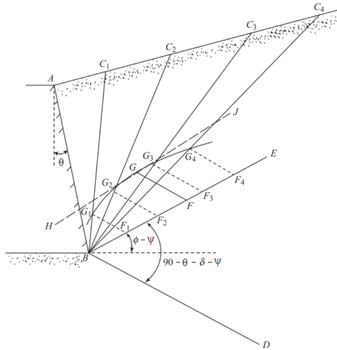
Figure 4.10. Modified Culmann method for estimation of seismic active pressure (Das and Ramana, 2010).
