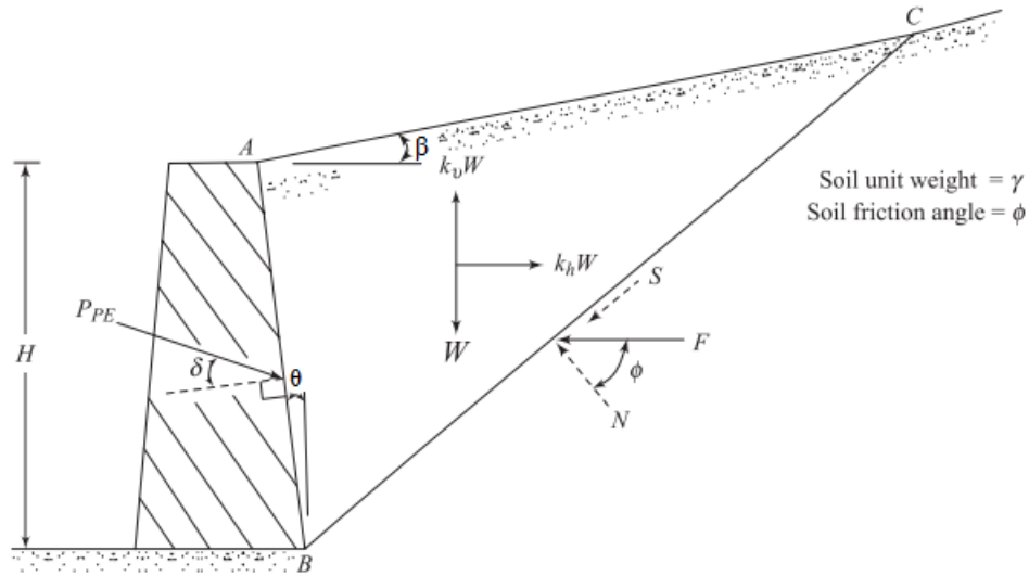
Figure 4.2. Seismic passive earth pressure regarding Mononobe-Okabe (Özcan , 2007).
