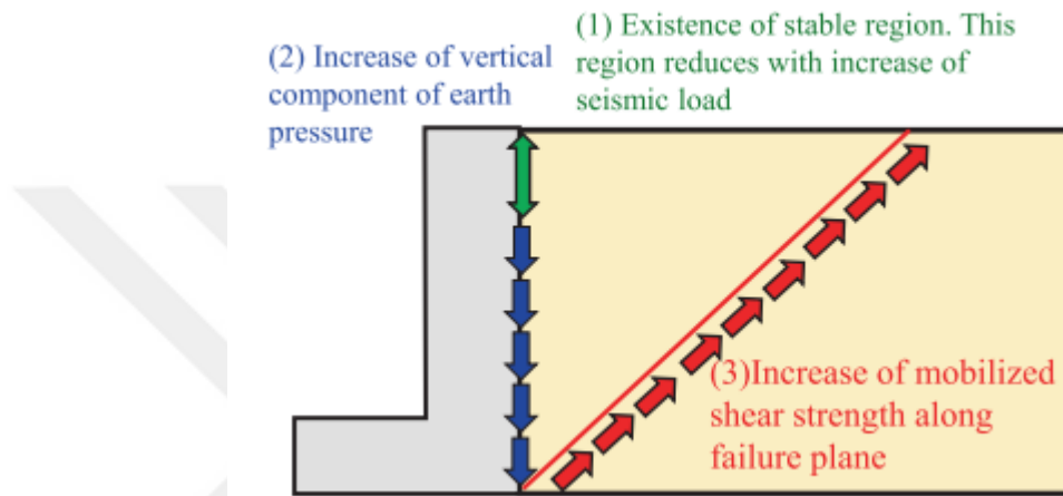
Figure 5.1. Backfill cohesion's impact on seismic stability of retaining walls (Nakajima et al., 2023).
