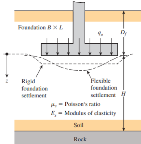
Figure 3.21. Elastic settlement for rigid and footing (Das and Sivakugan, 2018).
