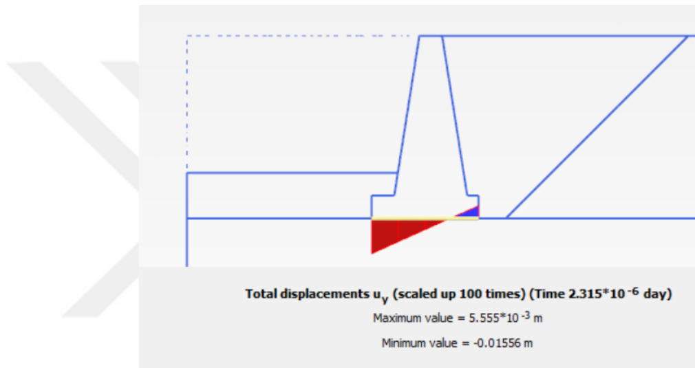
Figure 7.21. Total vertical displacement of the fourth wall design under dynamic condition.
