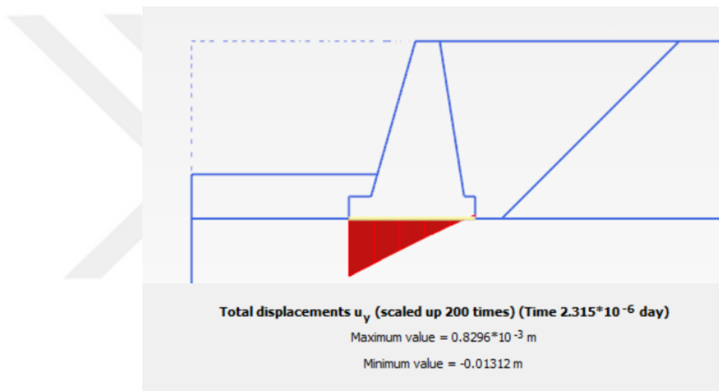
Figure 7.17. Total vertical displacement of the third wall design under dynamic condition.
