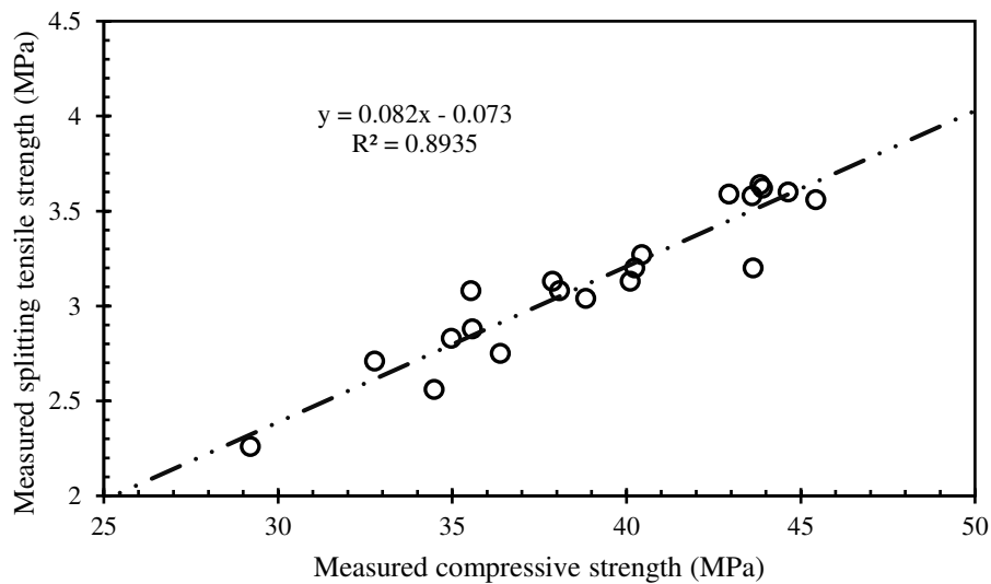
Figure 23: Relationship between compressive strength and splitting tensile strength.
