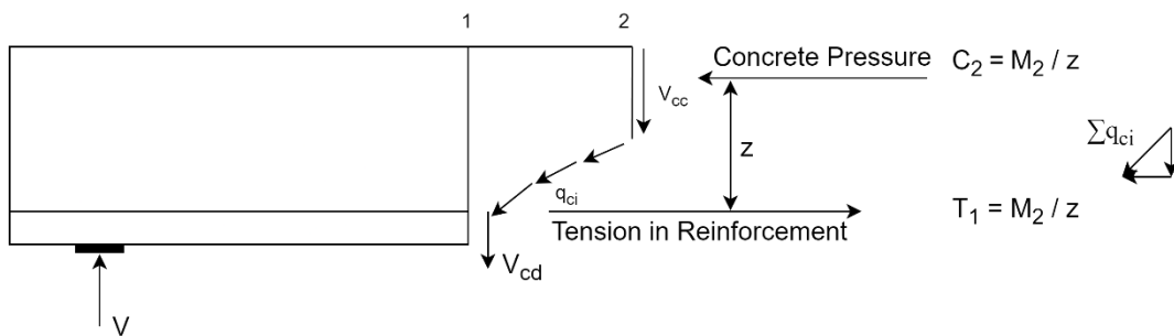
Figure 2.8. Transfer of shear force in reinforced concrete beam(Ersøy et al., 2012)
