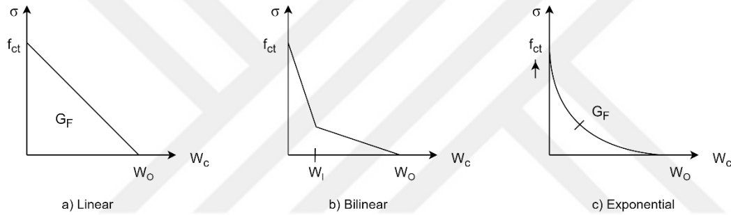
Figure 3.5. Tensile behavior of concrete after cracking (Demir et al., 2016)
