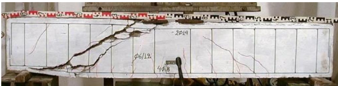
Figure 4.3. Damaged condition of ST120 beam after the test
