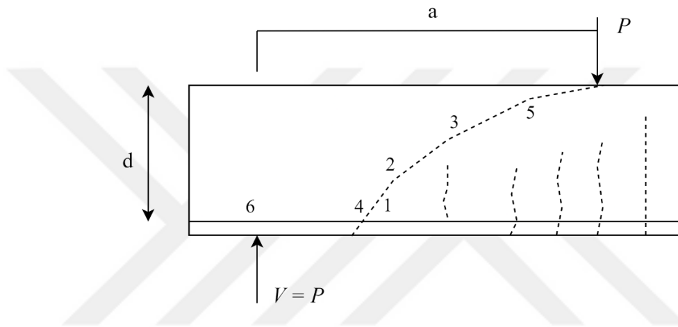
Figure 2.5. Oblique Crack Formation (Ersoy et al., 2012)
