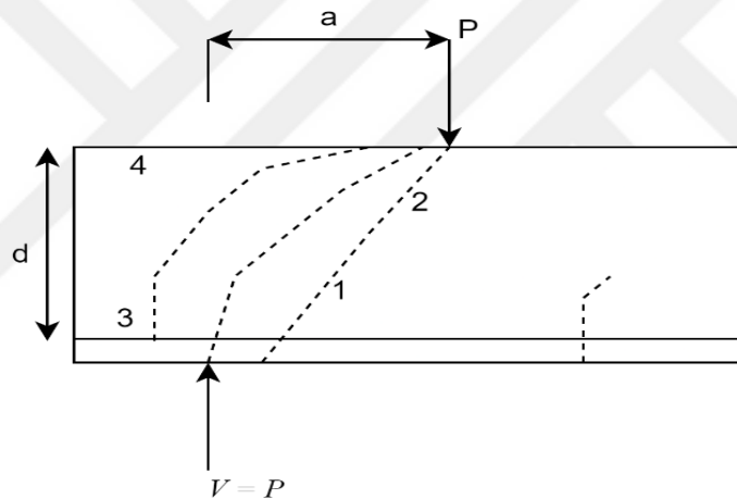
Figure 2.7. Formation of Oblique Cracks (Ersøy et al., 2012)
