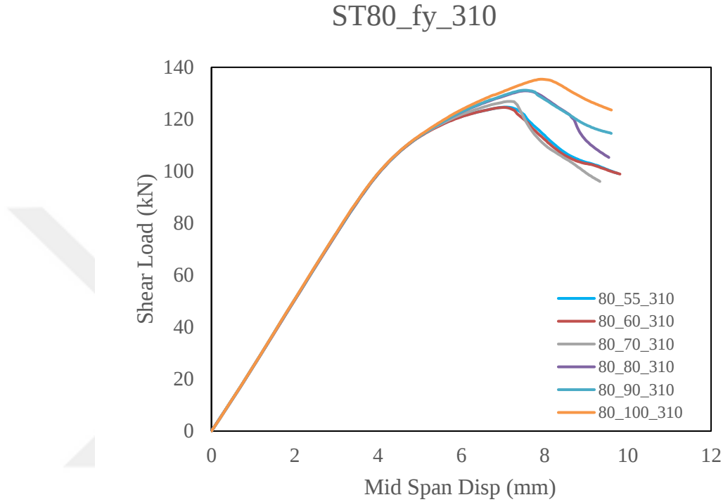
Figure 3.22. ST80 beam element type model results
