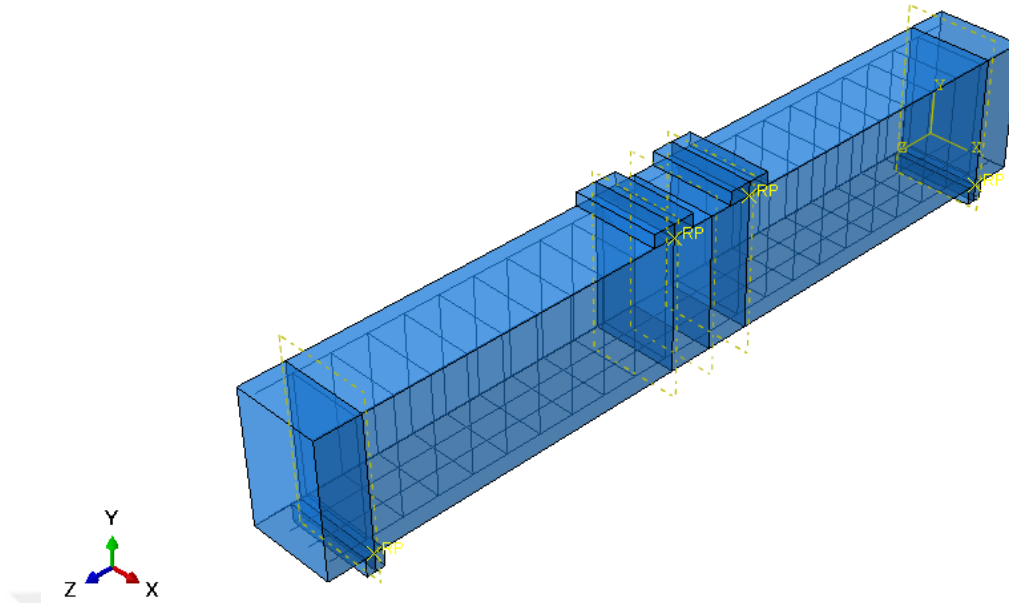
Figure 3.16. Assembly module
