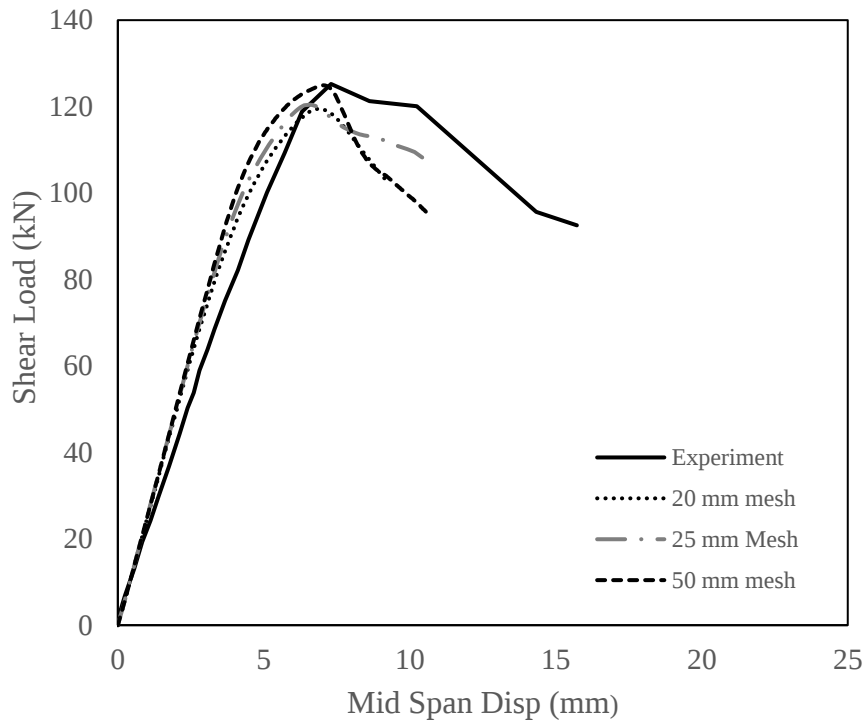
Figure 3.17. Element Size Sensivity Analysis
