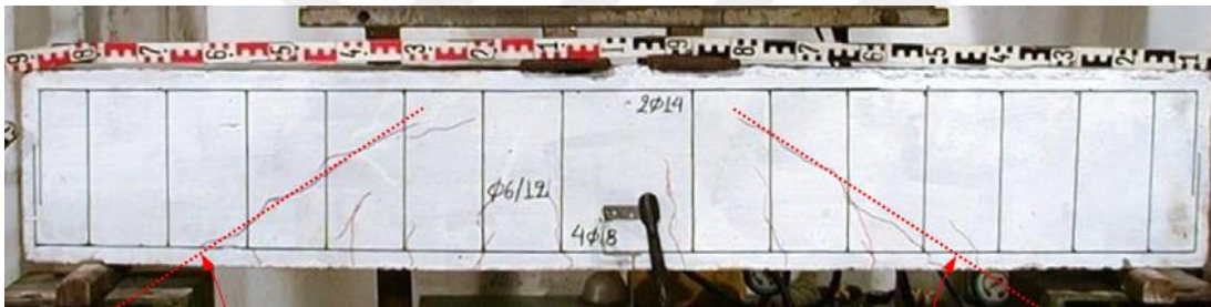
Figure 4.2. Pre-test condition of ST120 beam
