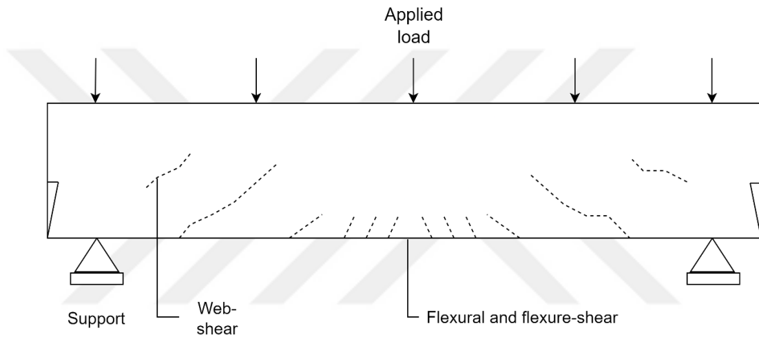
Figure 2.1. Schematic view of cracks in continuous beam (Doğangün, 2019)
