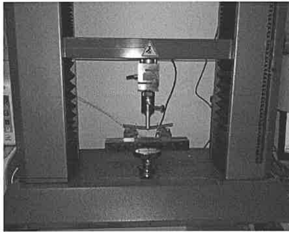
Figure 15. Experimental setup used for the flexural properties tests by
