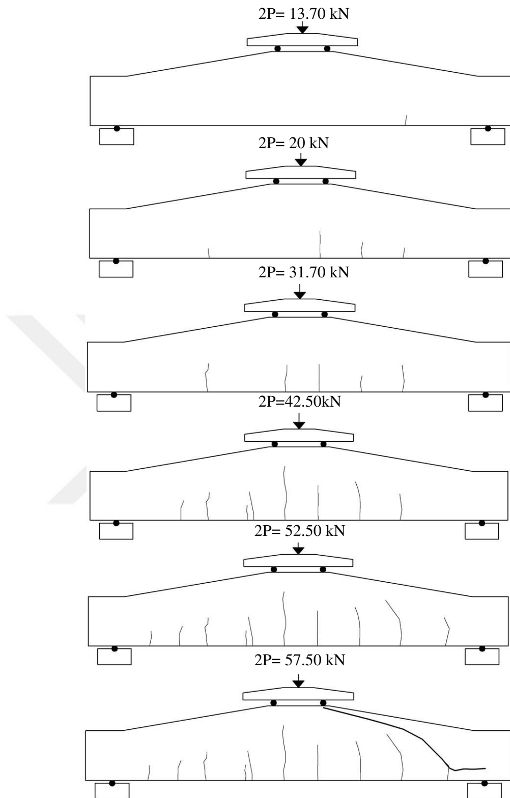
Figure 4.34 Crack Propagation of the Beam (B2-H10-0)
