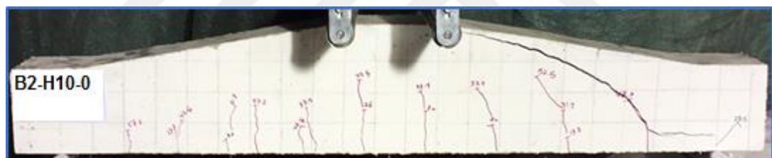
Figure 4.2 Shear Failure for Beam (B2-H10-0)
