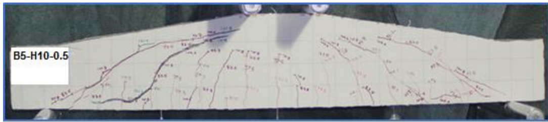
Figure 4.5 Shear Failure for Beam (B5-H10-0.5)
