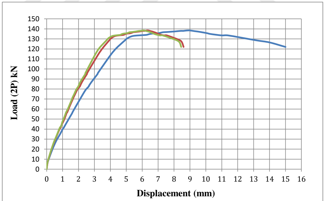
Figure 4.22 Load-Displacement Relationship for the Beam (B9-H15-1) (Haunched Beam at 15^\circ with Steel Fiber 1%)
