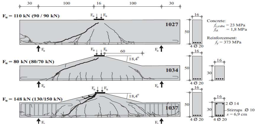
Figure 2.7 Tests Beams Examined by Mörsch (1922) [Adapted from Nghiep (2011)]
