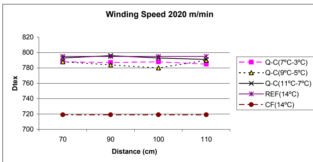
Figure 5.29 Count – Distance Effect (2020 m/min winding speed)
