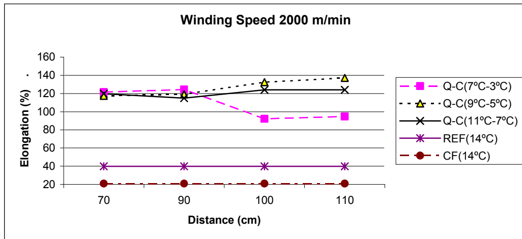
Figure 5.17 Elongation – Distance Effect (2000 m/min winding speed)
