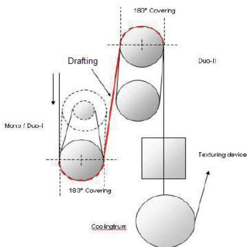
Figure 2.13 Drafting rollers [33]
