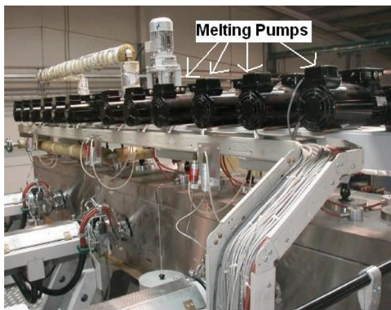
Figure 2.8 Spinning pump [31]
