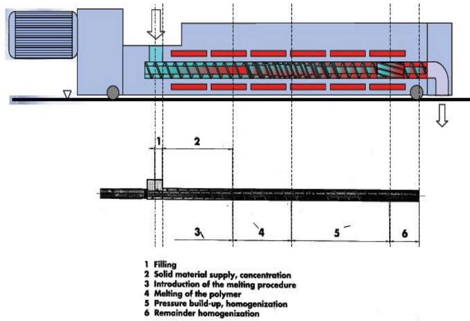
Figure 2.7 Extruder model [32,33]
