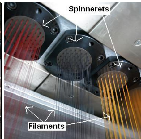
Figure 2.9 Spinnerets[31]
