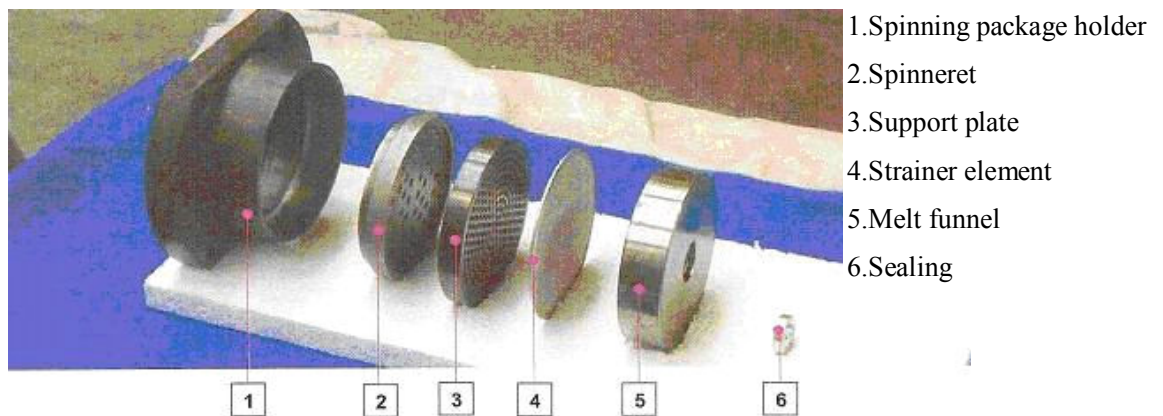
Figure 4.3 Components of the spinning package [42]
