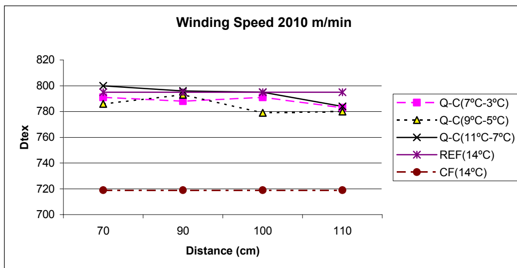
Figure 5.28 Count – Distance Effect (2010 m/min winding speed)
