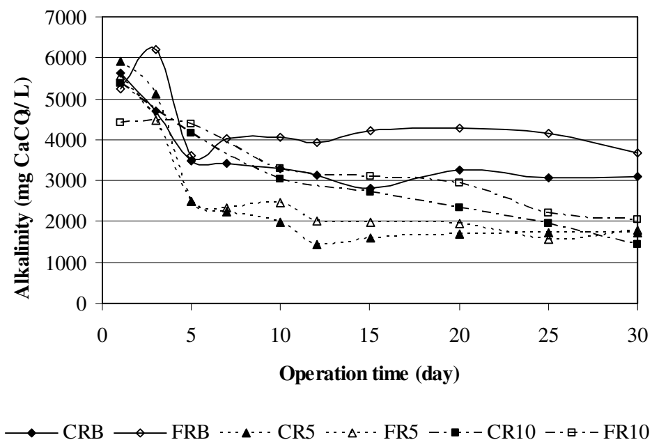
Figure 4.7 Total alkalinity changes in reactor contents of \text{CR}_B , \text{FR}_B , \text{CR}_5 , \text{FR}_5 , \text{CR}_{10} , and \text{FR}_{10} during operation period
