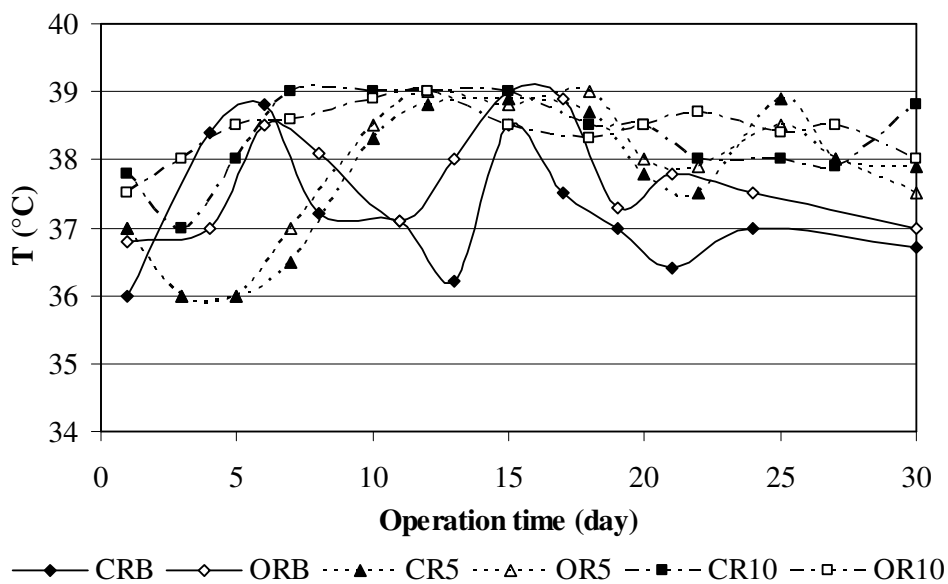
Figure 4.38 Temperature changes in reactor contents of \text{CR}_\text{B} , \text{OR}_\text{B} , \text{CR}_5 , \text{OR}_5 , \text{CR}_{10} , and \text{OR}_{10} during operation period
