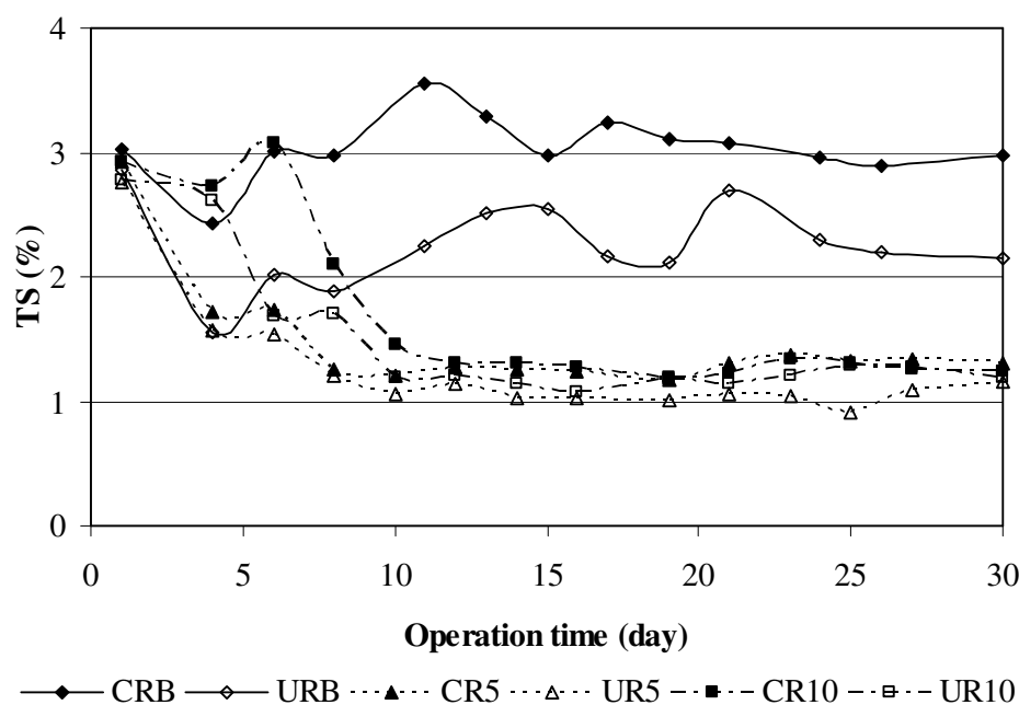
Figure 4.60 Total solids changes in reactor contents of \text{CR}_B , \text{UR}_B , \text{CR}_5 , \text{UR}_5 , \text{CR}_{10} , and \text{UR}_{10} during operation period
