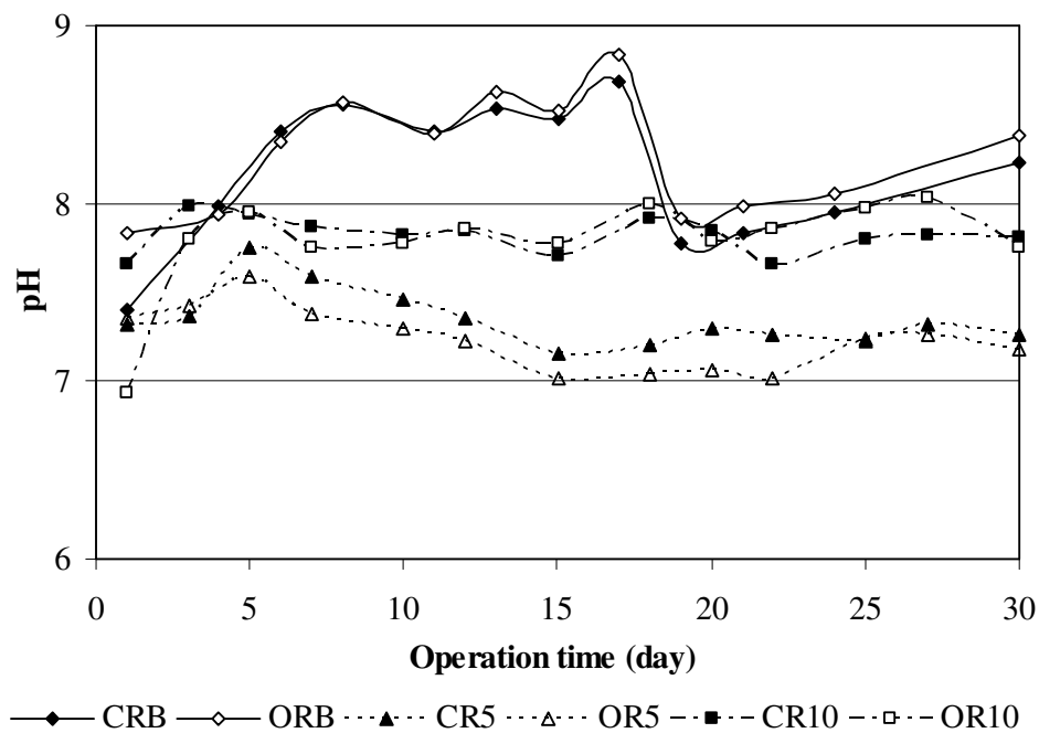
Figure 4.39 pH changes in reactor contents of \text{CR}_\text{B} , \text{OR}_\text{B} , \text{CR}_5 , \text{OR}_5 , \text{CR}_{10} , and \text{OR}_{10} during operation period
