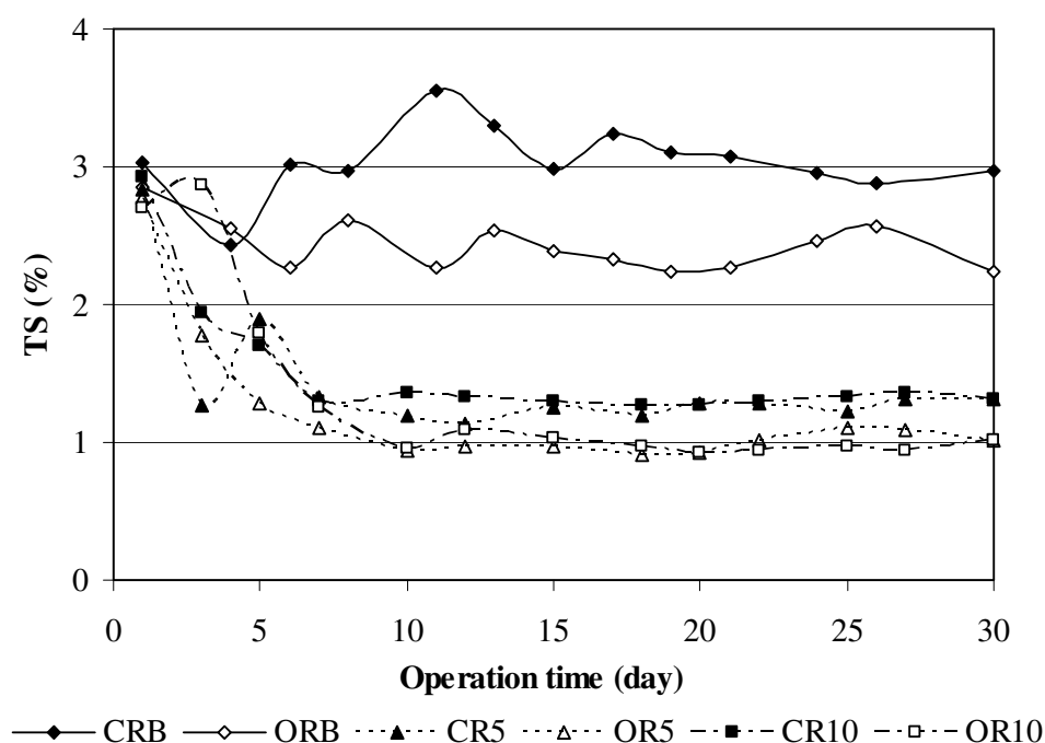
Figure 4.41 Total solids changes in reactor contents of CR B , OR B , CR 5 , OR 5 , CR 10 , and OR 10 during operation period
