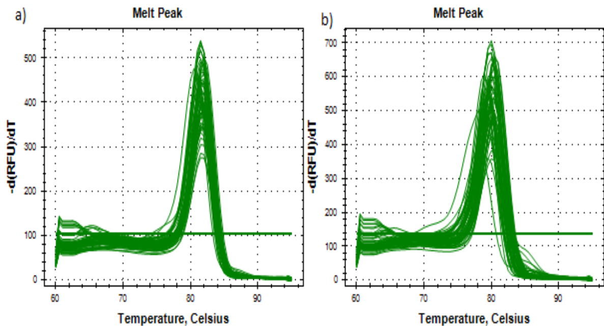
Figure 4.3. qPCR results of hsa-mir-192. Both Figures show that expression was successful, but there is no difference between methylated and unmethylated, benign and malign samples. These peaks represent a normal distribution. The normal distribution is symmetric and has a bell-shaped curve with a single peak. a) methylated, b) unmethylated
