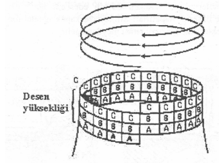
Figure 3.16 Helical positions of rows in a fabric with three feeders [19]
