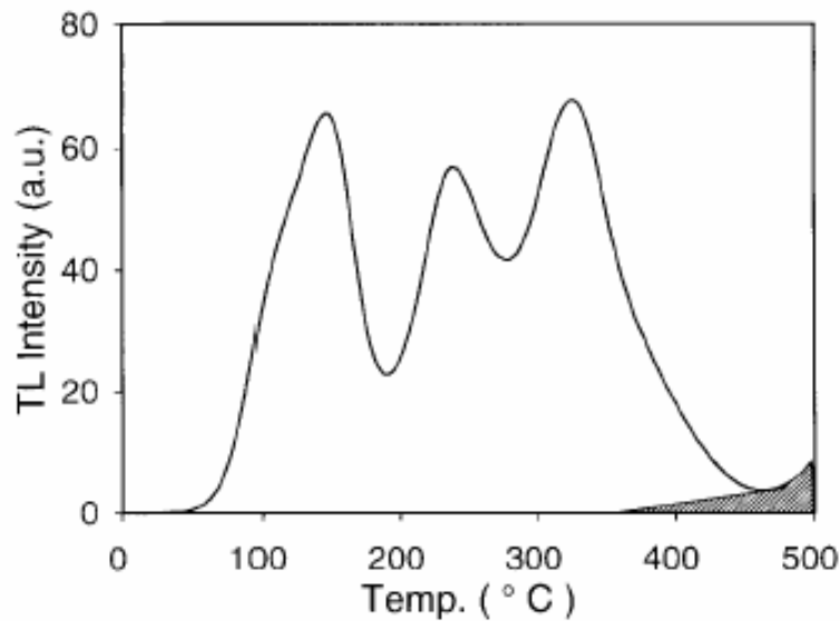
Figure 2.2 Typical TL glow curve from a sedimentary K-feldspar sample given a beta dose of 8 Gy in addition to the natural dose (approximately 200 Gy). The 150°C peak evident in this figure has been created by the recent beta dose; it is not usually evident in the natural signal as it has normally decayed away. The shaded area is the background radiation observed when the sample is heated a second time with no additional irradiation [15]
