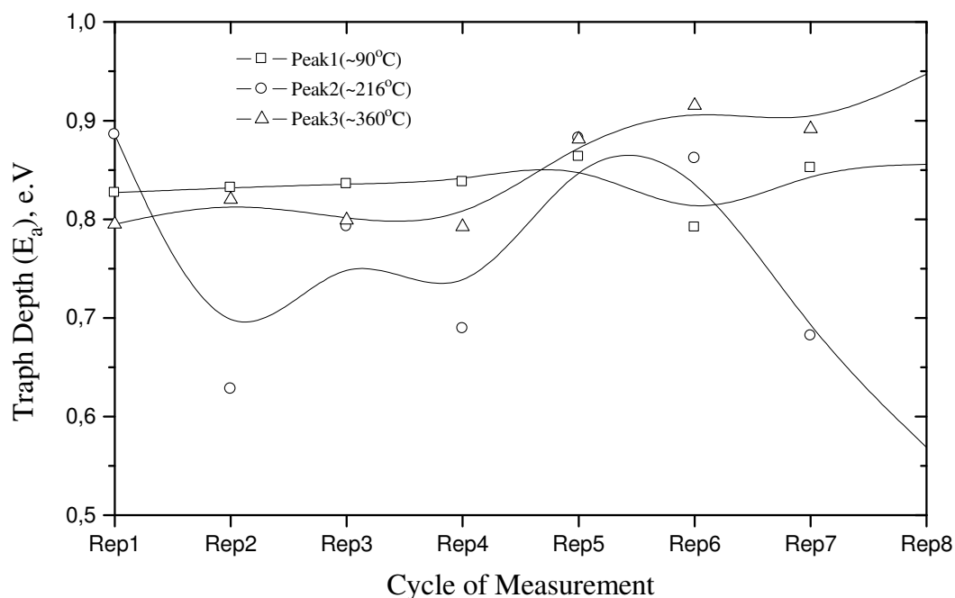
Figure 5.11 The effect of experimental cycles on the trap depth ( E_a ) of traps of TL peaks of annealed quartz sample at 500 °C for 1h.
