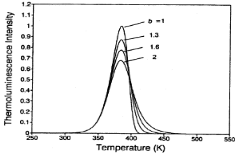
Figure 2.5 Comparison of first-order ( b=1 ), second-order ( b=2 ) and intermediate-order ( b=1.3 and 1.6 ) TL peaks, with E=1 eV, s=1 \times 10^{12} \text{ s}^{-1} , n_0=N=1 \text{ m}^{-3} and \beta=1 \text{ K/s} (from [21])
