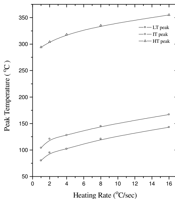
Figure 5.48 The alteration in the peak temperatures of glow peaks of unannealed synthetic quartz samples versus heating rates
