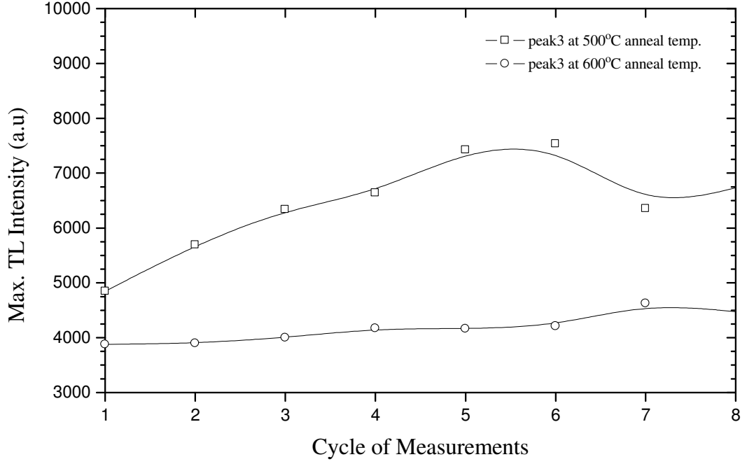
Figure 5.10 The variation of maximum TL intensity ( I_m ) of peak 3 of annealed quartz sample at 500 and 600 °C for 1 h with respect to cycle of measurement
