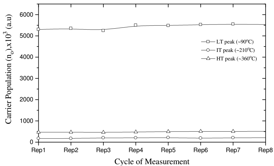
Figure 5.14 The effect of experimental cycles on the carrier populations ( n_o ) in traps of TL peaks of annealed quartz sample at 600 °C for 1 h.
