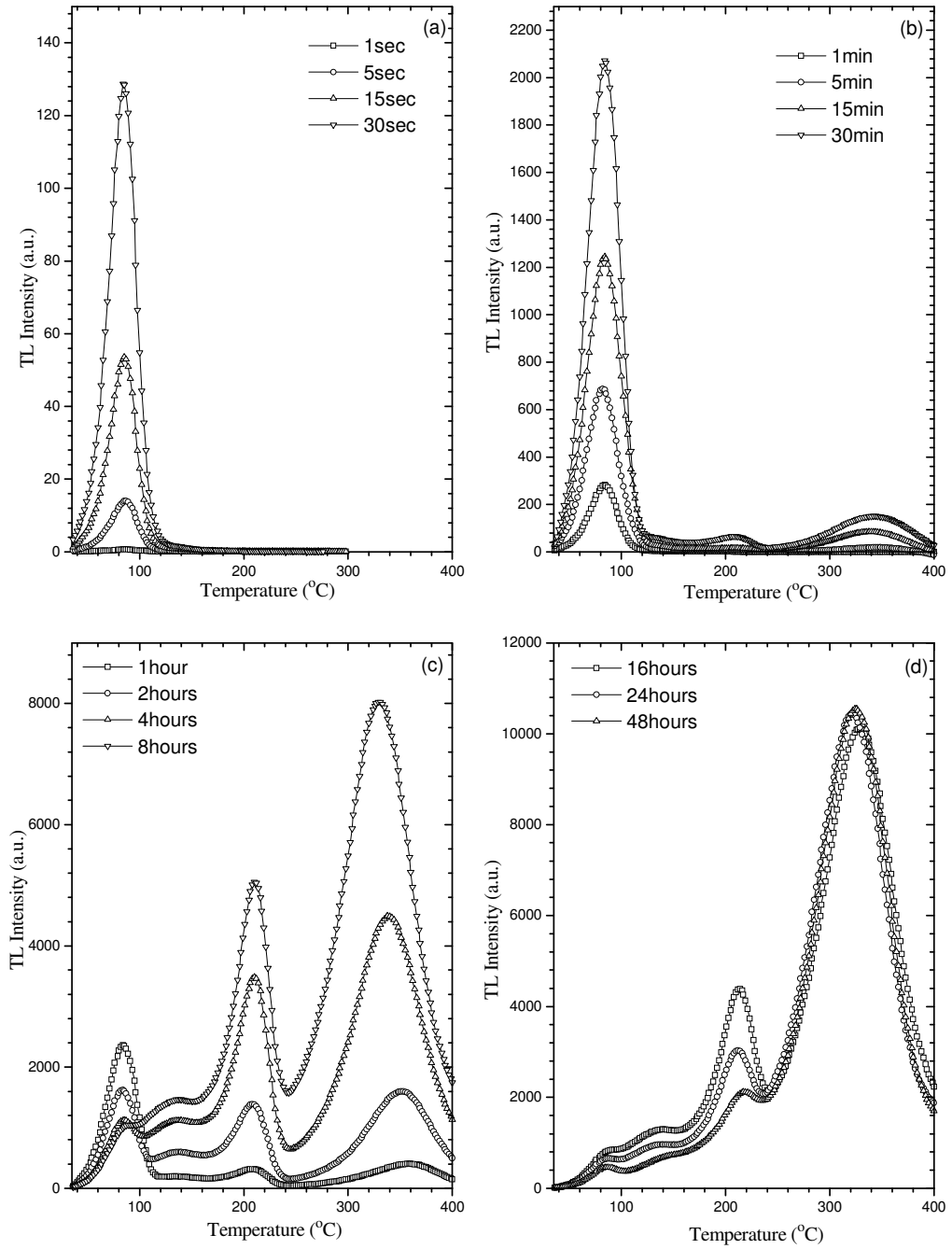
Figure 5.36 The variation of intensities of TL glow curves of one unannealed natural quartz samples after different dose levels
