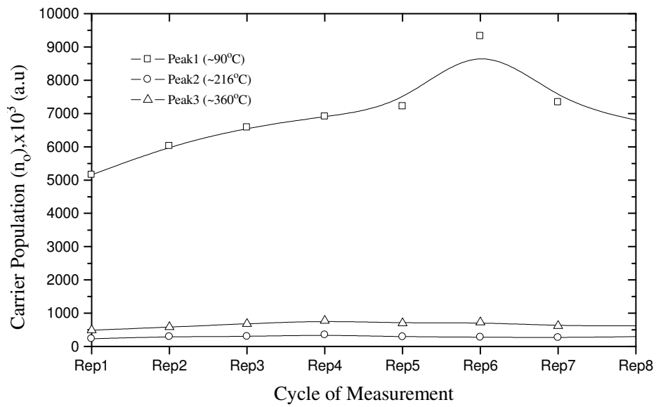
Figure 5.13 The effect of experimental cycles on the carrier populations ( n_o ) in traps of TL peaks of annealed quartz sample at 500 °C for 1 h.
