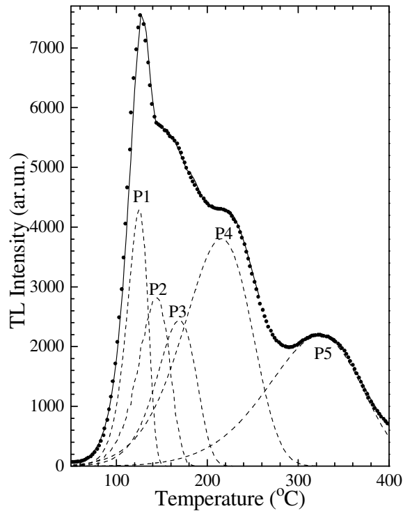
Figure 5.1 A typical analysed glow curve of annealed quartz at 600 °C for 1 h measured after \approx 30 Gy irradiation at RT. The glow curve was measured by heating the sample to 400 °C at a heating rate of 1^\circ\text{C s}^{-1} . In the figure, solid circles represent the experimental points
