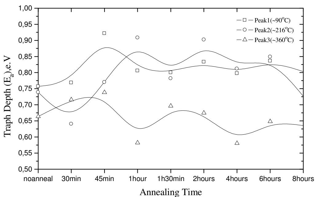
Figure 5.19 The effect of annealing time on the trap depth ( E_a ) of traps of TL peaks of quartz sample after annealing at 600 °C
