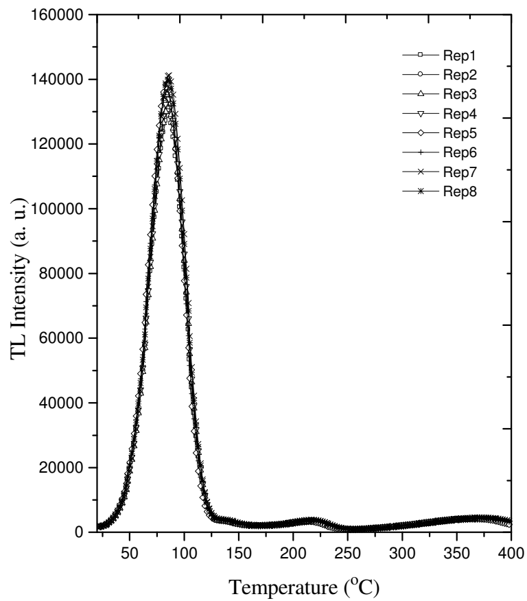
Figure 5.7 The variation of intensities of TL glow curves of annealed natural quartz sample at 600 ^\circ\text{C} for 1 h with cycles of measurements
