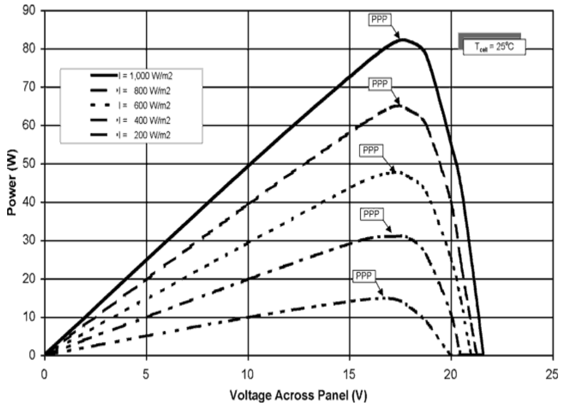
Figure 4.5 Power output of a photovoltaic panel at different levels of solar irradiance. The notation PPP defines the peak power point. Data is for a cell temperature of 25°C and an air mass of 1.5
