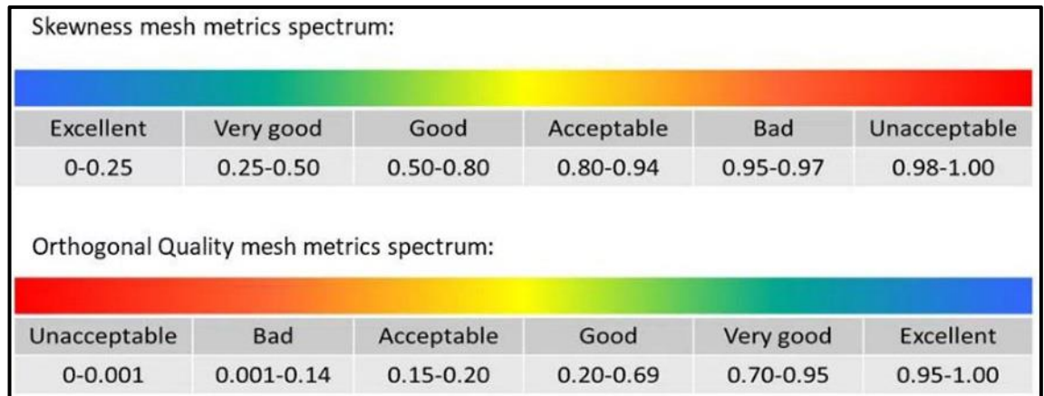
Figure 3.12 Mesh quality
