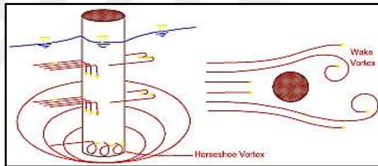
Figure 2.1 Around a cylindrical pier, there are horseshoe and wake vortices (Ipa and Di 2017)
