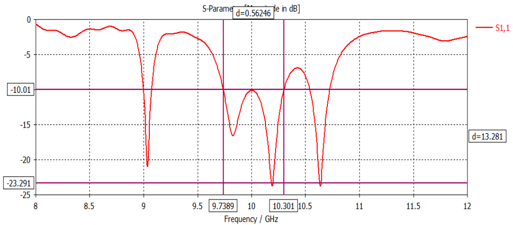
Figure 5.11: Slot Length 10 mm Return Loss
