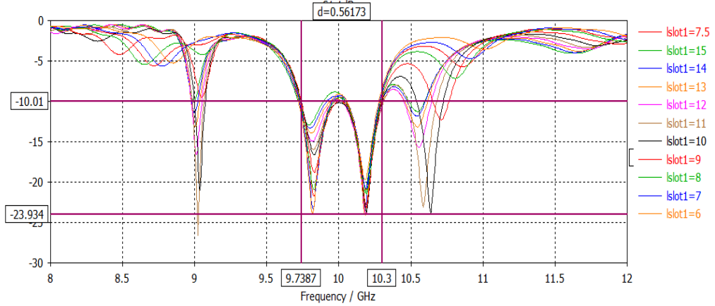
Figure 5.10: Variation Length of Slot
