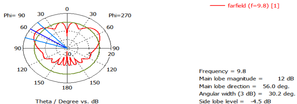
Figure 5.29: Radiation Pattern at 9.8 GHz
