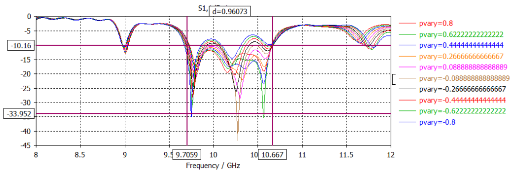
Figure 5.40: Varying Position of Slot
