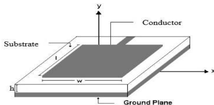
Figure 1.1: Microstrip Patch Antenna Cofiguration
