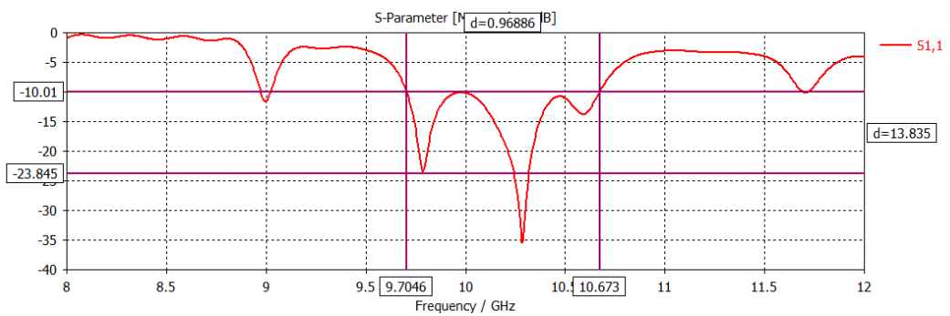
Figure 5.37: Return Loss
