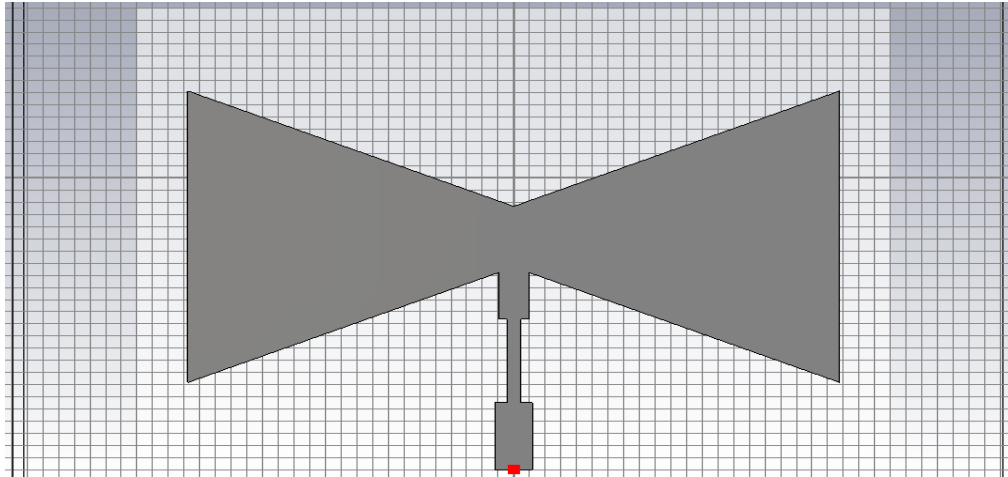
Figure 3.1: Bowtie Antenna
