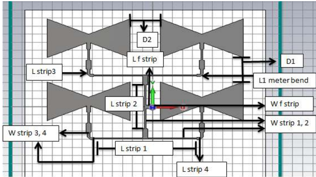
Figure 5.5: 2 \times 2 Bowtie Patch Antenna Array
