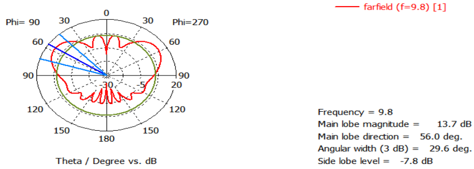
Figure 5.25: 2D Radiation Pattern
