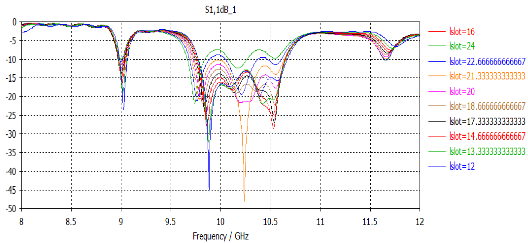
Figure 5.30: Variation Length of Slot
