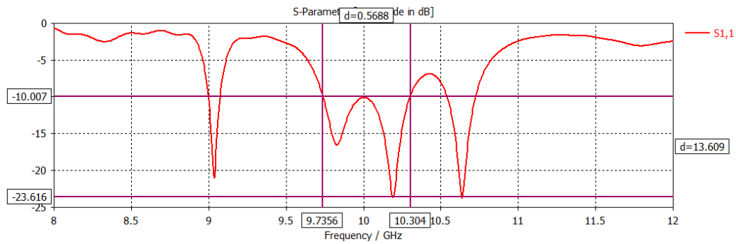
Figure 5.14: Return Loss
