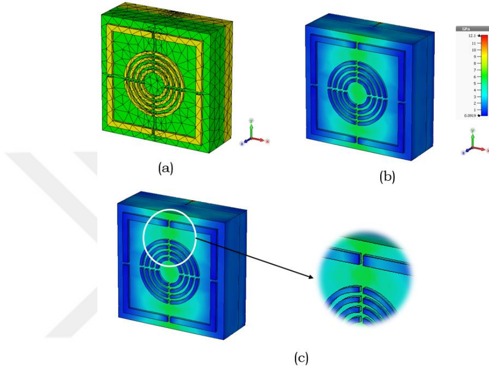
Figure 7.3 Meshed view (a), Von Mises stress view (b) and the place that maximum Von Mises stresses occurred view of the wide-band absorber (c)
