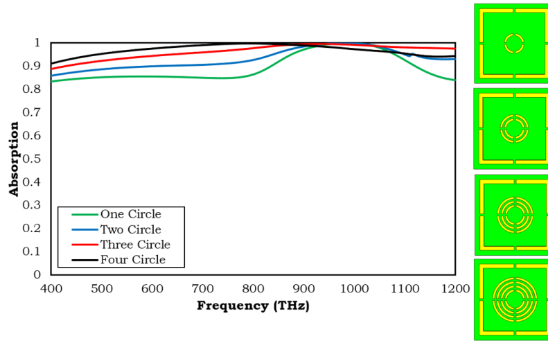
Figure 7.4 Absorption curves of the one, two, three, and four circled simulations of the wide-band absorber in the visible and ultraviolet frequency range (400-1200 THz)
