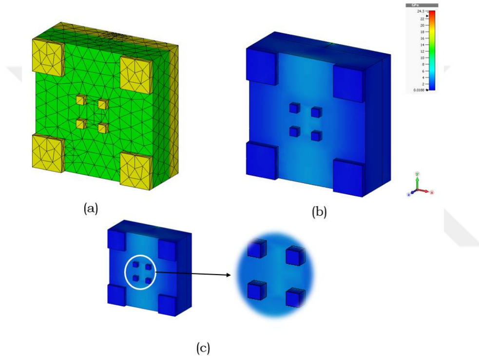
Figure 6.3 Meshed view (a), Von Mises stress view (b) and the place that maximum Von Mises stresses occurred view of the square-strip MTM absorber design (c)
