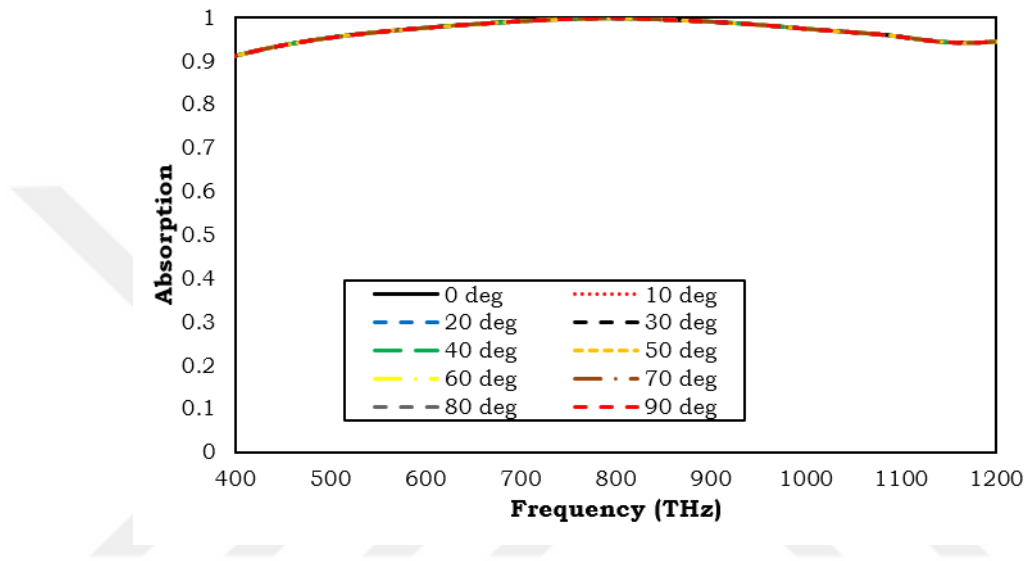
Figure 7.6 Absorption response of the wide-band absorber for different polarization angles under normal incidence mode of the electromagnetic radiation
