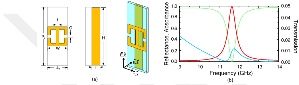
Figure 2.4 Unit cell design of “Perfect Metamaterial Absorber” (a), and frequency response of the design (b), red color represents absorption, light green color represents reflection, transmission represented with light blue color [48]
