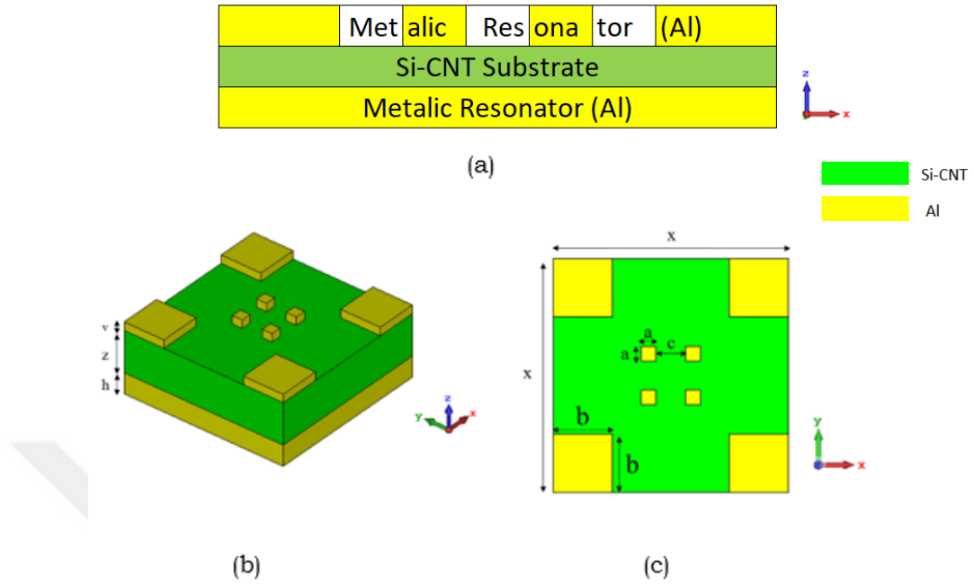
Figure 6.1 Side view (a), isometric view (b), and front view (c) of the square-strip MTM structure
