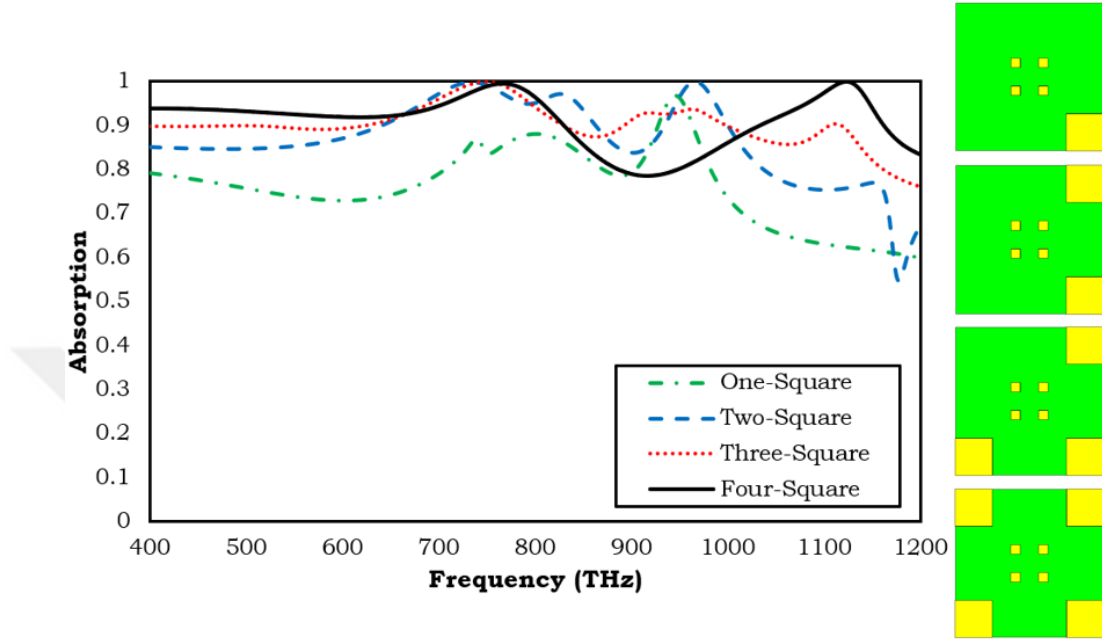
Figure 6.4 Absorption curves of the one, two, three, and four squares with center patch in the visible and ultraviolet frequency range (400-1200 THz)
