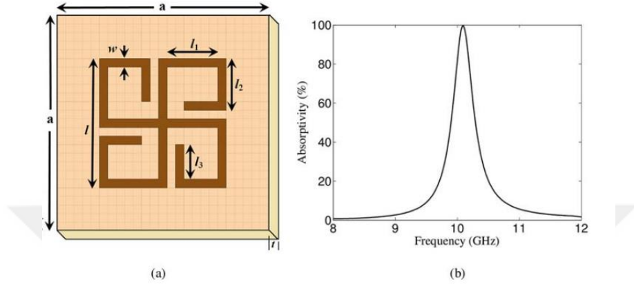
Figure 2.5 Structural representation (a), simulation results (b) of ultrathin polarization-insensitive microwave absorber design [49]
