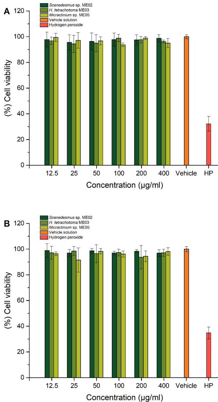
Figure 4.3 The viability of (A) HeLa and (B) MCF-7 cells after 48 h incubation with various concentrations of microalgal extracts.
