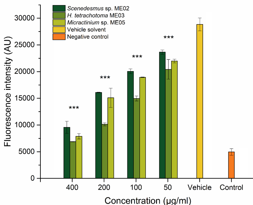
Figure 4.4 Inhibitory effects of the microalgal extracts on intracellular ROS generation in H 2 O 2 -induced MCF-7 cells. All values are represented as mean \pm SD (n =3). Asterisks indicate the significance of the samples with respect to the vehicle solution.
