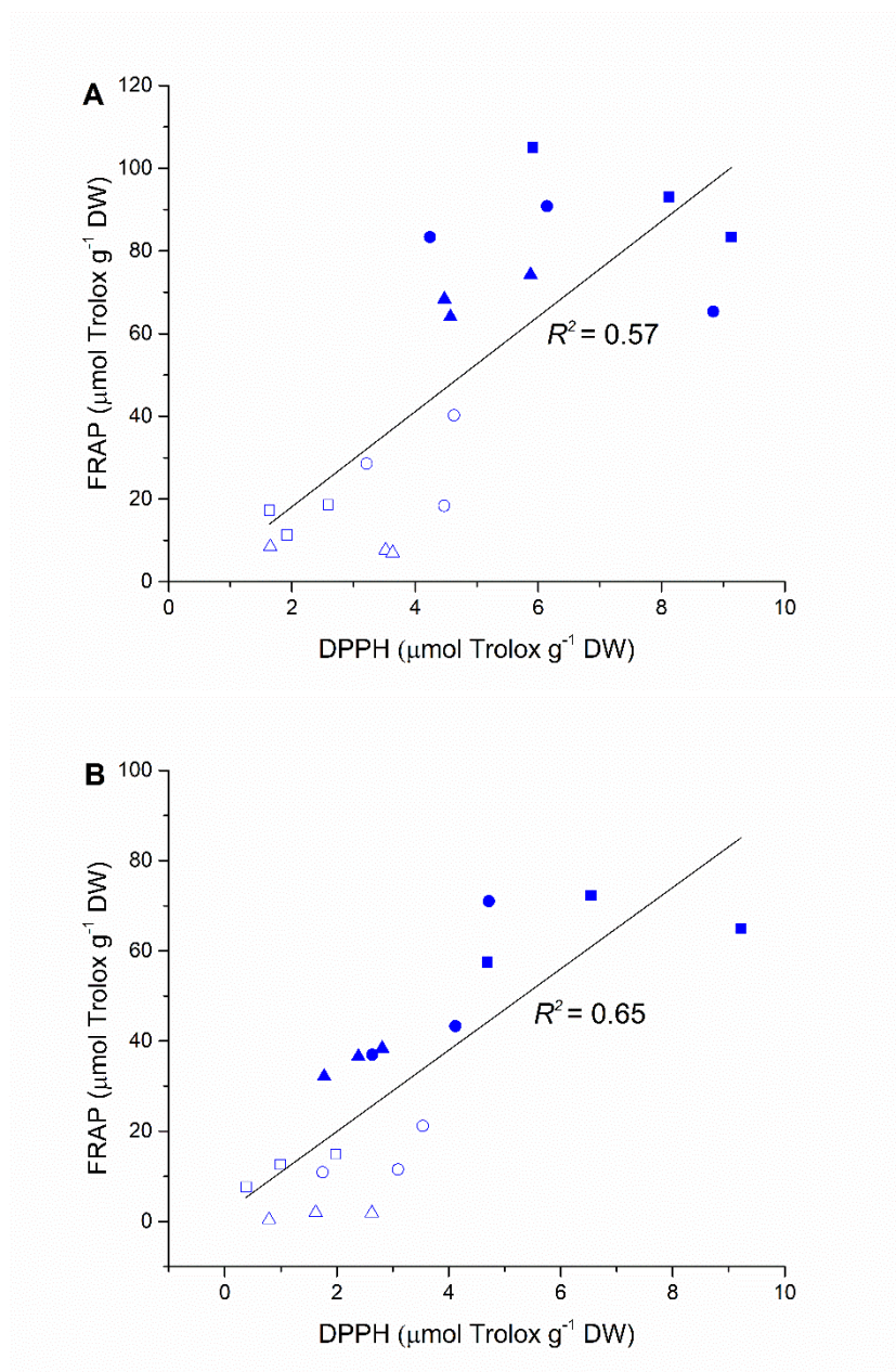
Figure 4.2 Relationship between DPPH and FRAP assays for (A) mixotrophically and (B) heterotrophically cultivated Micractinium sp. ME05. Results of both assays were expressed as micromoles of Trolox equivalent per gram dry weight. The black line represents the regression line. Empty squares, filled squares, empty triangles, filled triangles, empty circles and filled circles represent hexane, methanol, water, acetone, ethyl acetate and ethanol extracts, respectively.
