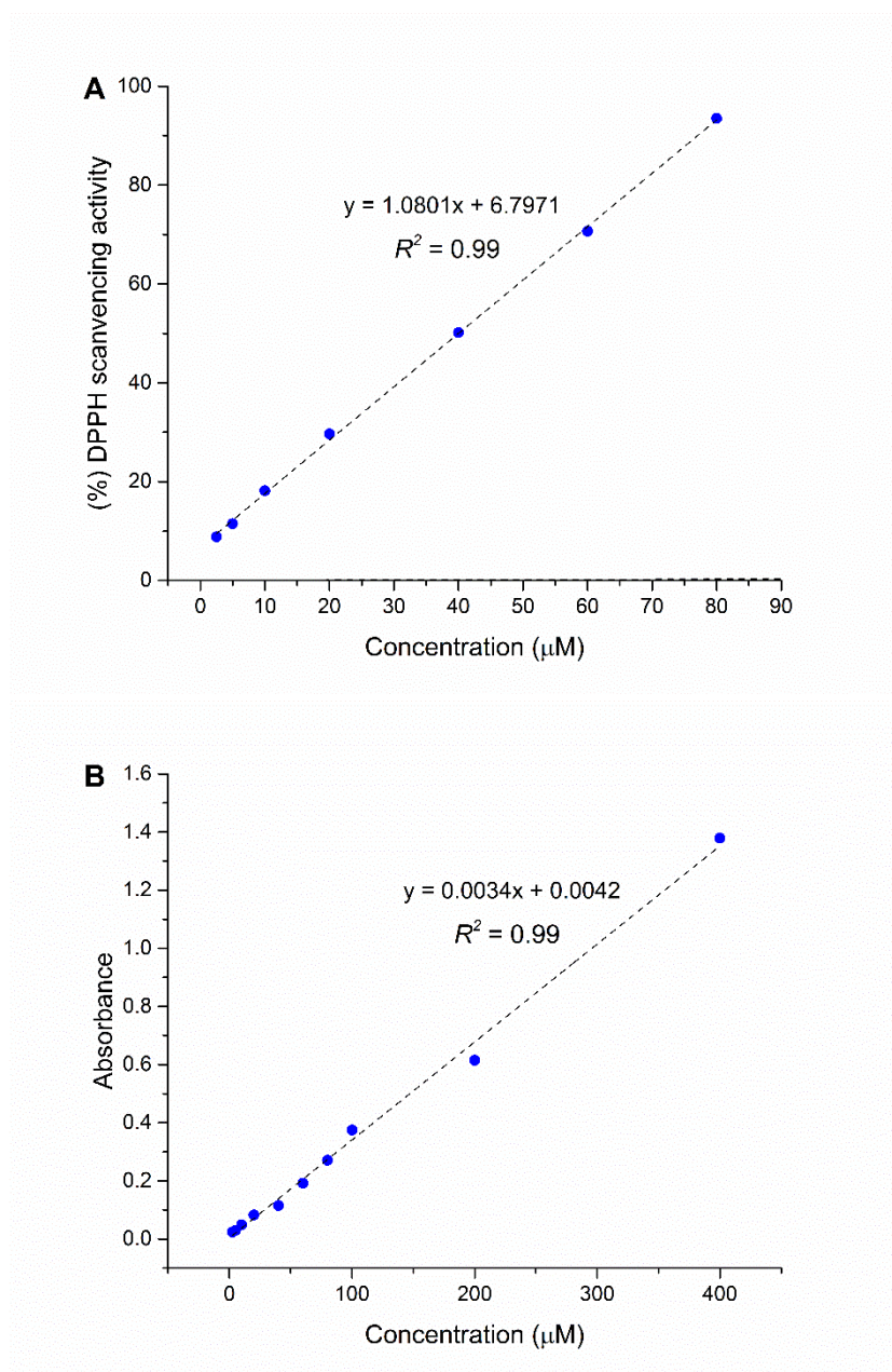
Figure 6.3 The standard curves of (A) DPPH assay and (B) FRAP assay prepared with serially diluted trolox solutions. The regression equations used in calculation of trolox equivalents are represented on the regression line.
