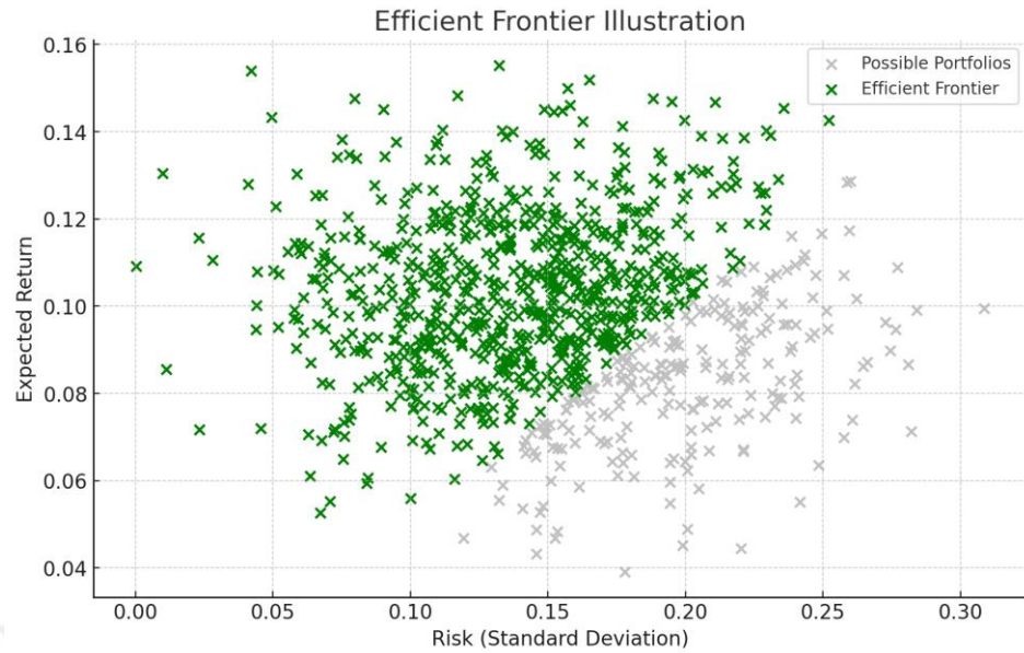
Figure 4.2: Efficient Frontier
