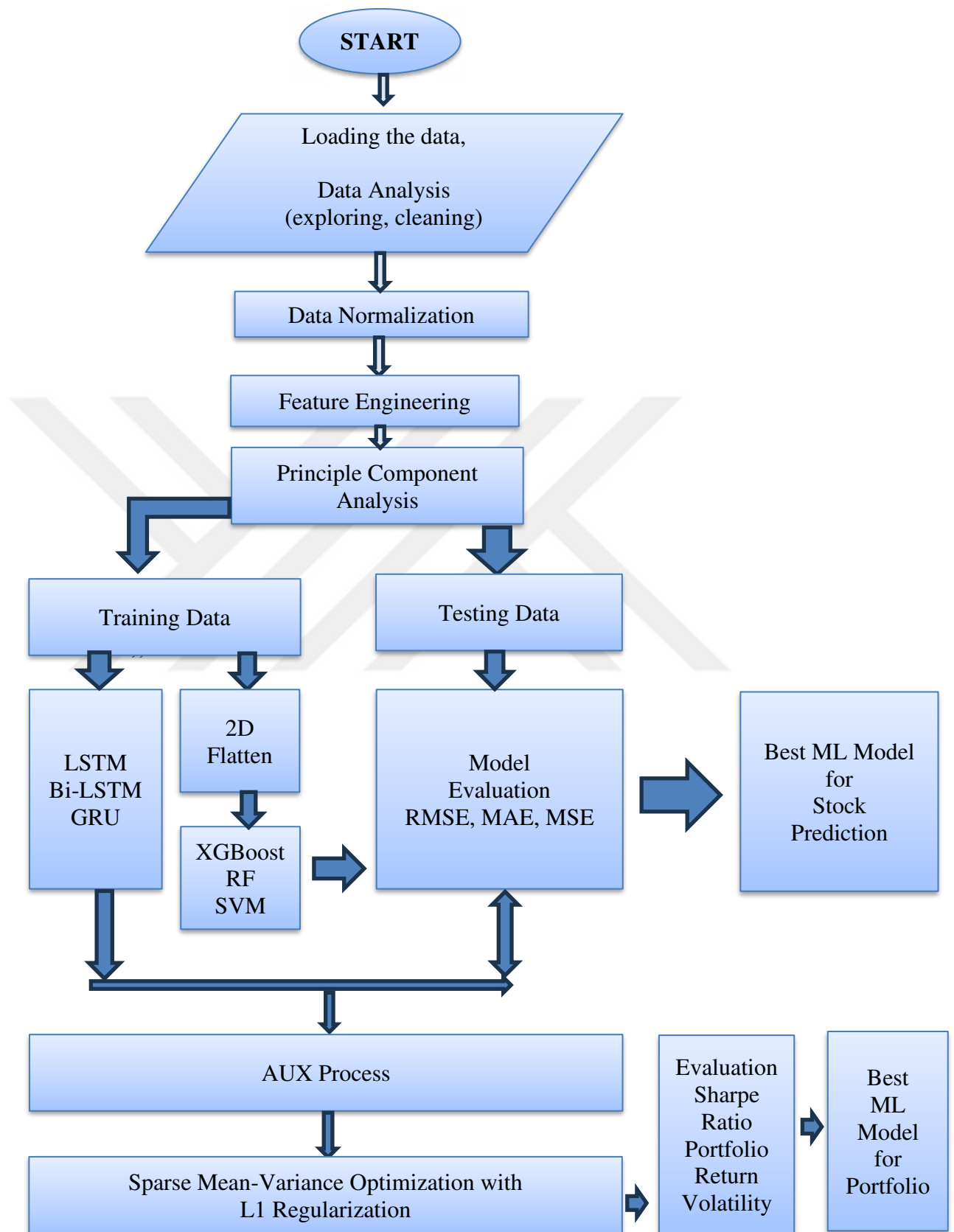
Figure 5.1.: Research Framework
