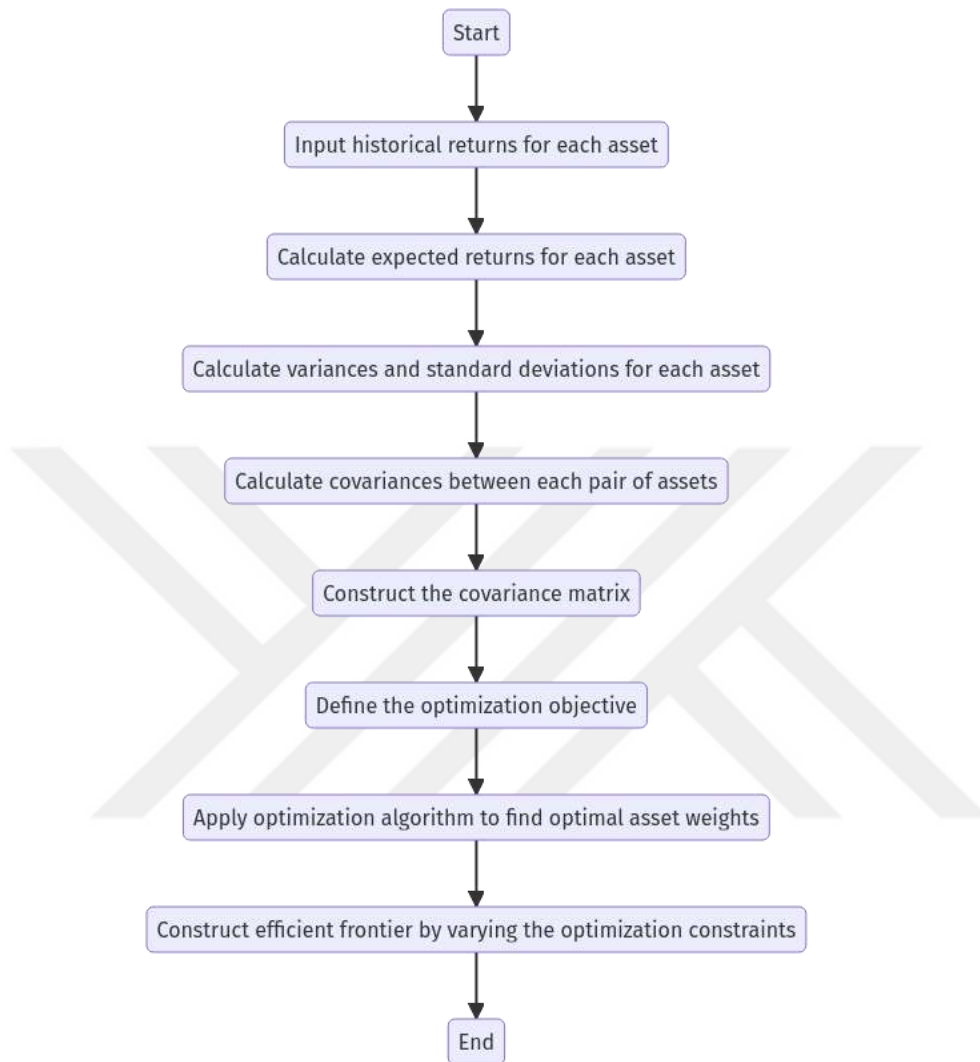
Figure 4.1: Flowchart of Markowitz Portfolio Theory
