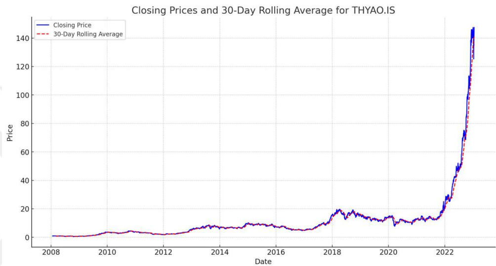
Figure 5.2: Closing Prices and 30-Day Rolling Average for THYAO.IS
