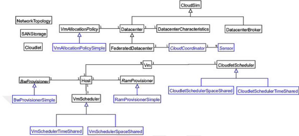
Figure 4.2: CloudSim Class Diagram.
