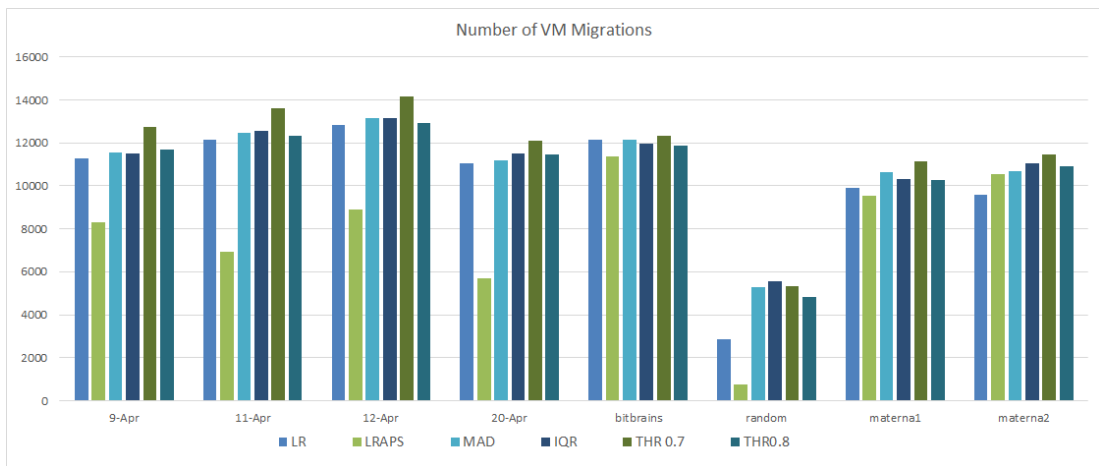
Figure 4.5: Number of VM Migrations.
