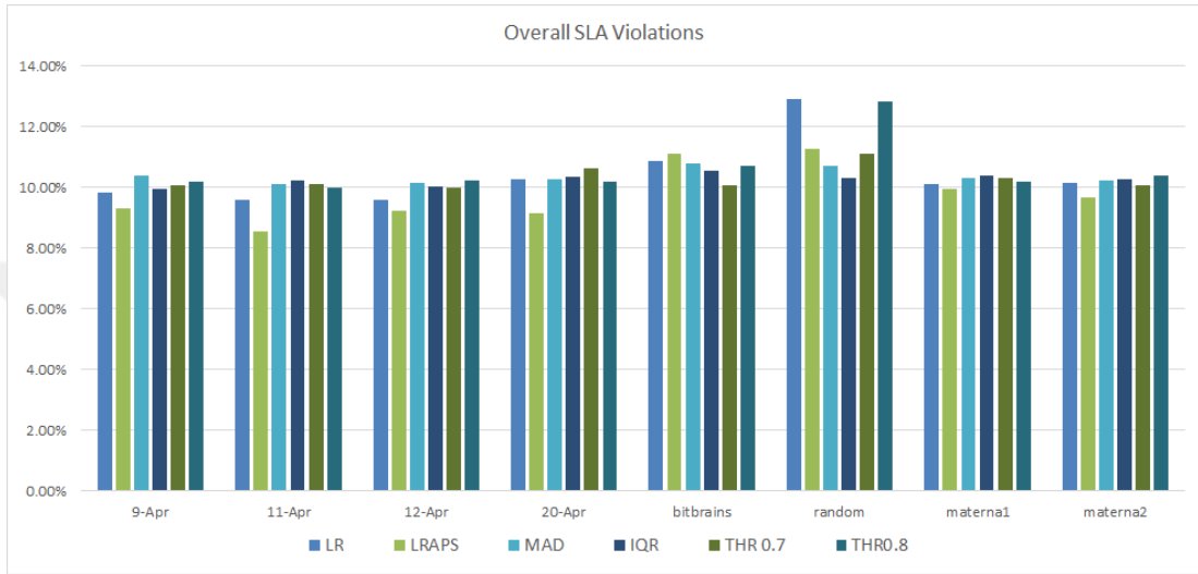
Figure 4.4: Overall SLA Violations.
