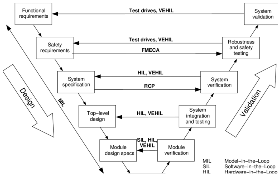
Figure 2.5: V Diagram for Embedded Design [5]
