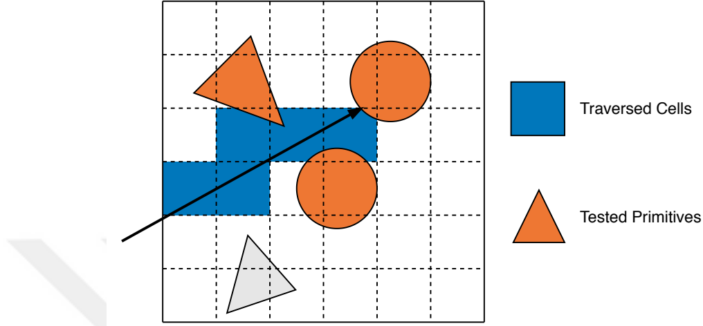
Figure 2.1: A uniform grid structure
