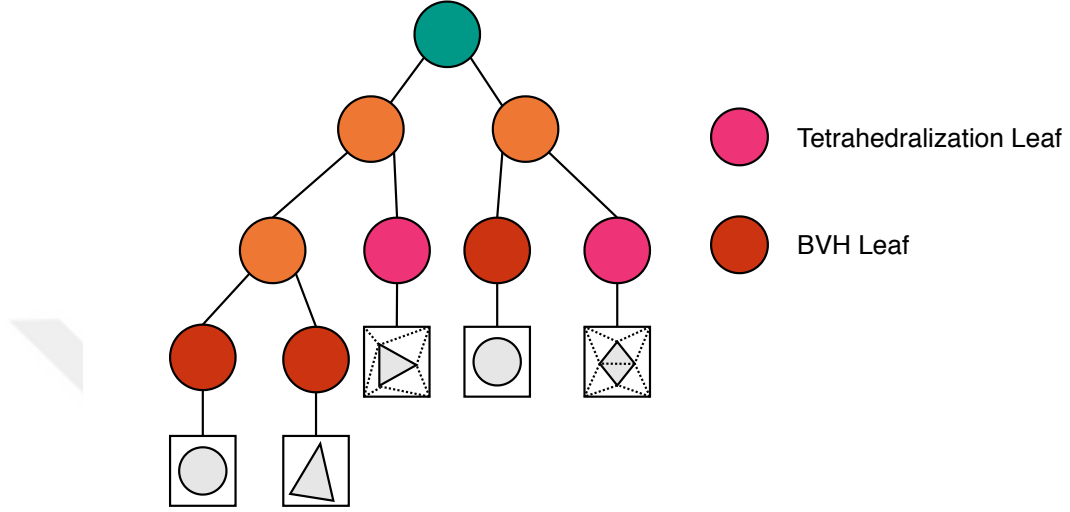
Figure 3.1: Bounding Volume Hierarchy-Tetrahedralization hybrid (BTH) acceleration structure.
