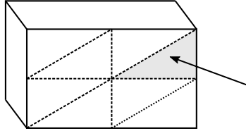
Figure 3.2: Finding the initial tetrahedron in a bounded tetrahedralization. The initial tetrahedron can be found using the bounding face that the ray hits (shaded region).
