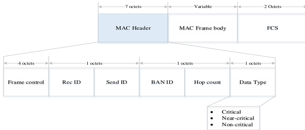
Figure 4.2: IA-MAC Format
