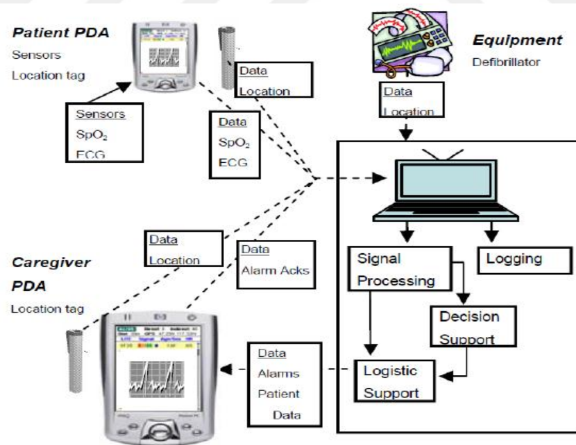
Figure 3.4: Architecture of SMART
