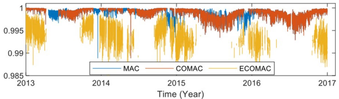
Figure 3.18. Variation of the first mode shape (MAC, COMAC and ECOMAC) between 2013-2017.
