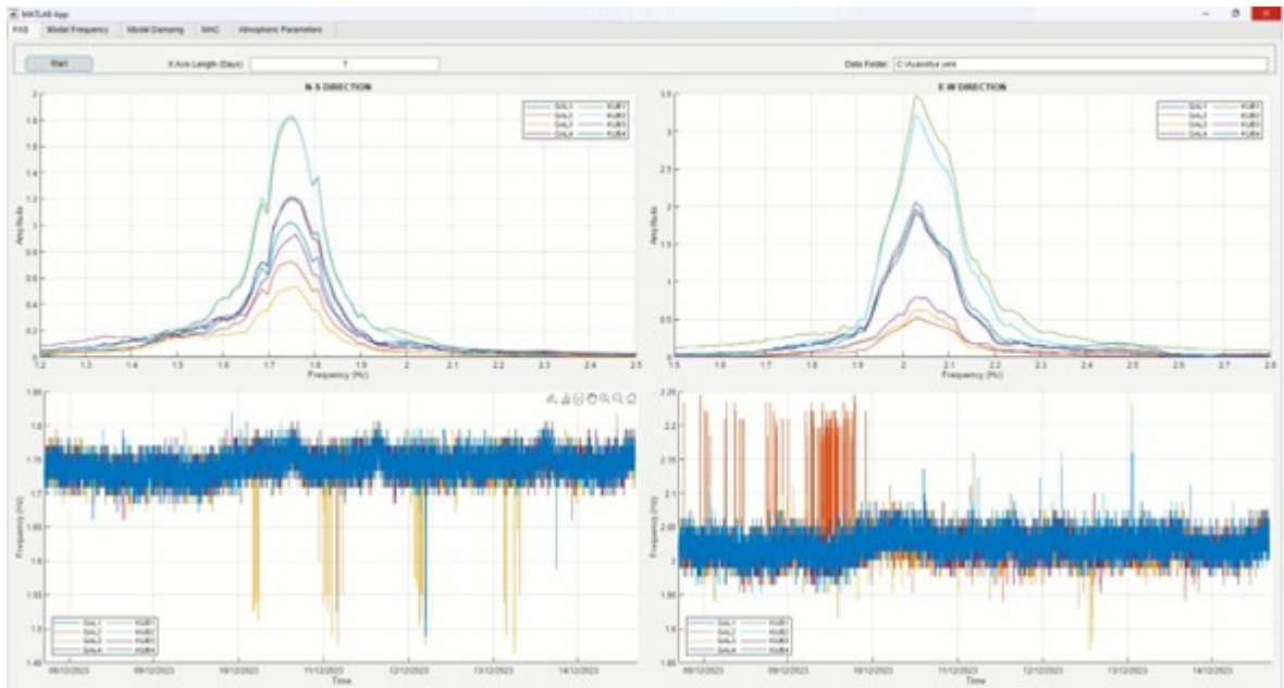
Figure 5.6. The screenshot of the "FAS" tab in the "Monitoring Module".
