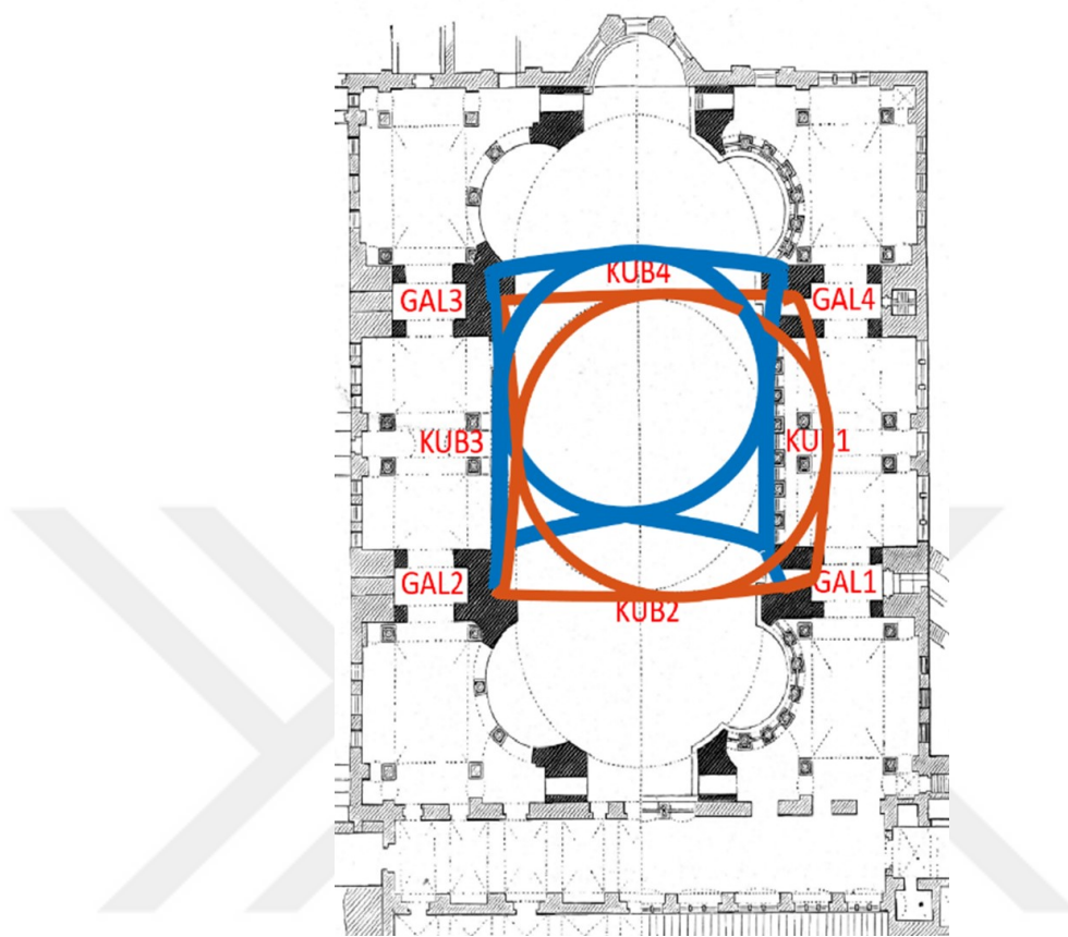
Figure 3.1. The first and second mode shapes of Hagia Sophia, top view.
