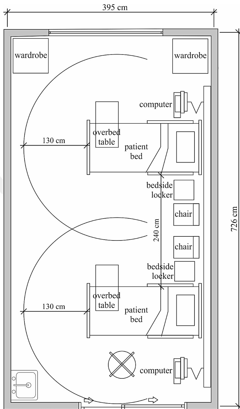
Figure C.20. Sample plan of a double-bed intensive care inpatient room according to the MH standard (2010)
