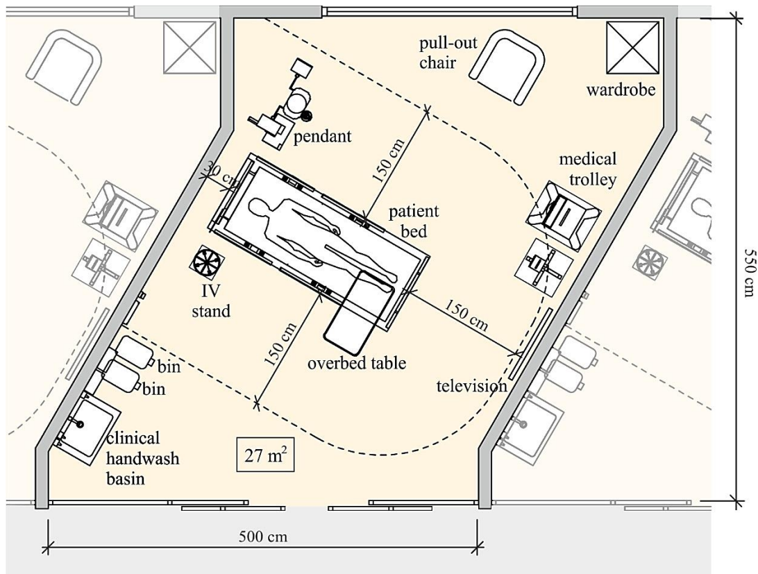
Figure 4.12. Proposed intensive care inpatient room
