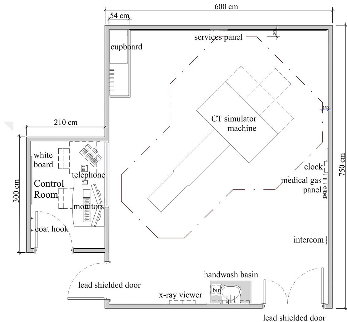
Figure B.8. Sample plan of a CT simulator room according to the AHIA standard (2017d)
