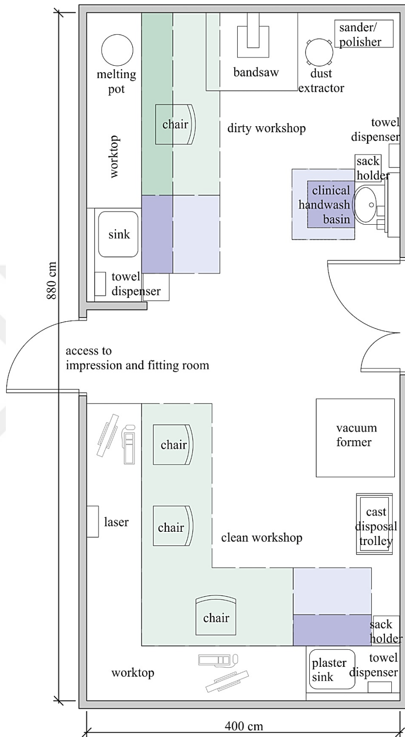
Figure B.16. Sample plan of a molding workshop according to the DH standard (2013a)
