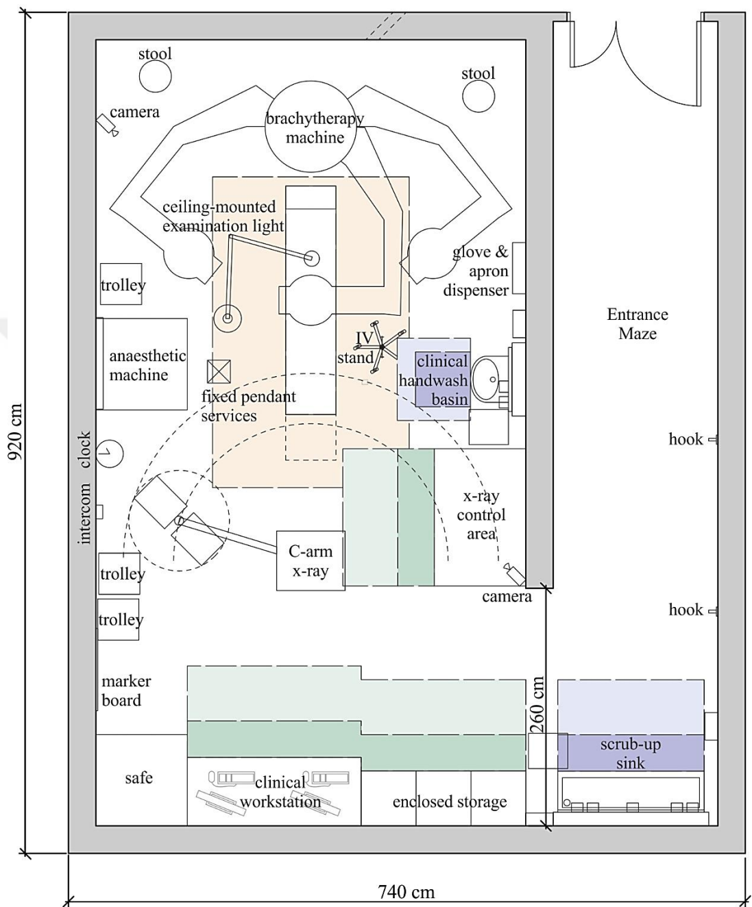
Figure B.6. Sample plan of an internal radiotherapy bunker according to the DH standard (2013a)
