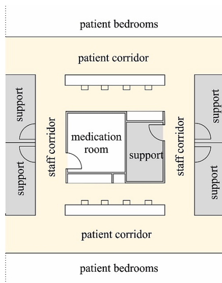
Figure 4.14. A sample schematic plan of a nurse station
