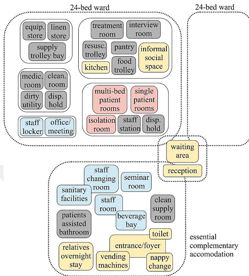
Figure C.2. The functional relationship diagram of an inpatient care service according to the DH standard (2013b)
