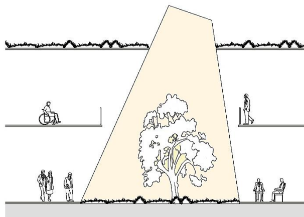
Figure 4.18. Schematic drawing of a skylight in healthcare facilities
