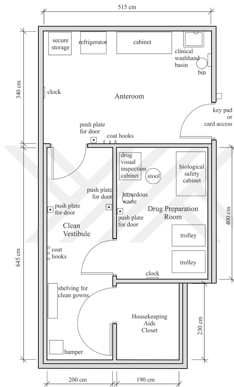
Figure A.7. Sample plan of a chemotherapy preparation module according to the DVA standard (2009)
