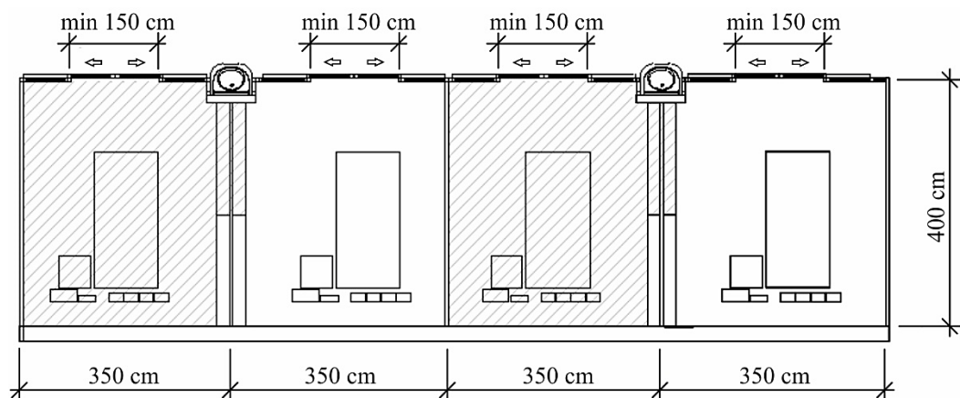
Figure C.19. Sample plan of arena-type intensive care inpatient area according to the MH standard (2012)
