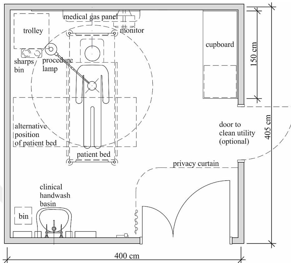
Figure B.14. Sample procedure room plan according to the AHIA standard (2017e)
