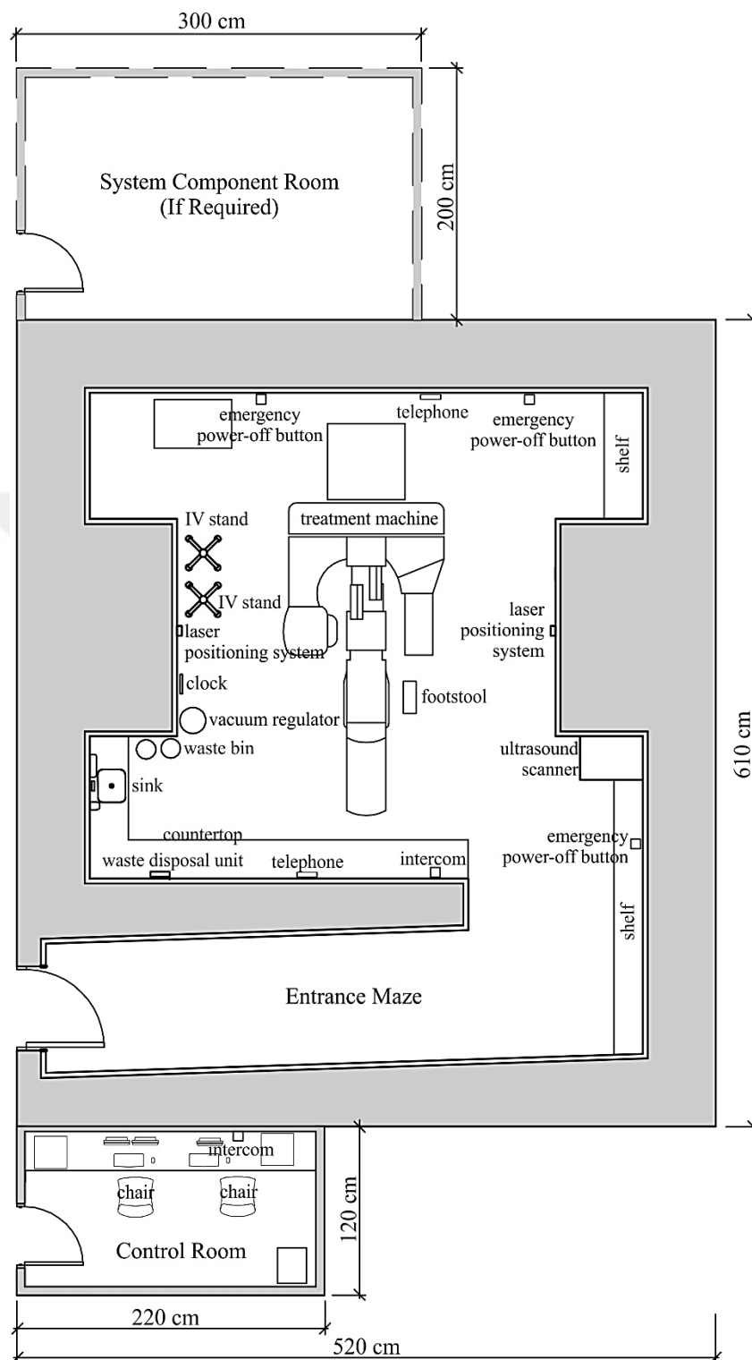
Figure B.5. Sample plan of an external radiotherapy bunker according to the DVA standard (2008)
