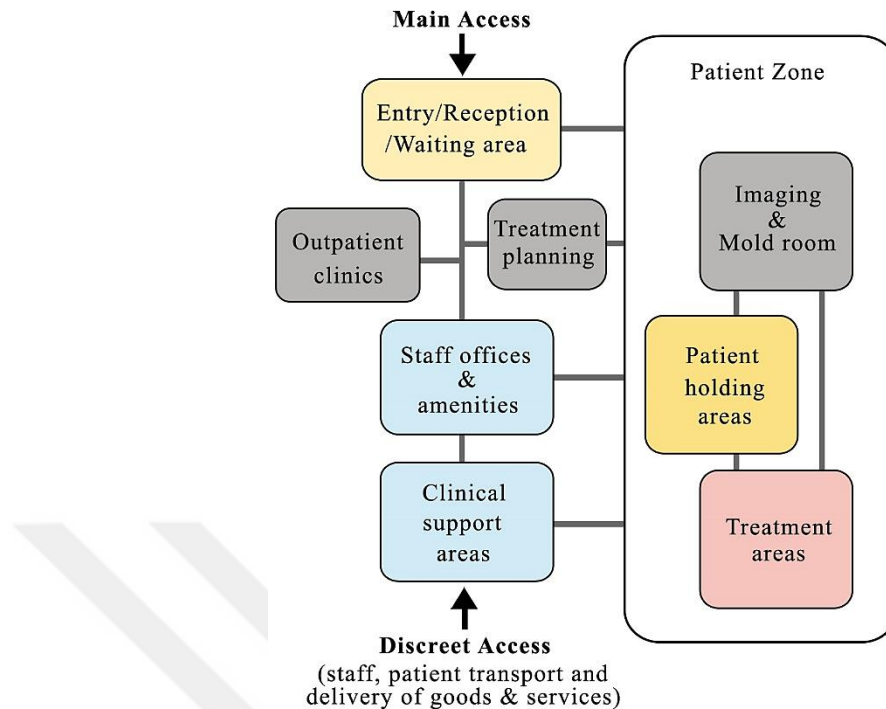
Figure B.1. The functional relationship diagram of a radiation oncology department according to the AHIA standard (2016c)
