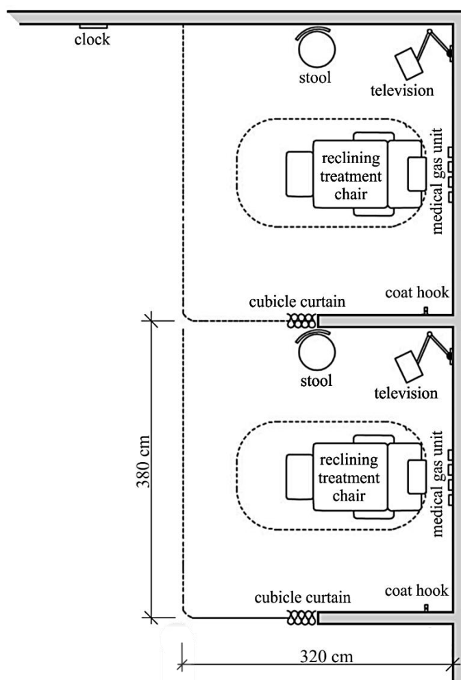
Figure A.5. Sample plan of a chemotherapy arena according to DVA standard (2009)
