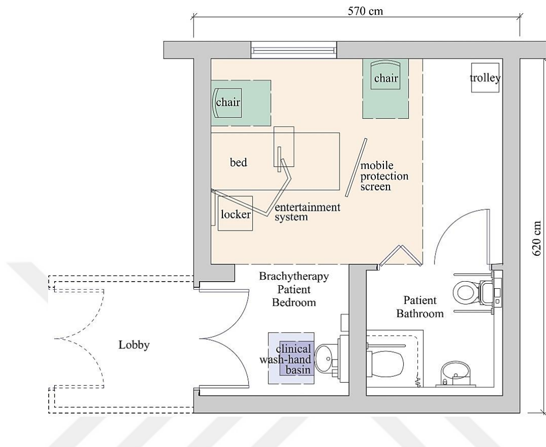
Figure C.11. Sample plan of an unsealed-source brachytherapy room according to the DH standard (2013a)
