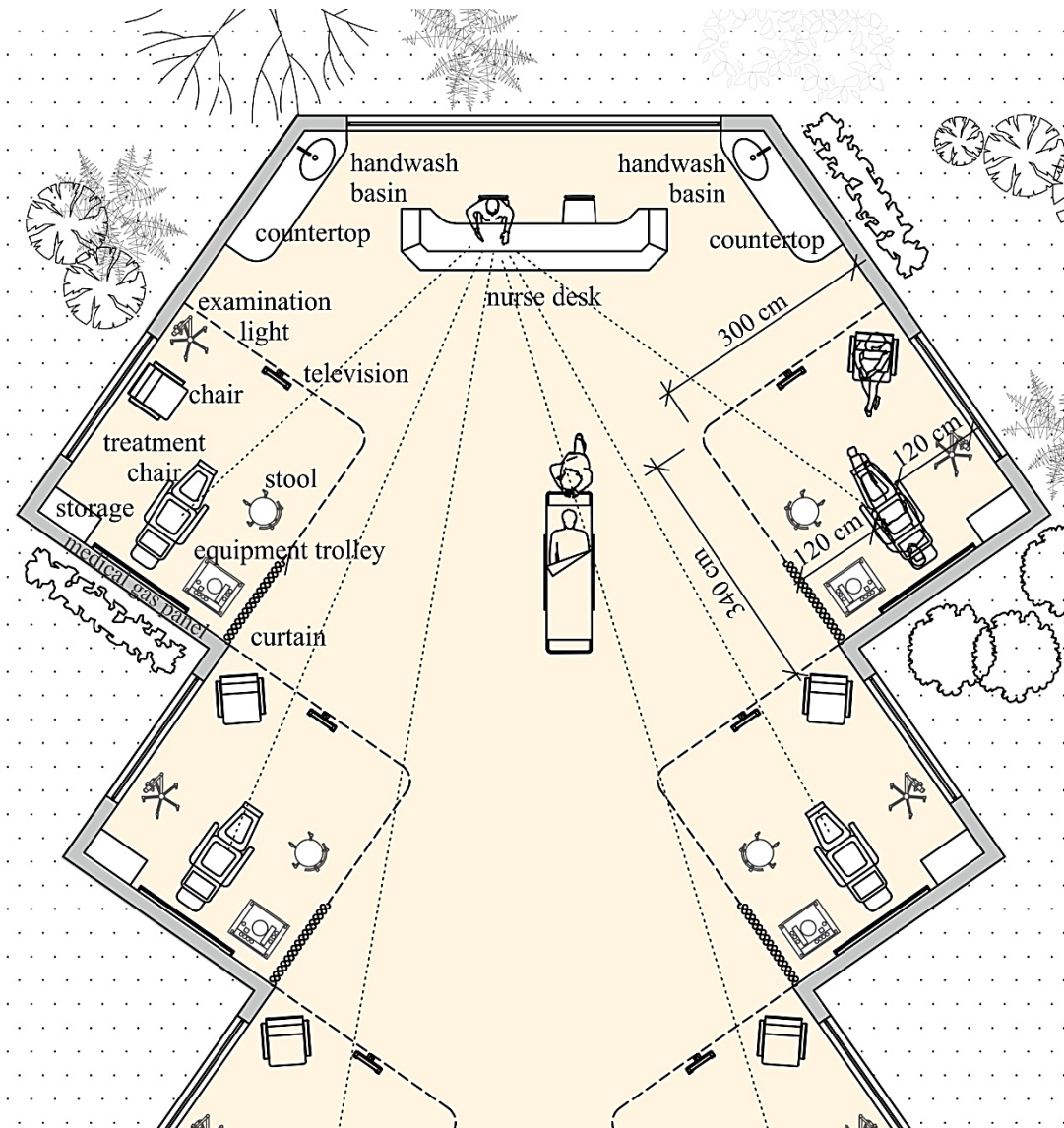
Figure 4.5. Proposed schematic drawing of a chemotherapy arena
