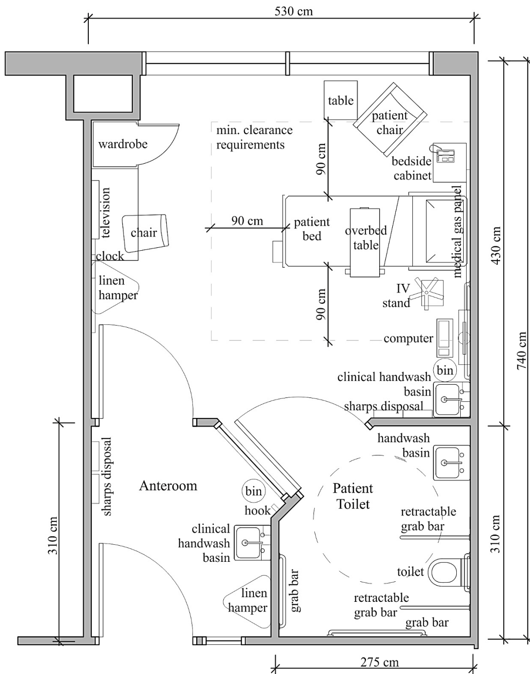
Figure C.14. Sample plan of an isolation inpatient room according to the DVA standard (2011)
