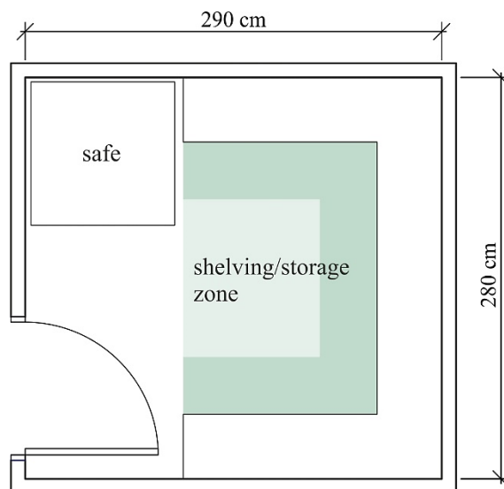
Figure B.7. Sample plan of a sealed radioactive source storage according to the DH standard (2013a)
