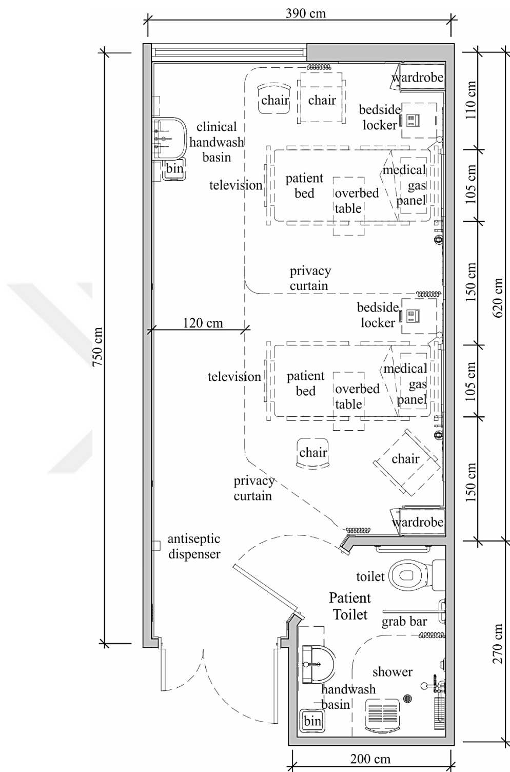
Figure C.6. Sample plan of a two-bed acute care inpatient room according to the AHIA standard (2018c)
