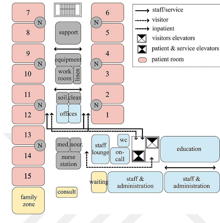
Figure C.4. Schematic plan of an intensive care inpatient service according to the DVA standard (2011)
