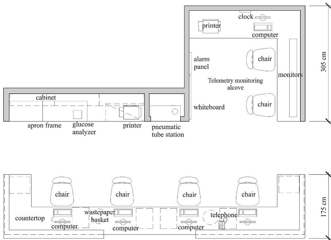
Figure C.21. Sample plan of a nurse station according to the DVA standard (2011)
