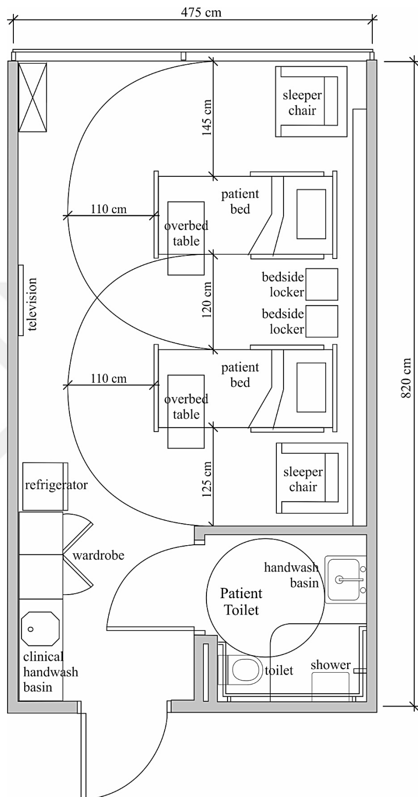
Figure C.16. Sample plan of a double-bed acute inpatient room according to the MH standard (2010)
