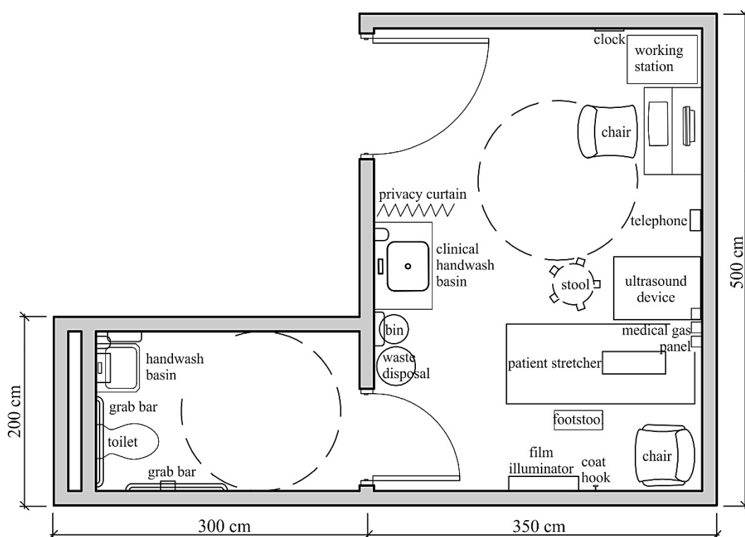
Figure B.12. Sample plan of an ultrasound room according to the DVA standard (2008)
