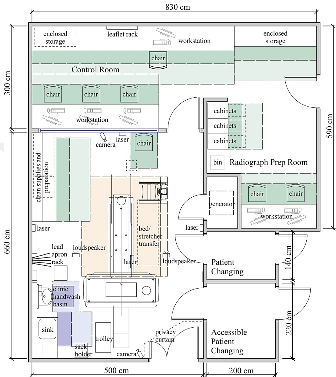
Figure B.10. Sample plan of an imaging module according to the DH standard (2013a)
