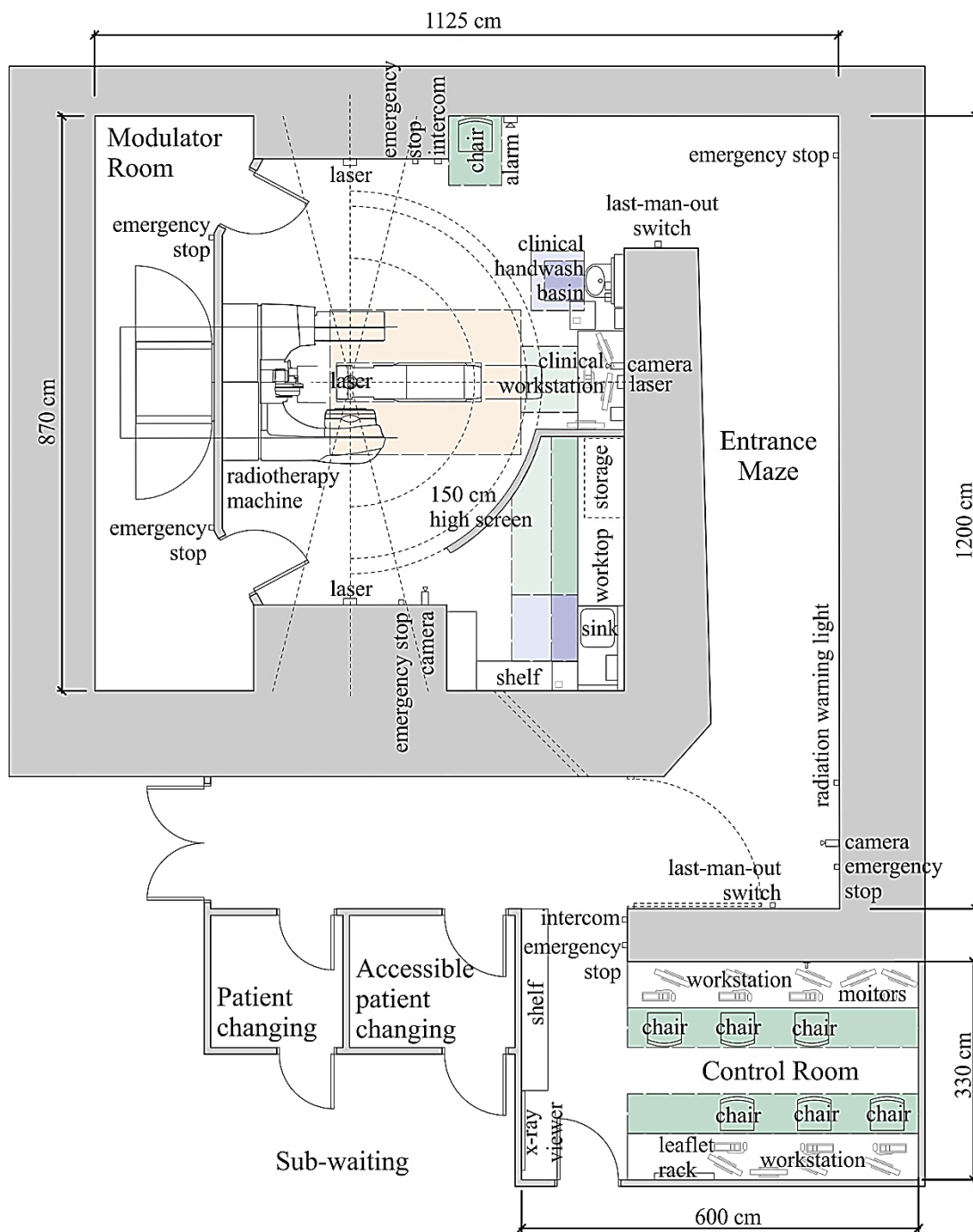
Figure B.4. Sample plan of an external radiotherapy bunker according to the DH standard (2013a)
