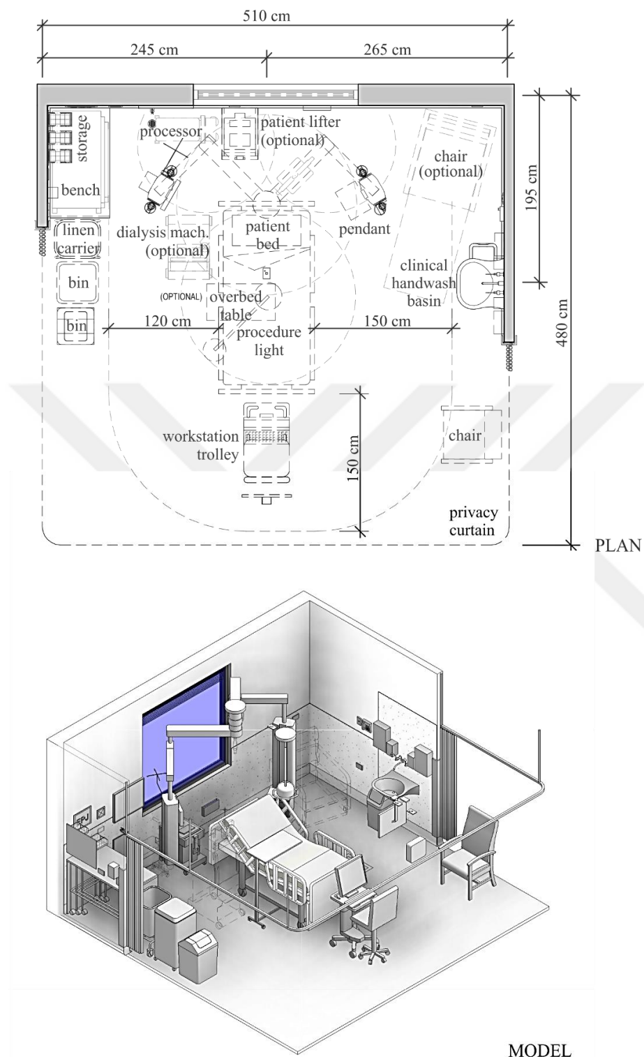
Figure C.9. Sample plan and model of an intensive care inpatient bay according to the AHIA standard (2019c)
