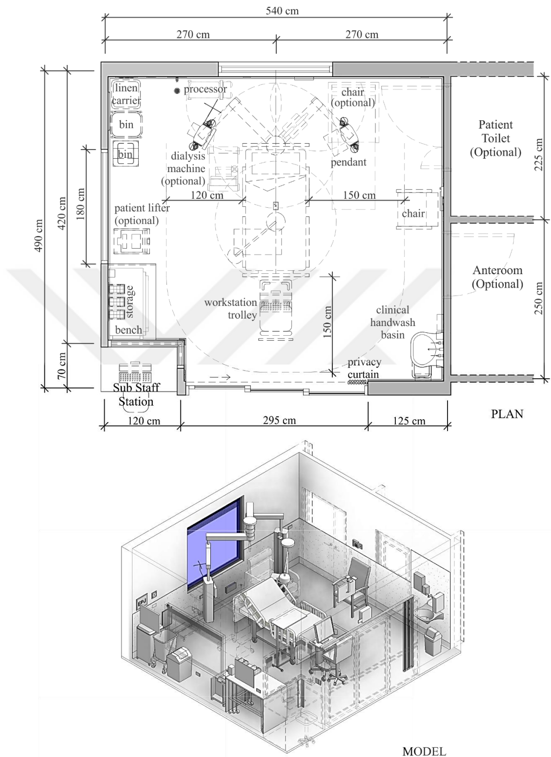
Figure C.8. Sample plan and model of an intensive care inpatient room according to the AHIA standard (2019d)
