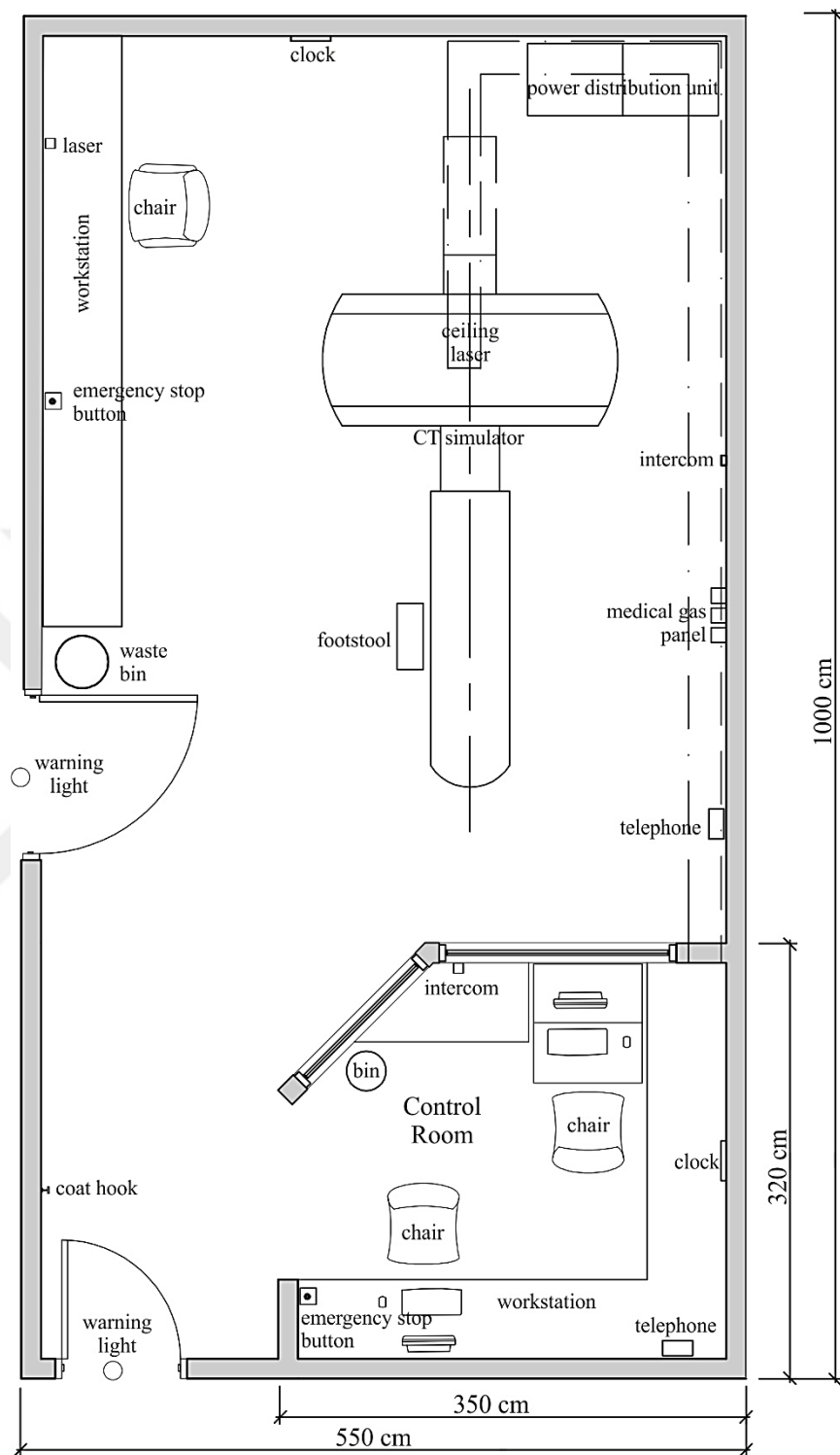
Figure B.11. Sample plan of a CT simulator room according to the DVA standard (2008)
