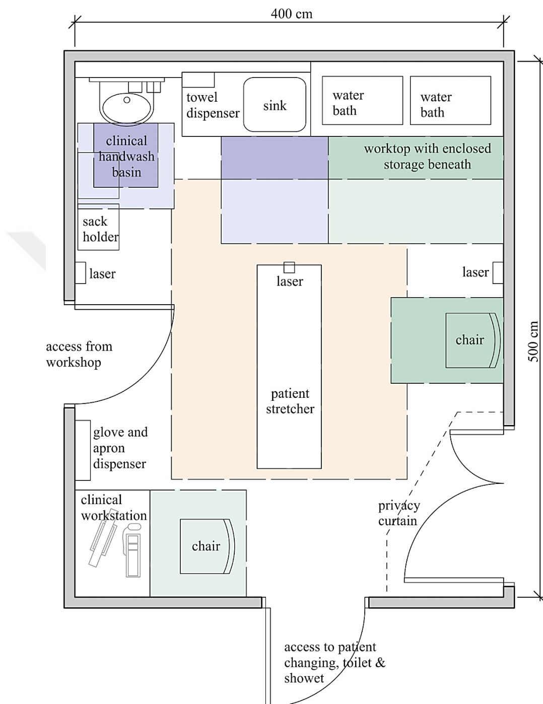
Figure B.15. Sample plan of an impression and fitting room according to the DH standard (2013a)
