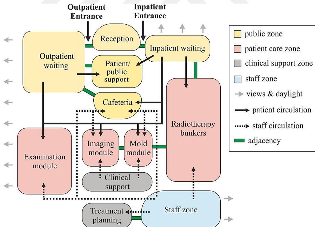
Figure 4.2. Proposal diagram for internal function relations of a radiation oncology department
