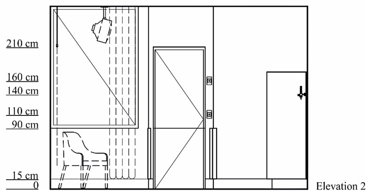
Figure B.17. Sample drawings of a patient preparation and recovery room according to the AHIA standard (2017a)
