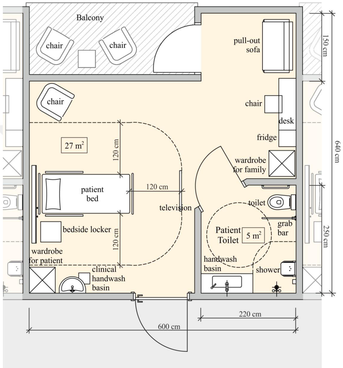
Figure 4.11. Proposed acute care inpatient room
