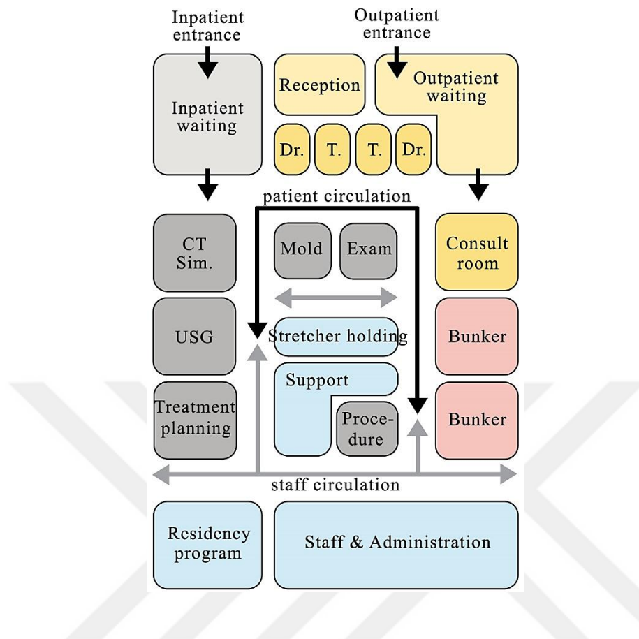
Figure B.3. The functional relationship diagram of a radiation oncology department according to the DVA standard (2008)
