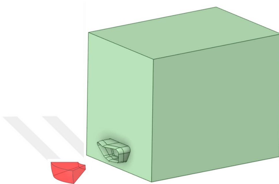
Figure 2.23. RCS Analysis Illumination Outlines
