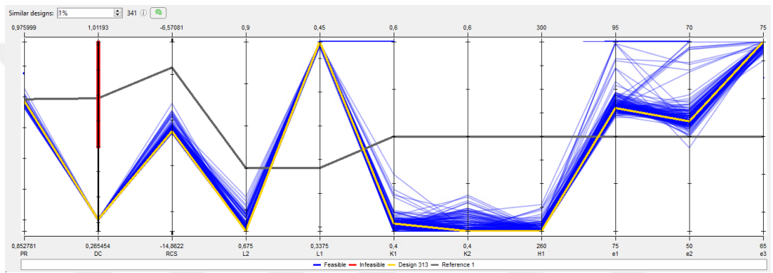
Figure 4.15. Design Optimization DC Investigation
