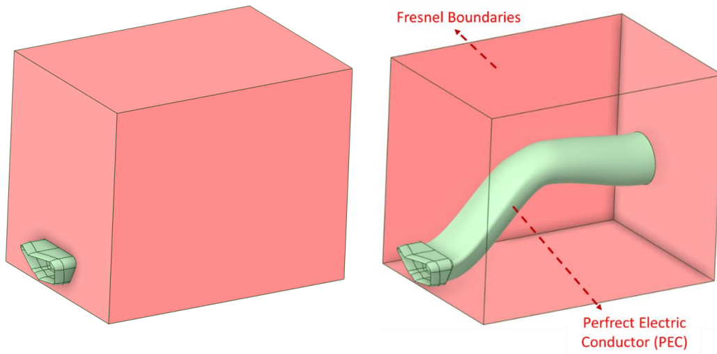
Figure 2.22. RCS Analysis Model
