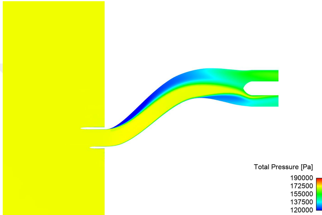
Figure 5.5. Flow Field Total Pressure Contour
