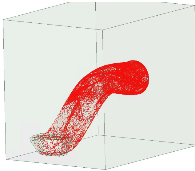
Figure 5.14. VTR Image of 5 th Bounce
