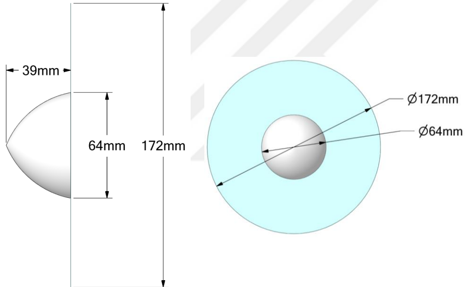
Figure 4.1. Design AIP Geometry Dimensions
