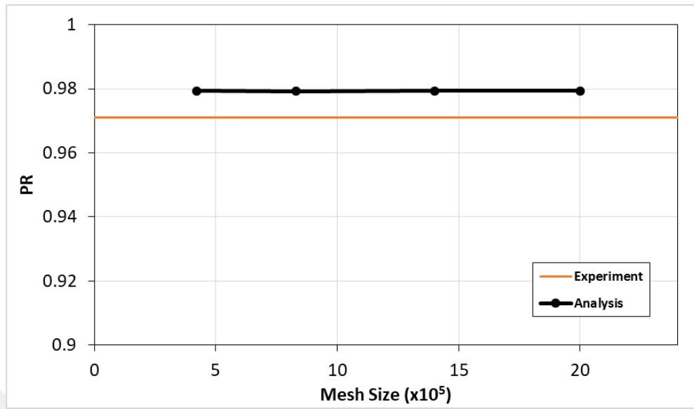
Figure 3.16. S-Shaped Duct Mesh Independence Study PR Results with Experimental Results [43]
