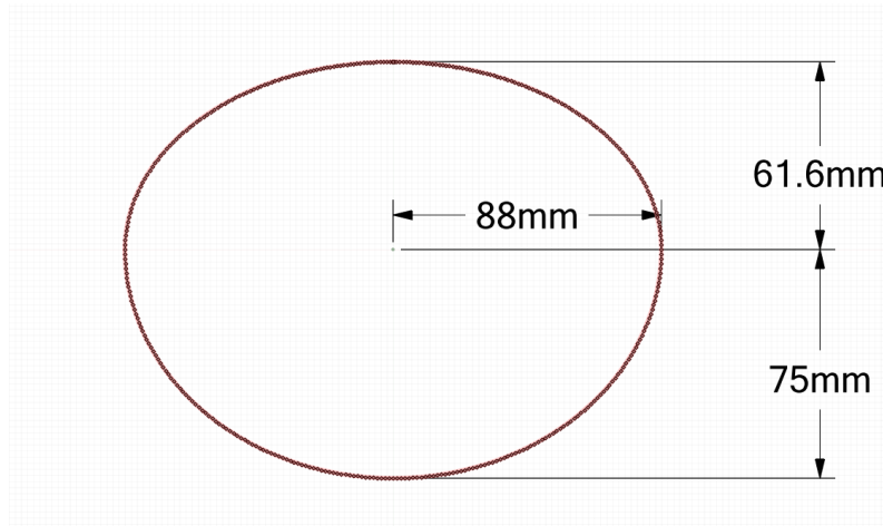
Figure 4.19. Optimized Intake Duct Middle Station Dimensions
