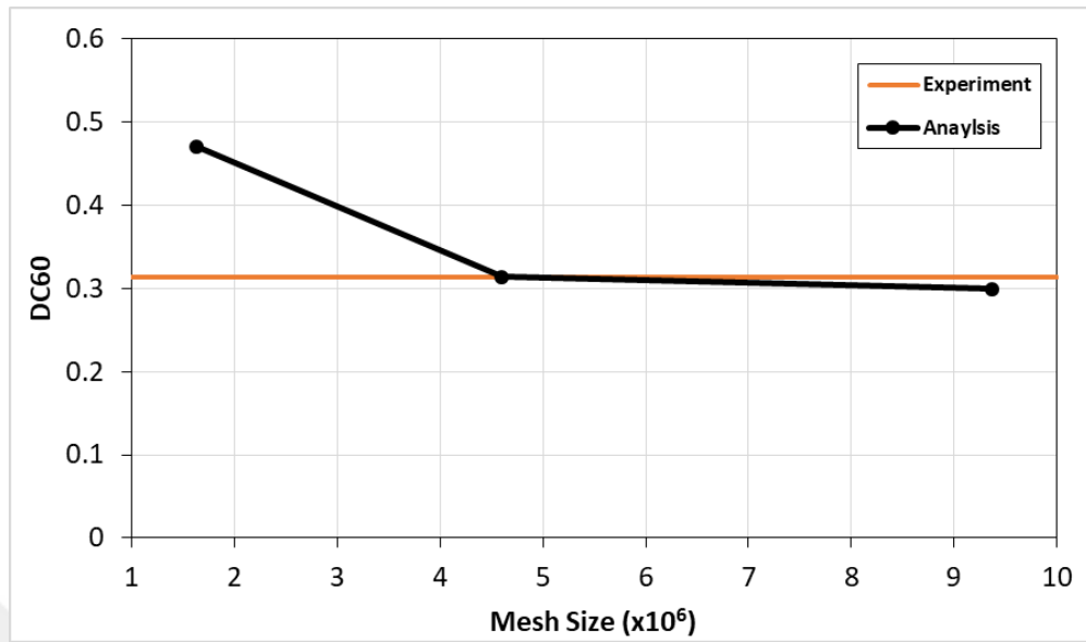
Figure 3.7. RAE M2129 Mesh Independence Study DC Results with Experimental Results [19]
