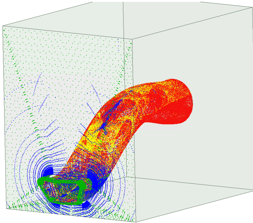
Figure 5.15. VTR Image of Bounces
