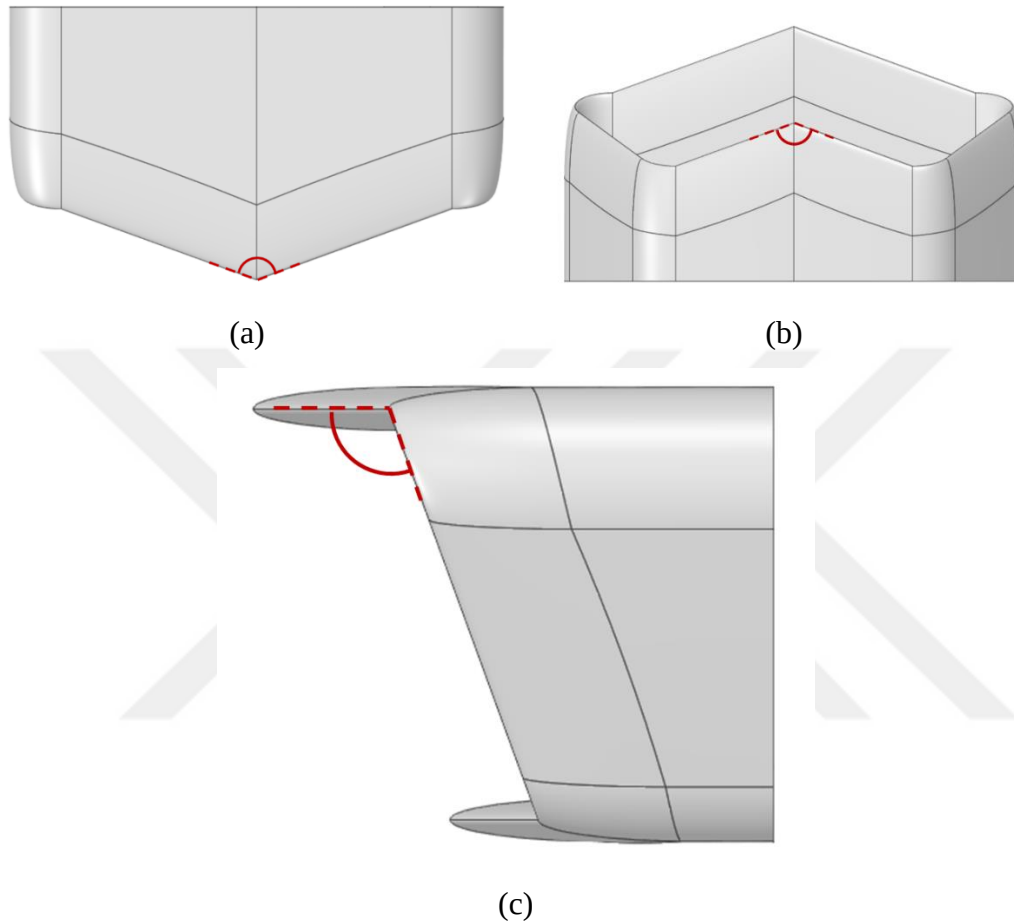
Figure 2.4. Intake Angular Definitions. (a) Upper Lip Horizontal Angle; (b) Lower Lip Horizontal Angle; (c) Lip Vertical Angle
