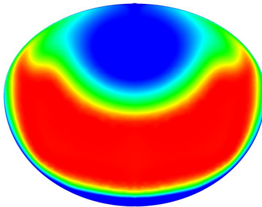
Figure 5.6. PR Contour at the Throat Station
