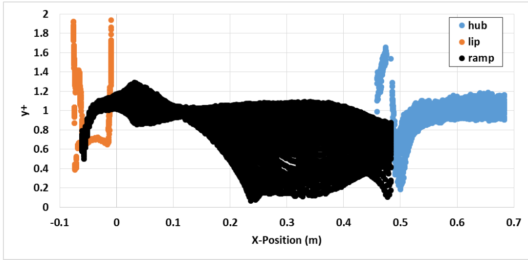
Figure 3.8. RAE M2129 y^+ Output of the “Medium” Mesh
