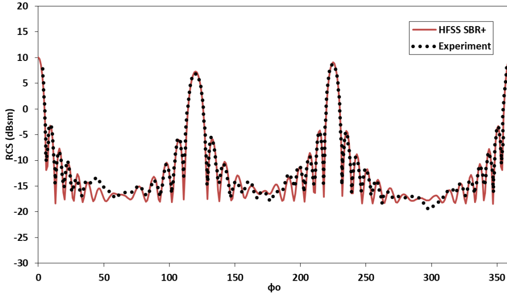
Figure 3.20. Triangular Prism Results Comparison with Experimental Data [21]
