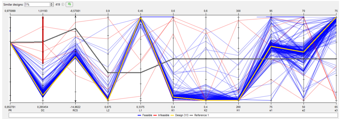
Figure 4.14. Design Optimization PR Investigation
