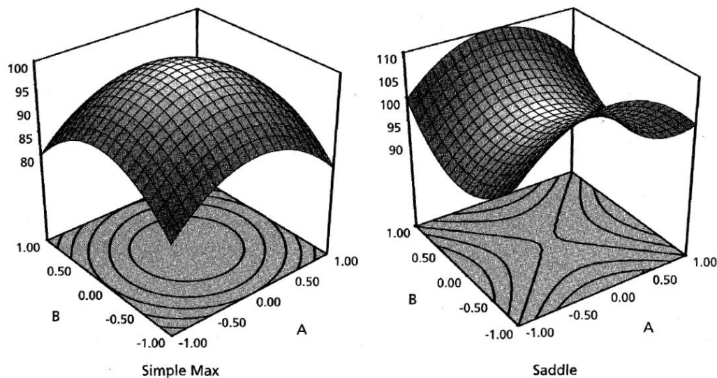
Figure 2.12. Response Surfaces. (a) Simple Maximum; (b) Saddle, [30]
