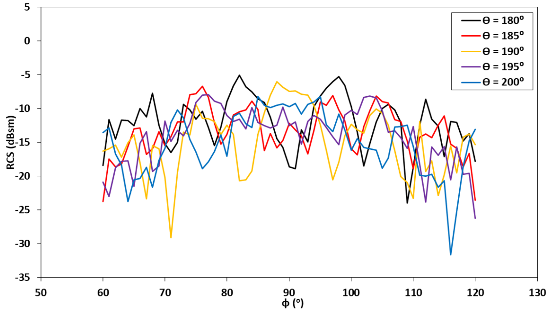
Figure 5.9. RCS Values of the Optimized Intake
