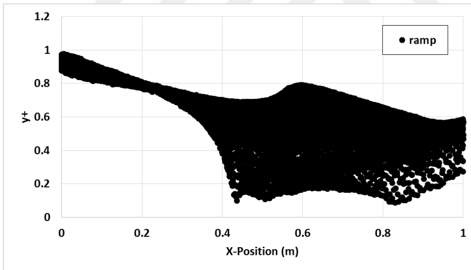
Figure 3.18. S-Shaped Duct y^+ Output of the “Medium” Mesh
