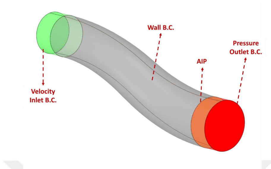
Figure 3.11. S-Shaped Duct Boundary Conditions
