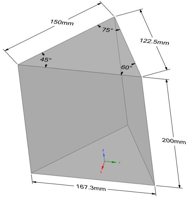
Figure 3.19. Triangular Prism Model
