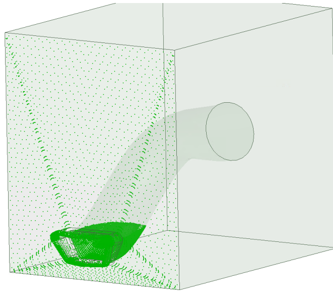
Figure 5.10. VTR Image of 1 st Bounce
