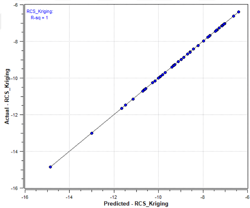
Figure 4.13. Surrogate Model RCS Output
