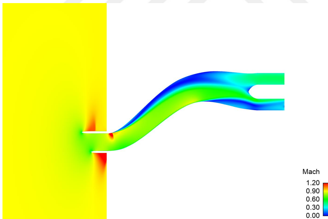
Figure 5.1. Mach Contour of the Validation Case
