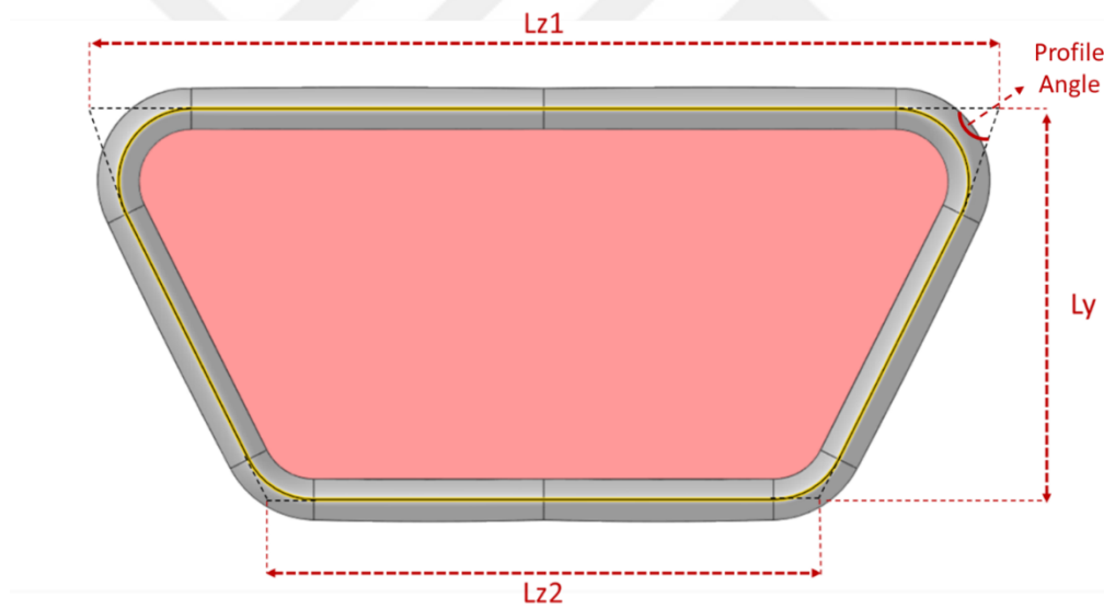
Figure 2.3. Intake Dimensional Definitions
