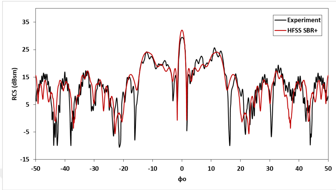
Figure 3.25. Simple Duct Results Comparison with the Experimental Data [22]
