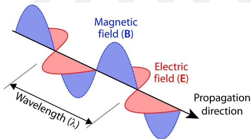
Figure 2.19. Electromagnetic Wave [39]
