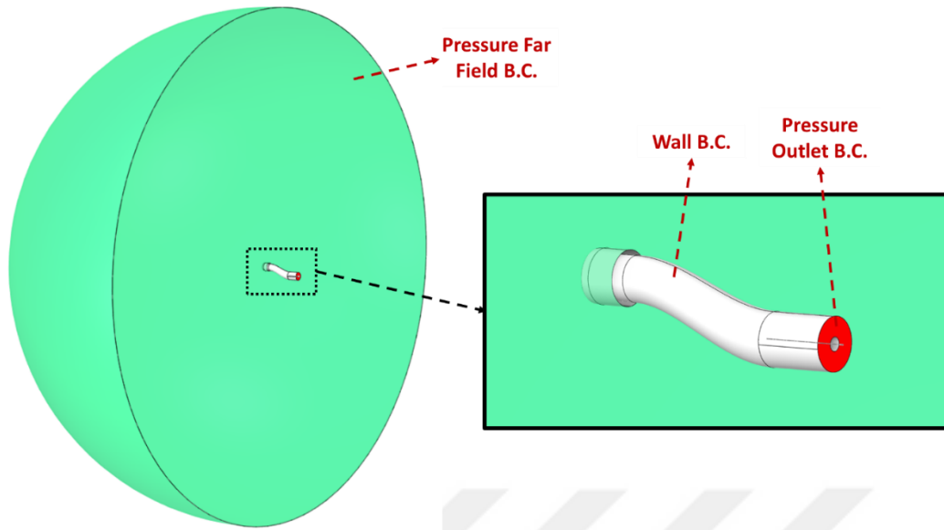
Figure 3.2. RAE M2129 Boundary Conditions
