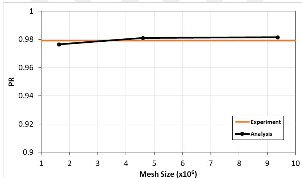
Figure 3.6. RAE M2129 Mesh Independence Study PR Results with Experimental Results [19]
