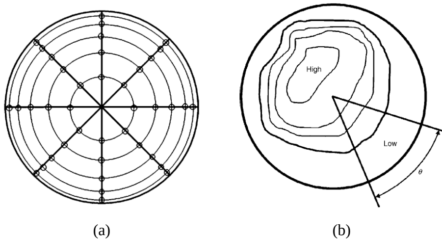
Figure 1.2. AIP Definitions. (a) Pressure Probe Placements; (b) Sector Definition for DC60 [4]
