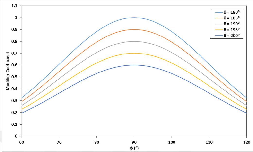
Figure 2.25. Gaussian Modifier for \theta Angle Sweeps
