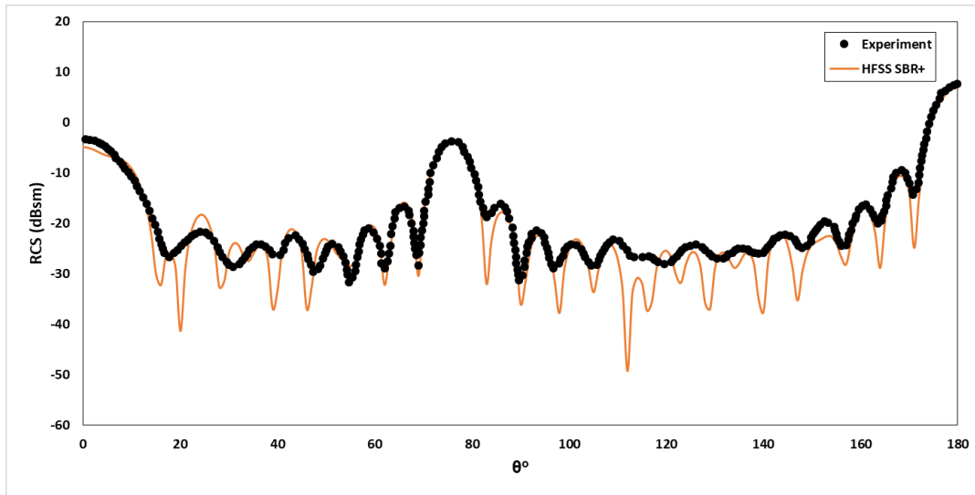
Figure 3.22. Truncated Cone Results Comparison with Experimental Data [21]
