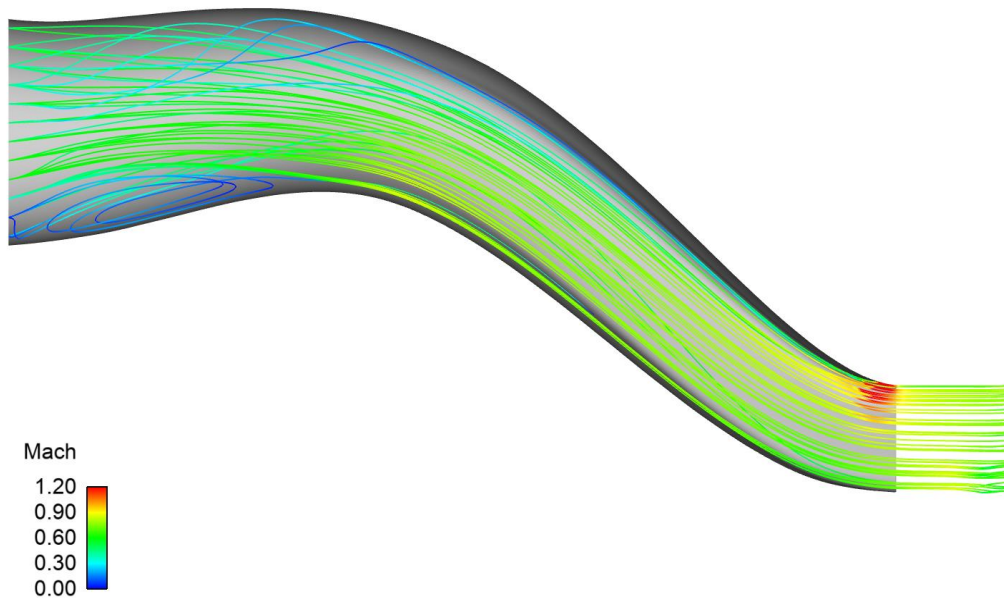
Figure 5.3. Mach Streamline Inside the Duct
