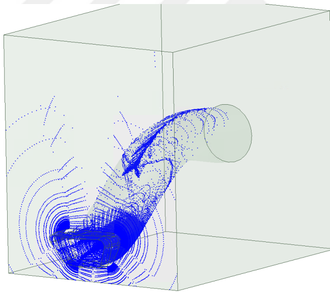
Figure 5.11. VTR Image of 2 nd Bounce
