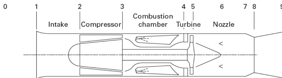
Figure 1.1. Simple Turbojet Engine Illustration [2]
