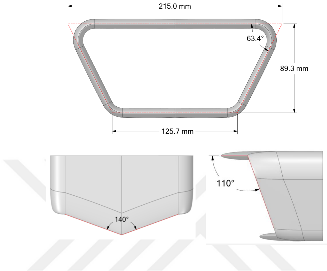
Figure 4.2. Design Intake Lip Dimensional Details
