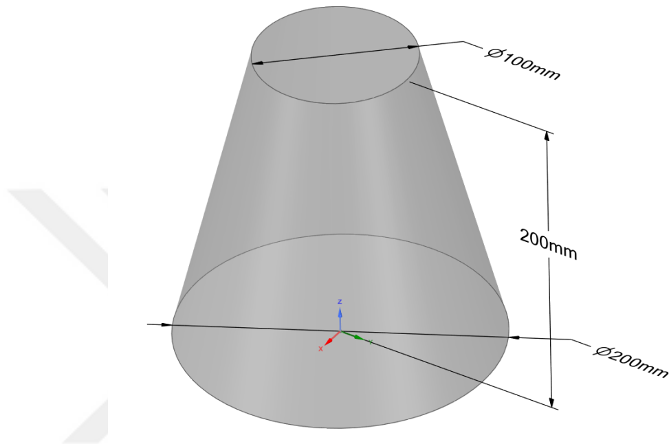
Figure 3.21. Truncated Cone Model
