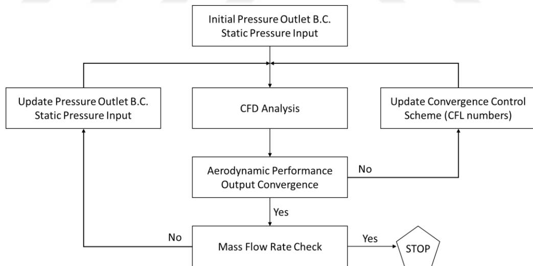
Figure 2.17. CFD Analysis Approach Schematic
