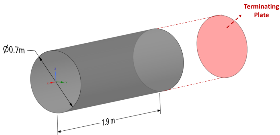
Figure 3.24. Simple Duct Model
