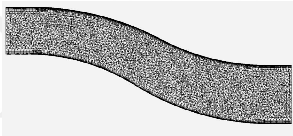
Figure 3.12. S-Shaped Duct Mesh Independence Study – Very Coarse Mesh
