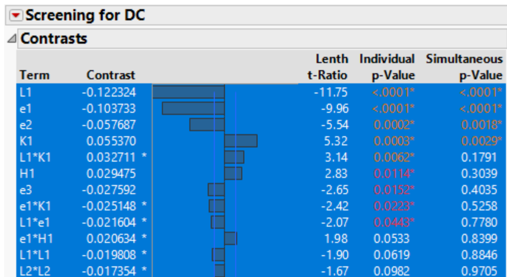
Figure 4.9. DOE – DC Results
