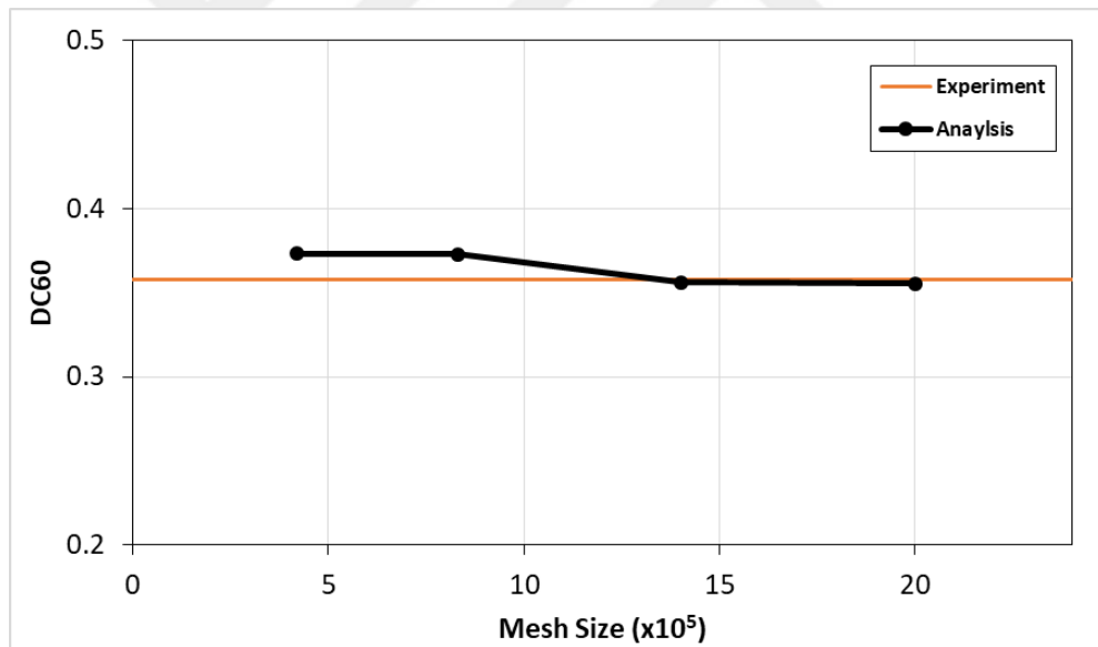
Figure 3.17. S-Shaped Duct Mesh Independence Study DC Results with Experimental Results [43]
