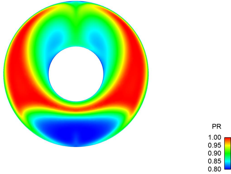
Figure 5.8. PR Contour at the AIP Station
