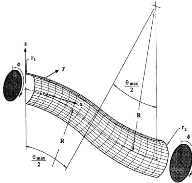
Figure 3.9. S-Shaped Duct Model Details [43]
