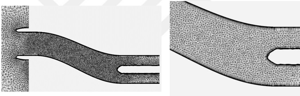
Figure 3.3. RAE M2129 Mesh Independence Study – Coarse Mesh
