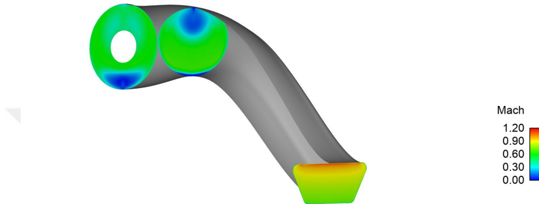
Figure 5.2. Mach Contours of the Main Stations
