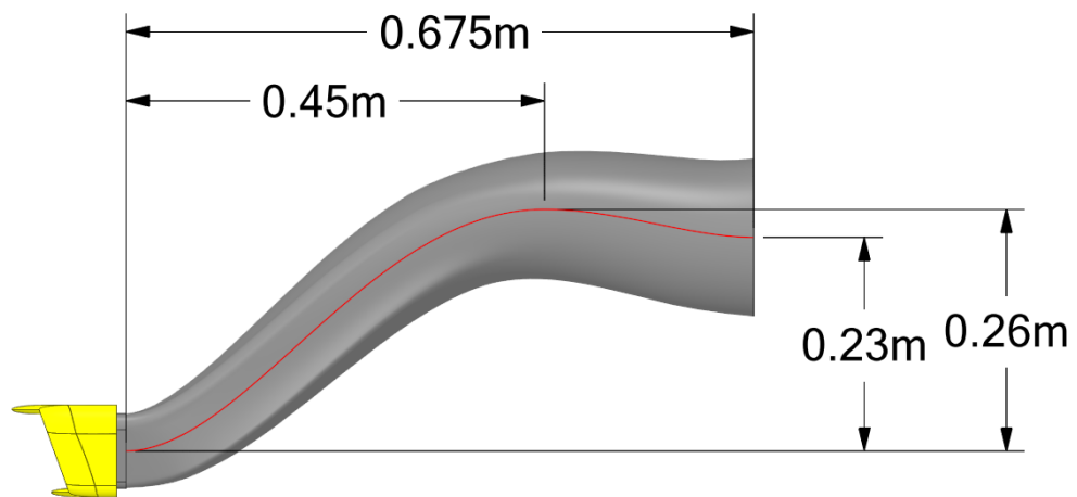
Figure 4.18. Optimized Intake Duct Dimensions
