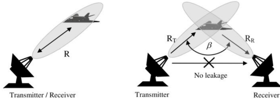
Figure 2.20. Monostatic and Bistatic Radar Configurations [40]
