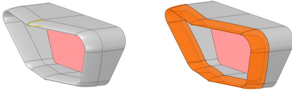
Figure 2.5. Intake Lip Airfoil Profile and Swept Surface Profile
