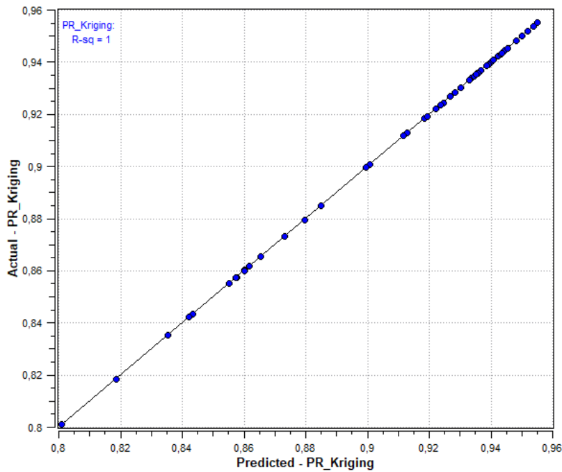
Figure 4.11. Surrogate Model PR Output
