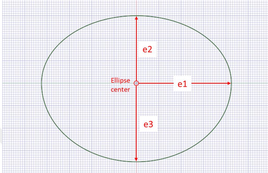
Figure 2.8. Middle Station Profile and Parameters
