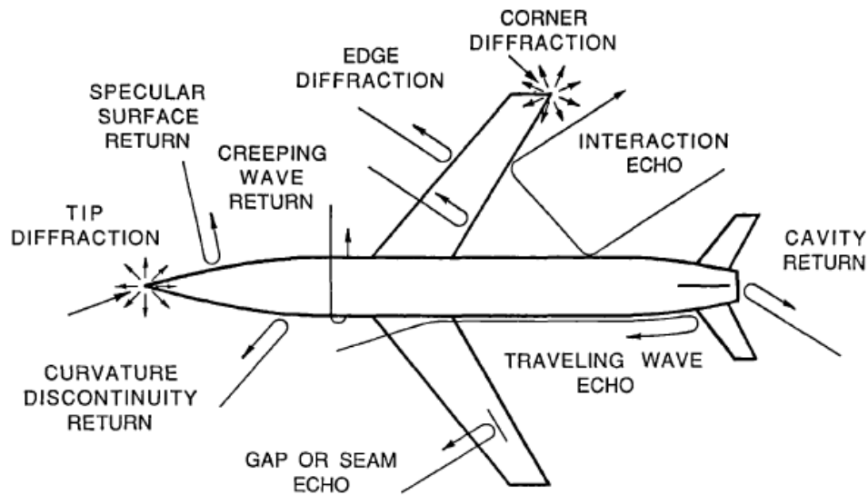
Figure 2.21. Aircraft Echo Scattering Mechanisms [10]
