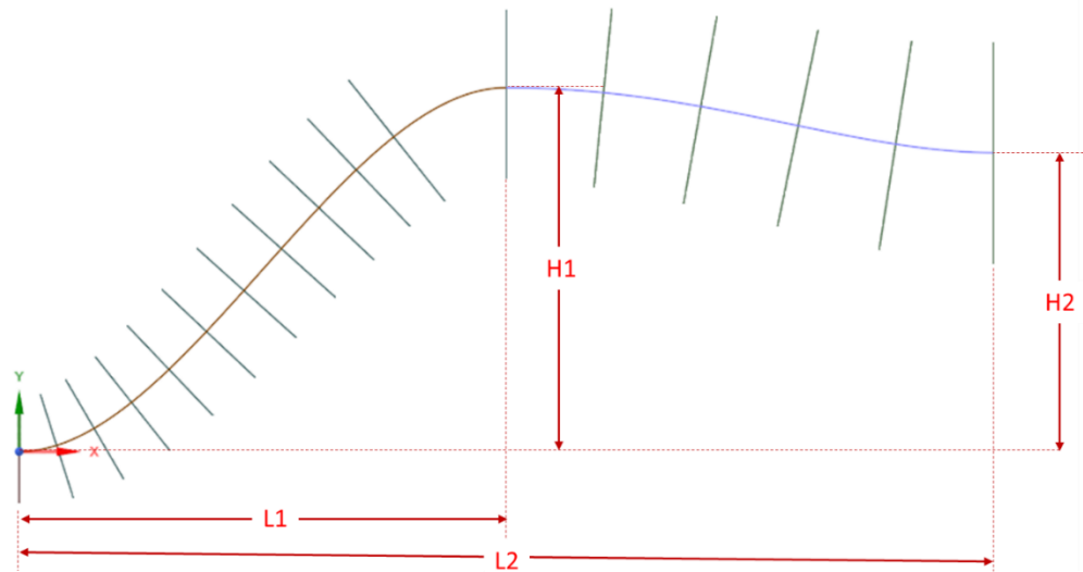
Figure 2.11. 2 nd Duct Dimensional Parameters
