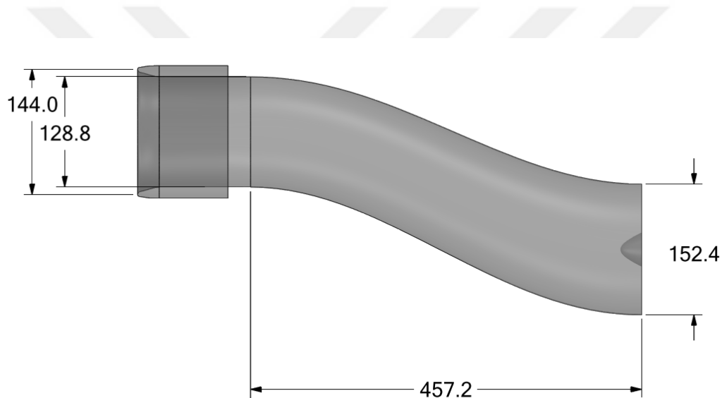
Figure 3.1. RAE M2129 Model (dimensions in mm)
