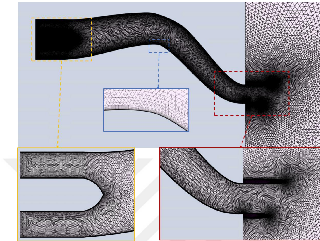
Figure 2.16. Sample Mesh with Refinement Regions
