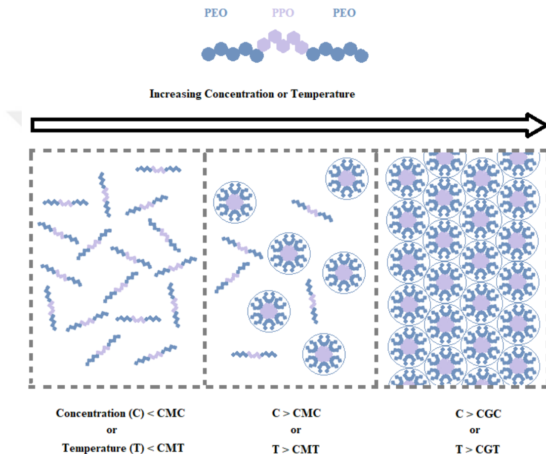
Figure 1.2.1.4. Due to the increasing concentration and temperature surfactants firstly micelle and then gel formation (Cho, 2009).
