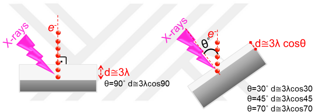
Scheme 2. Schematic representation of Angle Resolved XPS and the sampling depth.
