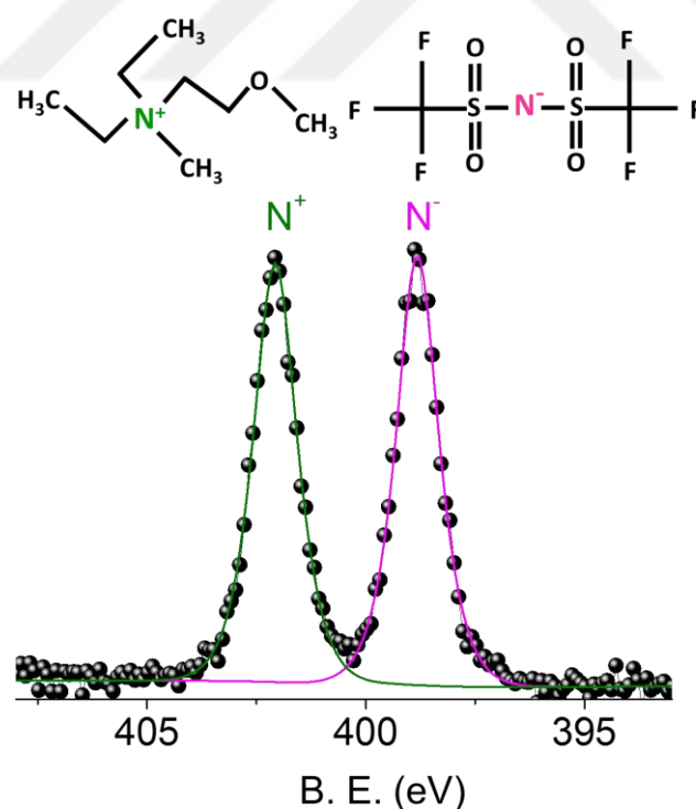
Figure 15. N1s core level XP spectra of DEME- TFSI representing molecular structure and well-resolved two different nitrogen species.
