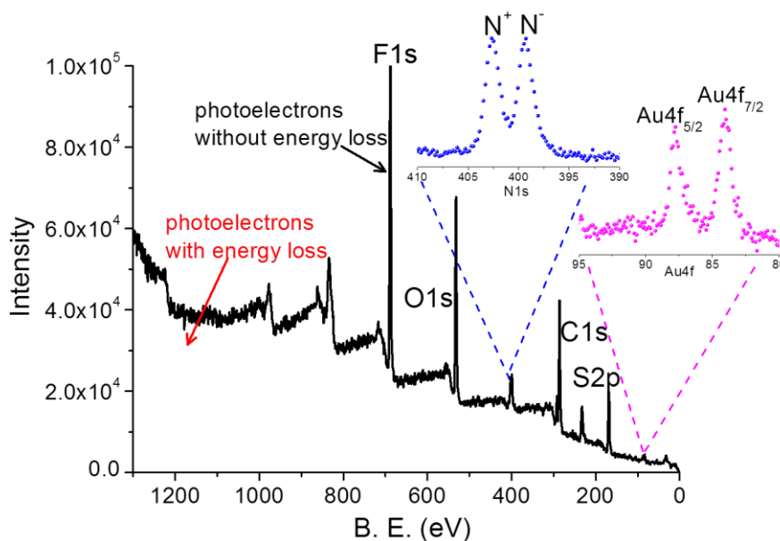
Figure 5. XP survey of DEME-TFSI on Au-electrode representing the photoelectrons' contribution to the spectrum and the detected elements. High resolution Au4f and N1s regions are given inlet.
