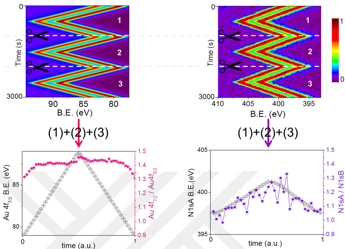
Figure 29. Time-resolved Au4f and N1s spectral regions while the recorded in the forward direction while a 5 V TRW excitation is imposed from one of the metal electrodes and extracted B.E. positions of the Au4f 7/2 and N1sA peaks, together with computed intensity ratio.
