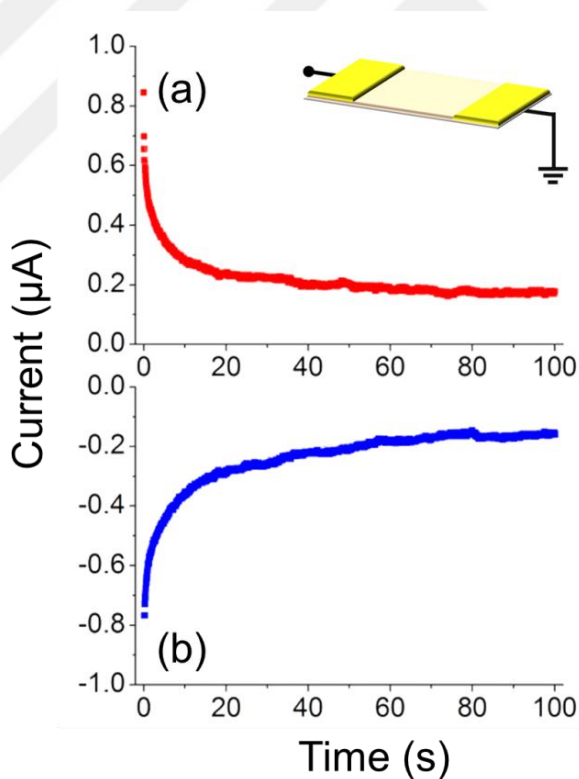
Figure 23. Measurement of current with respect to time for (a) +3V to 0V and (b) -3V to 0V potential application.
