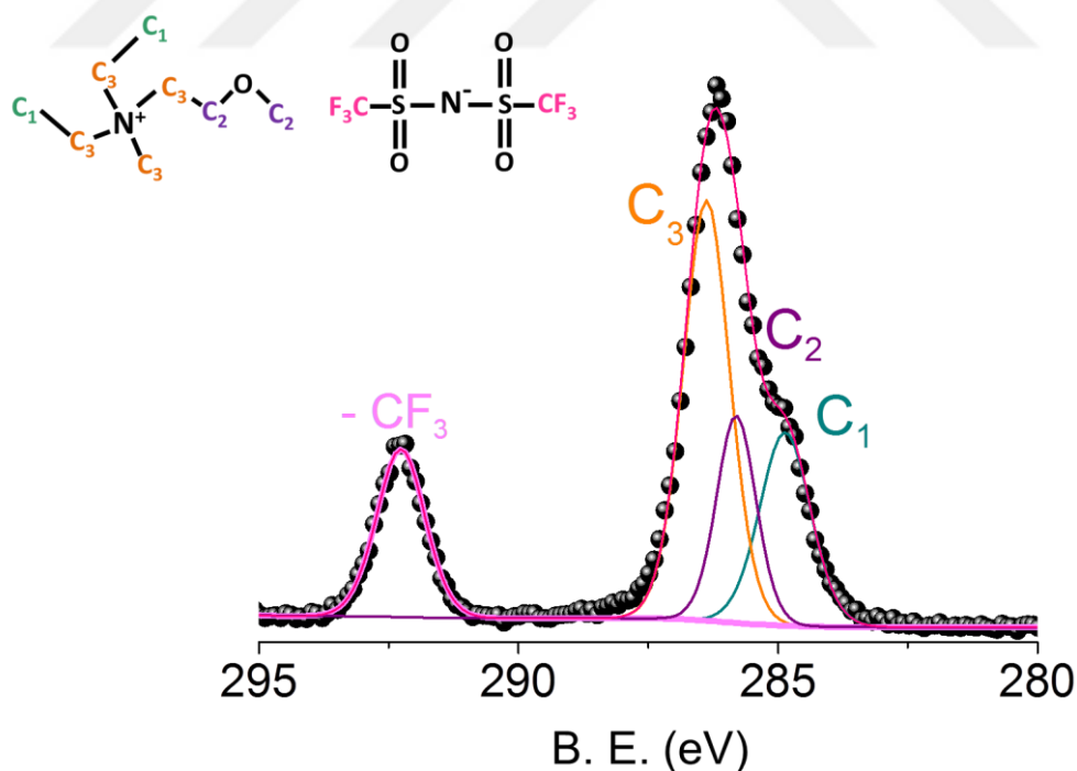
Figure 16. C1s region of DEME-TFSI.
