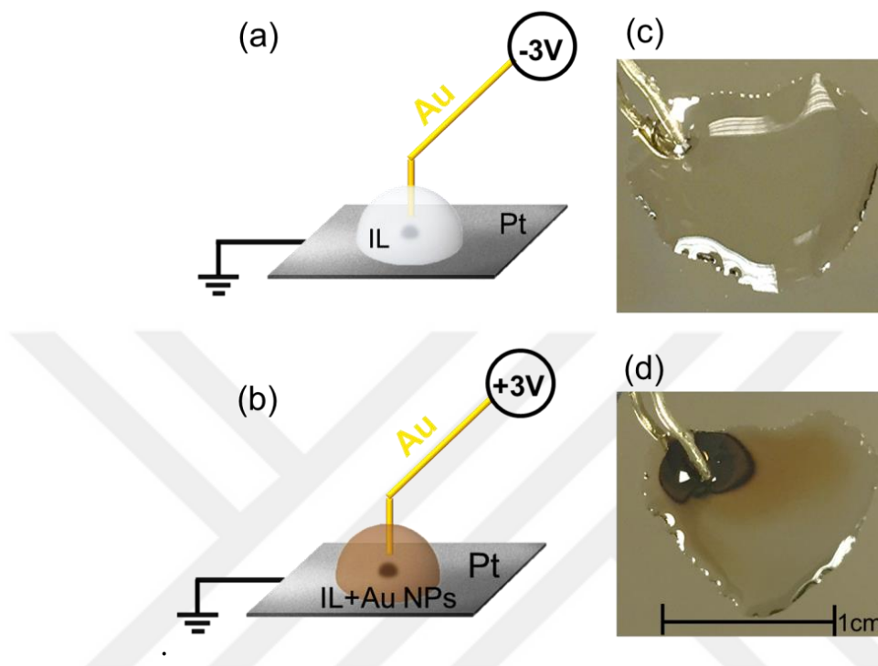
Figure 35. Schematic representation of experimental set-up corresponding (a) -3V (b) +3V potential application to Au-electrode. Images of the devices after ~60 hours under (c) -3V and (d) +3V external stress.
