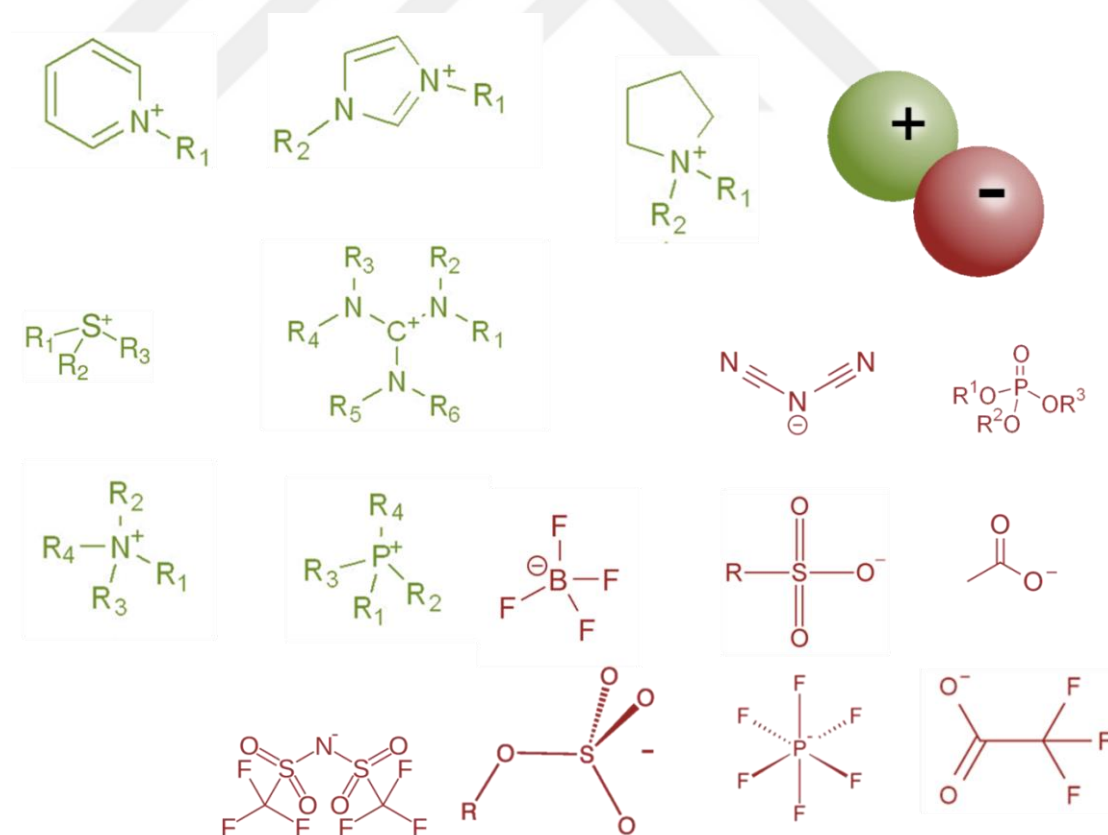
Figure 2. Chemical structures of common cations and anions of ILs.
