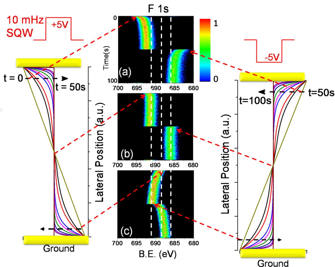
Figure 21. Time-resolved XP spectra of F1s region under 10 mHz 5V SQW excitation and recorded at three different lateral positions, corresponding (a) point1, (b) point 4 and (c) point 9 in Figure 20. Schematic representation of potential changes along the channel for positive (left) and negative (right) cycles. “Reproduced by permission of the PCCP Owner Societies. http://pubs.rsc.org/en/content/articlelanding/2016/cp/c6cp04933h#!divAbstract ”
