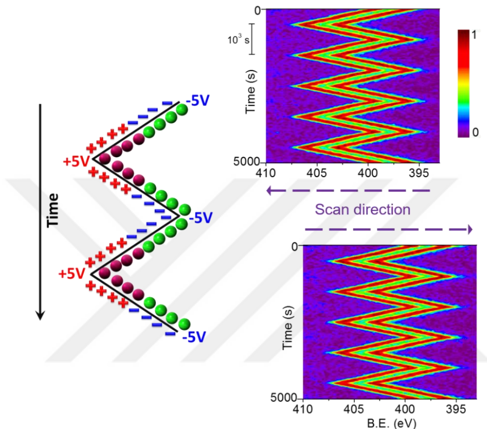
Figure 27. Time-resolved N1s spectral region while the recorded in the forward and reverse directions, while a 5 V TRW excitation is imposed from one of the metal electrodes. The responses of cationic (pink) and anionic (green) fragments to imposed potential change are illustrated.
