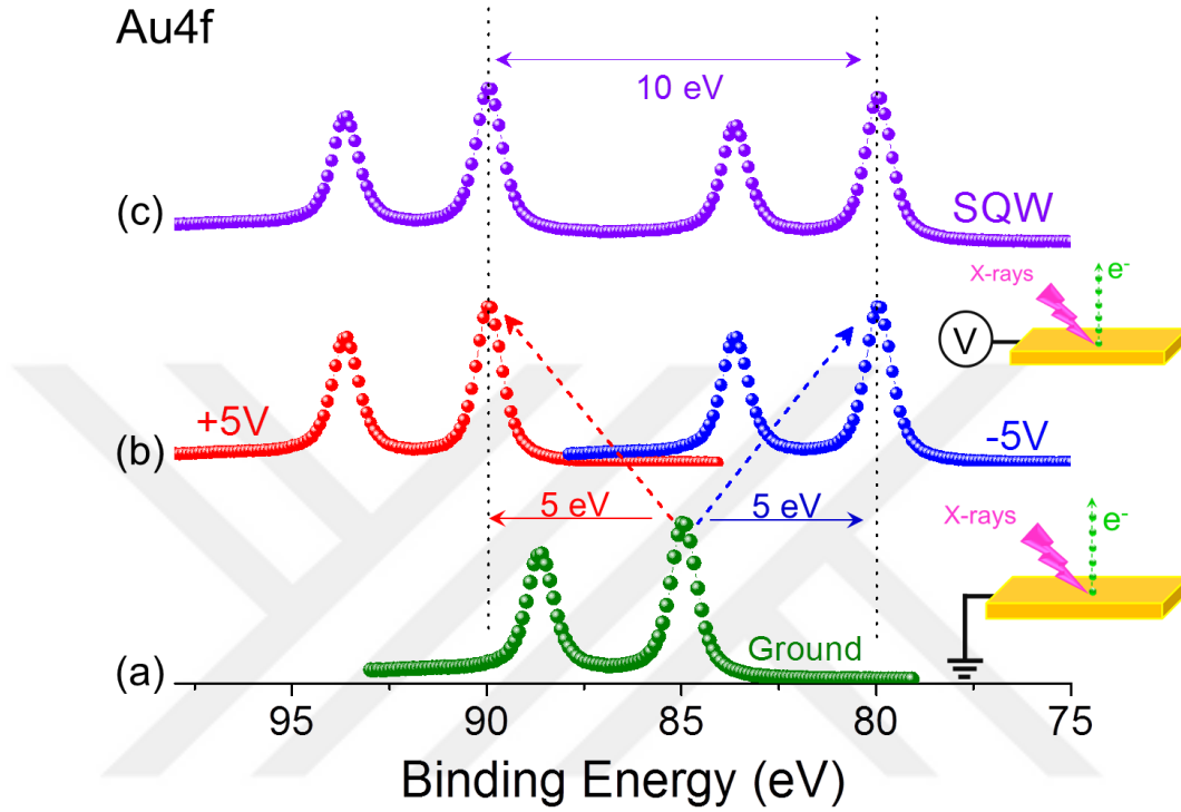
Figure 7. XPS spectra of a conducting gold metal's Au4f region when sample is (a) grounded, (b) subjected to +5V and -5V D.C. voltage bias and (c) SQW excitation of 5V amplitude with 1 kHz frequency.
