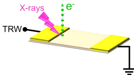
Figure 25. Schematic illustration of (a) preparation and impregnation of device (b) XPS analysis in source and drain geometry.
