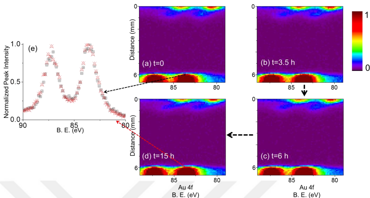
Figure 33. XP spectrum of Au4f region, recorded in the line scan mode from source towards drain electrodes;(a)at the beginning of the experiment ( t=0 ), after (b)3.5 hours ( t=3.5 h),(c) 6 hours ( t=6 h) and (d)15 hours ( t=15 h) during the continuous application of +3V D.C. external potential. (e) Au 4f spectra, normalized in intensity, acquired from the position d=6.0 mm at the beginning of -3V experiment (black) and after 15 hours (red).
