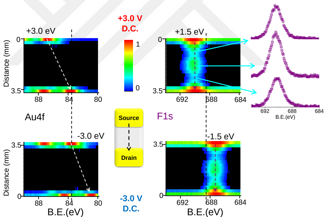
Figure 18. XP spectra of Au4f and F1s regions, recorded in the line scan mode between the two gold electrodes, containing a porous polymer film impregnated with the ionic liquid DEME-TFSI, under the application of +3 (upper part) or -3V (lower part) D.C. bias. The IL is thicker in the middle of the device as reflected by the intensity of the F1s spectra chosen at three representative positions along the line, shown as insets.
