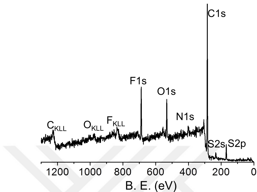
Figure 13. Typical XP survey of ionic liquid DEME-TFSI
