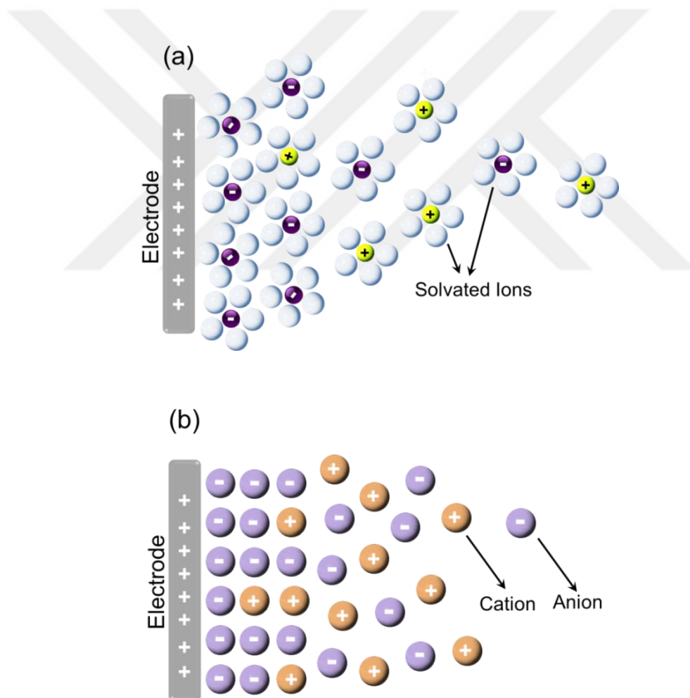
Figure 3. Schematic representation of (a) Classical EDL model and (b) EDL model for ILs.
