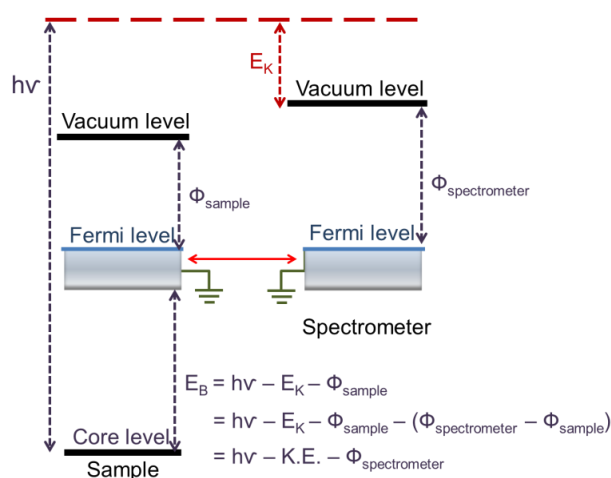
Scheme 1. Schematic illustration of relation between the energy levels and the work function in XPS for the sample (left), the spectrometer (right).
