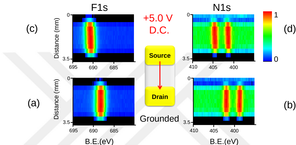
Figure 17. XP Line Scan spectra of F1s and N1s regions between the electrodes when grounded (a) - (b) and when +5 V is applied to one of the electrodes (c) - (d). N1s region has two peaks corresponding to N - and N + moieties.
