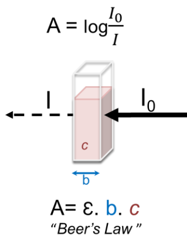
Figure 4. Schematic representation corresponding to adsorption of incoming radiation I_0 through a solution and transmitted light I .
