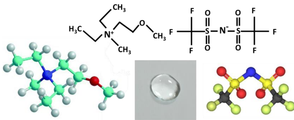
Figure 12. N,N – Diethyl - N - methyl - N - (2-methoxyethyl) ammonium bis (trifluoromethanesulfonyl) (DEME-TFSI) and its molecular structure.
