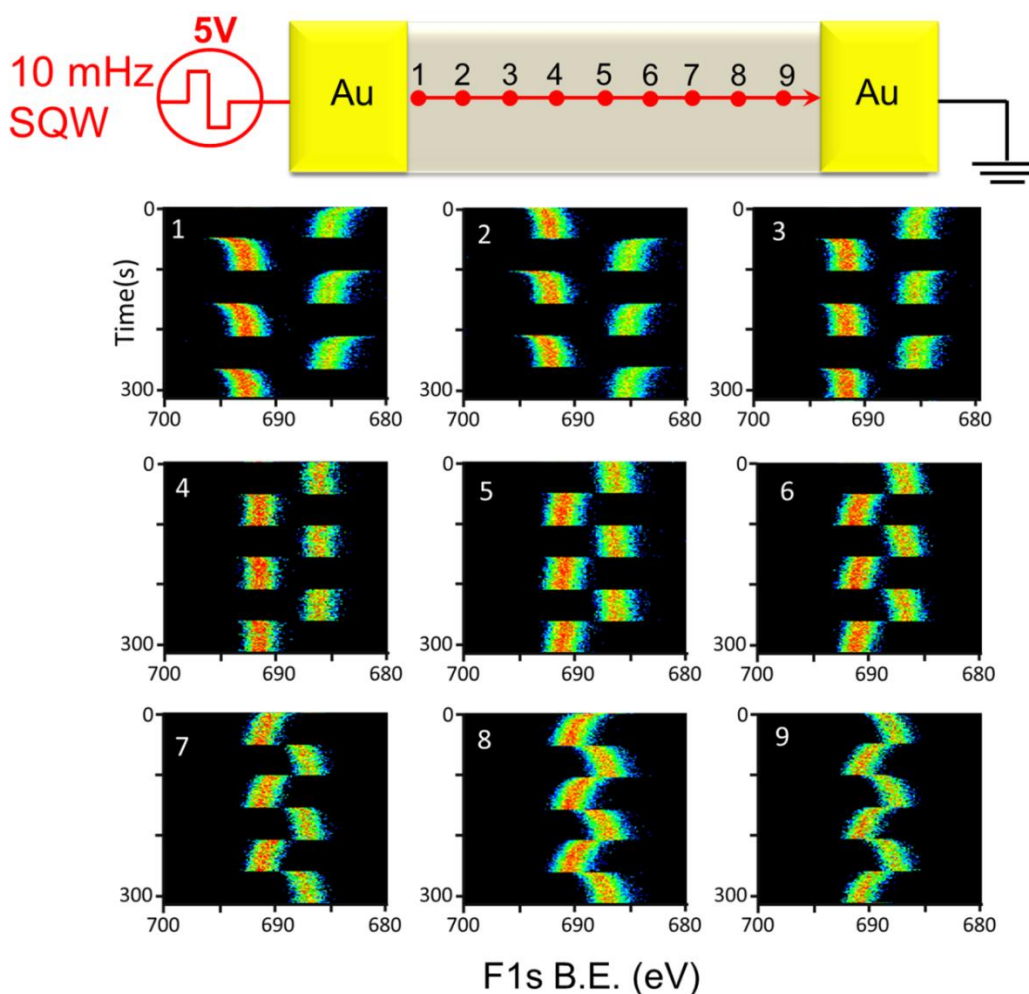
Figure 20. Time-resolved F1s XP spectra recorded at nine different lateral positions across the metal electrodes with 800 \mu\text{m} step-size between each point. Reproduced by permission of the PCCP Owner Societies. http://pubs.rsc.org/en/content/articlelanding/2016/cp/c6cp04933h#!divAbstract ”
