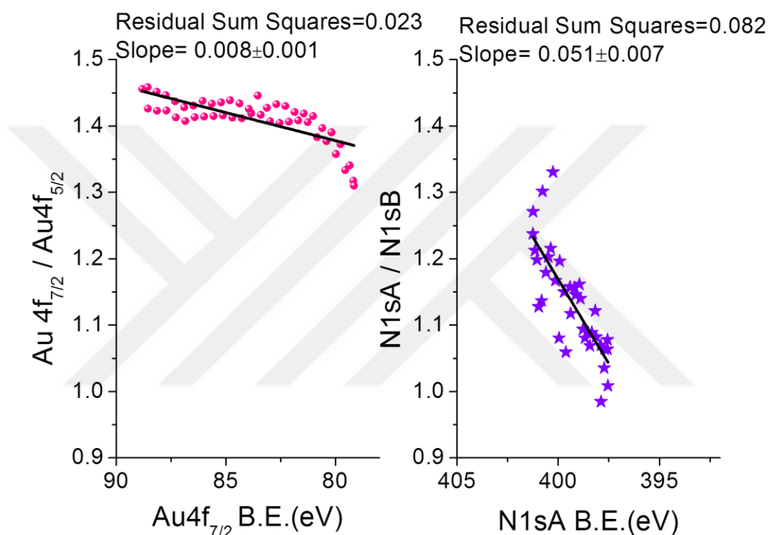
Figure 30. Evaluated data for Au4f and N1s spectral regions representing the residual sum of squares and slopes together with standard deviations.
