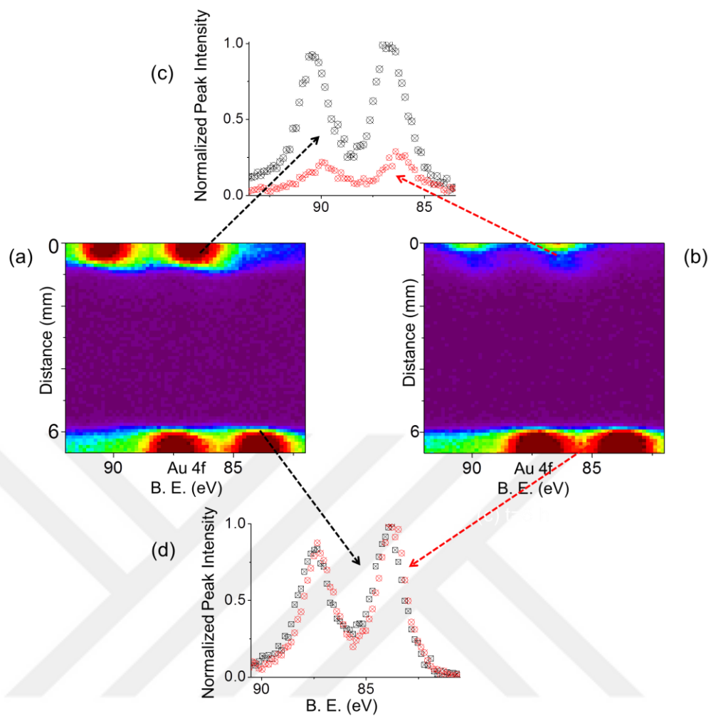
Figure 32. XP line spectrum recorded (a) at the beginning of experiment and (b) after 14 hours same in the Figure 31 (a) and (d). Normalized Au 4f spectra from the two points on the line at different positions are given in; (c) at 500 \mu\text{m} and (d) at 6000 \mu\text{m} away from the polarized electrode.
