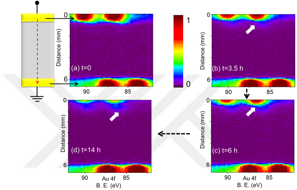
Figure 31. XP spectrum of Au4f region, recorded in the line scan mode from source towards drain electrodes;(a)at the beginning of the experiment (t=0), after (b)3.5 hours (t=3.5 h),(c) 6 hours (t=6 h) and (d)14 hours (t=14 h) during the continuous application of +3V D.C. external potential. Schematic illustration represents the line scan direction and the source - drain geometry including the electrical connections.
