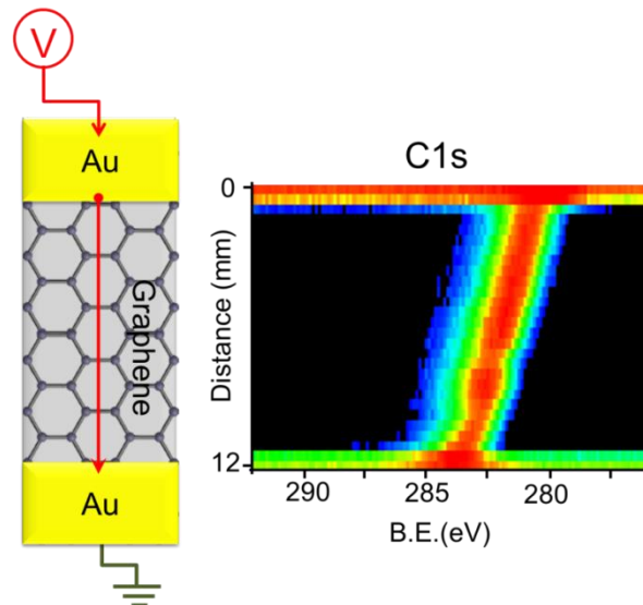
Figure 19. Schematic representation of two-electrode graphene device and smoothly varying voltage change across the electrodes when source electrode was exposed to -4V D.C. potential.
