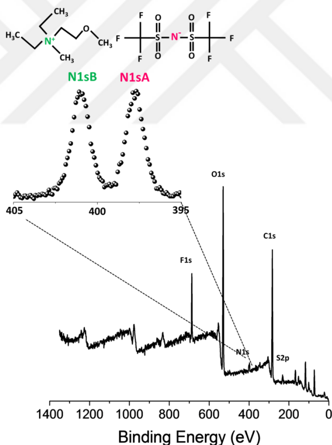
Figure 26. Survey XP spectrum of the Ionic Liquid DEME-TEFSI molecular structure and the corresponding N1s region inset.
