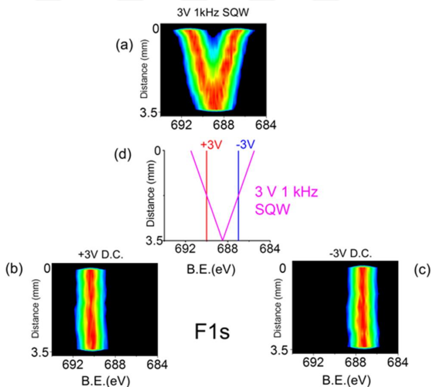
Figure 22. F1s region recorded in line scan mode across two Au electrodes under application of (a) 1 kHz SQW with amplitude of 3V (b) +3V D.C. and (c) -3V D.C. Similar data acquired. (d) Simulation of F1s binding energy positions under corresponding electrical stimulus. “Reproduced by permission of the PCCP Owner Societies. http://pubs.rsc.org/en/content/articlelanding/2016/cp/c6cp04933h#!divAbstract ”
