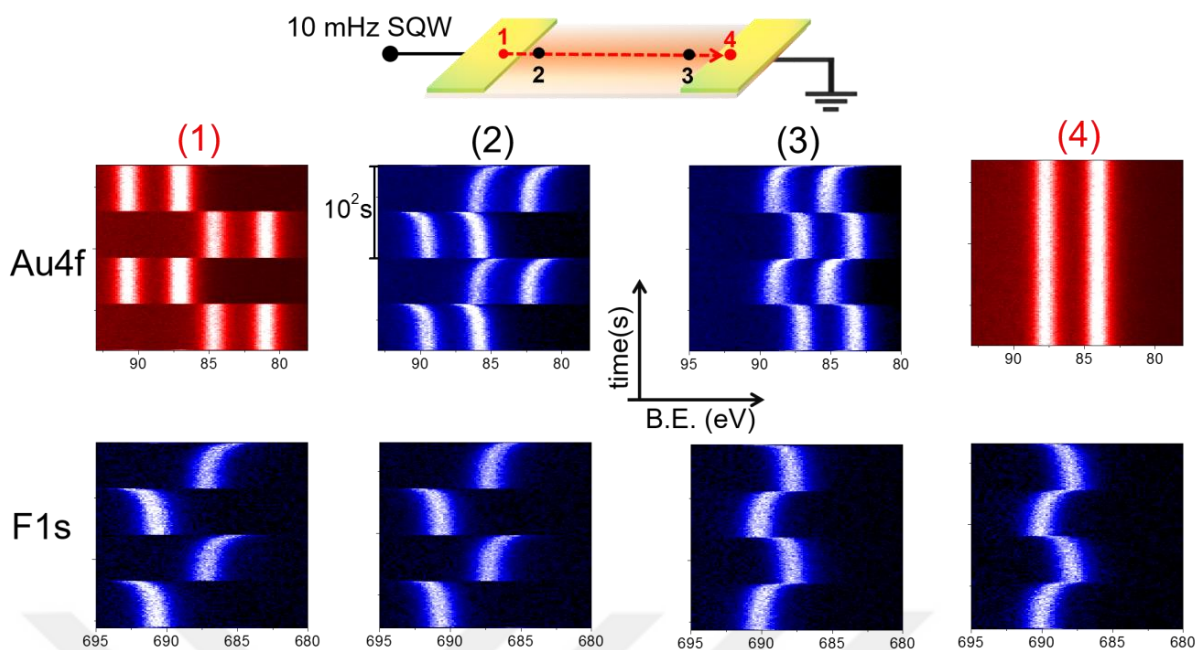
Figure 40. Time-resolved XP spectra of Au 4f and F1s regions under 10 mHz SQW excitation and recorded at four different lateral positions.
