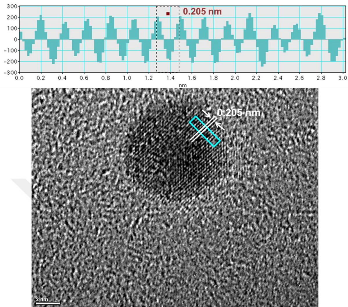
Figure 38. TEM image of Au NPs in DEME-TFSI and the distance profile on top from the marked region.
