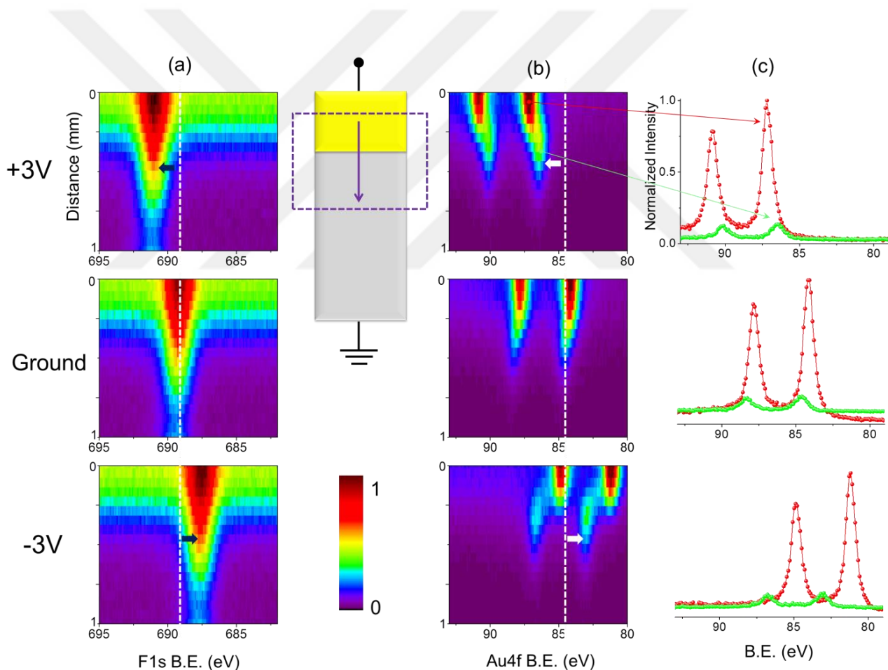
Figure 34. XPS spectra of (a) F1s and (b) Au4f region in line scan mode along 1 mm from the source - electrode point recorded under application of +3V, 0V (grounded) and -3V D.C. potential. (c) Au4f XPS spectra recorded in a higher resolution ( normal scan mode ) on Au electrode (red) and at interfacial region (green).
