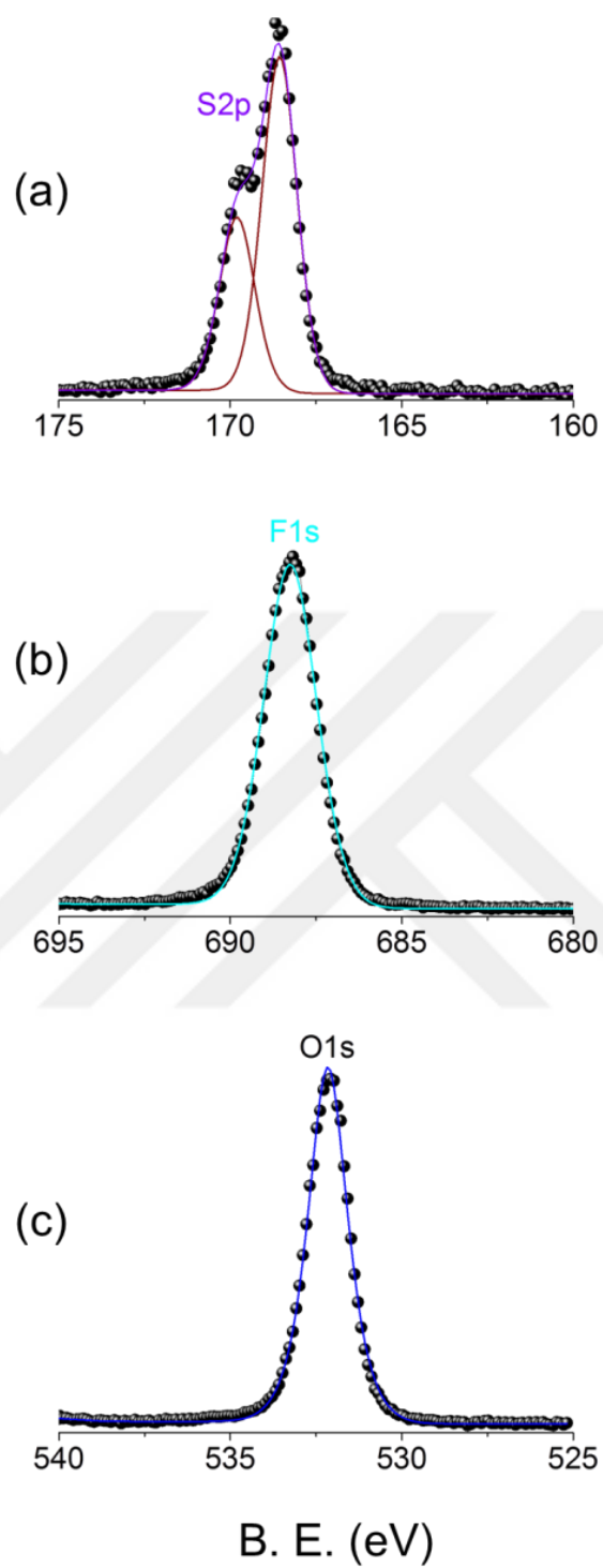
Figure 14. XP spectra of (a) S2p (b) F1s and (c) O1s regions.
