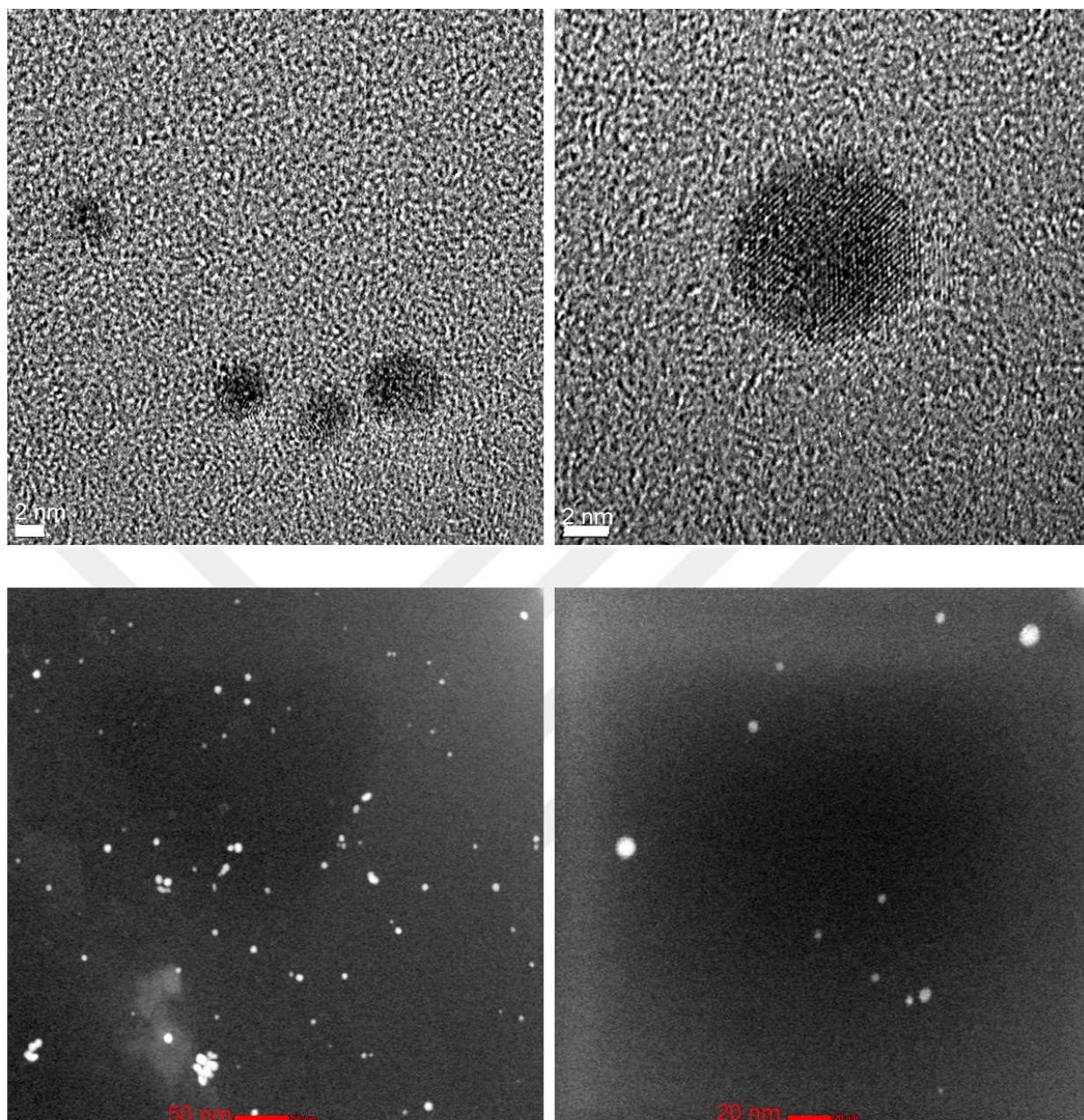
Figure 37. TEM images of Au NPs in DEME-TFSI ionic liquid.
