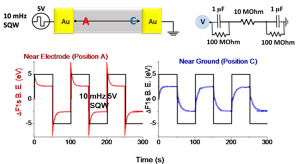
Figure 24. Simulations of potential developed at near electrode region and near ground region under 5V 10 mHz SQW. Equivalent circuit model represents the resistors and capacitors. “Reproduced by permission of the PCCP Owner Societies. http://pubs.rsc.org/en/content/articlelanding/2016/cp/c6cp04933h#!divAbstract ”
