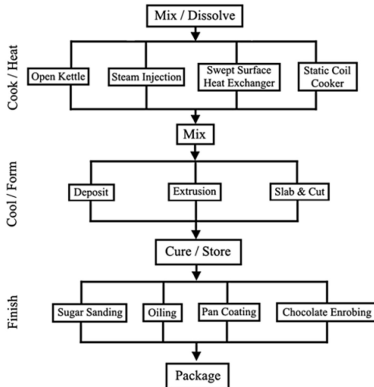
Figure 1.1. Schematic Representation of Gelatin-based Candy Production (Hartel et al. , 2018)
