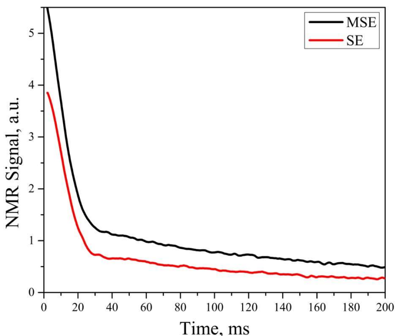
Fig. 3.9. Representative signals of SE and MSE sequences for the SCG40 (30%) samples
