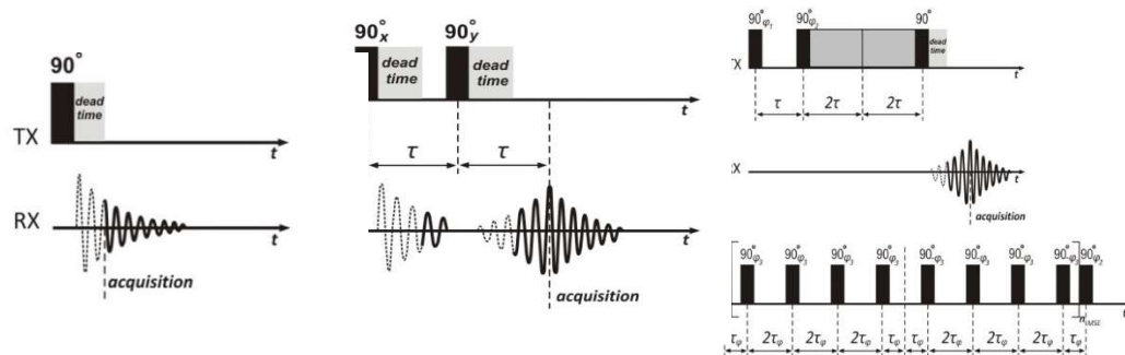
Figure 3.7. Pulse diagrams for FID, SE and MSE Sequences (Grunin, Oztup, Guner, & Baltaci, 2019)
