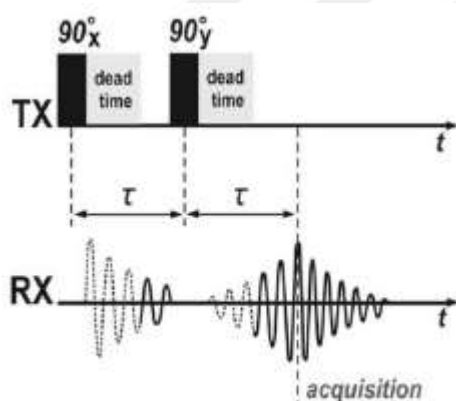
Figure 1.9. Pulse diagram of SE (L. Grunin et al., 2019) pulse sequence
