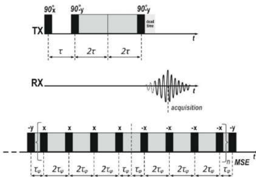
Figure 1.10. Pulse diagram of MSE (L. Grunin et al., 2019) pulse sequence
