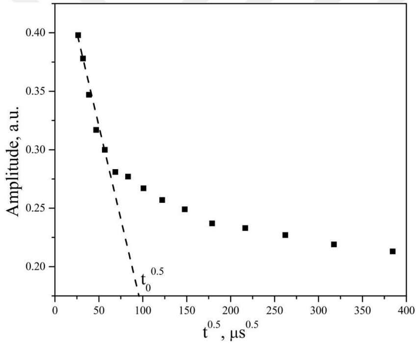
Fig. 3.10. An example of the determination of the parameter t^{0.5} in Goldman-Shen Experiment
