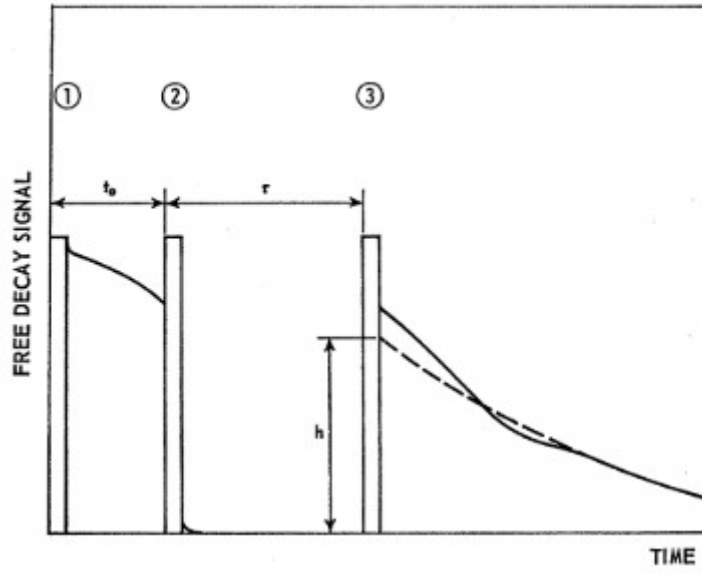
Figure 1.11. Goldman-Shen pulse sequence to study spin diffusion (Goldman & Shen, 1966)
