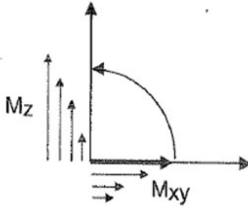
Figure 1.5. Recovery of longitudinal component while transverse magnetization vector decays (Hashemi, 2010)
