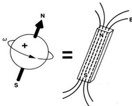
Figure 1.3. The charged nucleus rotating with angular frequency \omega with the spin rotation axis (Hashemi, 2010)
