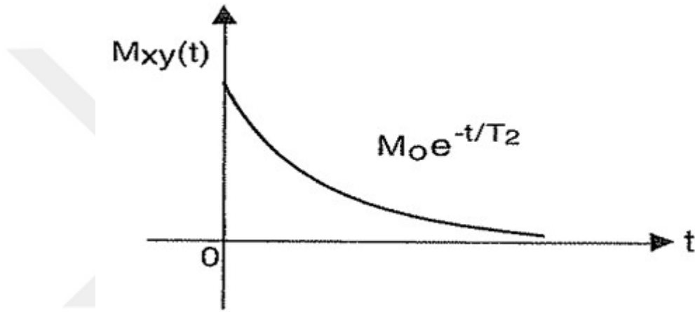
Figure 1.7. Decay of the transverse magnetization (Hashemi, 2010).
