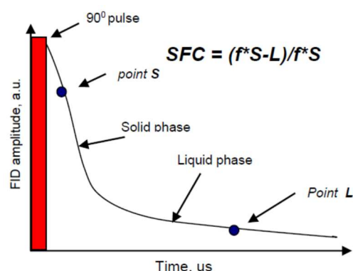
Figure 3.6. A representative FID signal and SFC
