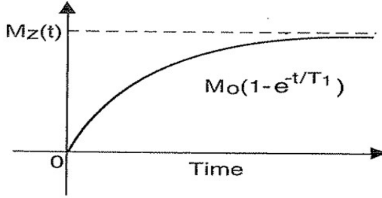
Figure 1.6. Recovery longitudinal magnetization (Hashemi, 2010).
