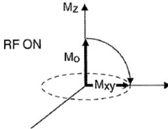
Figure 1.4. Flipping of the longitudinal magnetization vector into the x-y plane (Hashemi, 2010)
