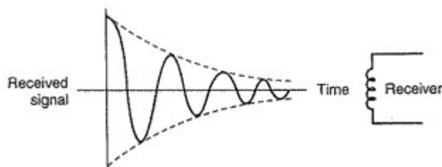
Figure 1.8. The decaying sinusoidal waveform of the received signal (FID) (Hashemi, 2010)
