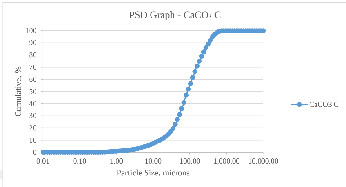
Figure 4.3. \text{CaCO}_3 C PSD Analysis
