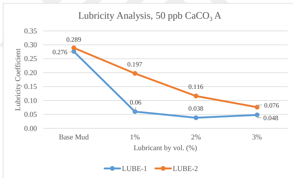
Figure 5.7. Lubricity Performance Analysis, 50 lb/bbl CaCO 3 A
