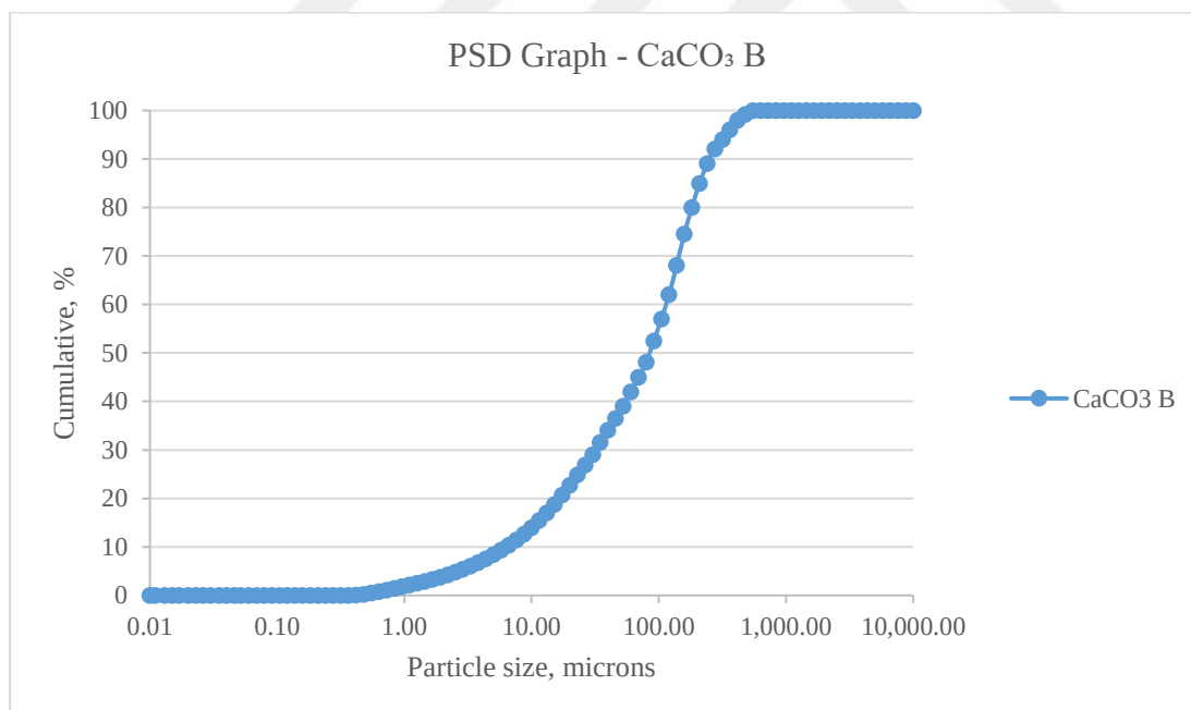
Figure 4.2. CaCO 3 B PSD Analysis
