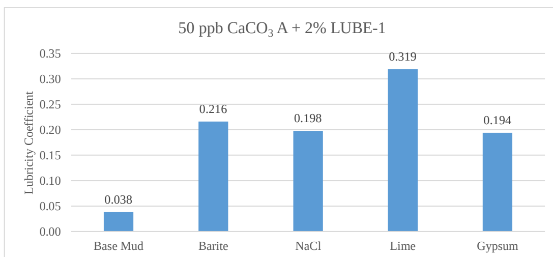
Figure 5.15. Lubricity Coefficient Comparison (50 ppb \text{CaCO}_3 A + 2% LUBE-1)
