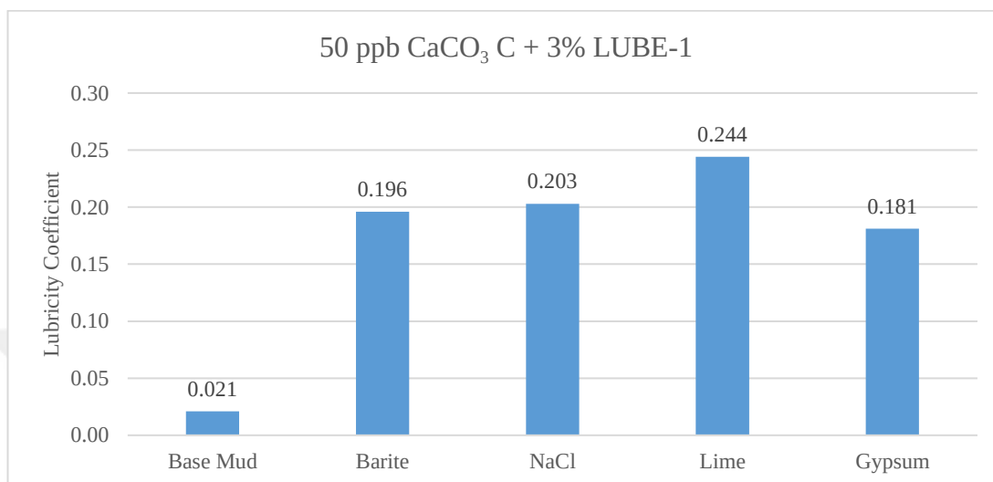
Figure 5.17. Lubricity Coefficient Comparison (50 ppb \text{CaCO}_3 C + 3% LUBE-1)
