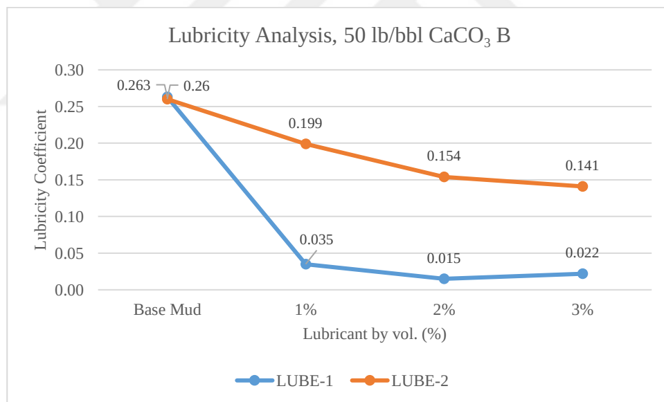
Figure 5.9. Lubricity Performance Analysis, 50 lb/bbl CaCO 3 B
