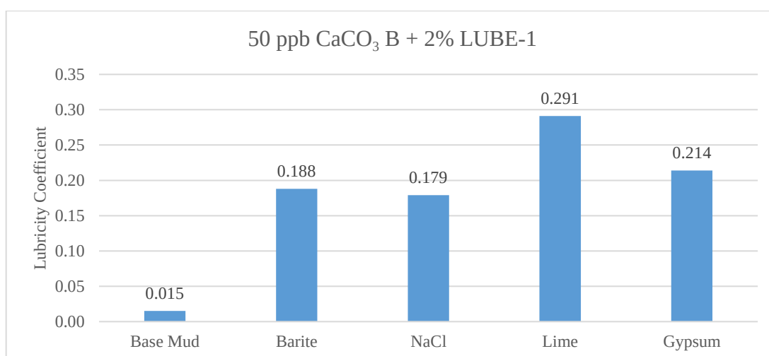
Figure 5.16. Lubricity Coefficient Comparison (50 ppb \text{CaCO}_3 B + 2% LUBE-1)
