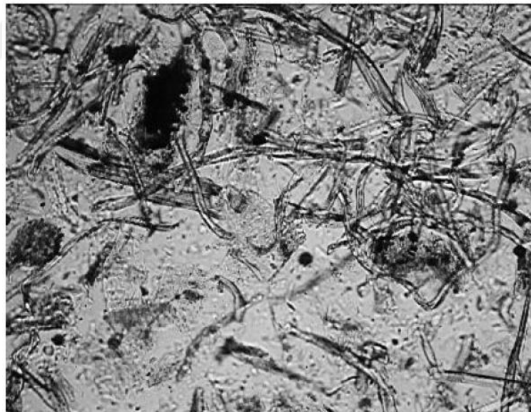
Figure 2.10. Micronized Cellulose Fibers Used in Test Data. Typical 20 micron diameter with lengths of 2 to 200 microns. (Verret et al, 2000)
