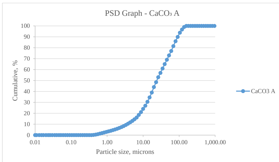
Figure 4.1. CaCO 3 A PSD Analysis
