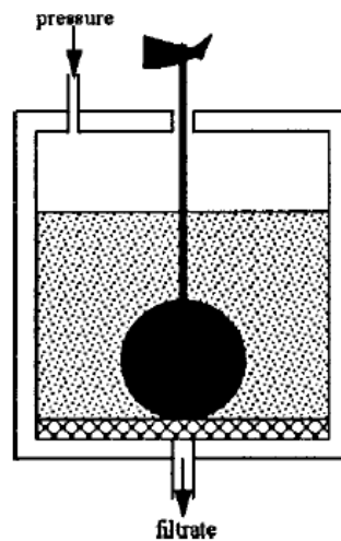
Figure 2.4. Stickance Tester. (Reid et al, 1999)
