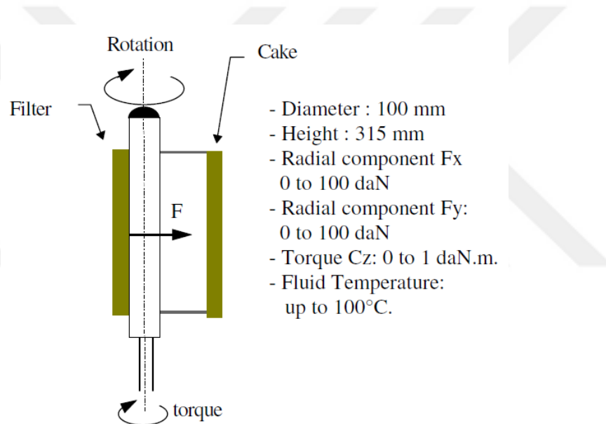
Figure 2.5. Figure and Specifications of Lubricity Captor (Isambourg et al, 1999)
