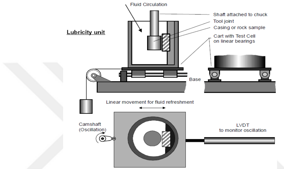
Figure 2.6. Lubricity Unit (Knox et al, 2005)
