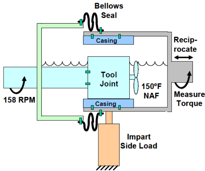
Figure 2.1. Schematic of Full-scale Lubricity Testing Device (Schamp et al, 2006)
