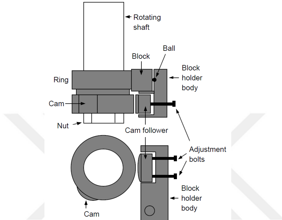
Figure 2.3. Modified lubricity tester. cross-sectional view at the bottom and side view at the top. (Skalle et al, 1999)
