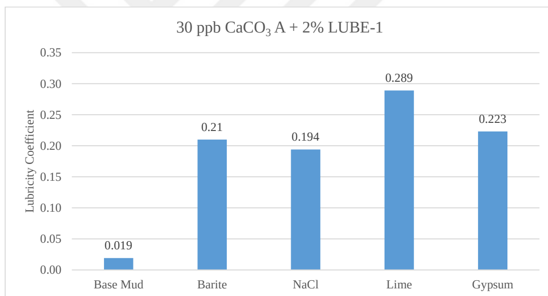
Figure 5.14. Lubricity Coefficient Comparison (30 ppb CaCO 3 A + 2% LUBE-1)
