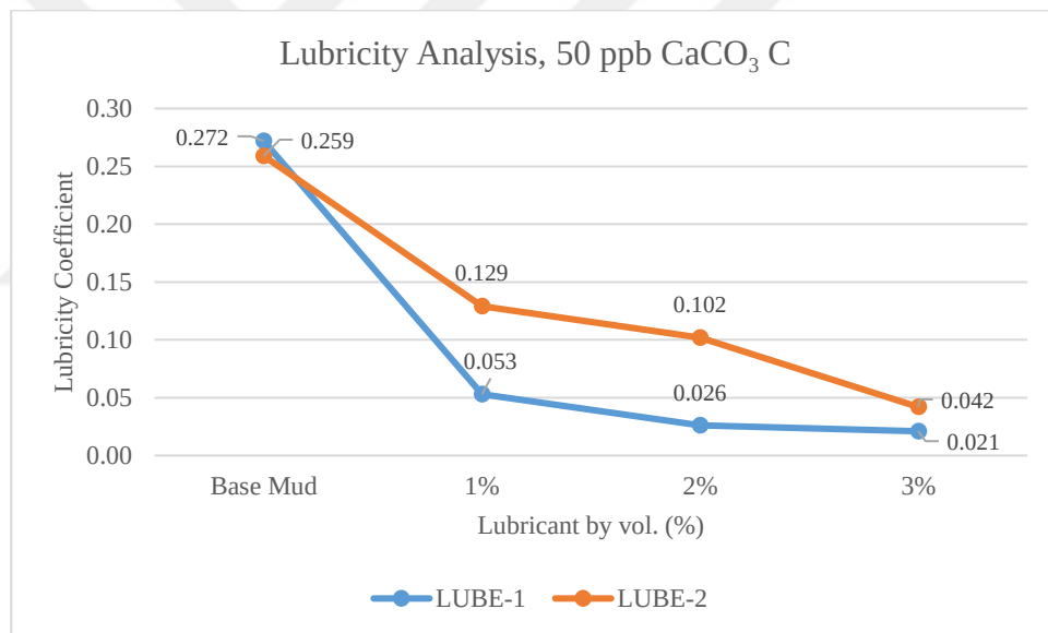
Figure 5.8. Lubricity Performance Analysis, 50 lb/bbl CaCO 3 C
