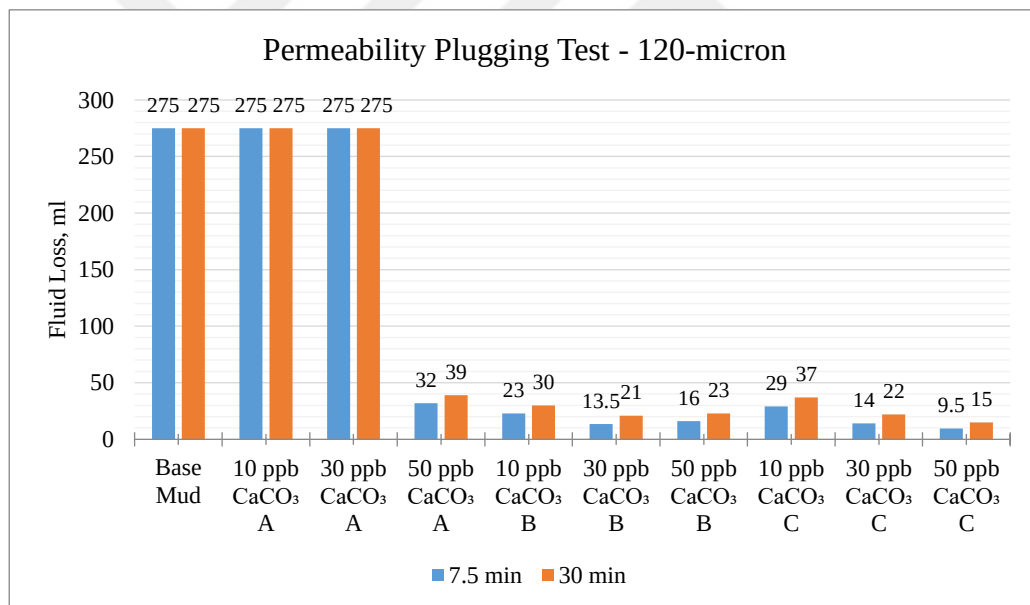
Figure 5.3. Permeability Plugging Test (120-micron)
