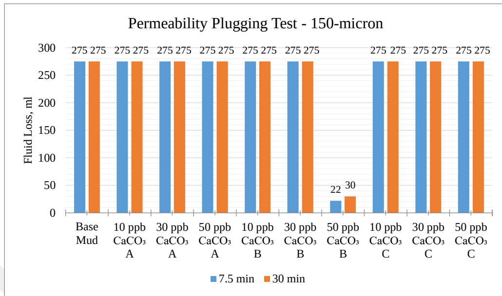
Figure 5.4. Permeability Plugging Test (150-micron)
