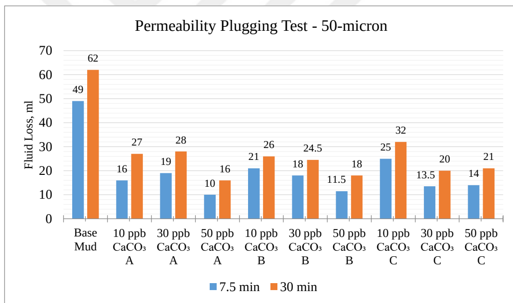
Figure 5.2. Permeability Plugging Test (50-micron)
