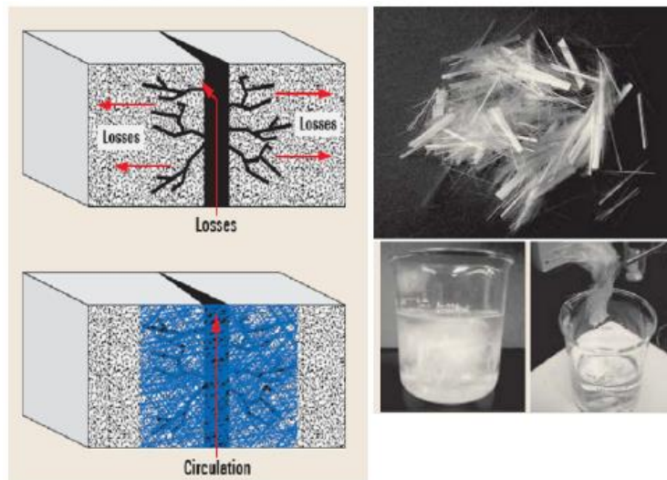
Figure 2.8. A4 Advanced Engineered Fibers (Qureshi et al, 2008)
