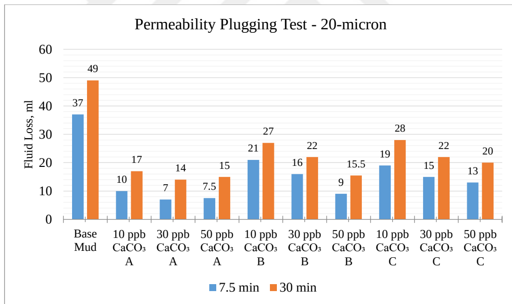
Figure 5.1. Permeability Plugging Test (20-micron)
