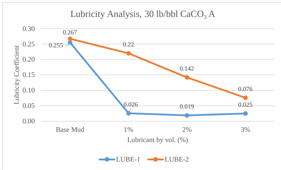
Figure 5.6. Lubricity Performance Analysis, 30 lb/bbl \text{CaCO}_3 A
