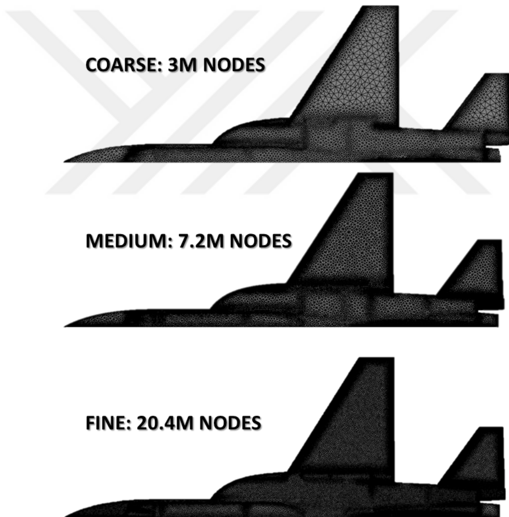
Figure 4.3: Surface Grid Densities Used in Grid Convergence Studies
