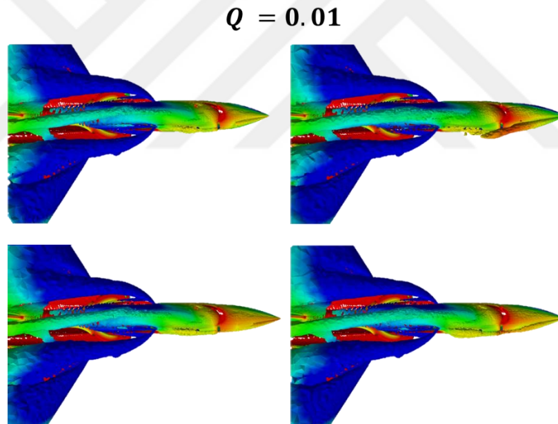
Figure 4.30: Q-criterion Iso-surfaces (TOP-VIEW) @ (0.2 Mach - 25° - AoA - 10° Beta) over the Base Configuration (Top-Left), Best Directional Stability Configuration (Top- Right), Lowest Drag Count Configuration (Bottom-Left), Moderately Optimal Configuration (Bottom- Right)
