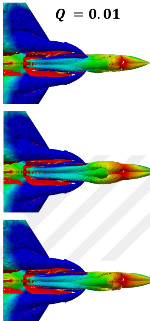
Figure 4.33: Q-criterion Iso-surfaces (TOP-VIEW) @ (0.2 Mach - 25°- AoA - 0° Beta) over the Base Configuration (Top), Best Directional Stability Configuration (Middle), Moderately Optimal Configuration (Bottom)
