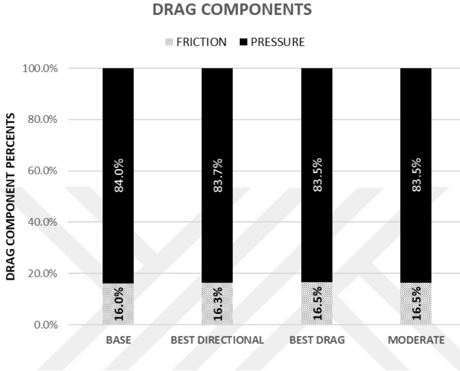
Figure 4.27: Drag Component Percentages for the Base, Best Directional Stability and Moderately Optimal Configurations
