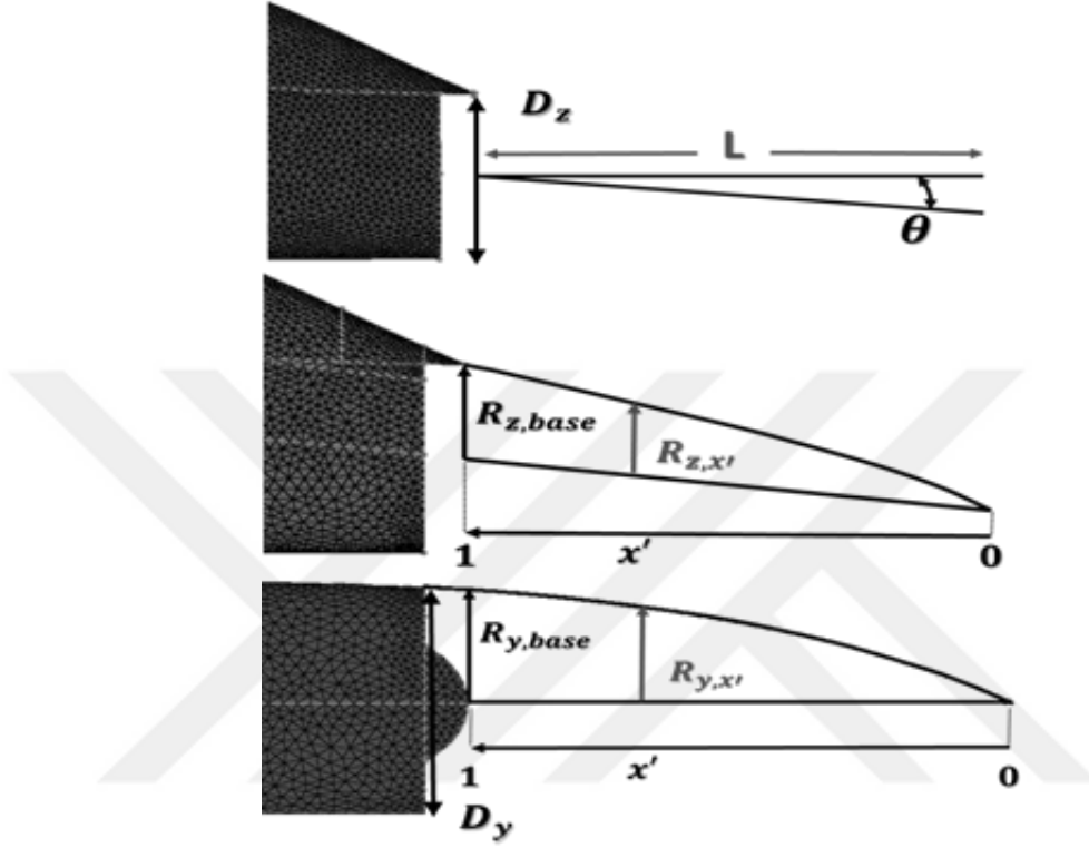
Figure 2.2: Lateral Cross-section Design Parameters
