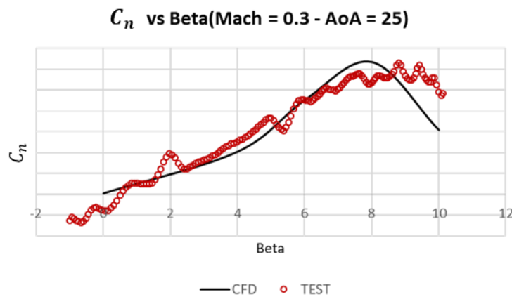
Figure 4.9: Variation of Yaw Moment Coefficient
