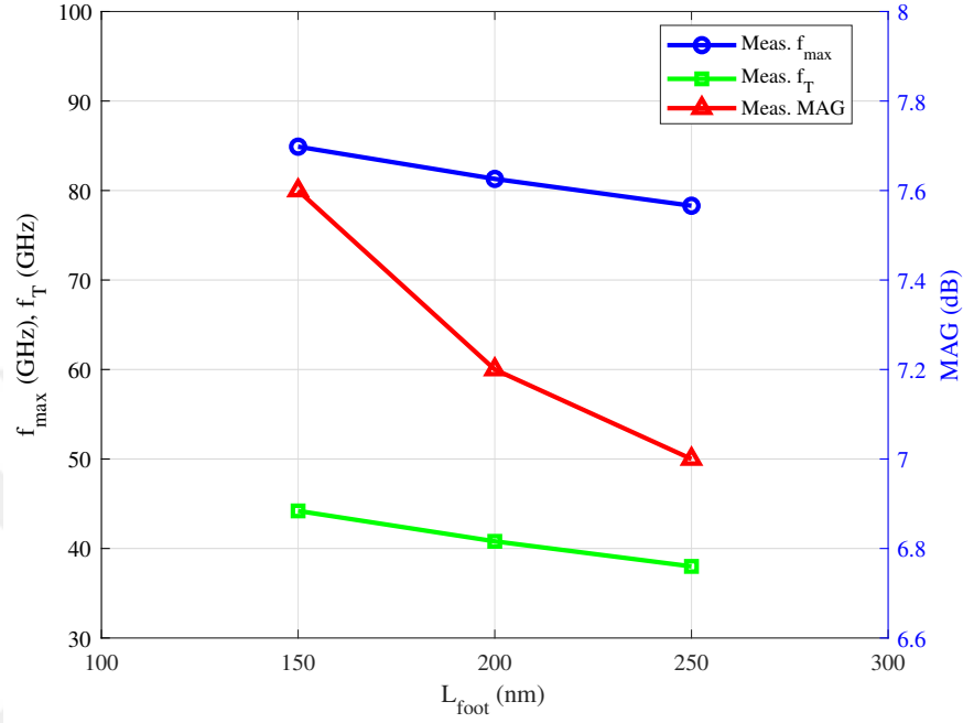
Figure 4.5: Measurement results of f_{\max} , f_T , and MAG at 35 GHz of a 4 \times 75 \mu\text{m} HEMT with 500 nm L_{\text{head}} with different L_{\text{foot}} values.
