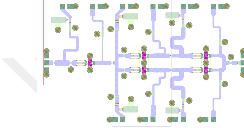
Figure 5.25: Three parts of the layout to analyze even-mode stability for each stage.
