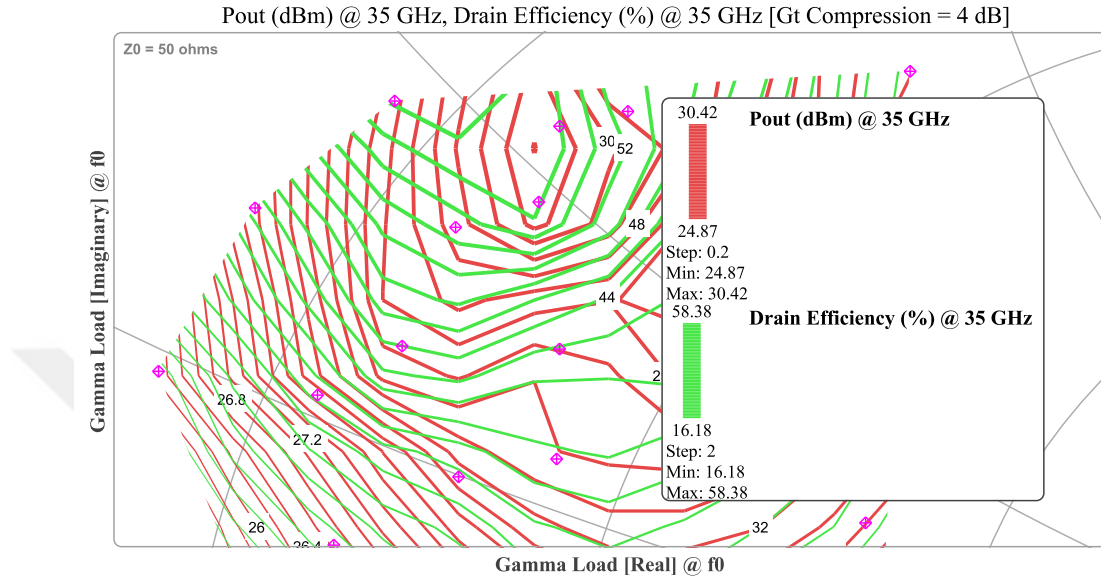
Figure 5.6: Output power and drain efficiency contours of the selected 4 \times 75 \mu\text{m} transistor at 35 GHz, drawn together.
