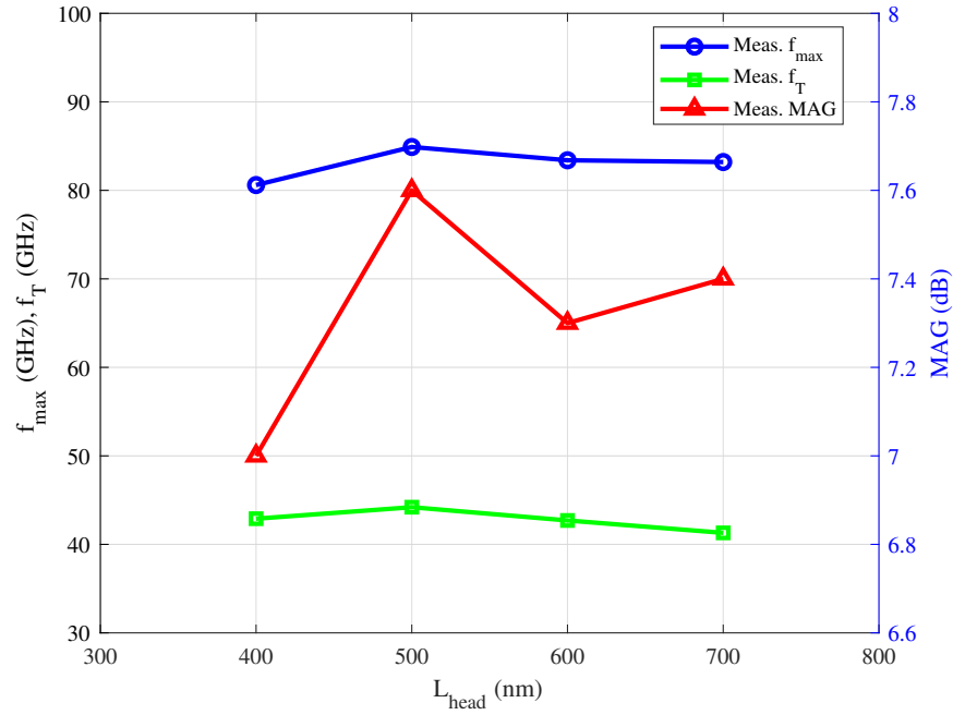
Figure 4.6: Measurement results of f_{\max} , f_T , and MAG at 35 GHz of a 4 \times 75 \mu\text{m} HEMT with 150 nm L_{\text{foot}} with different L_{\text{head}} values.
