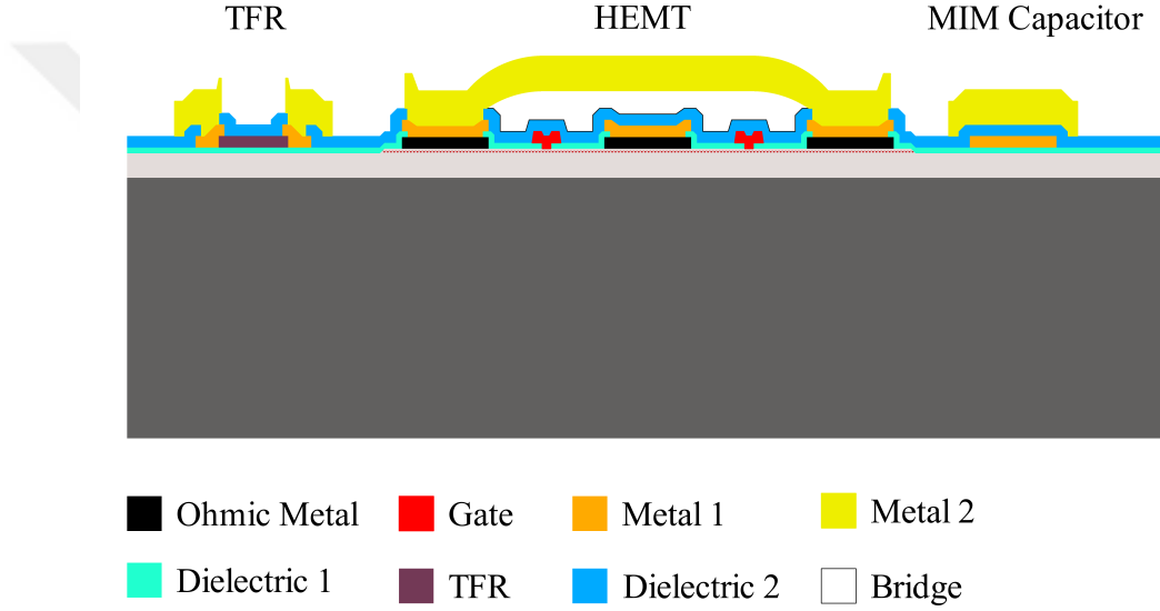
Figure 2.11: The cross-section of the structure showing the active device, MIM capacitor, and TFR.
