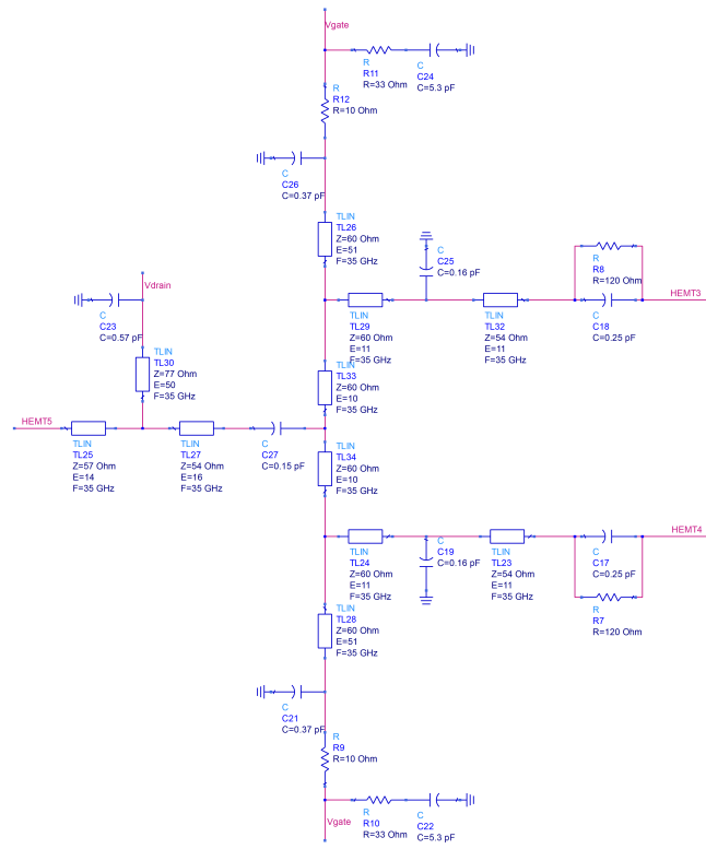
(a) Schematic
