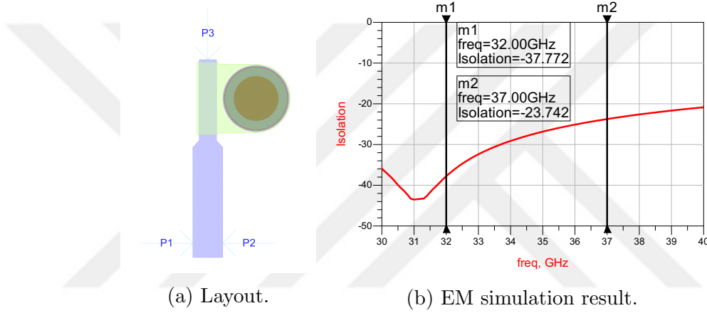
Figure 5.8: Layout and EM simulation result of drain bias network of the output stage transistors.
