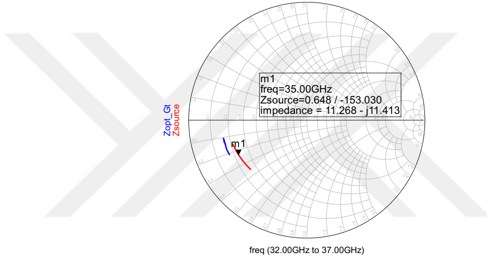
Figure 5.23: Source impedance of first stage transistors (red) and the optimum impedance for gain (blue) from 32 GHz to 37 GHz.
