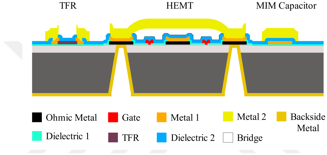
Figure 2.12: The cross-sectional view of the wafer after the back-side process.
