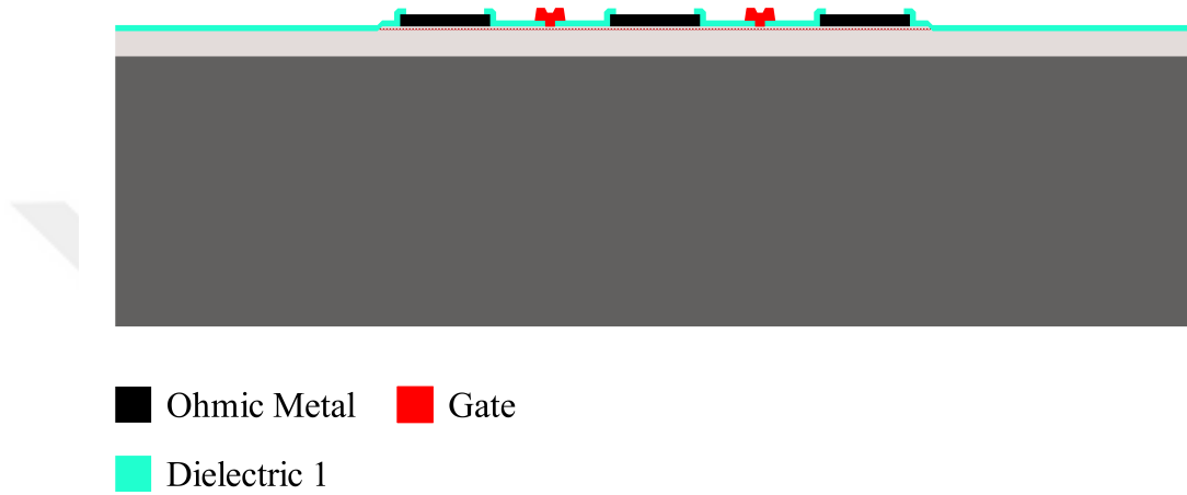
Figure 2.7: The cross-sectional view of the wafer after the gate formation.
