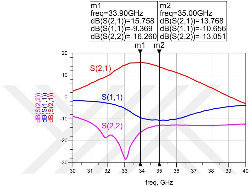
Figure 5.33: Small-signal simulation results of the final layout.
