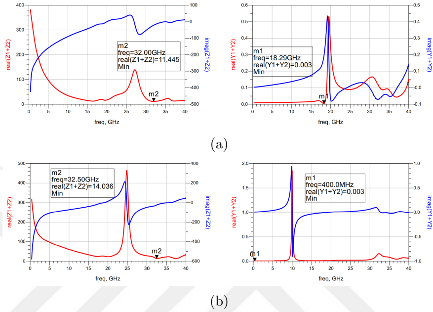
Figure 5.30: Impedance check using S-probe for even-mode stability: The sum of impedance and admittance values seen from S-probe positioned at the gate of second stage transistor (a) and at the drain of second stage transistor (b).
