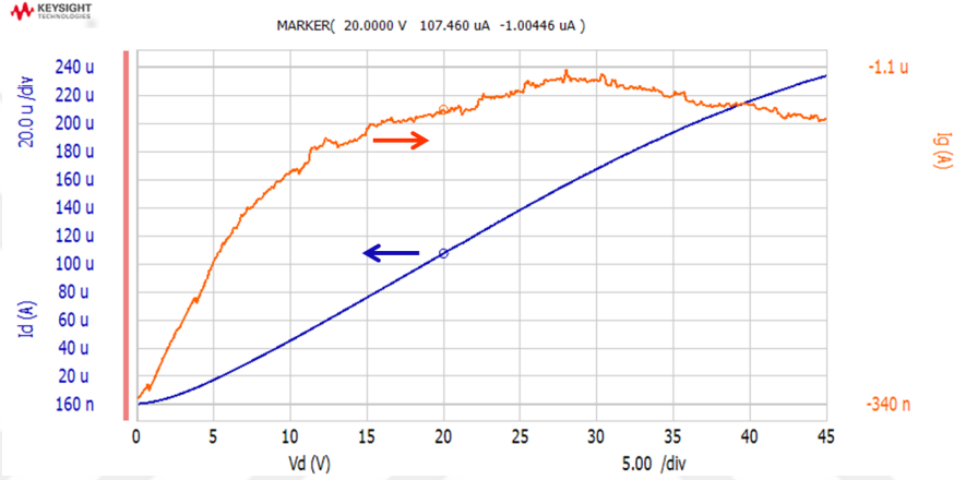
Figure 3.4: Drain and gate leakage currents of a 4\times 75\text{ }\mu\text{m} device.
