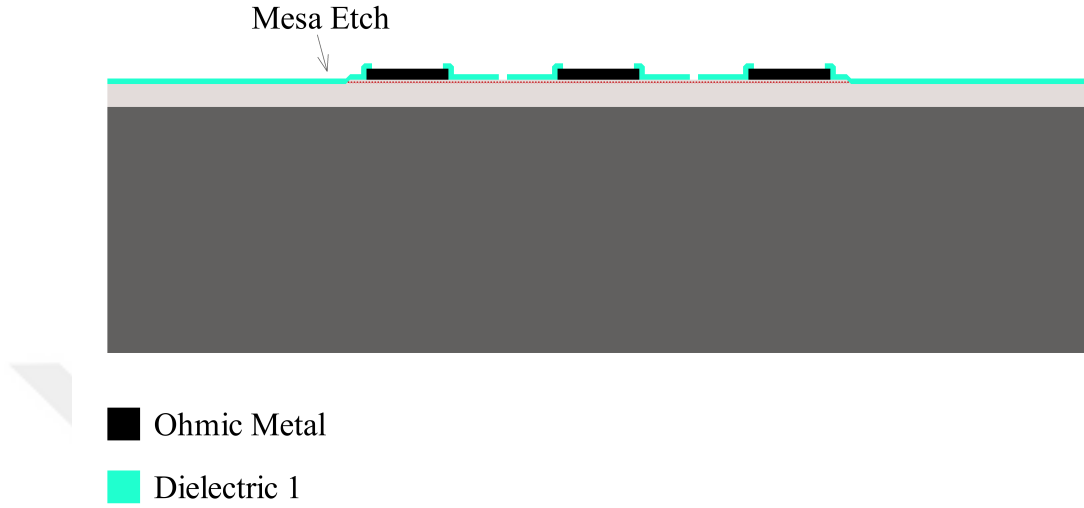
Figure 2.6: The cross-section of the wafer after mesa isolation and the first dielectric deposition.
