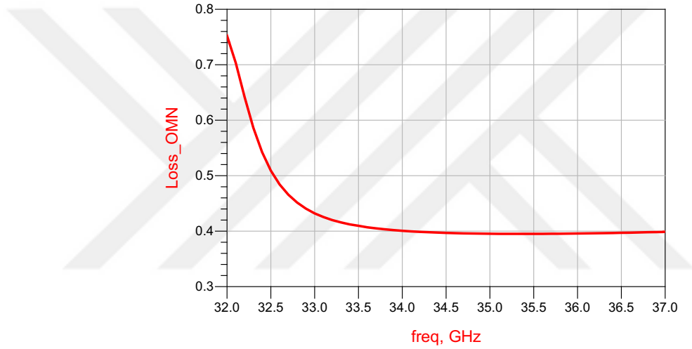
Figure 5.11: Insertion loss of the OMN from 32 GHz to 37 GHz.
