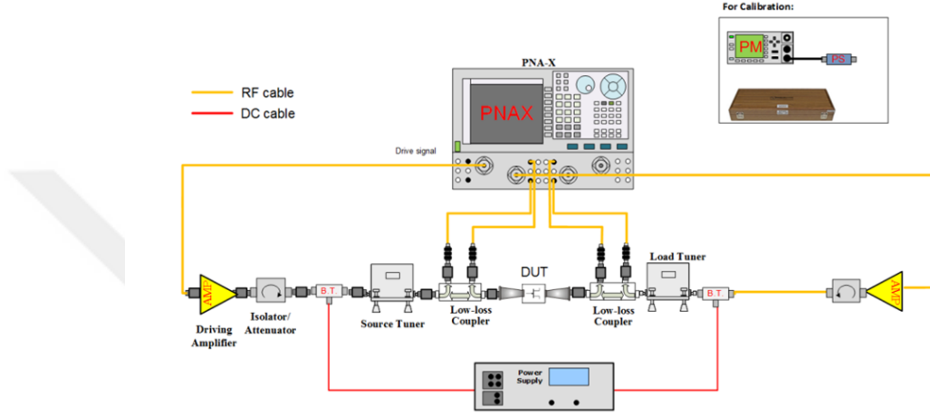
Figure 3.10: Schematic of the hybrid load-pull measurement setup.
