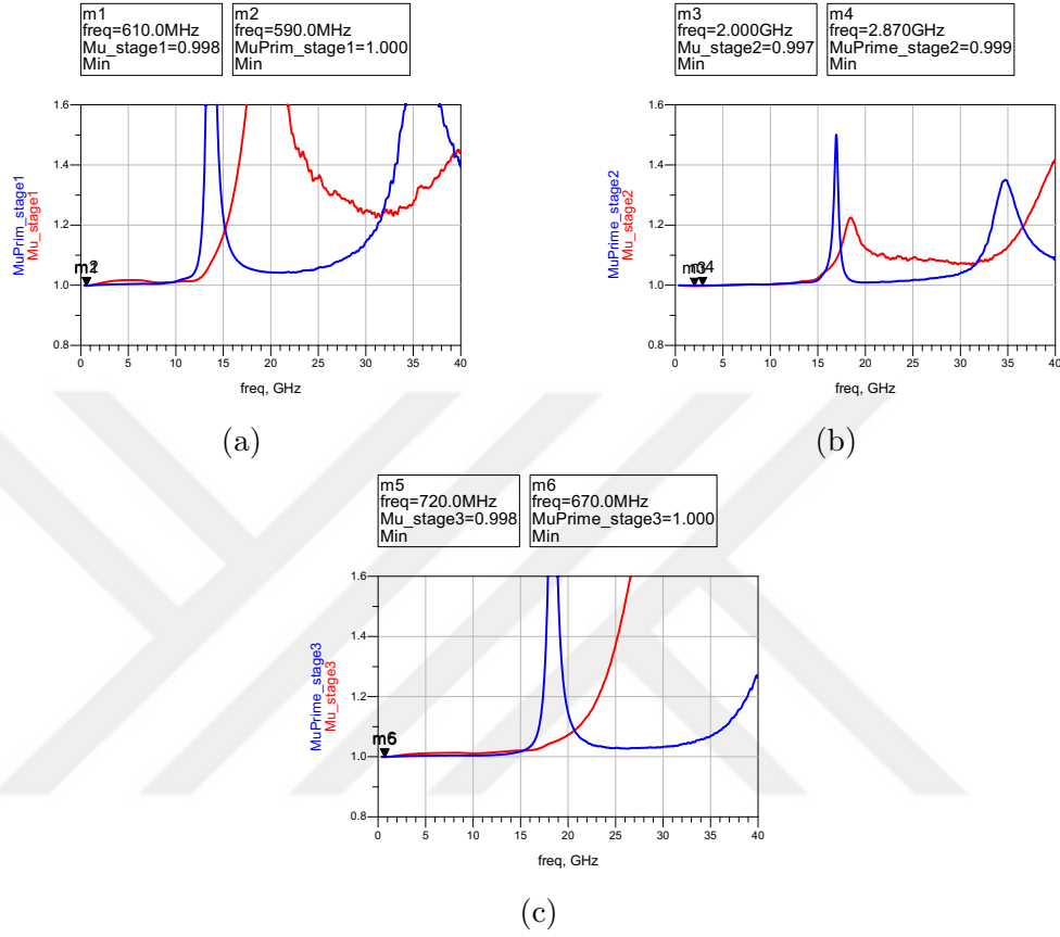
Figure 5.26: Even-mode stability results for three parts of MMIC: \mu and \mu' parameters for the first stage (a), second stage (b), and third stage (c).
