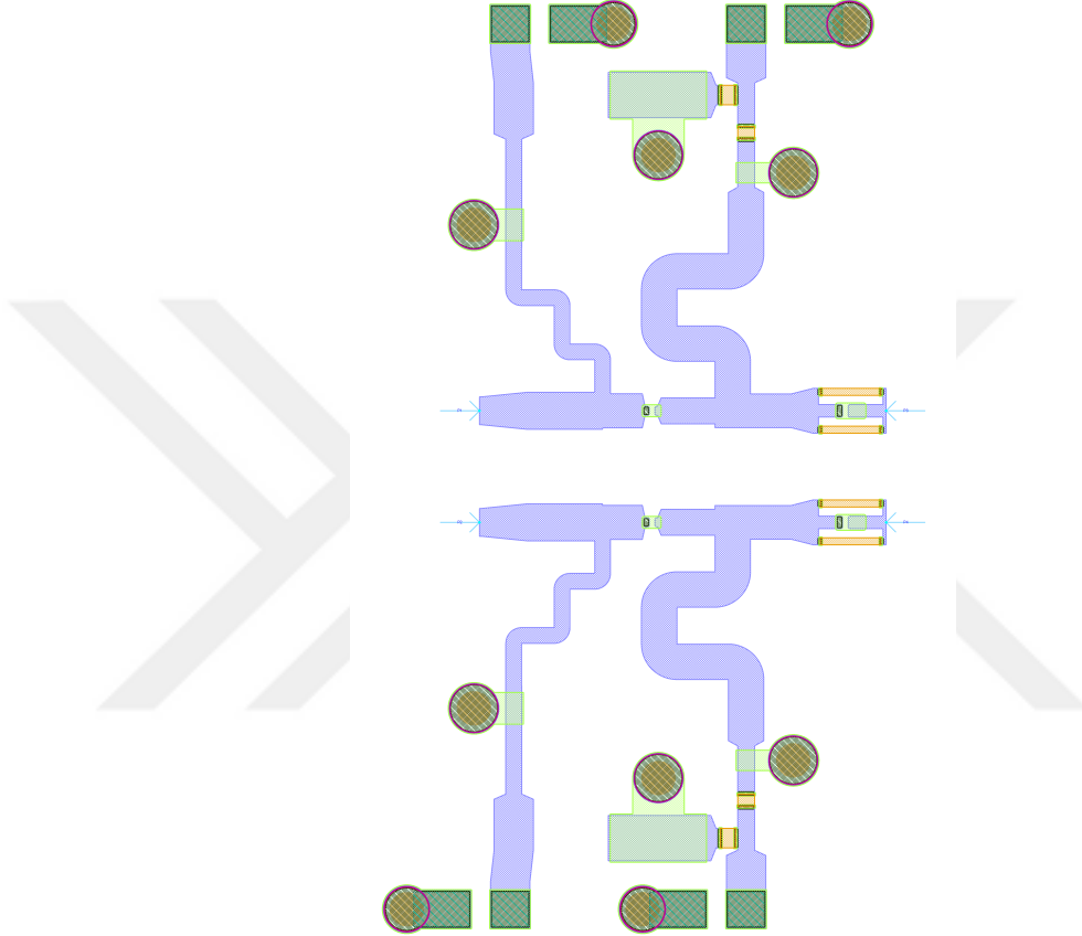
Figure 5.18: Completed layout of first interstage matching network.
