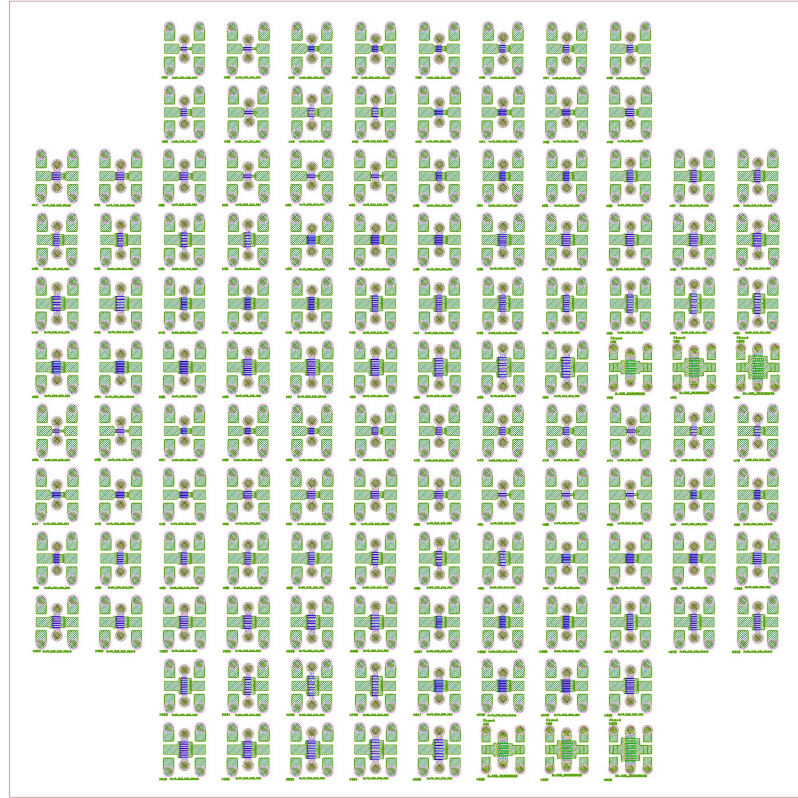
Figure 4.3: Photomask design for various HEMT structures.
