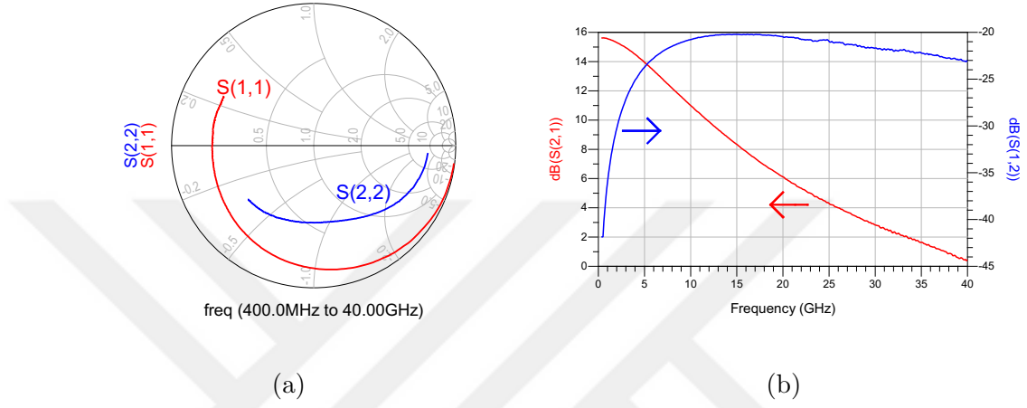
Figure 3.6: S-parameters of a 4 \times 75 \mu\text{m} HEMT; a) IRC ( S_{11} ) and ORC ( S_{22} ), b) Forward transmission ( S_{21} ) and reverse transmission ( S_{12} ).
