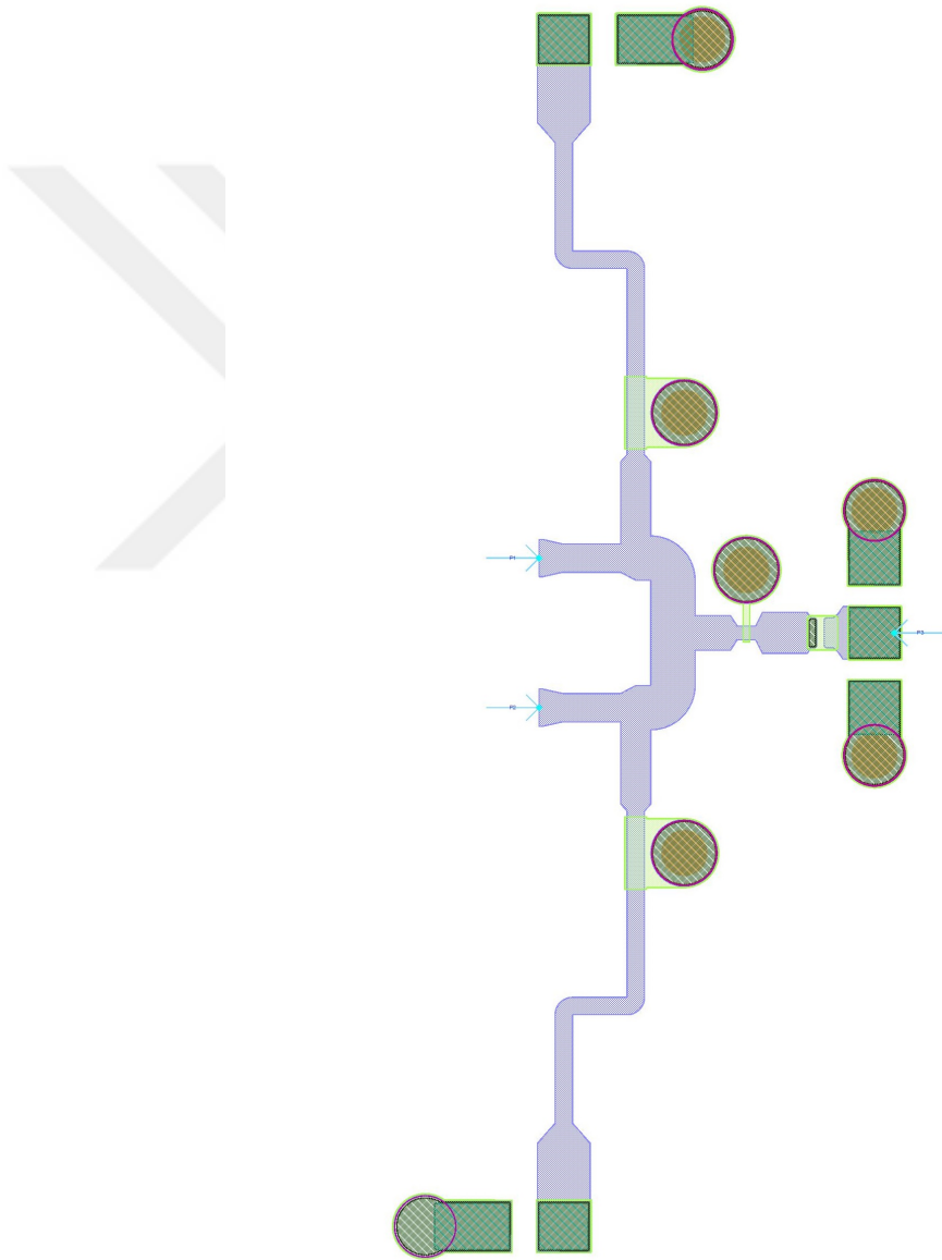
Figure 5.12: Completed layout of OMN.
