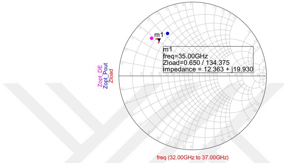
Figure 5.9: Load impedance shown to the transistors with the designed OMN from 32 GHz to 37 GHz (red), the optimum load impedance for maximum output power at 35 GHz (blue), the optimum load impedance for maximum drain efficiency at 35 GHz (magenta).
