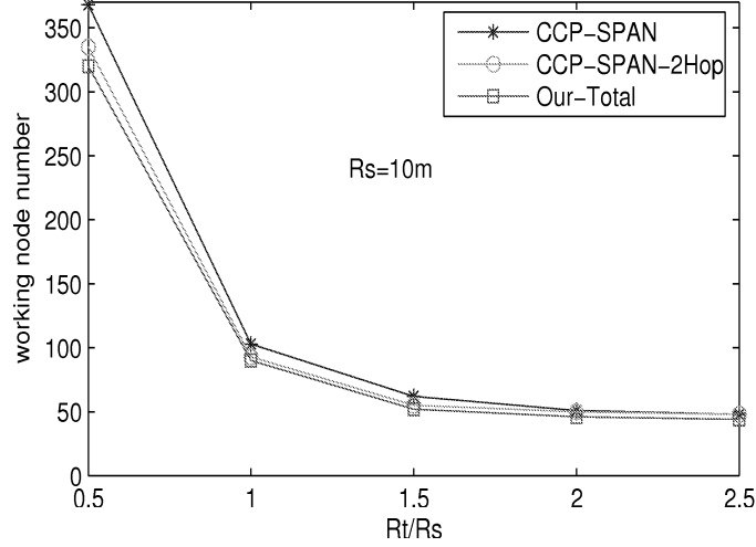
Figure 5.6: Working node count vs. R_t/R_s ratio.
