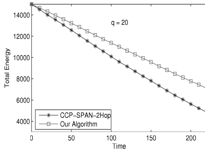
Figure 5.18: Total energy in nodes in a sample run when q = 20 .
