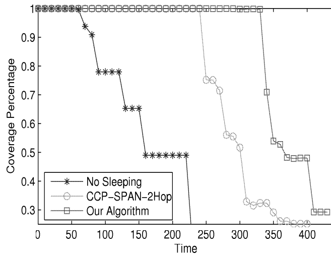
Figure 5.11: Coverage percentage in a sample run when R_t/R_s = 1 .
