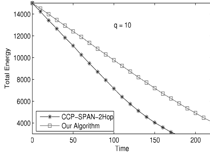
Figure 5.17: Total energy in nodes in a sample run when q = 10 .
