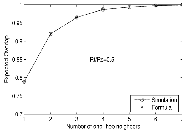
Figure 3.10: Expected overlap values from simulation and formula when R_t/R_s=0.5
