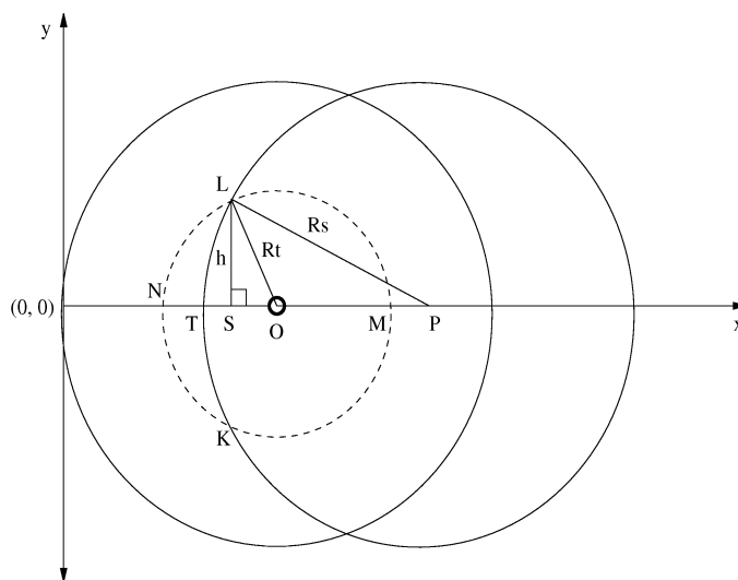
Figure 3.6: Height of the region projects on the left of center O.
