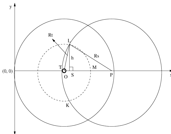
Figure 3.5: Height of the region projects on the right of center O.
