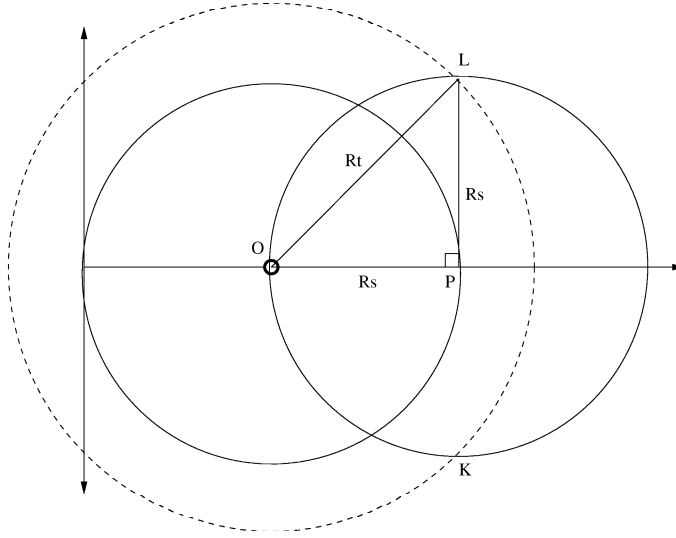
Figure 3.8: Border case when R_t > R_s .
