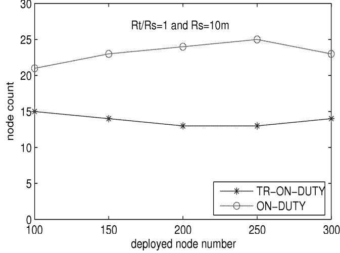
Figure 5.3: TR-ON-DUTY and ON-DUTY node count vs. Deployed node Count. R_s=10m and R_t=10m .
