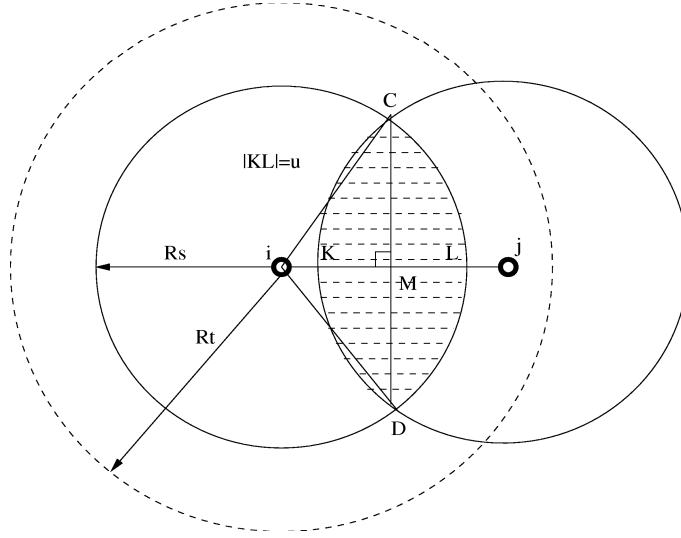
Figure 3.2: Overlap of node i 's sensing area by a neighbor j .
