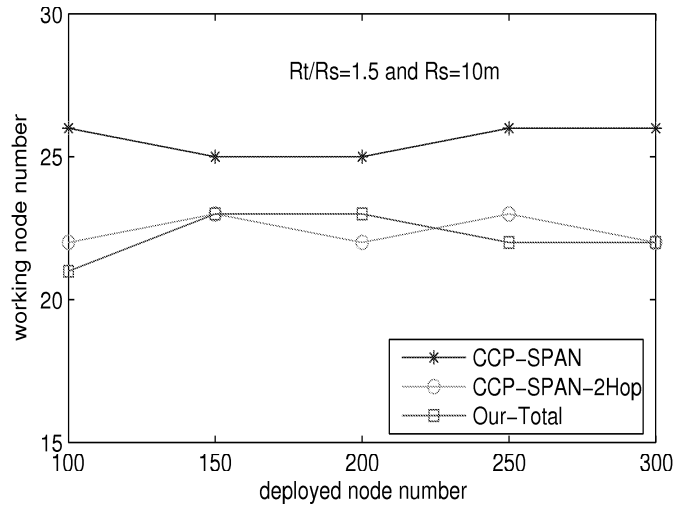
Figure 5.2: Working node count vs. Deployed node Count. R_s=10m and R_t=15m .
