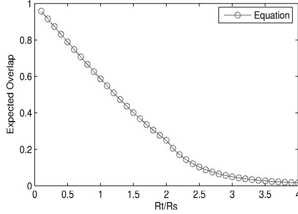
Figure 3.3: Expected overlap of a node's sensing area with different R_t/R_s ratios.
