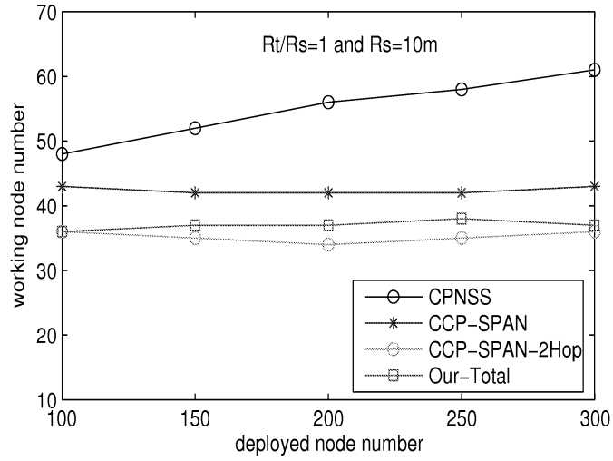
Figure 5.1: Working node count vs. Deployed node Count. R_s=10m and R_t=10m .
