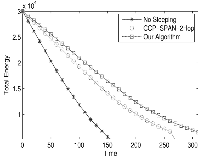
Figure 5.10: Total energy in nodes in a sample run when R_t/R_s = 0.5 .
