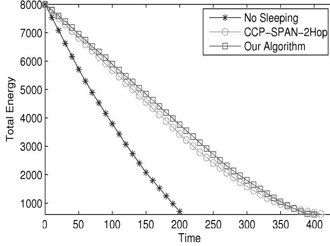
Figure 5.16: Total energy in nodes in a sample run when R_t/R_s = 1.5 .
