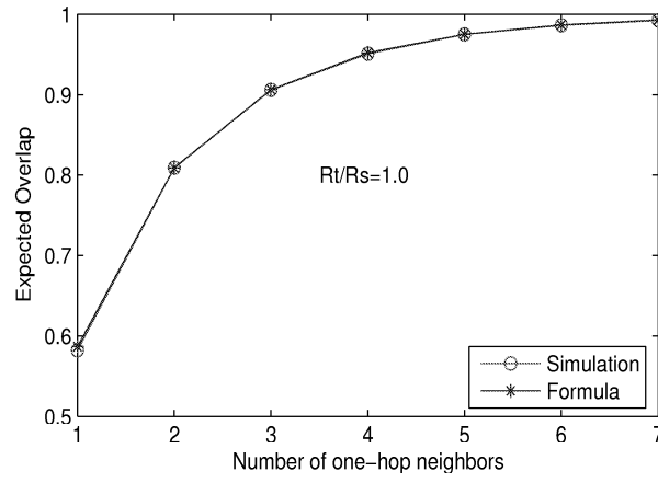
Figure 3.9: Expected overlap values from simulation and formula when R_t/R_s=1
