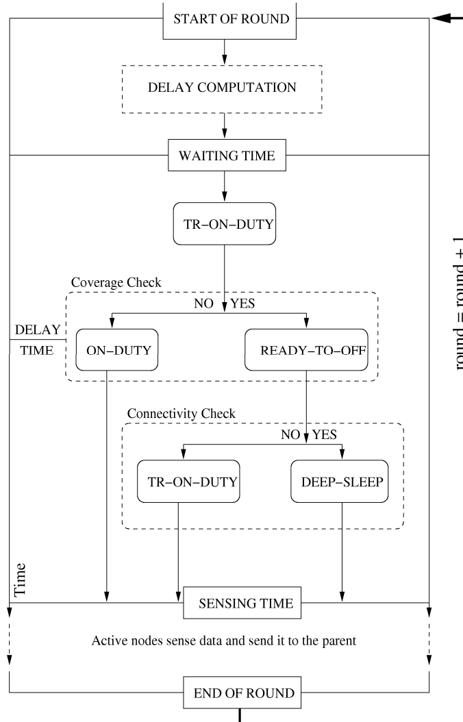
Figure 4.4: The overall mechanism to decide which mode a sensor node will be in each round.
