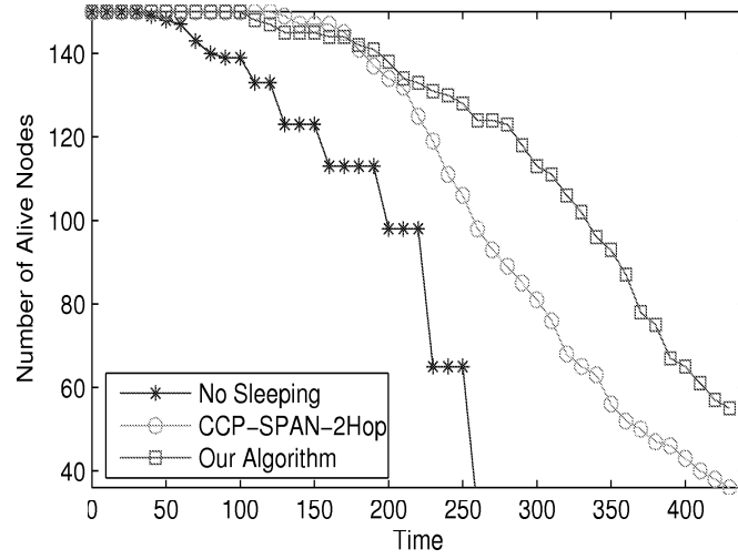
Figure 5.12: Number of still alive nodes in a sample run when R_t/R_s = 1 .
