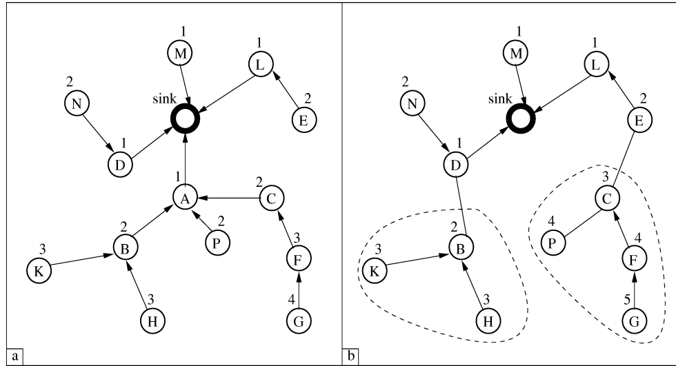
Figure 4.7: (a) The node A informs its neighbors about its death in the next round. (b) Tier numbers of children do not change (left enclosed region). No TierUpdate message is required. Tier numbers of children change (right enclosed region). Other children in the levels below are informed, and they update their tier numbers accordingly.
