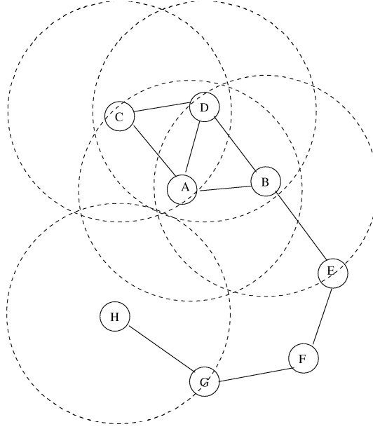
Figure 3.1: Node A's sensing area is totally covered by not only the one-hop nodes of A but also another node H.
