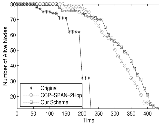
Figure 5.15: Number of still alive nodes in a sample run when R_t/R_s = 1.5 .
