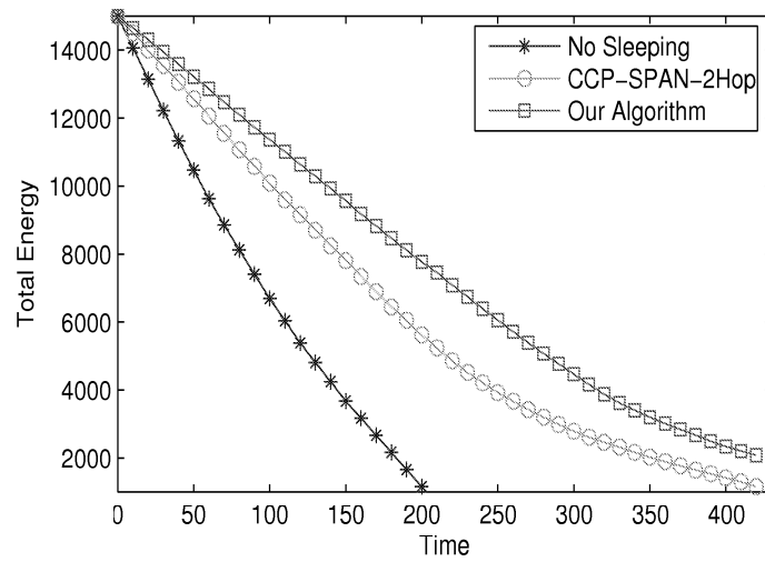
Figure 5.13: Total energy in nodes in a sample run when R_t/R_s = 1 .
