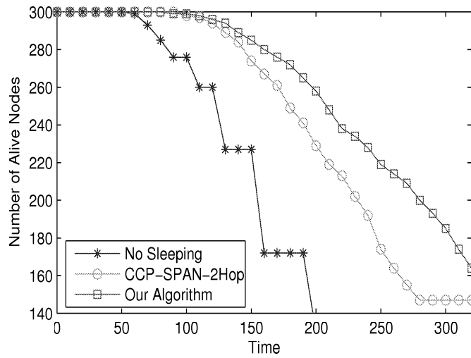
Figure 5.9: Number of still alive nodes in a sample run when R_t/R_s = 0.5 .
