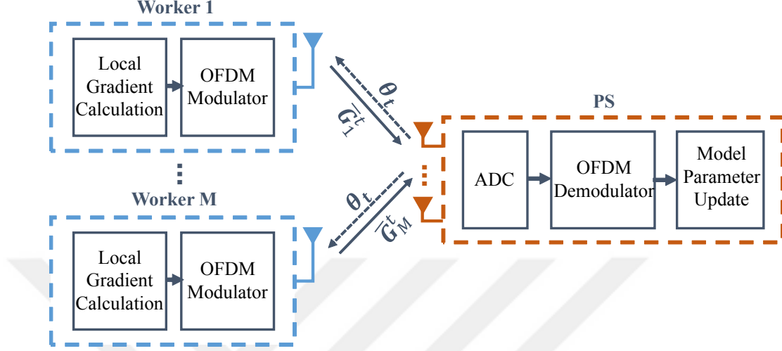
Figure 5.1: System model for distributed machine learning at the wireless edge.
