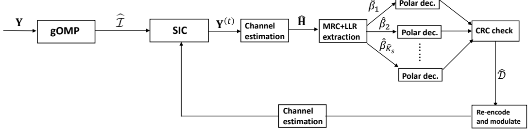
Figure 4.2: Decoding process of the proposed scheme (SNOP-URA) in a slot.
