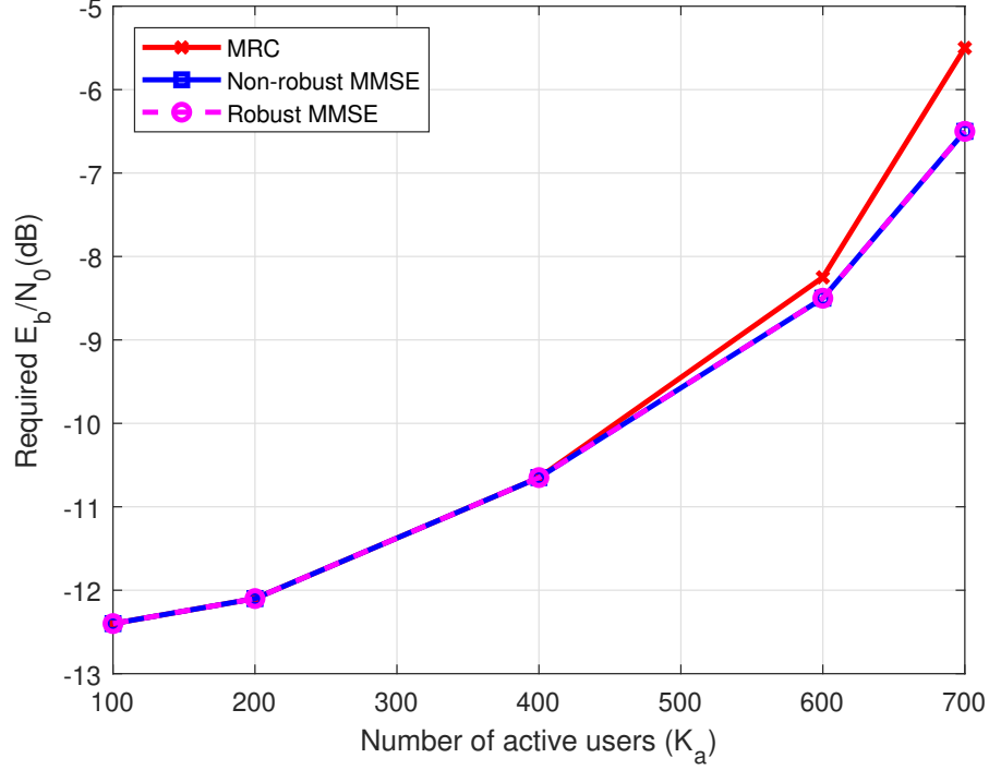
Figure 5.6: Required E_b/N_0 versus the number of active users with different user symbol estimators for multiplicative HWIs.
