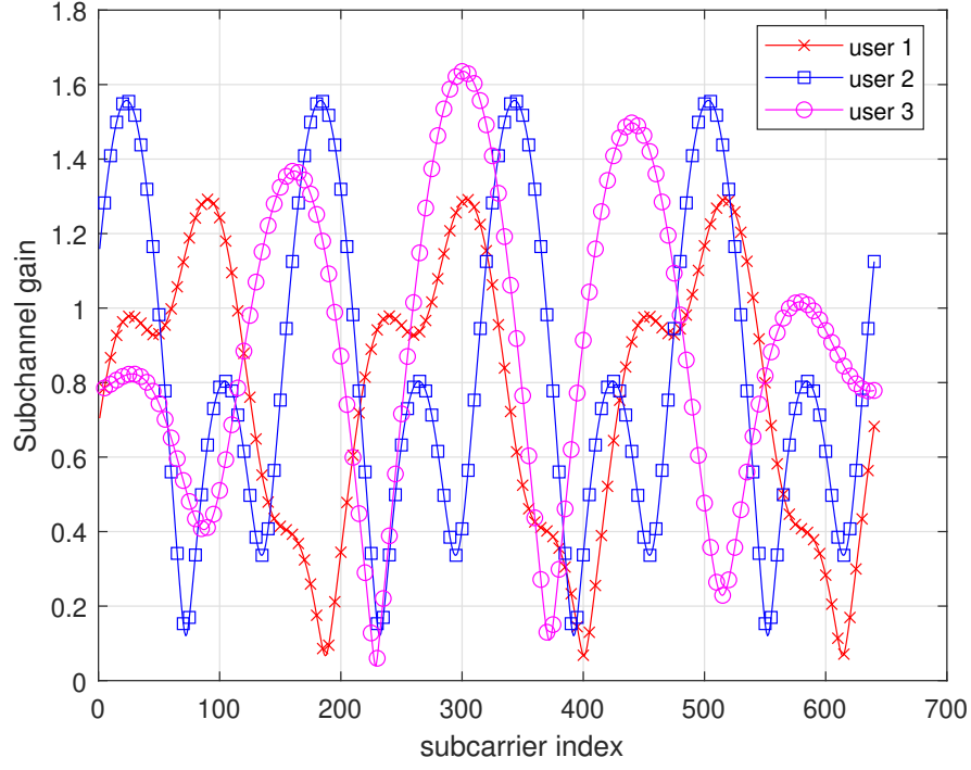
Figure 3.2: Frequency domain subchannel gain magnitudes of the multipath channels of three different users with 3 time-domain channel taps.
