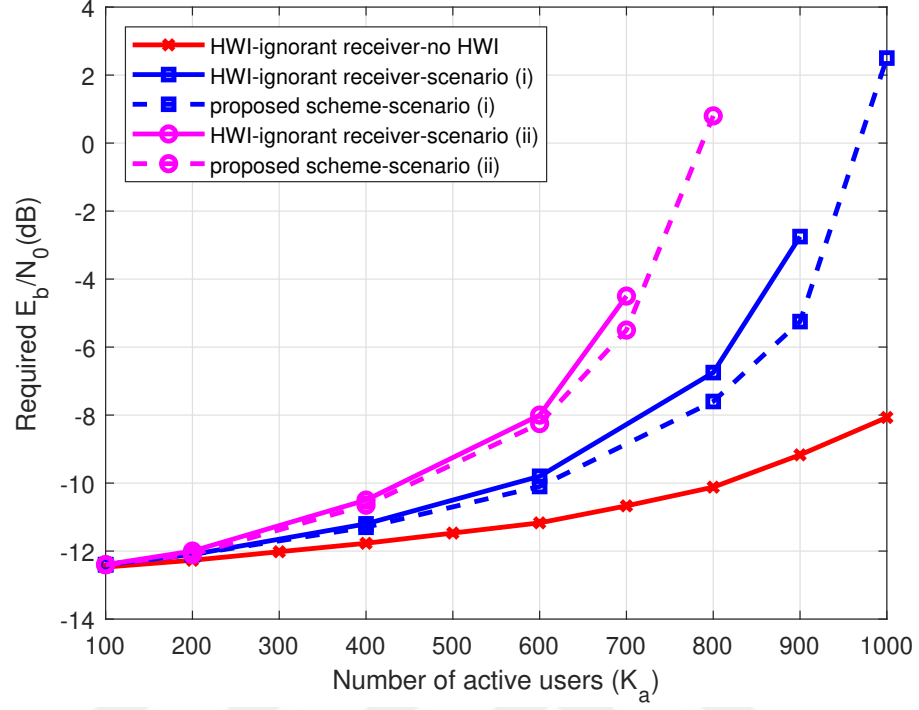
Figure 5.4: Required E_b/N_0 versus the number of active users with different multiplicative HWI scenarios and P_e \leq 0.05 .
