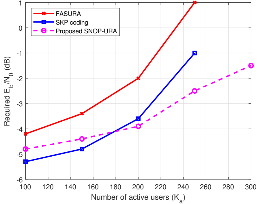
Figure 4.9: Required E_b/N_0 versus the number of active users of the proposed scheme and the state-of-the-art schemes in the literature for M = 8 and \epsilon = 0.1 .
