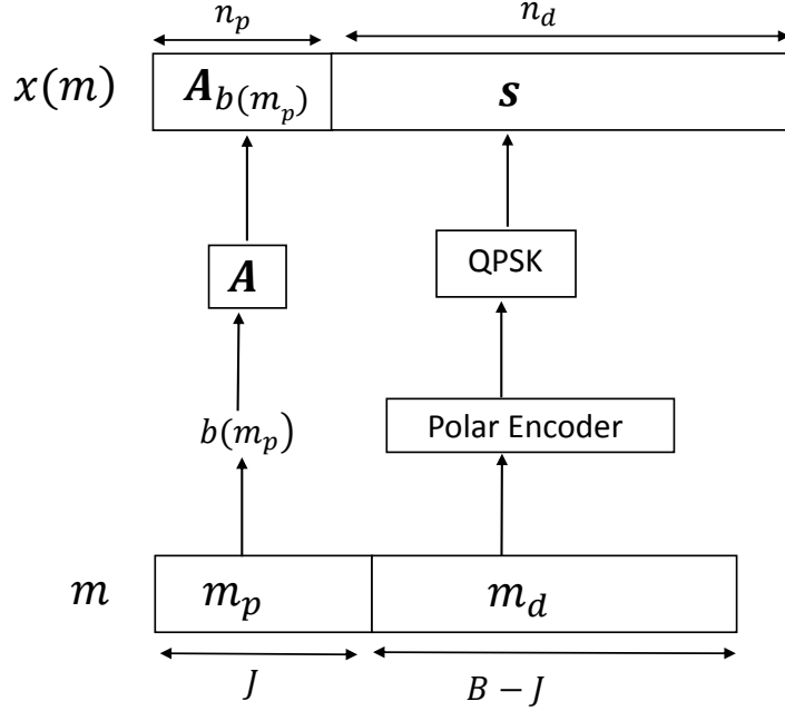
Figure 4.1: Encoding process of the proposed scheme for a user.
