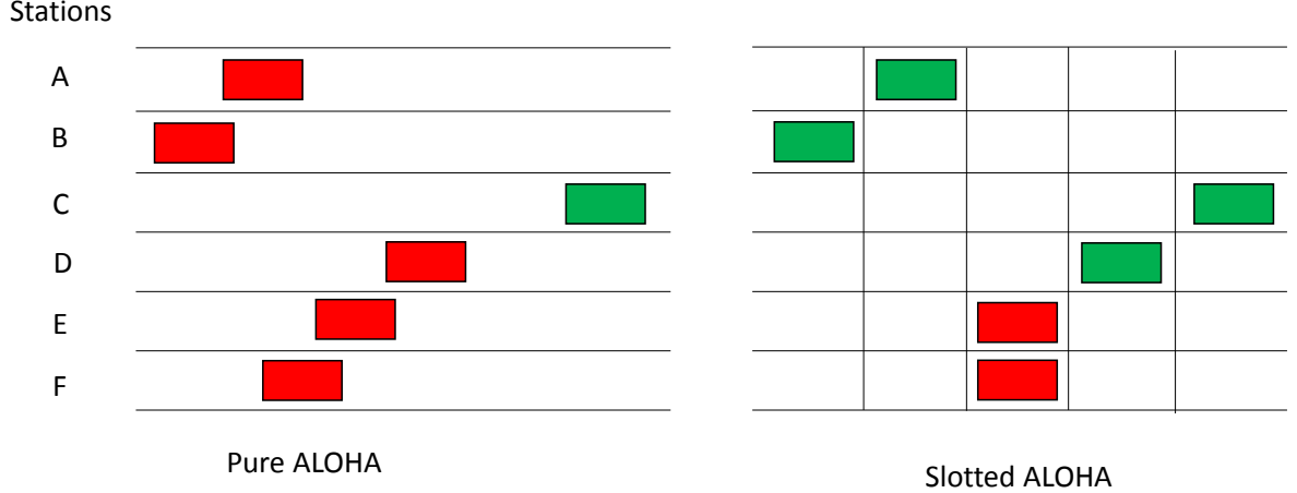
Figure 2.1: An illustration of pure and slotted ALOHA. Red boxes show the collided packets and green boxes are the successfully transmitted ones.
