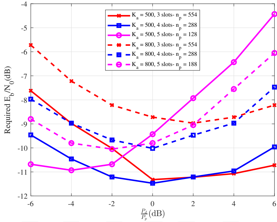
Figure 4.12: Required \frac{E_b}{N_0} with respect to power distribution of data and pilot parts for different pilot lengths.
