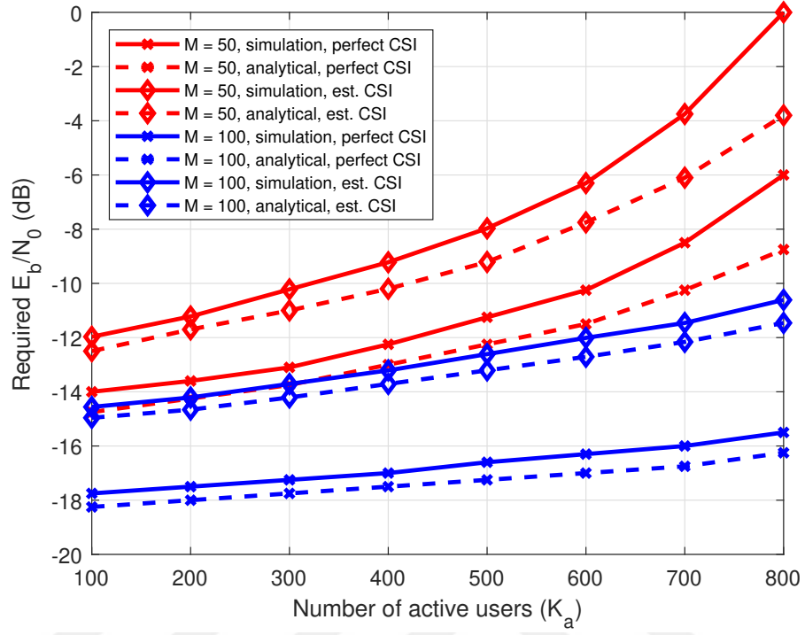
Figure 4.10: Required \frac{E_b}{N_0} versus the number of active users for different number of BS antennas.
