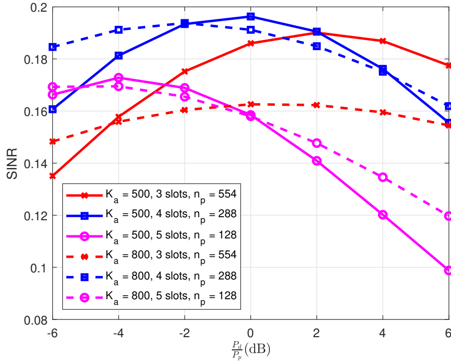
Figure 4.11: SINR values for different sets of parameters with respect to power distribution between pilot and data parts.
