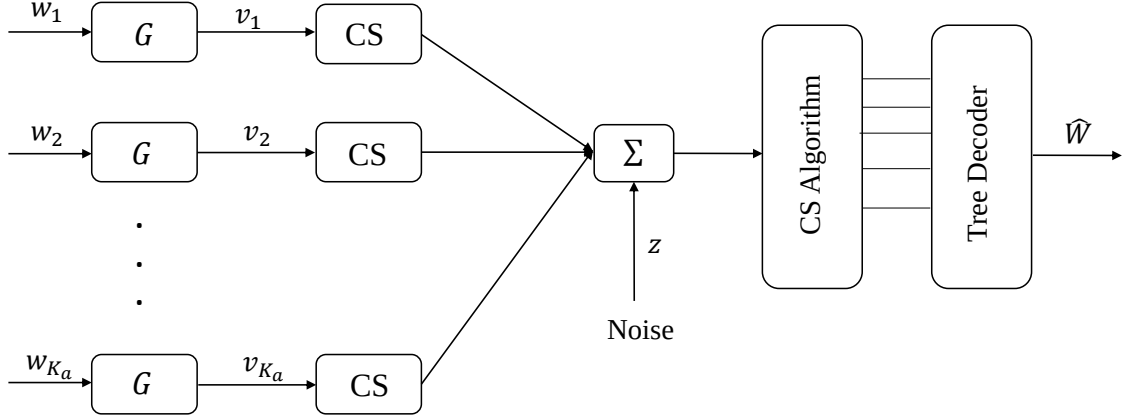
Figure 2.5: Encoding-decoding structure in coded compressed sensing.
