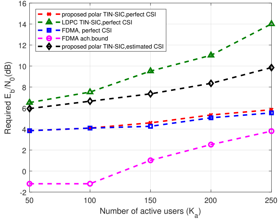
Figure 3.5: Minimum required E_b/N_0 for \epsilon \leq 0.1 , n = 30000 , B = 100 with different schemes for scenario (ii).
