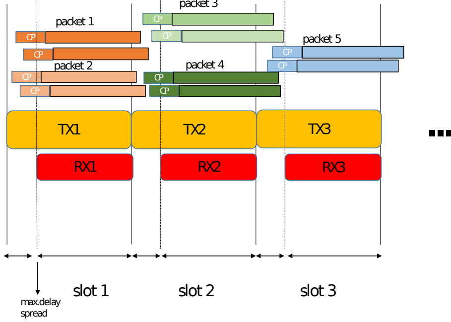
Figure 3.1: Transmission system model for two-tap multipath fading with a cyclic prefix longer than maximum delay spread.
