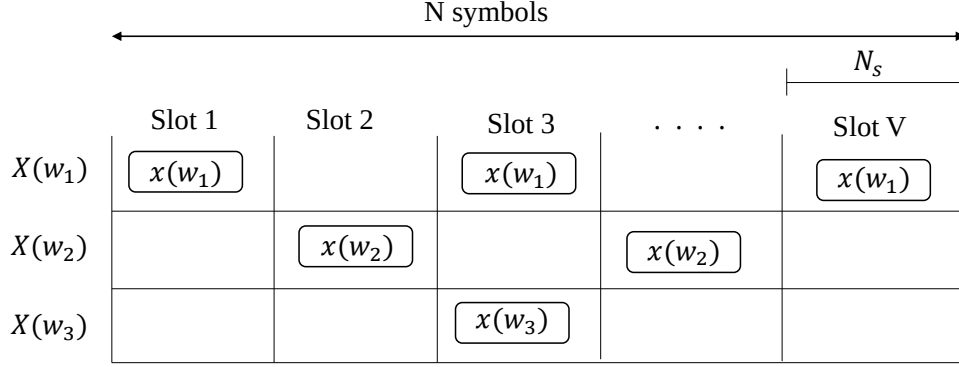
Figure 2.4: The slotted transmission structure in [30] based on T -fold IRSA.
