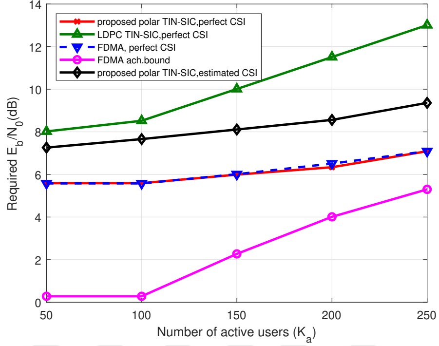
Figure 3.4: Minimum required E_b/N_0 for \epsilon \leq 0.1 , n = 30000 , B = 100 with different schemes for scenario (i).
