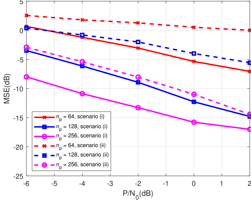
Figure 3.3: The MSE performance of the channel estimation algorithm for different pilot lengths.
