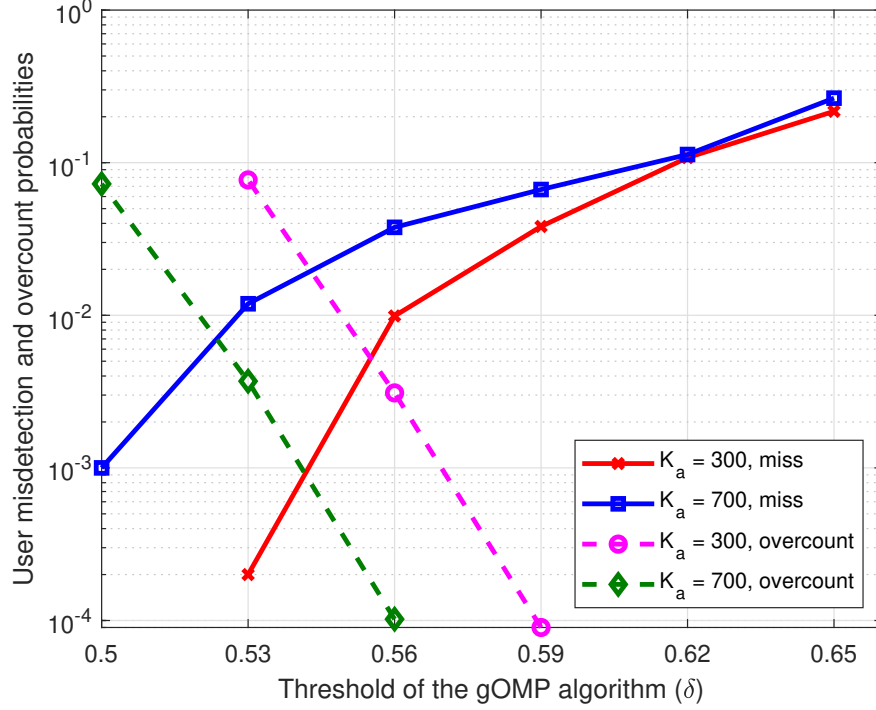
Figure 4.5: Misdetection and overcount probabilities of gOMP with respect to \delta for K_a = 300, 700 .
