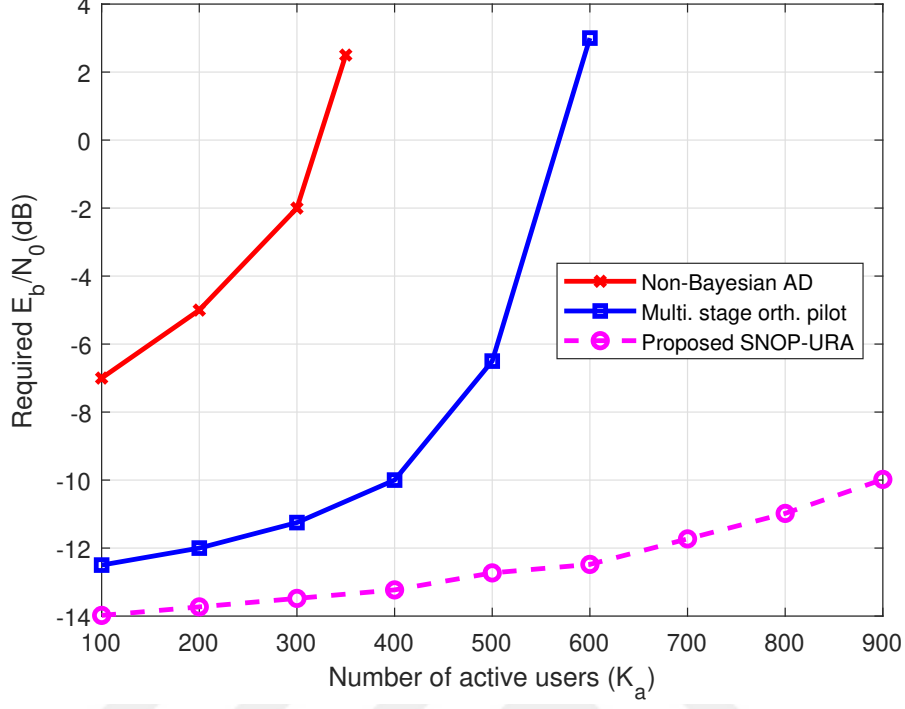
Figure 4.7: Required E_b/N_0 versus the number of active users for the short block-length regime ( L \approx 200 ) for \epsilon = 0.05 .
