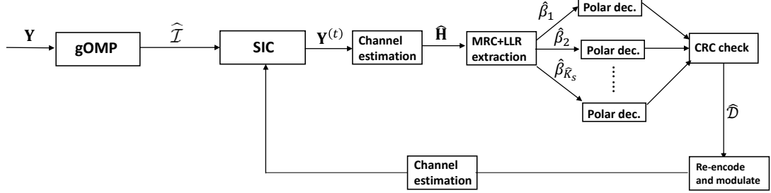
Figure 5.2: Decoding procedure of the proposed scheme in each slot.
