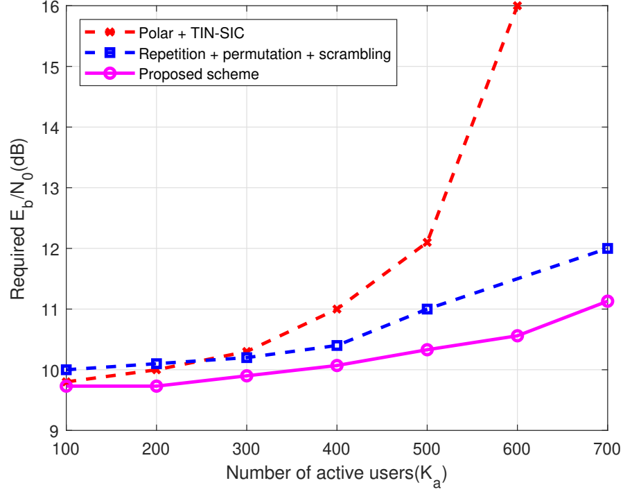
Figure 6.2: Required E_b/N_0 versus number of active users for fading MAC.
