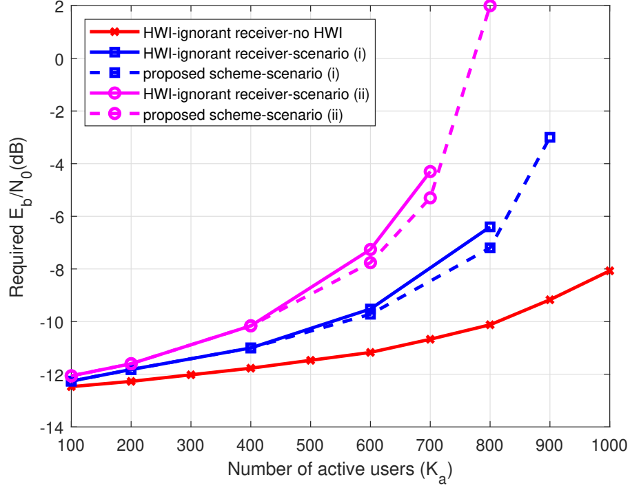
Figure 5.3: Required E_b/N_0 versus number of active users for different additive HWI scenarios and P_e \leq 0.05 .
