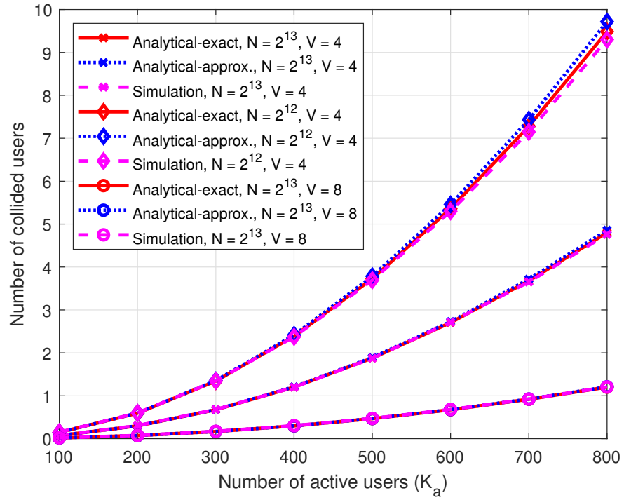
Figure 4.13: Average number of users in a collision with respect to number of active users for different number of pilot sequences and number of slots.
