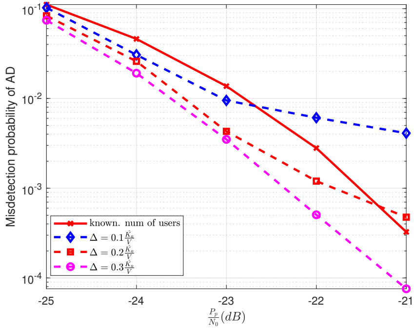
Figure 4.4: Misdetction probability of activity detection with different \Delta values for K_a = 300 .
