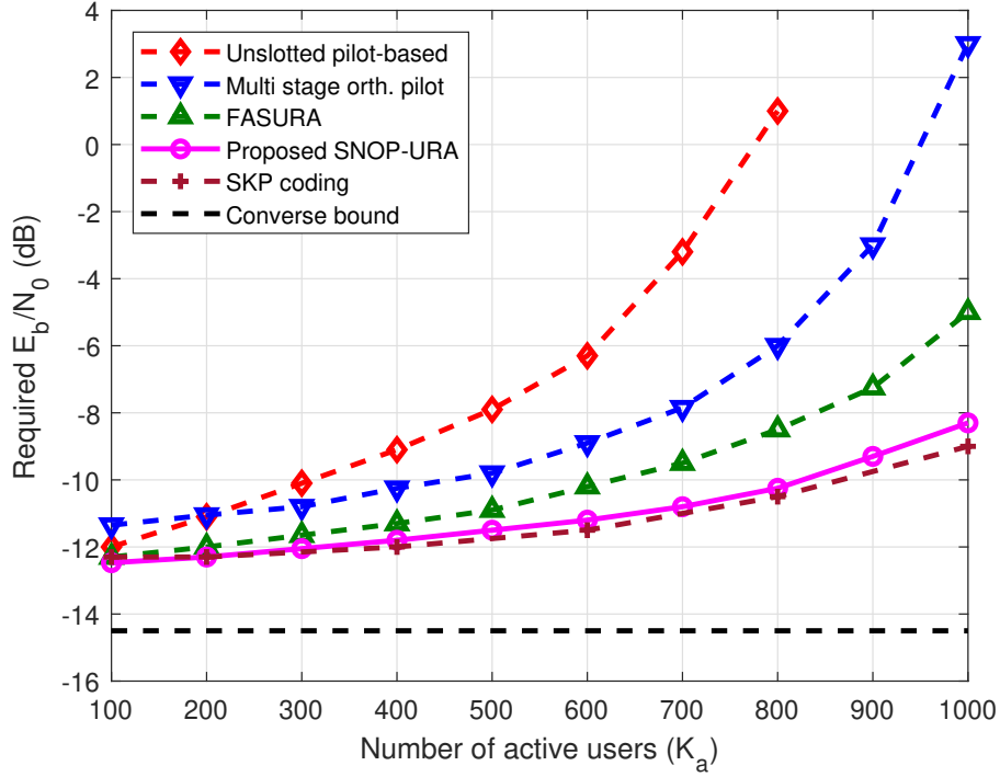
Figure 4.6: Required E_b/N_0 versus number of active users of the proposed scheme and the schemes in the literature for M = 50 and \epsilon = 0.05 .
