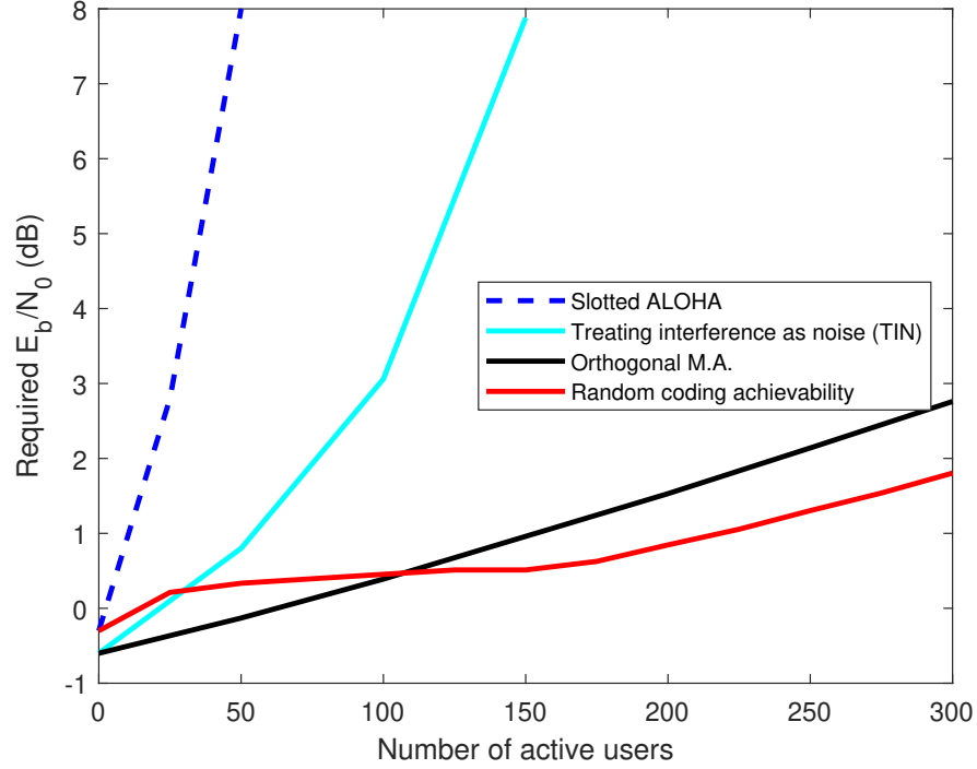
Figure 2.3: Required E_b/N_0 for versus the number of active users.
