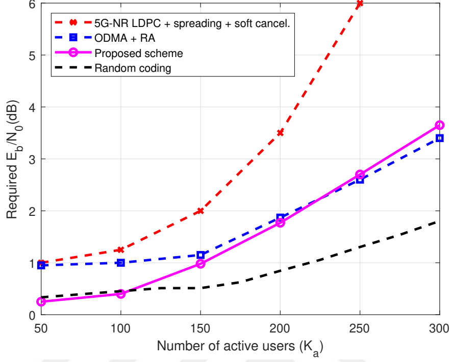
Figure 6.3: Required E_b/N_0 versus number of active users for GMAC.
