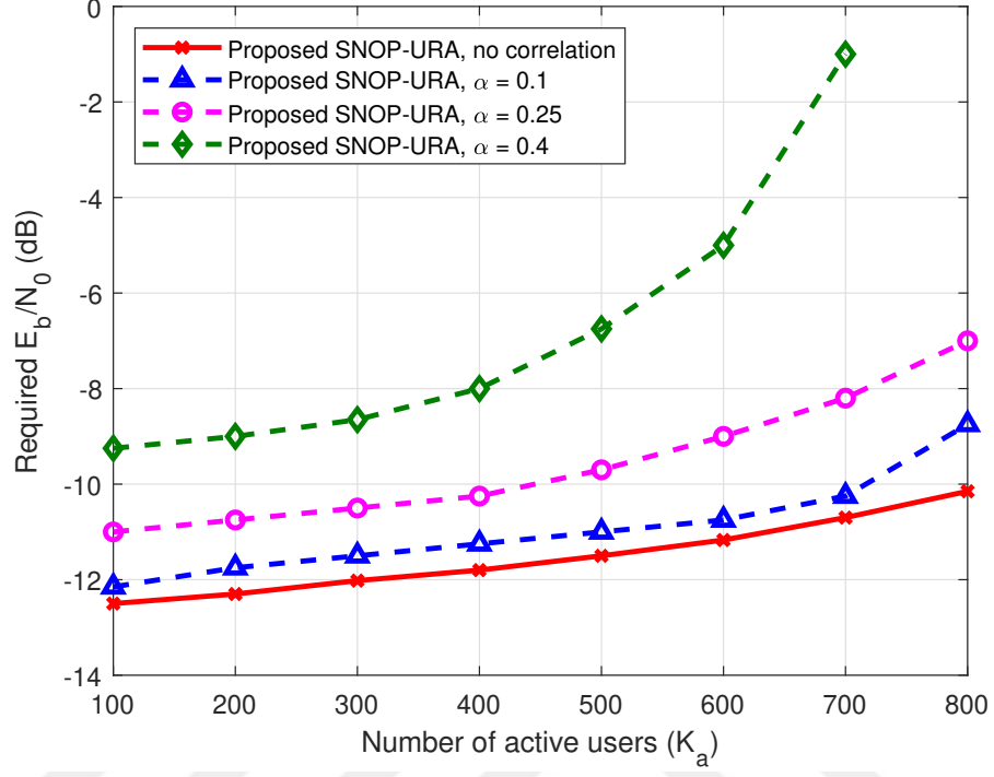
Figure 4.8: Required E_b/N_0 versus number of active users for different correlation levels among the antennas for \epsilon = 0.05 .
