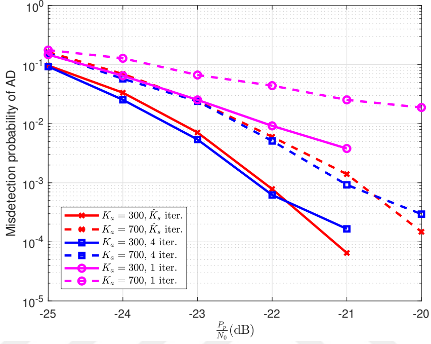
Figure 4.3: Misdetction probability of gOMP for different number of iterations for K_a = 300, 700 .
