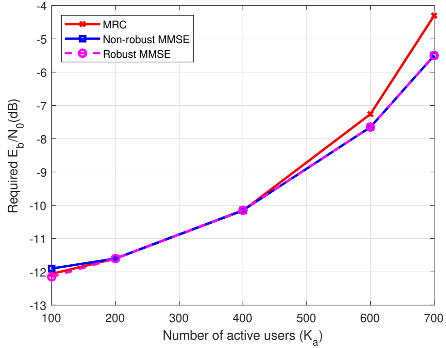
Figure 5.5: Required E_b/N_0 versus the number of active users with different user symbol estimators for additive HWIs.
