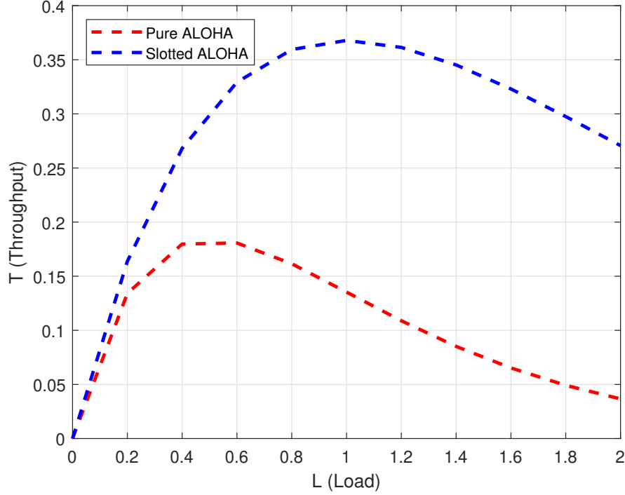
Figure 2.2: Throughput comparison of pure and slotted ALOHA.
