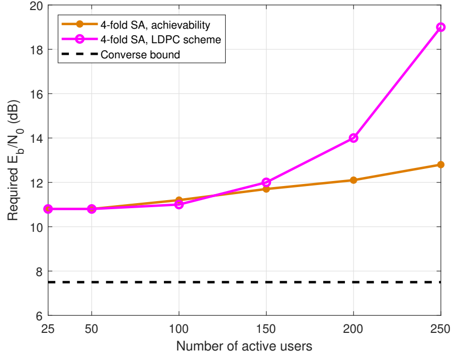
Figure 2.7: Required E_b/N_0 versus number of active users of the information theoretic limits for the fading case and the practical scheme in [49].
