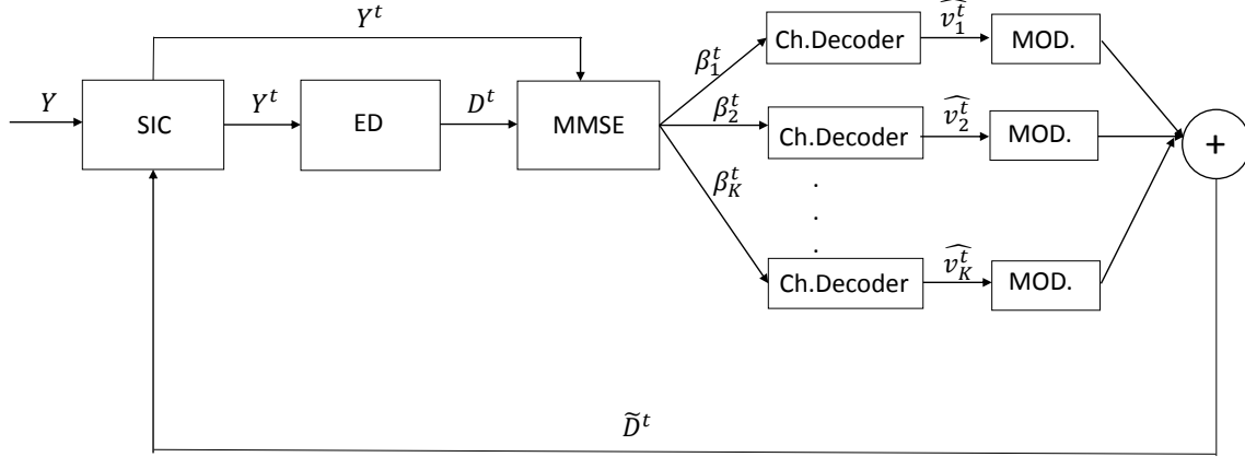
Figure 2.6: A typical decoding structure in random spreading.
